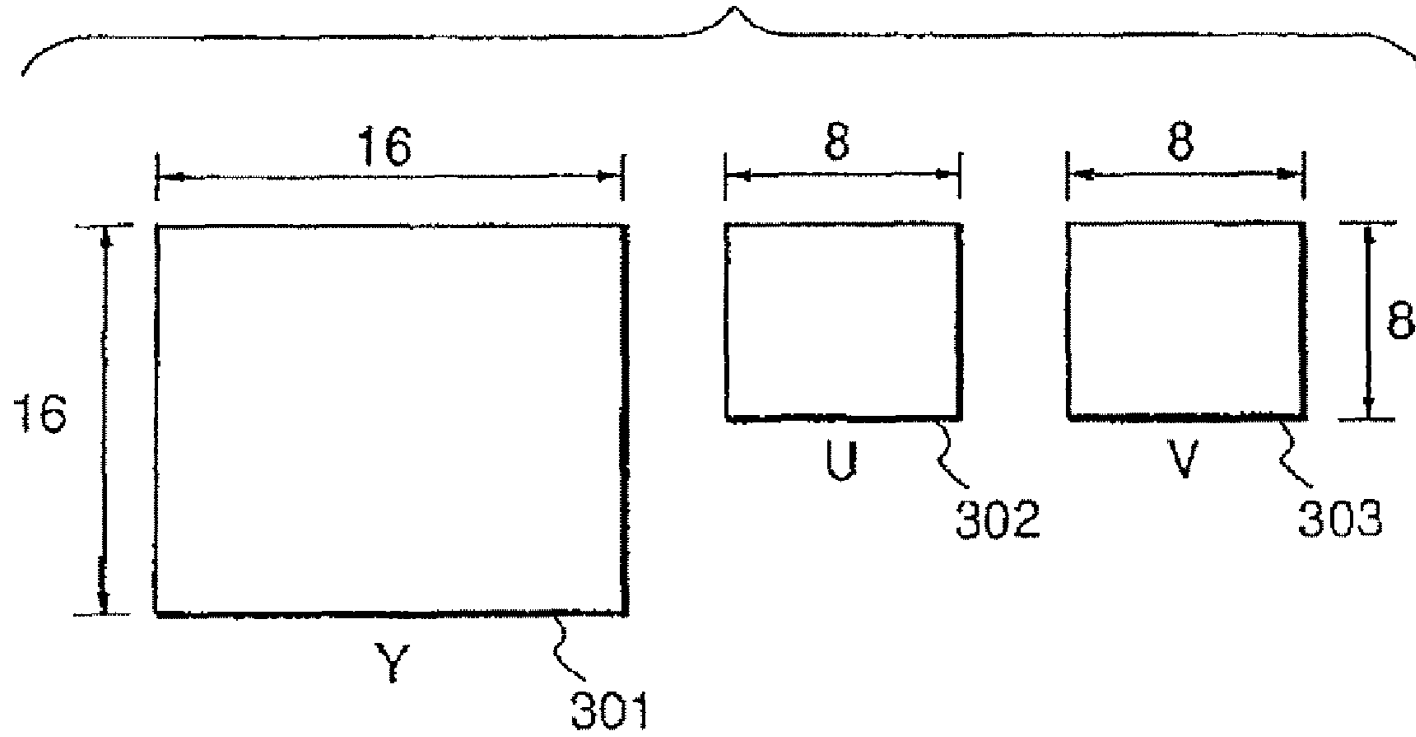
FIG. 3 (PRIOR ART)
