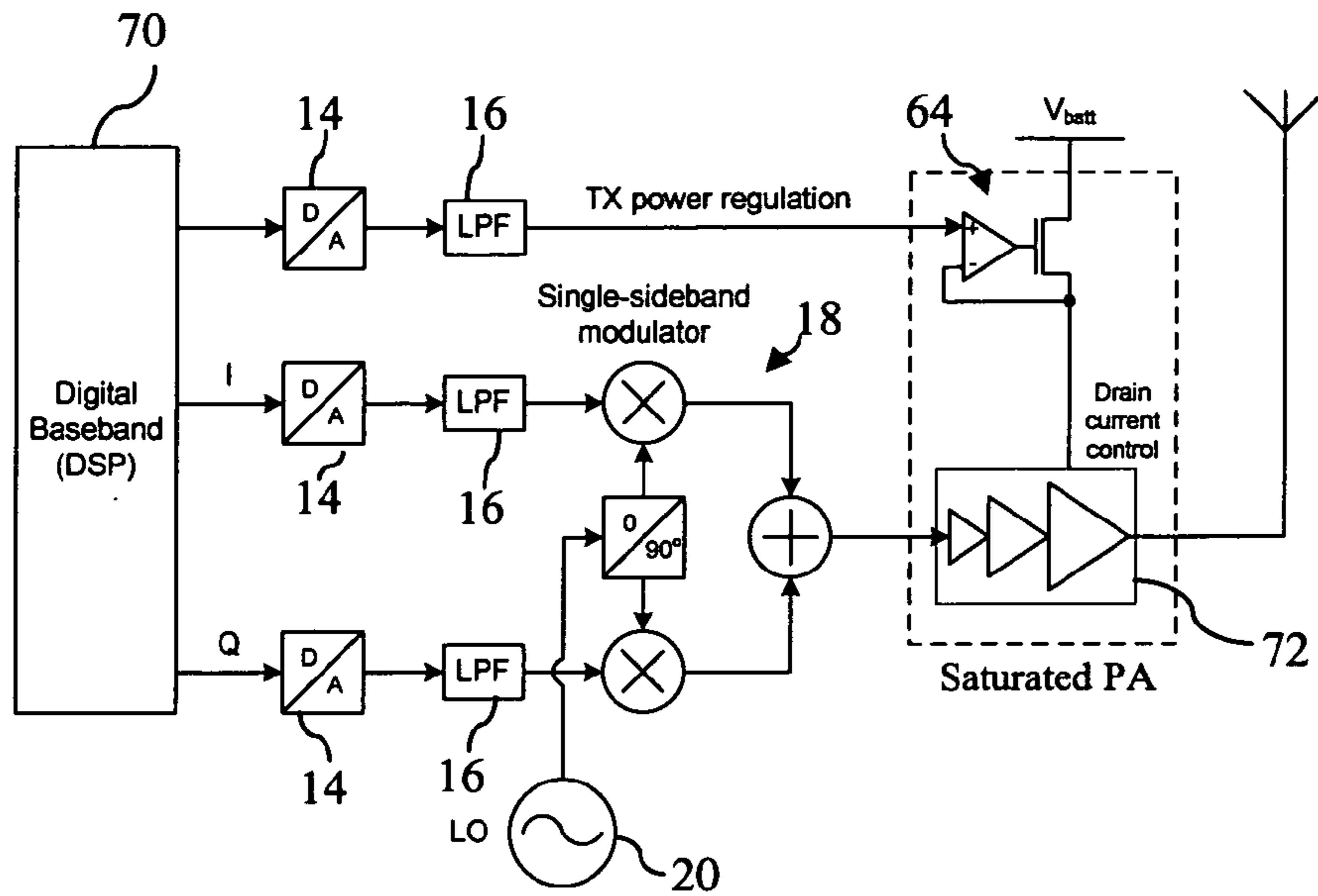
Fig. 7 (Prior Art)
