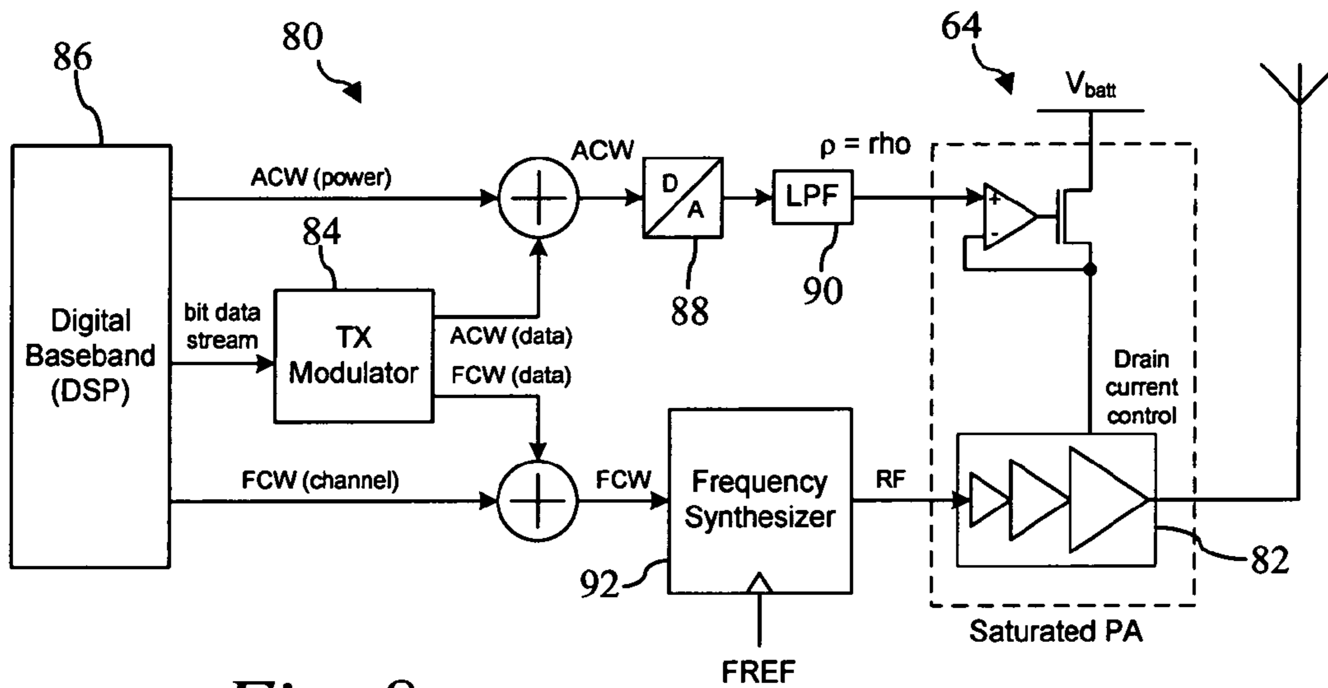
Fig. 8 (Prior Art)
