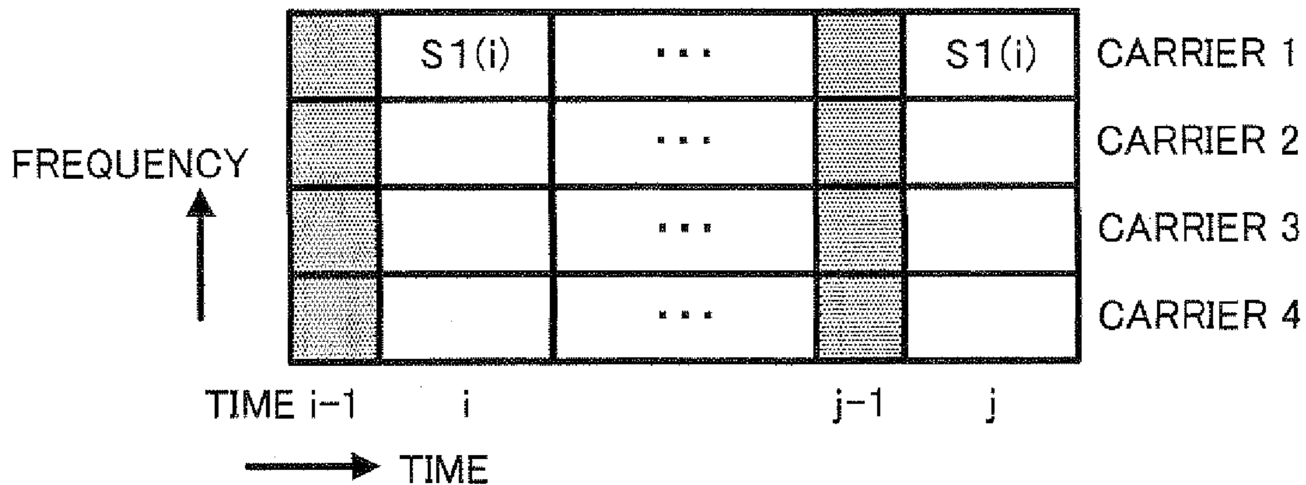
MODULATED SIGNAL A FRAME CONFIGURATION
