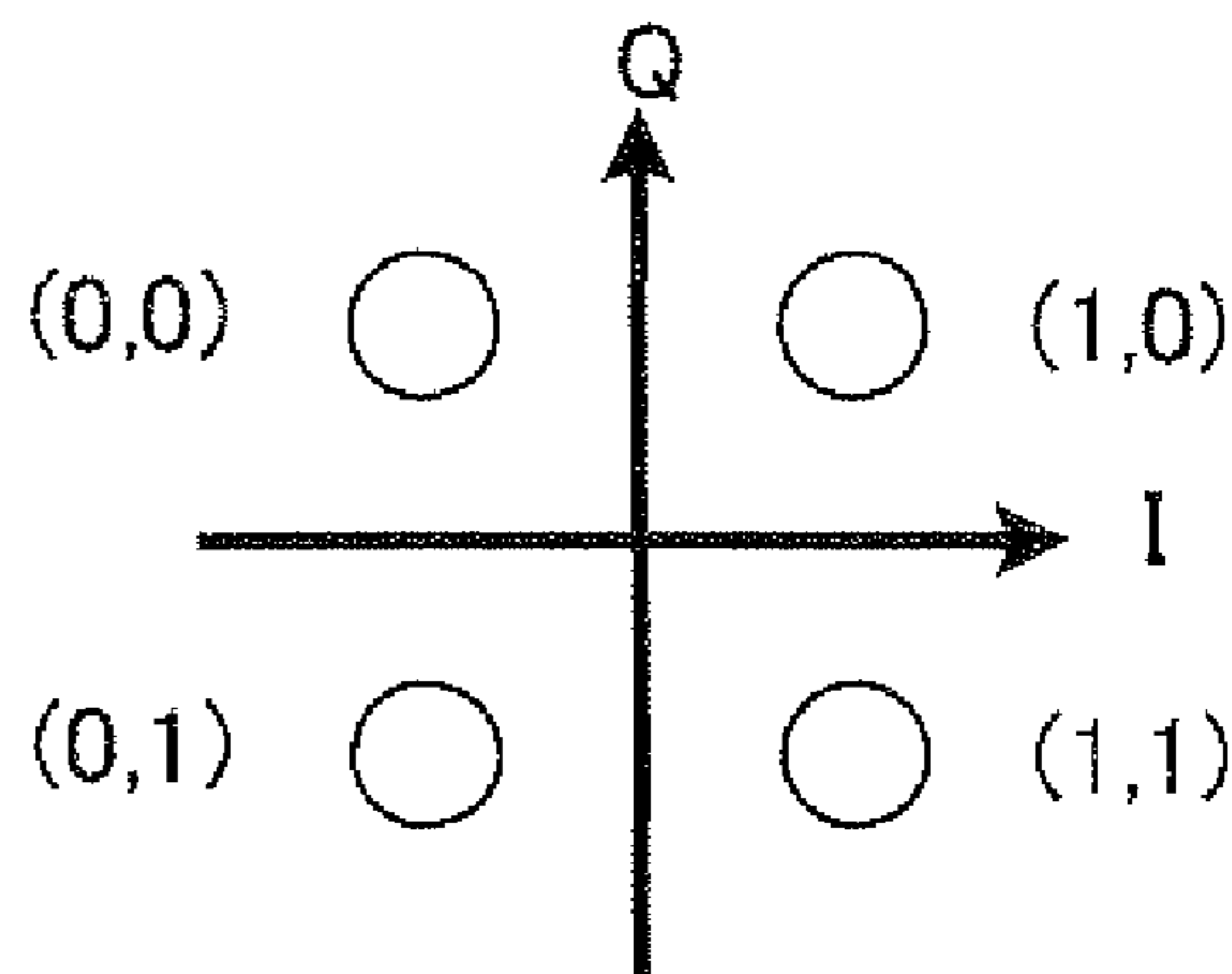
S1(i)' SIGNAL POINT ARRANGEMENT
