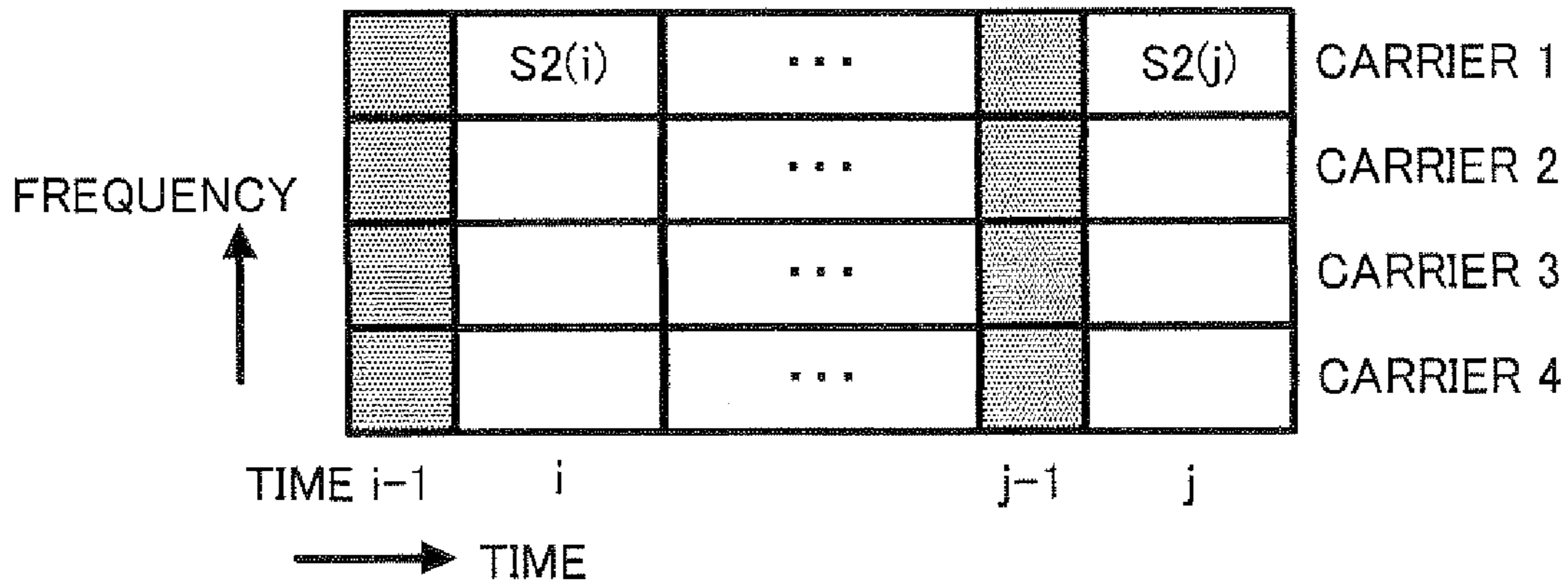
MODULATED SIGNAL B FRAME CONFIGURATION
