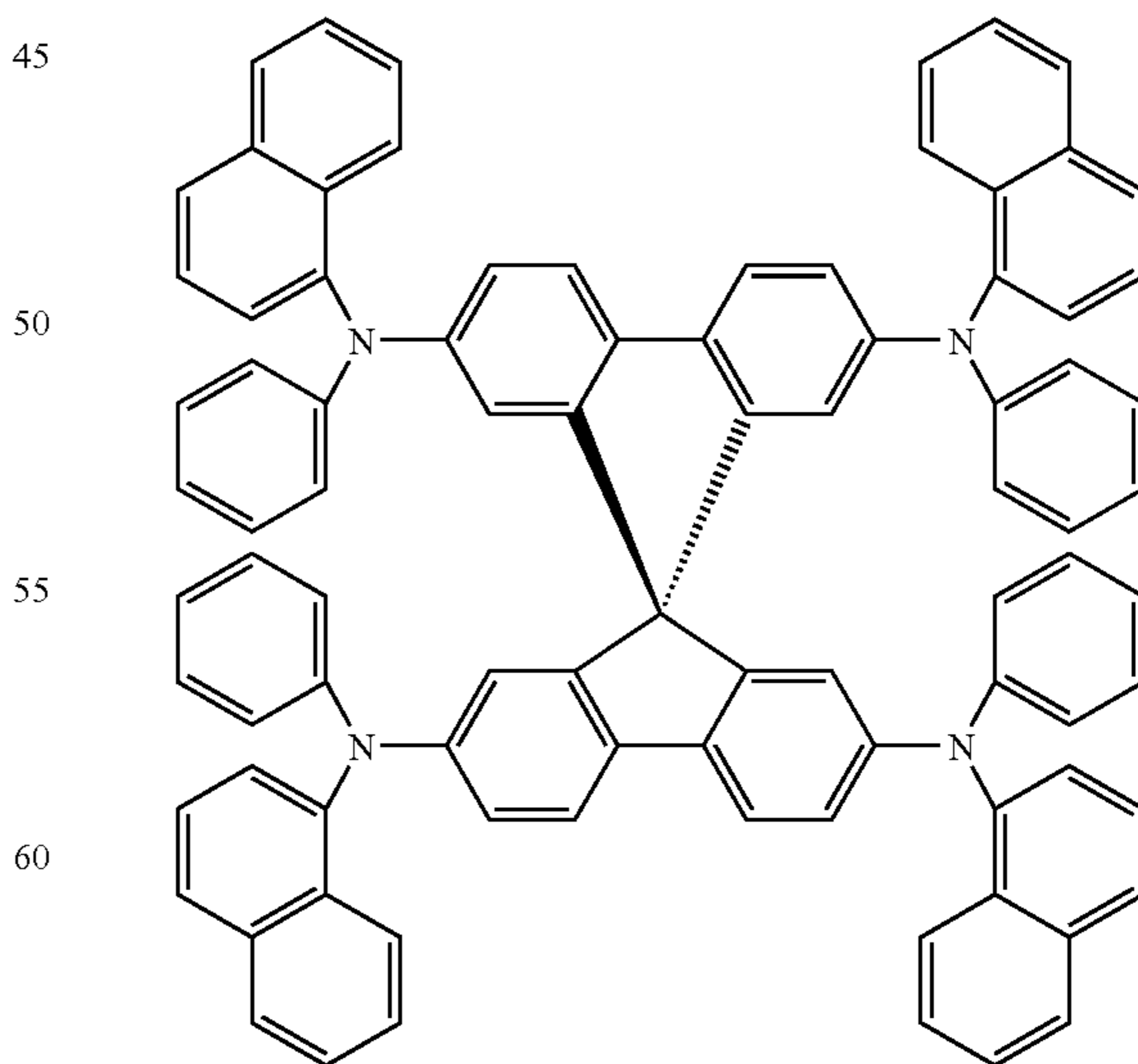
spiro-NPD
