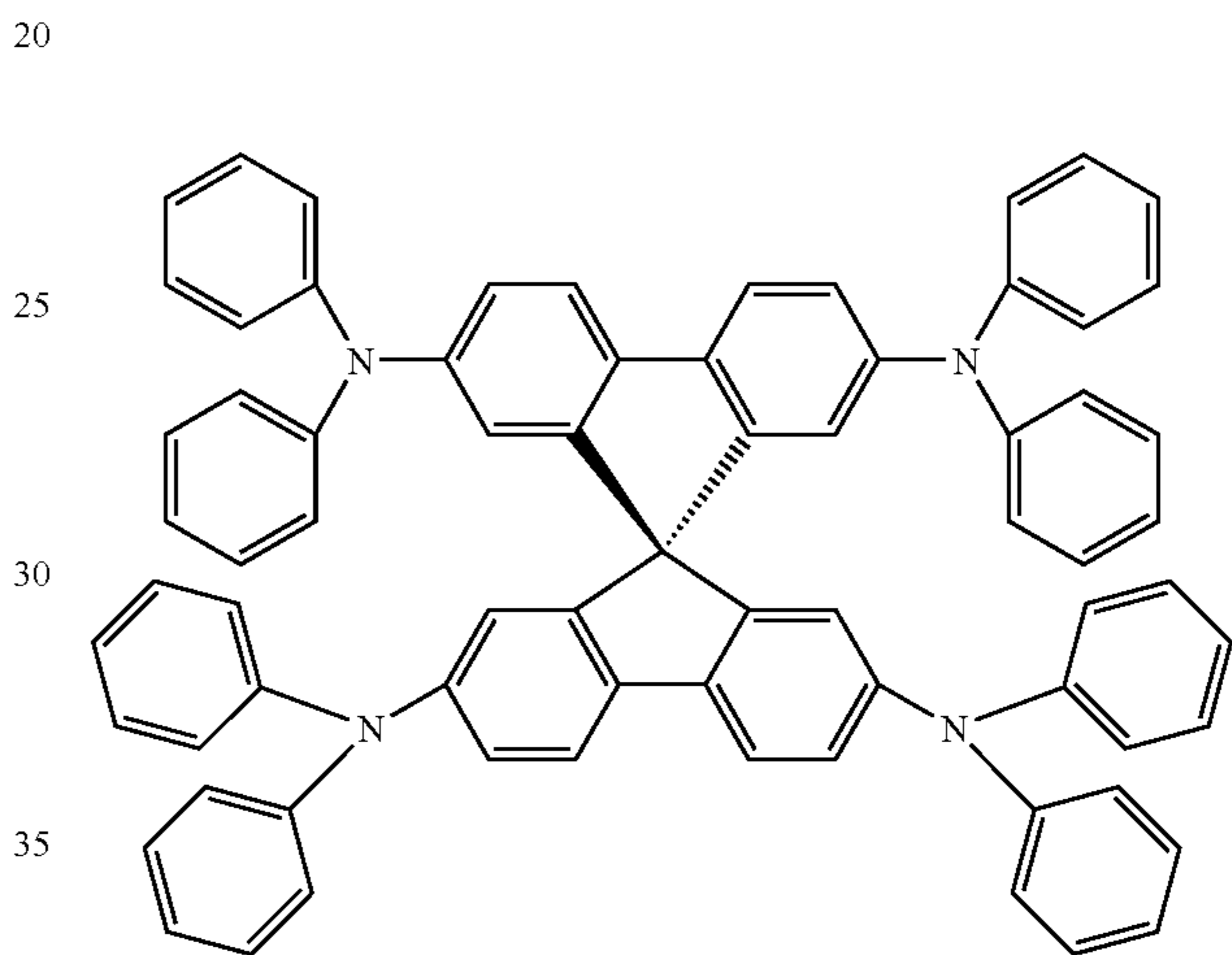
spiro-TPD
