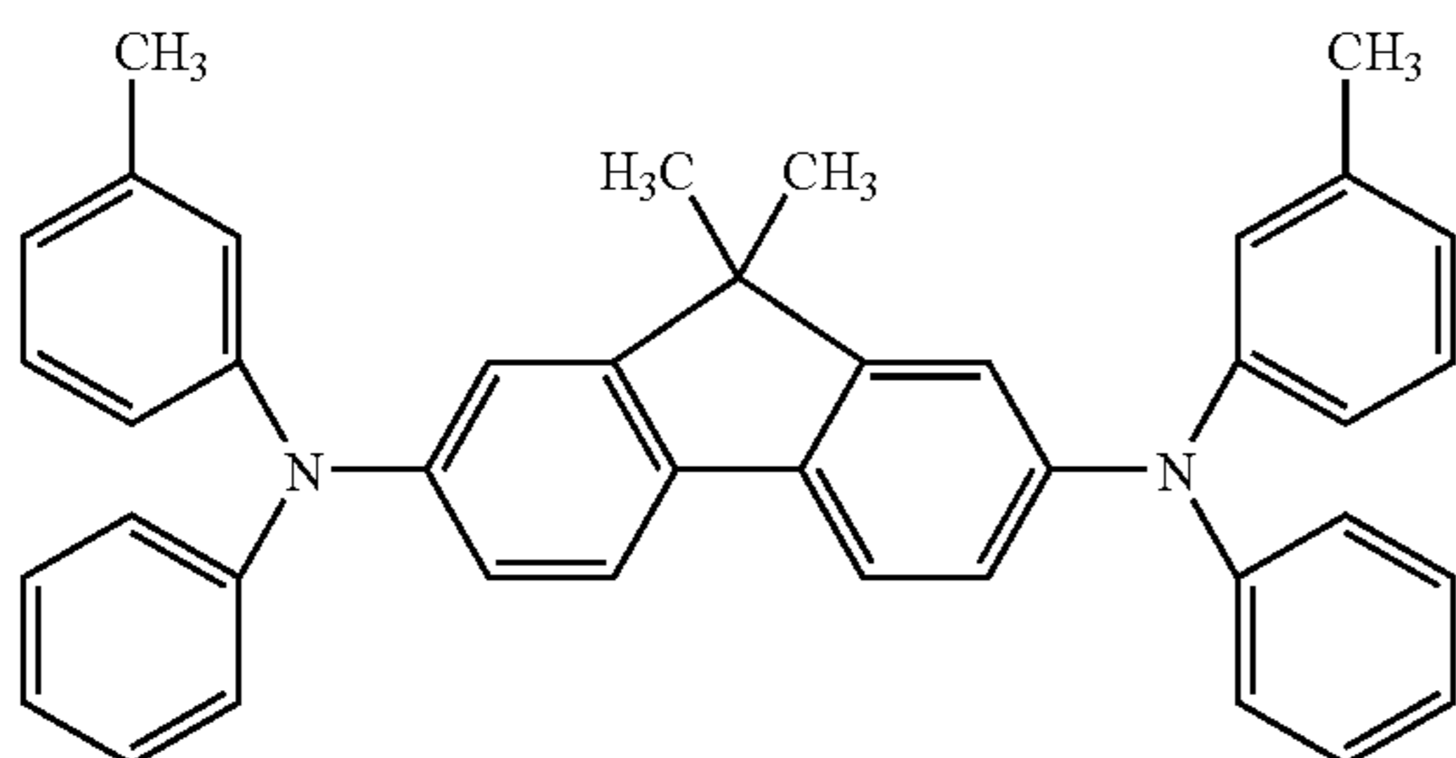
DTDPFL
