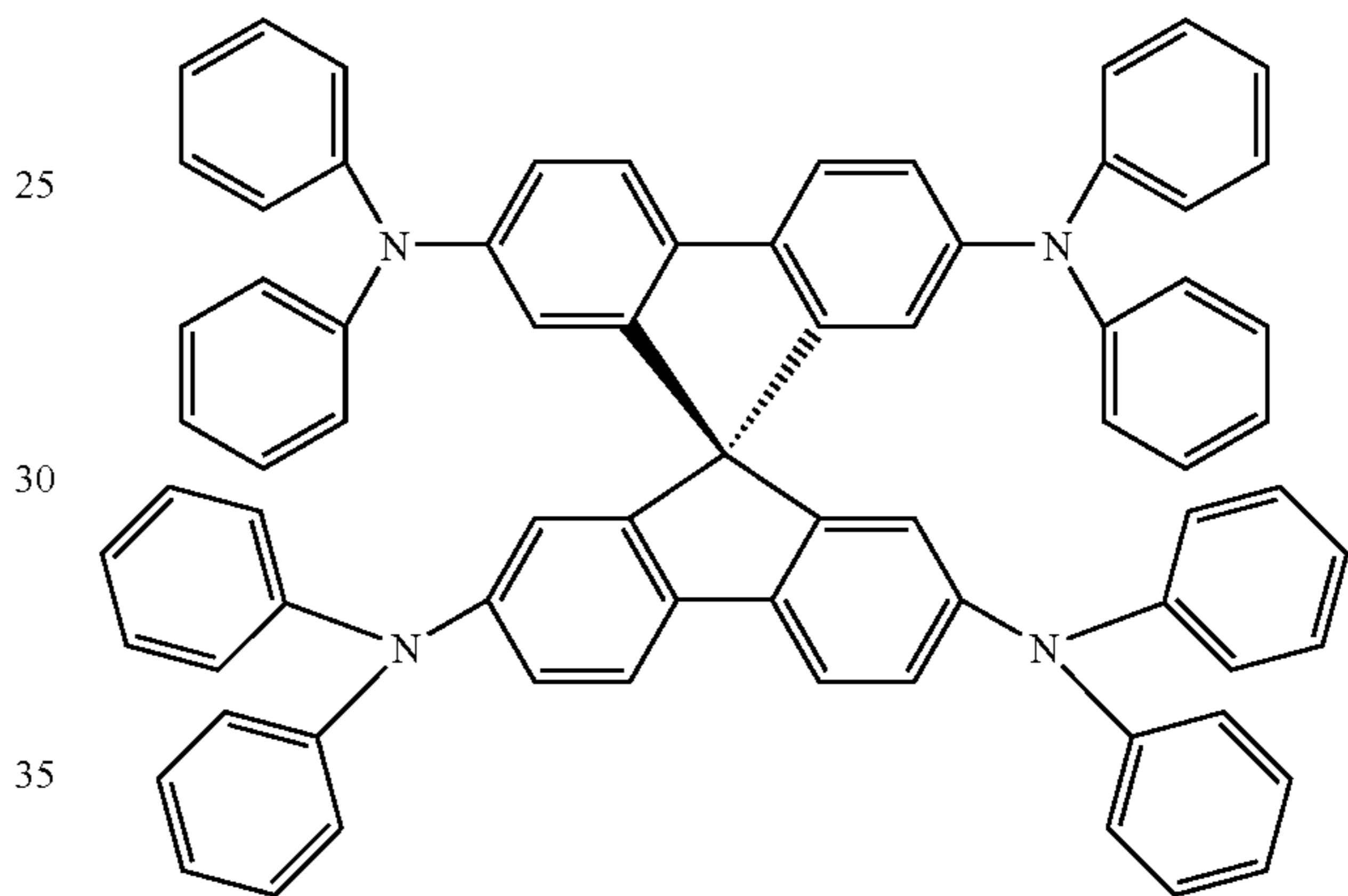
spiro-TPD
