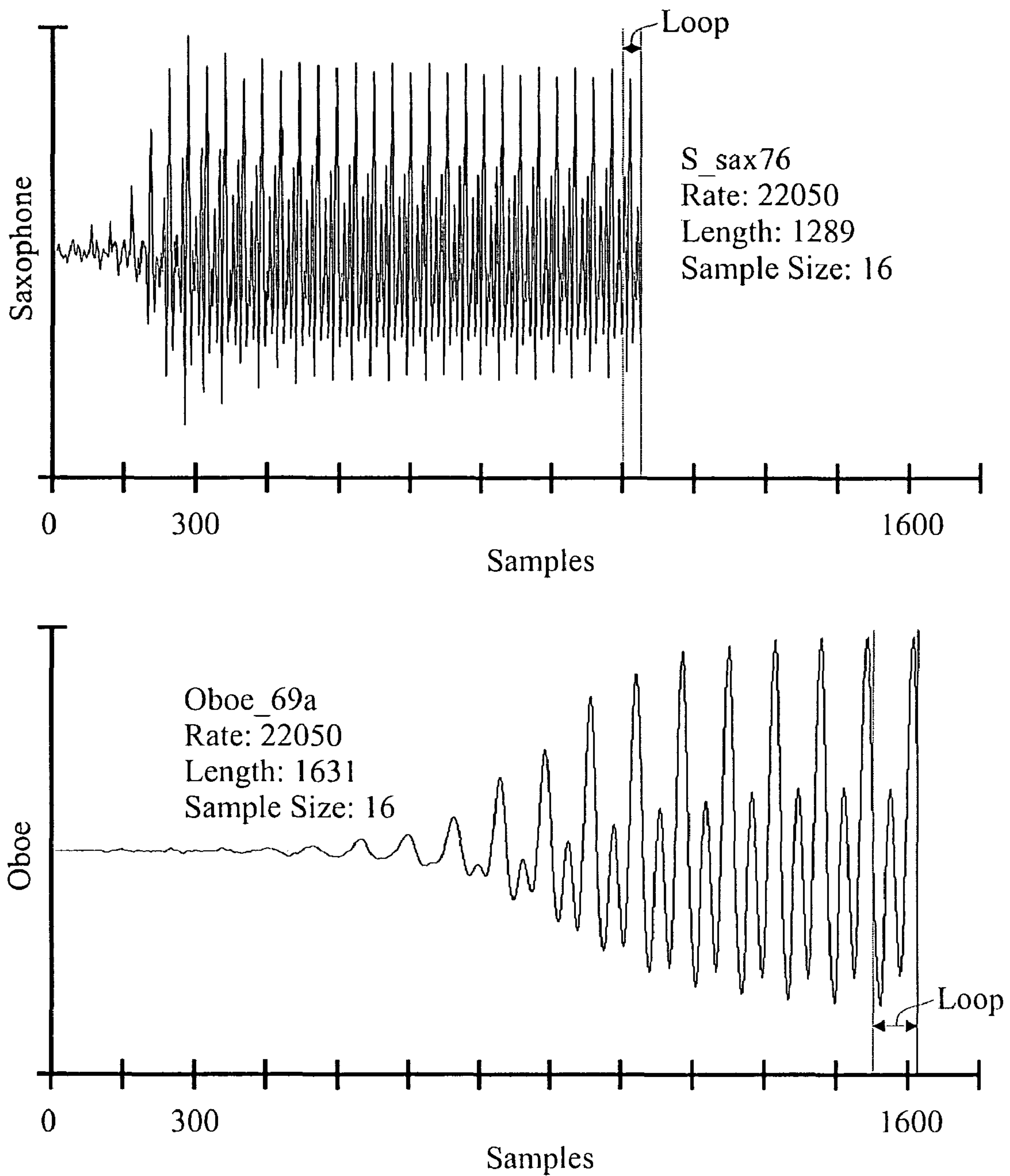
Figure 75 Prior Art Saxophone and Oboe Sounds
