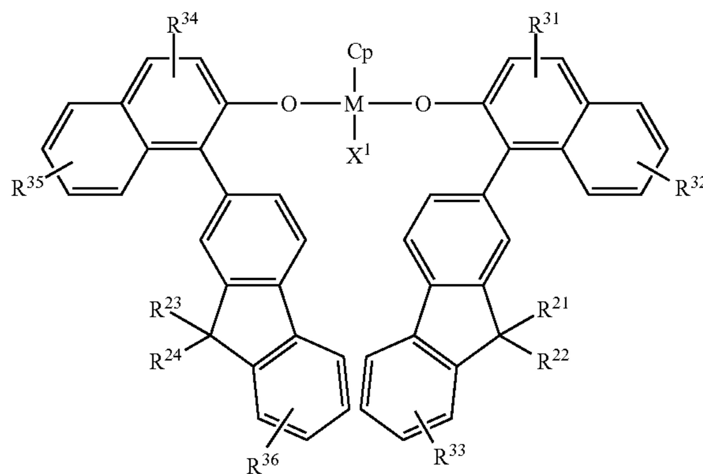
[Chemical Formula 1-5]
