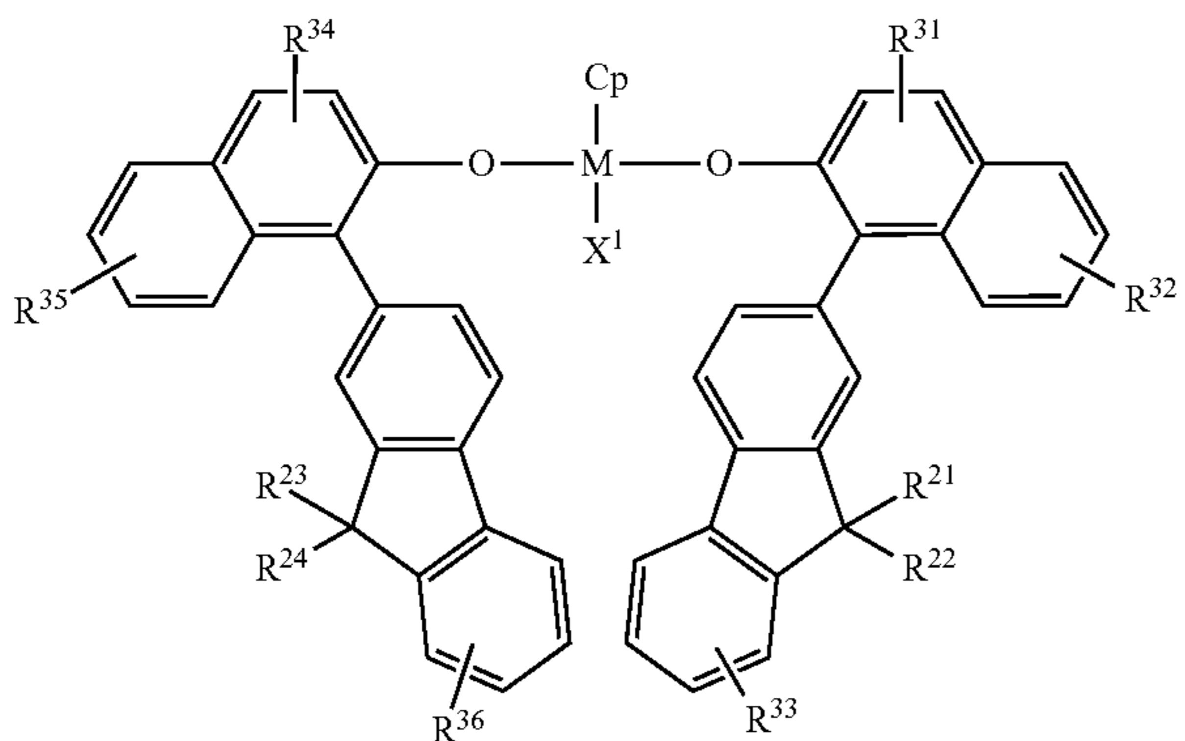
[Chemical Formula 1-5]
