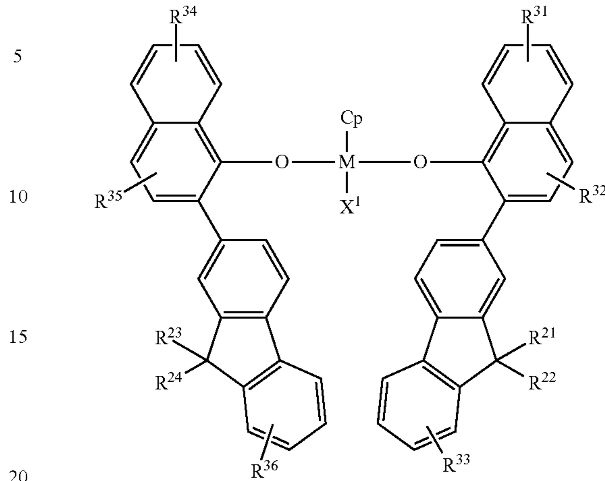
[Chemical Formula 1-3]
