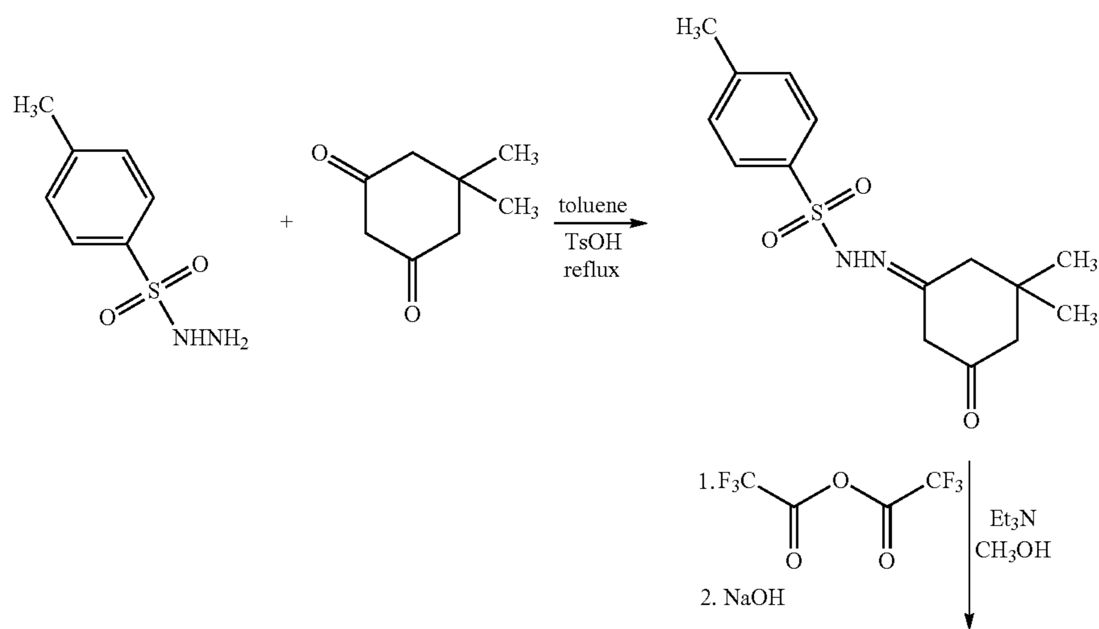
Scheme 6
