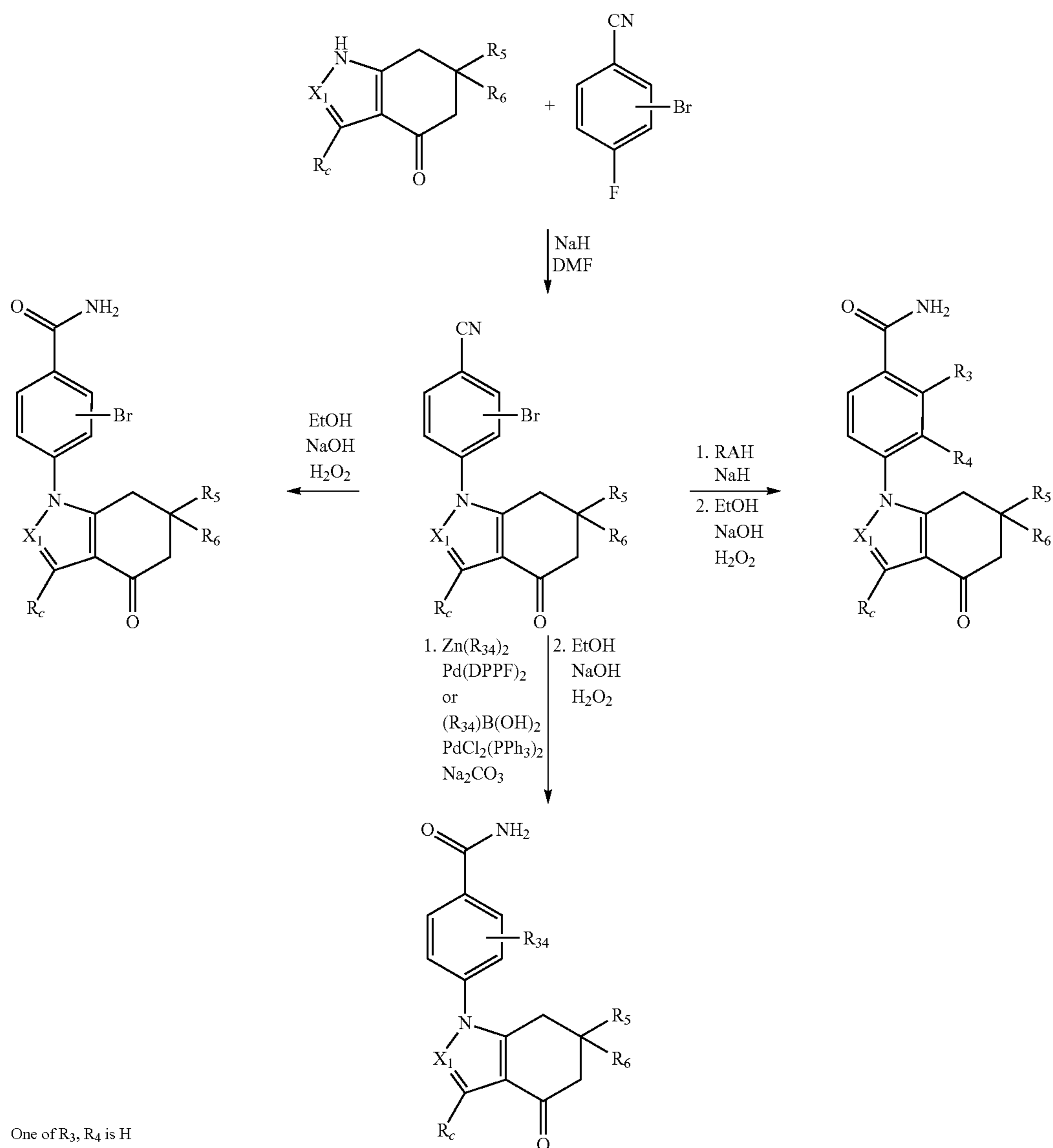
Scheme 9
