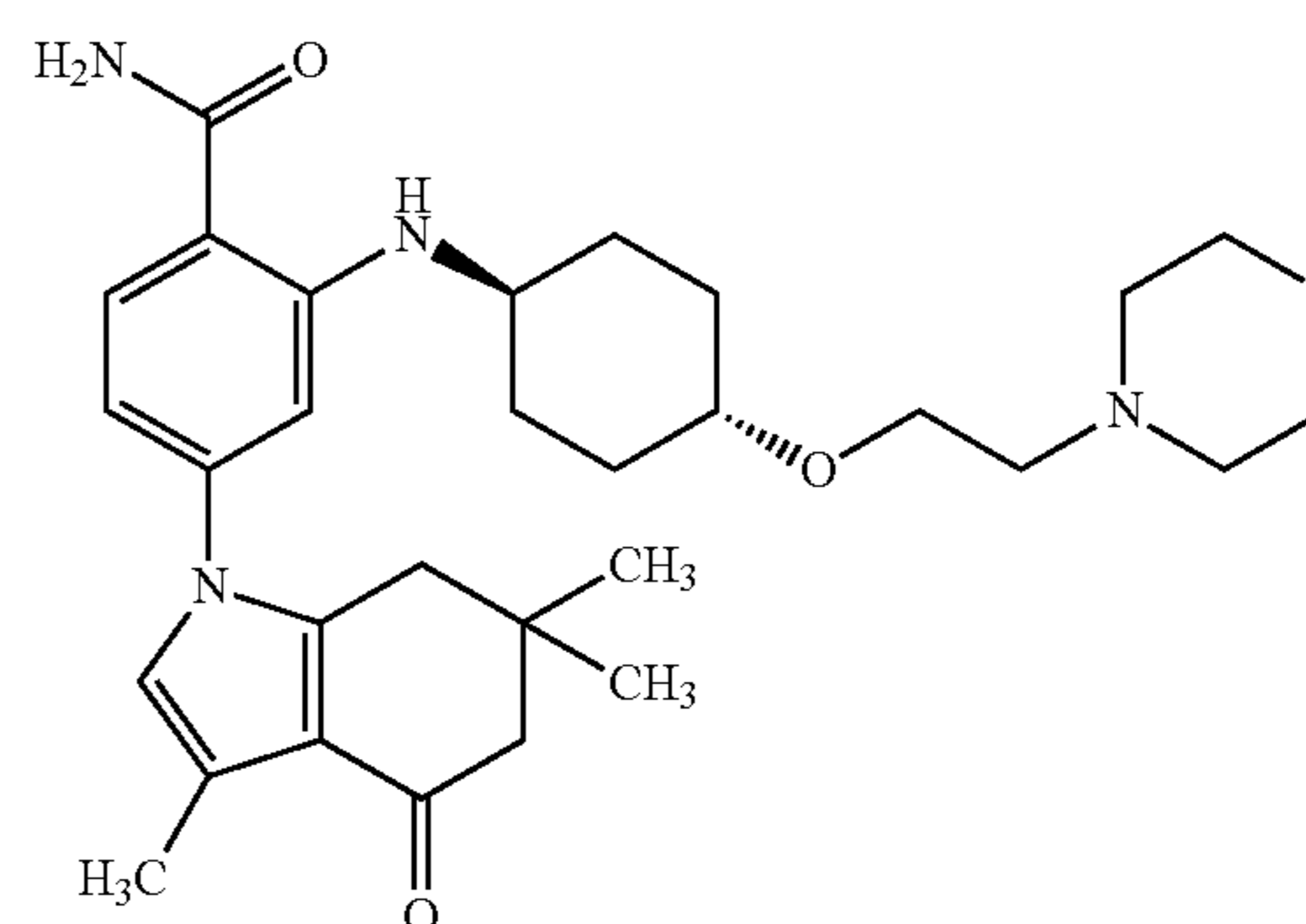
2-[trans-4-(2-Morpholin-4-yl-ethoxy)-cyclohexylamino]-4-(3,6,6-trimethyl-4-oxo-4,5,6,7-tetrahydro-indol-1-yl)-benzamide (Compound 9)
