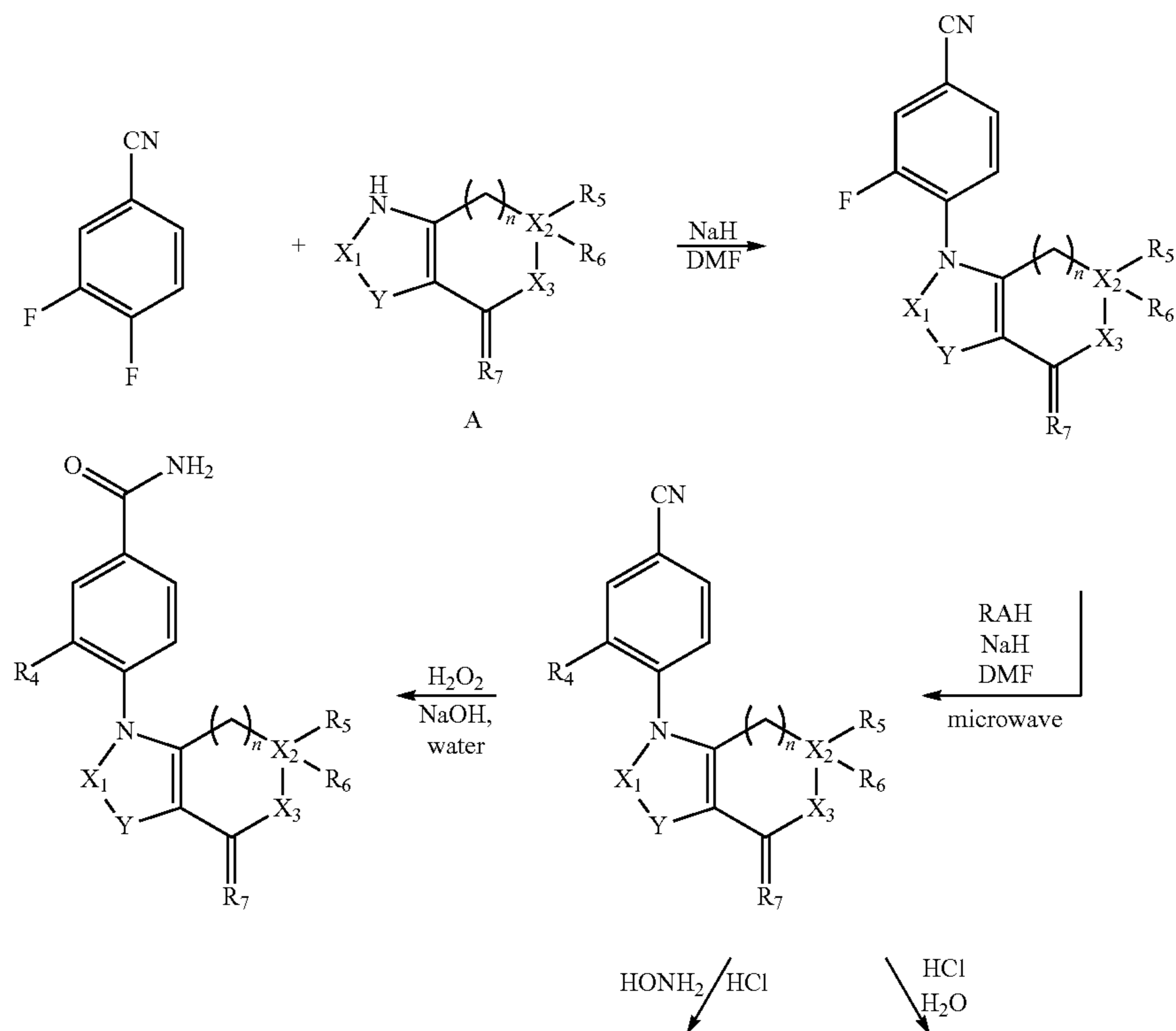
Scheme 8
