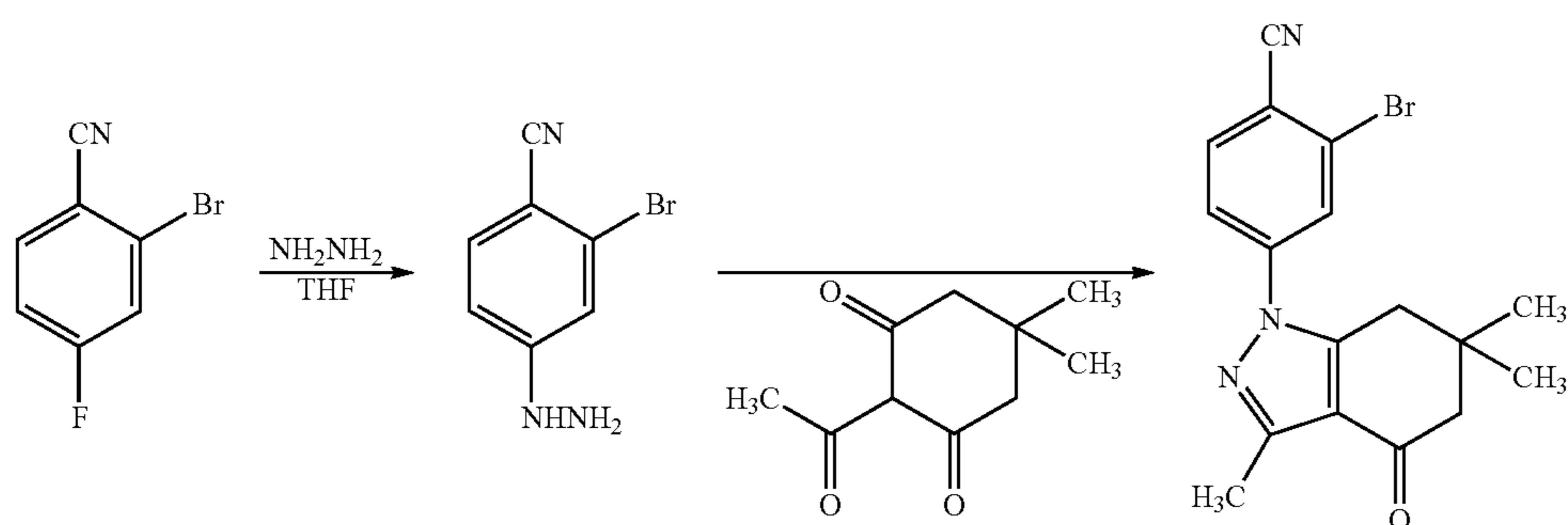
Scheme 4
