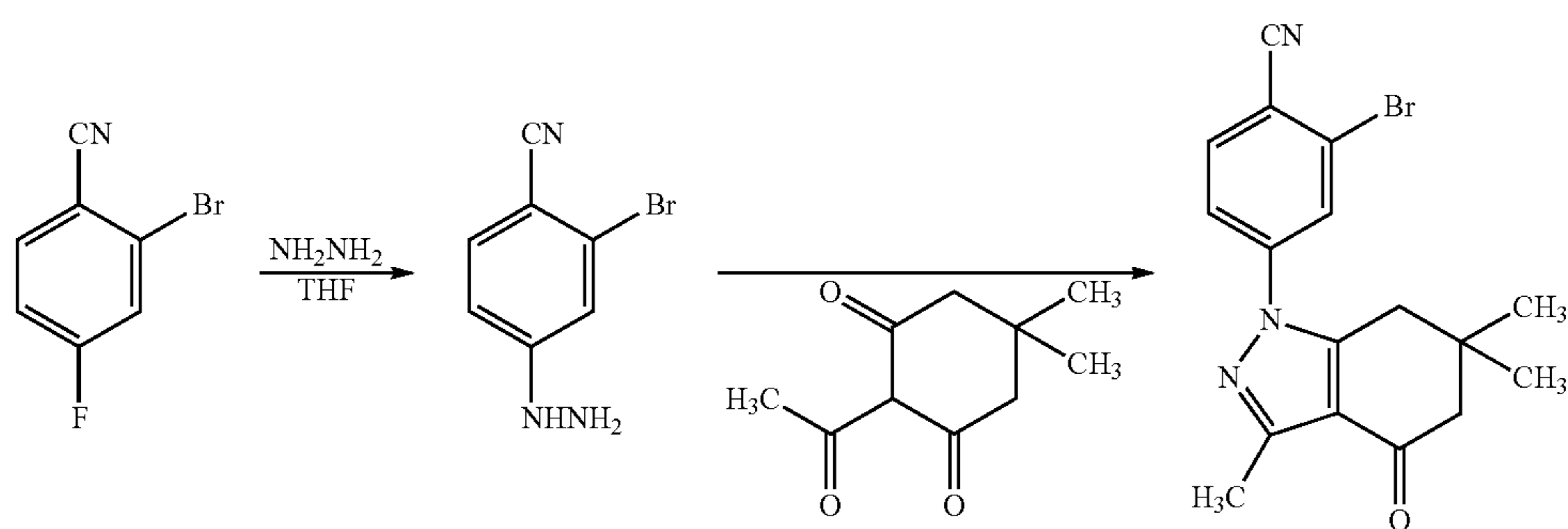
Scheme 4
