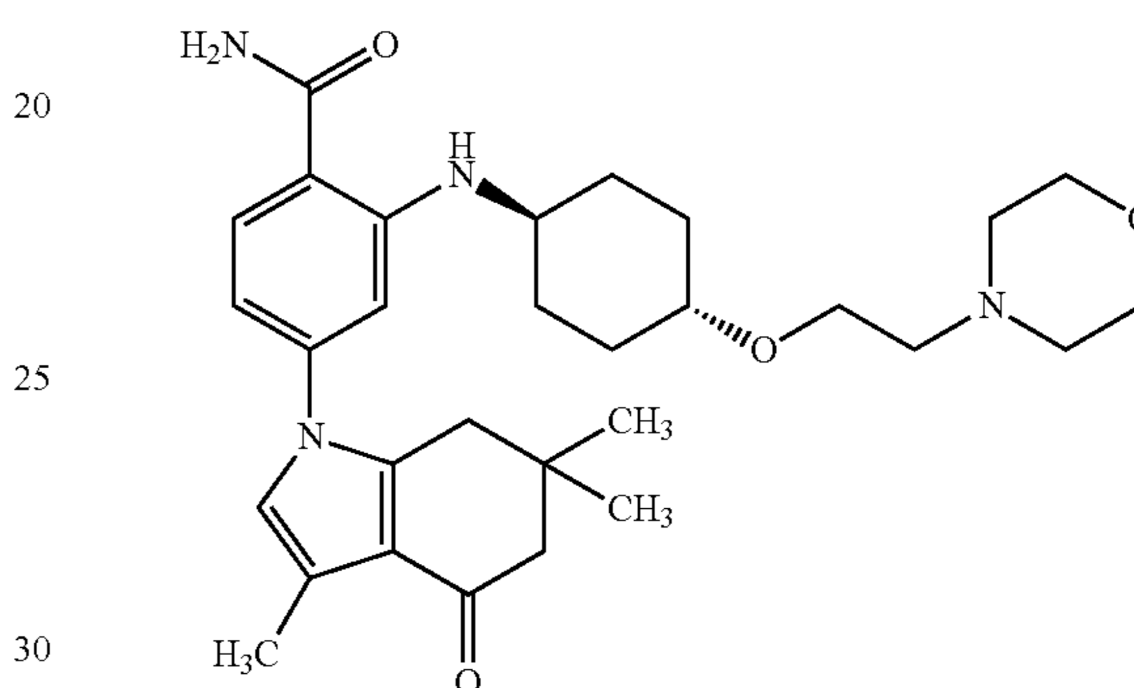
2-[trans-4-(2-Morpholin-4-yl-ethoxy)-cyclohexylamino]-4-(3,6,6-trimethyl-4-oxo-4,5,6,7-tetrahydro-indol-1-yl)-benzamide (Compound 9)
