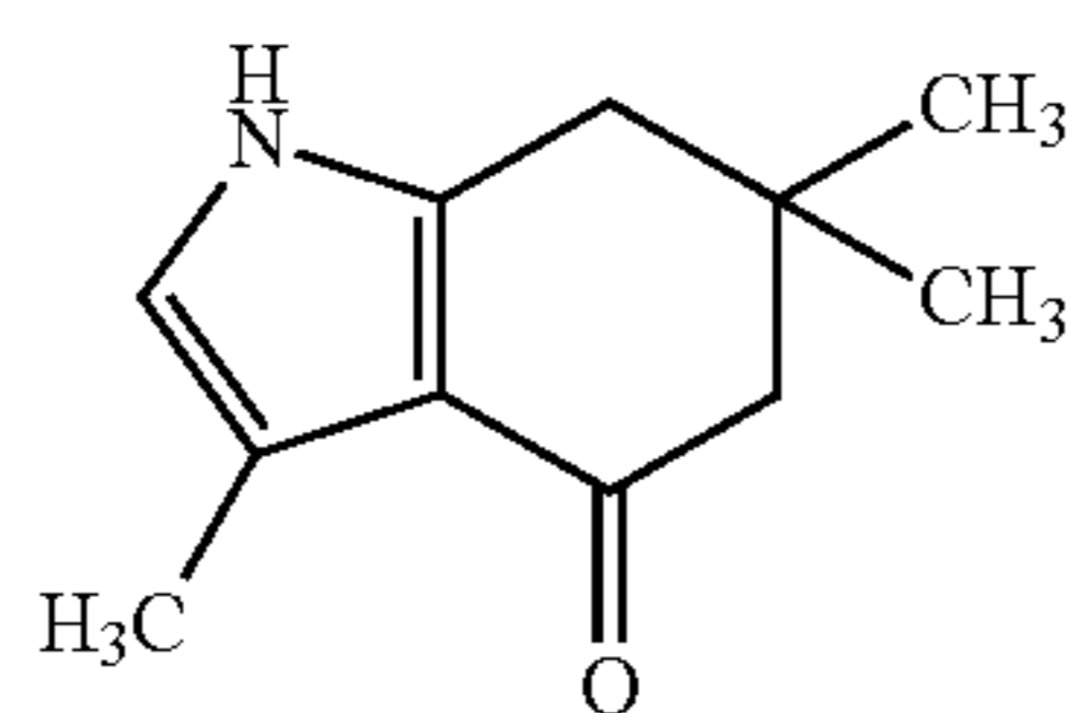
3,6,6-Trimethyl-1,5,6,7-tetrahydro-indol-4-one (Compound 1)
