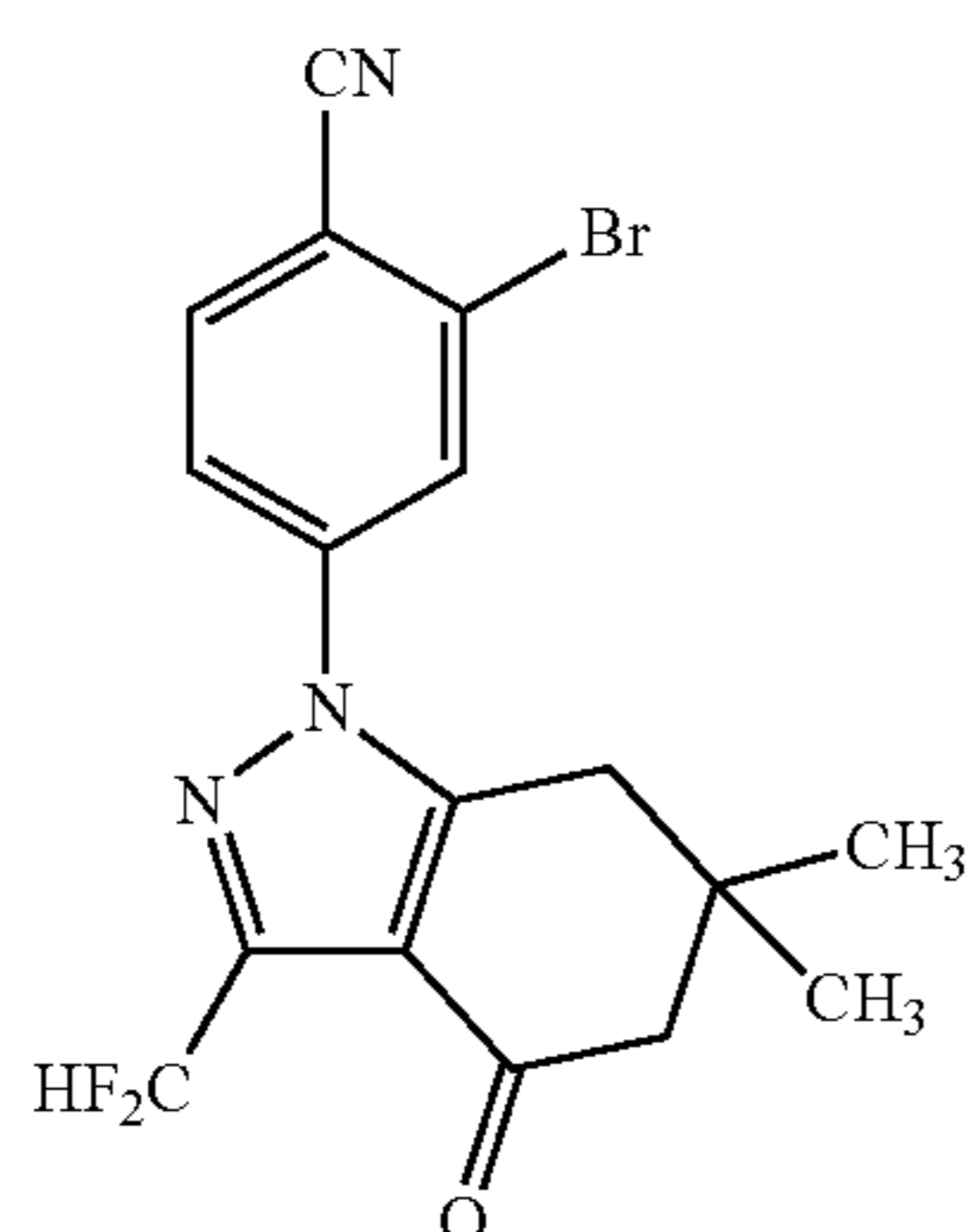
2-Bromo-4-(3-difluoromethyl-6,6-dimethyl-4-oxo-4,5,6,7-tetrahydro-indazol-1-yl)-benzonitrile (Compound 25)
