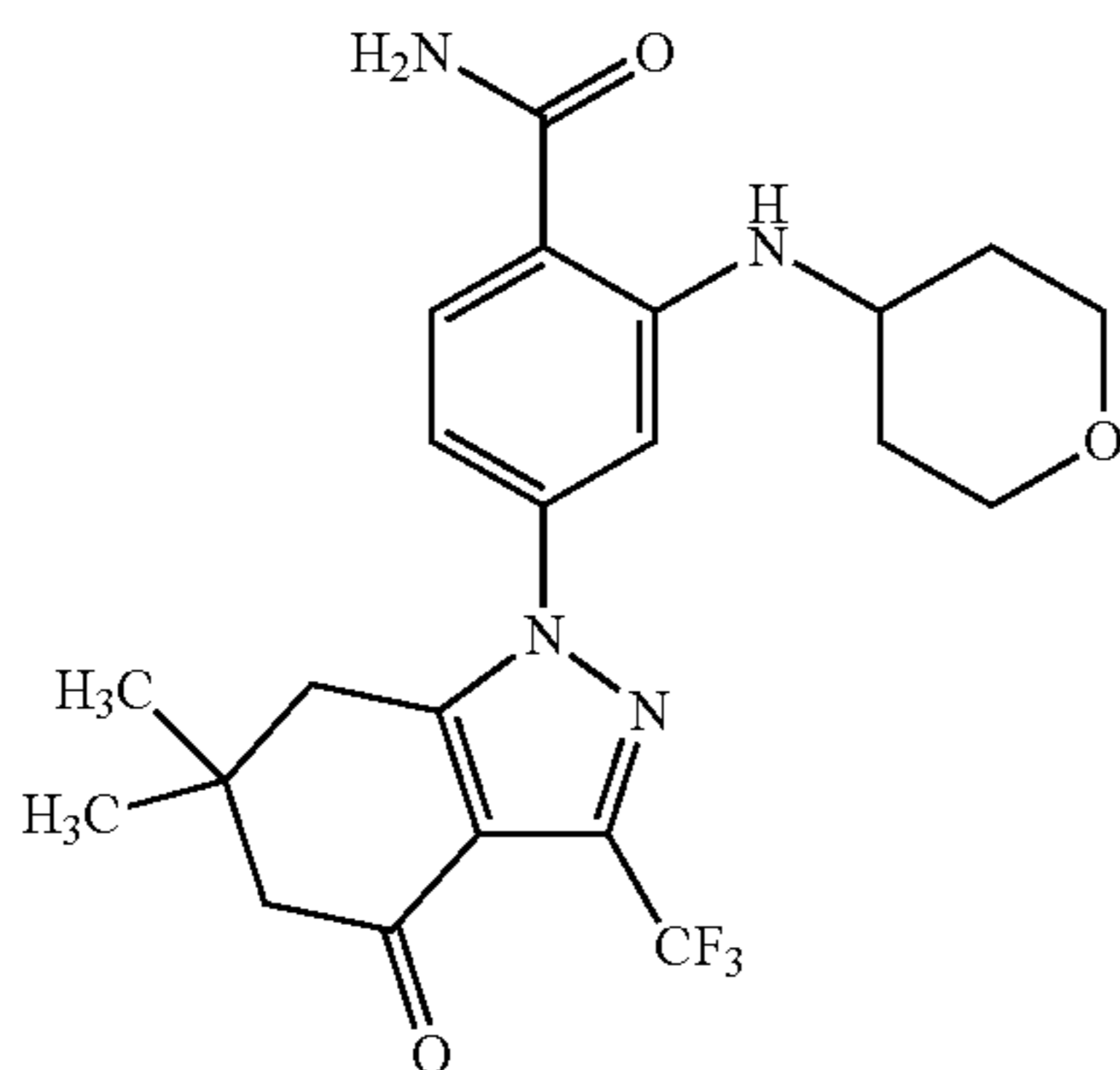
4-(6,6-Dimethyl-4-oxo-3-trifluoromethyl-4,5,6,7-tetrahydro-indazol-1-yl)-2-(tetrahydro-pyran-4-ylamino)-benzamide (Compound 23)
