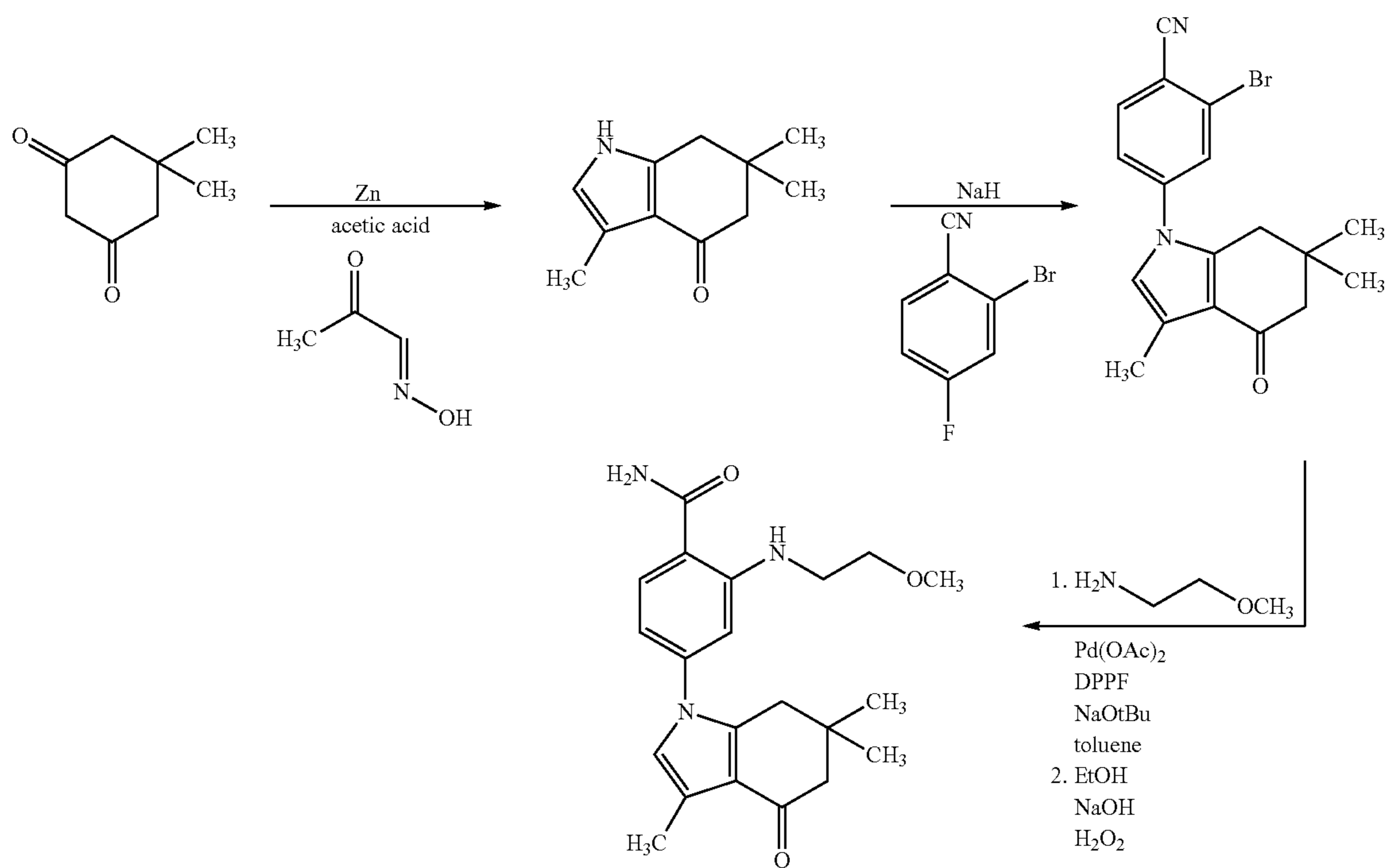
Scheme 3
