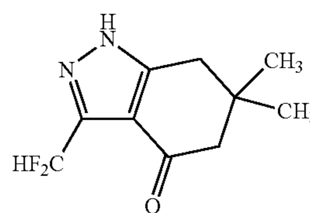
3-Difluoromethyl-6,6-dimethyl-1,5,6,7-tetrahydro-indazol-4-one (Compound 24)
