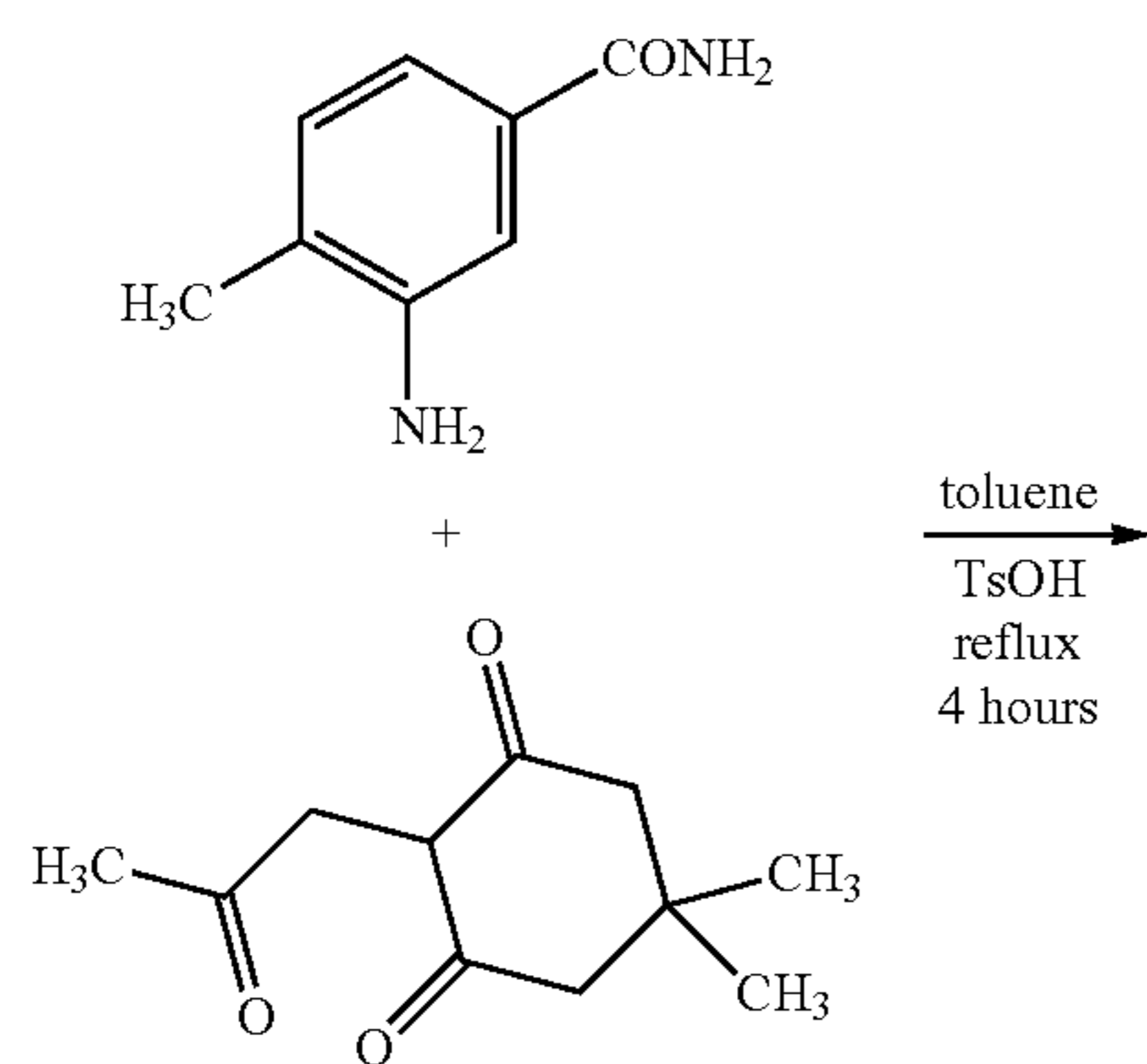
Scheme 7
