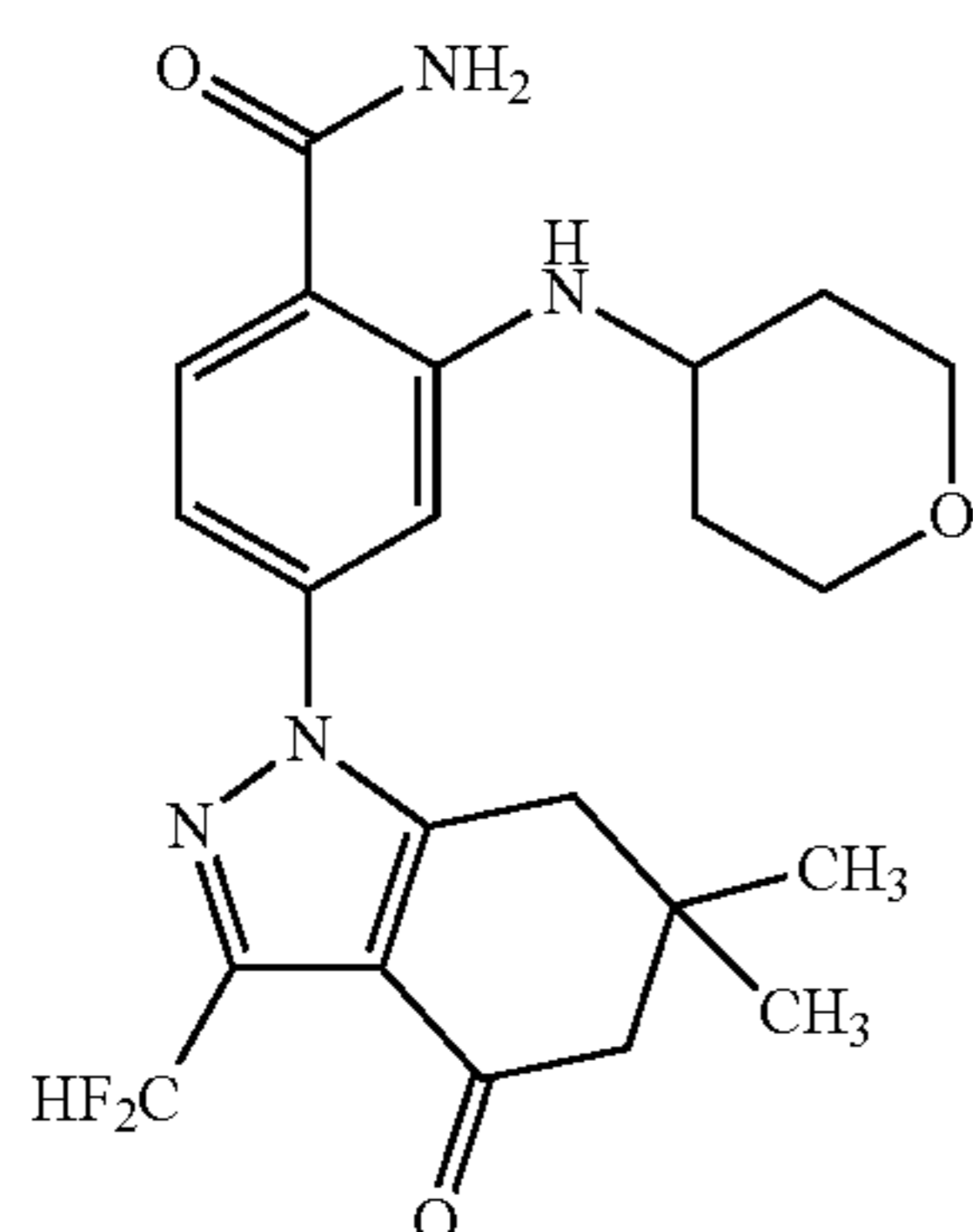
4-(6,6-Dimethyl-4-oxo-3-difluoromethyl-4,5,6,7-tetrahydro-indazol-1-yl)-2-(tetrahydro-pyran-4-ylamino)-benzamide (Compound 26)
