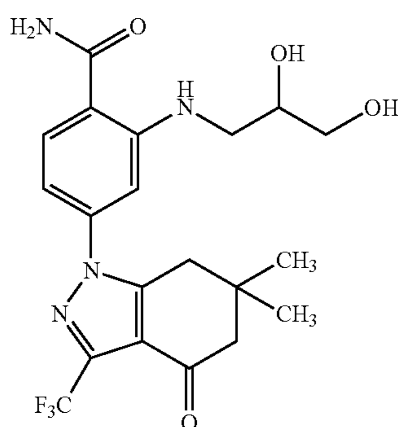
2-(2,3-Dihydroxy-propylamino)-4-(6,6-dimethyl-4-oxo-3-trifluoromethyl-4,5,6,7-tetrahydro-indazol-1-yl)-benzamide (Compound 30)
