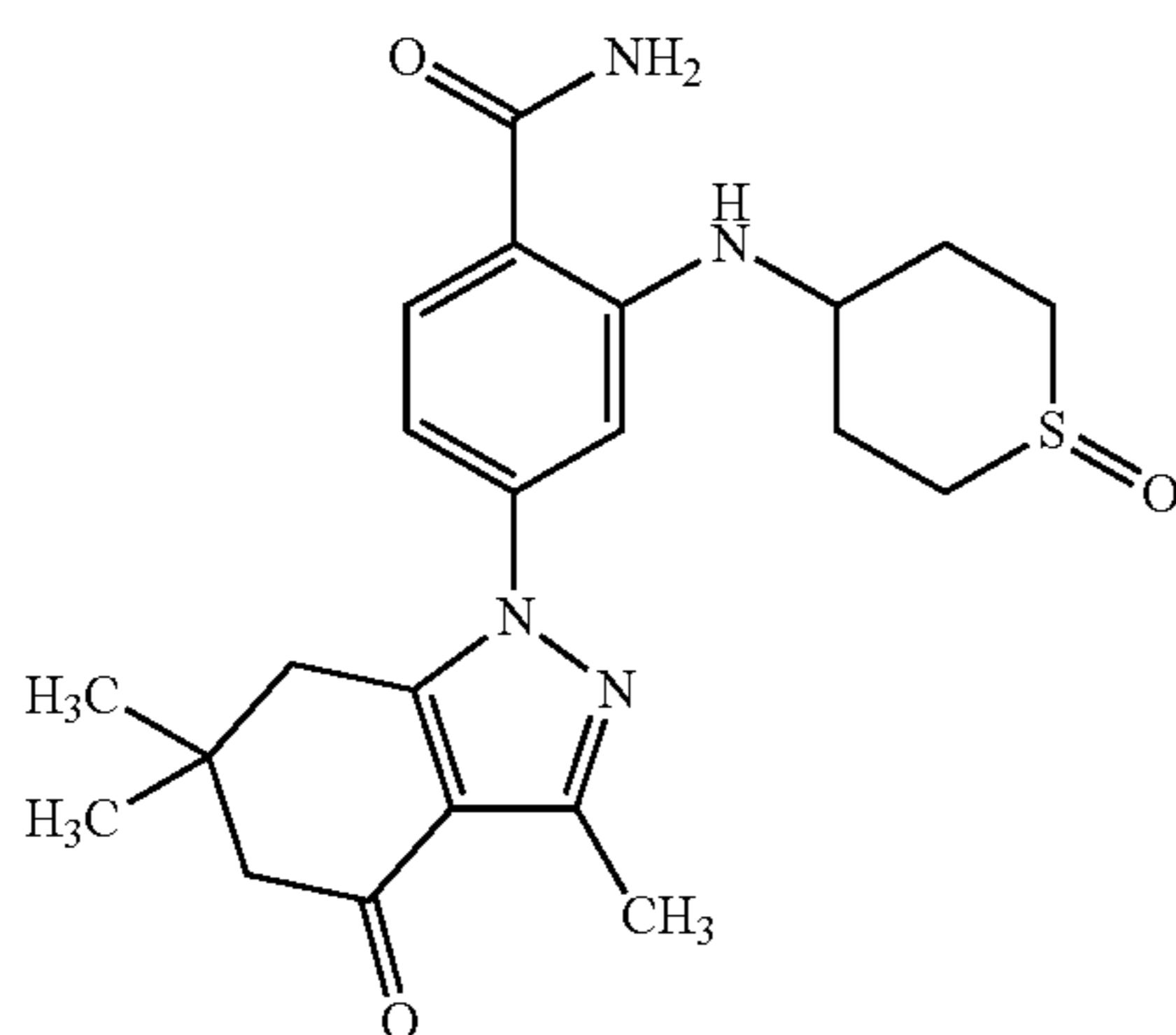
2-(1-Oxo-hexahydro-1-Tetrahydrothiopyran-4-ylamino)-4-(3,6,6-trimethyl-4-oxo-4,5,6,7-tetrahydroindazol-1-yl)benzamide (Compound 14)
