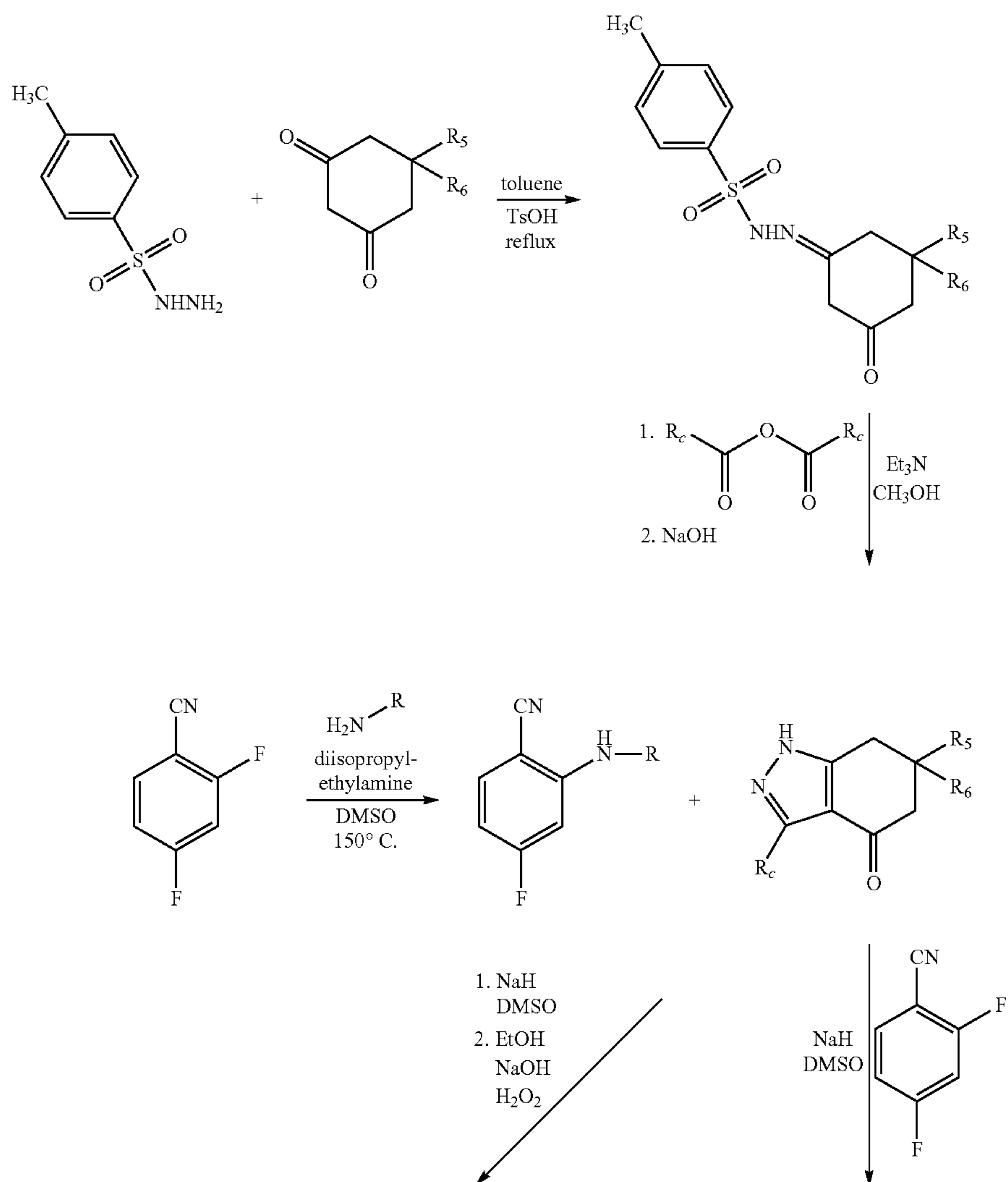
Scheme 5
