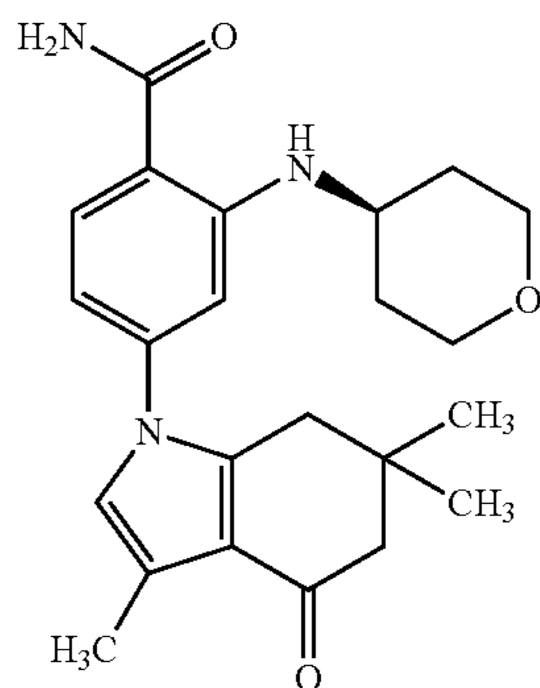
2-(Tetrahydro-pyran-4-ylamino)-4-(3,6,6-trimethyl-4-oxo-4,5,6,7-tetrahydro-indol-1-yl)-benzamide (Compound 4)
