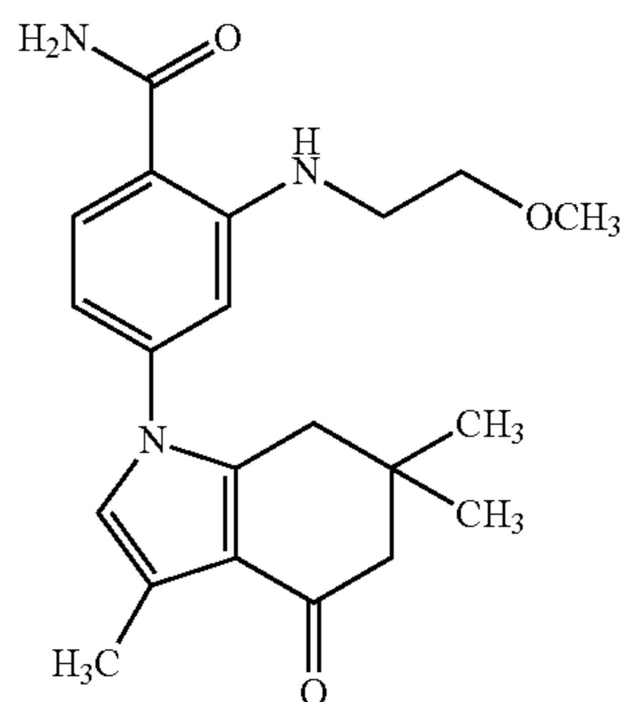
2-(2-Methoxy-ethylamino)-4-(3,6,6-trimethyl-4-oxo-4,5,6,7-tetrahydro-indol-1-yl)-benzamide (Compound 5)
