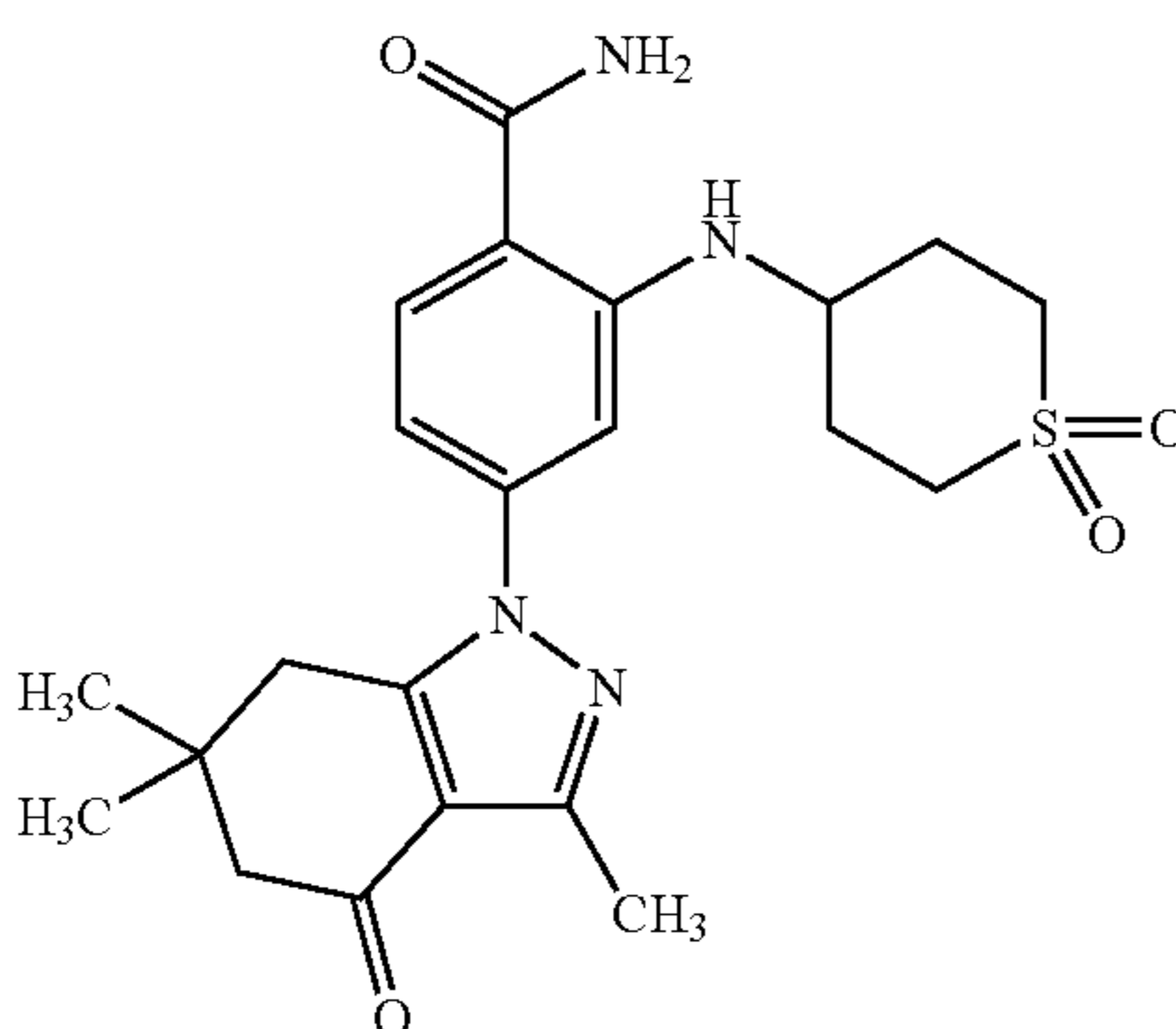
2-(1,1-Dioxo-hexahydro-1-Tetrahydrothiopyran-4-ylamino)-4-(3,6,6-trimethyl-4-oxo-4,5,6,7-tetrahydroindazol-1-yl)benzamide (Compound 15)
