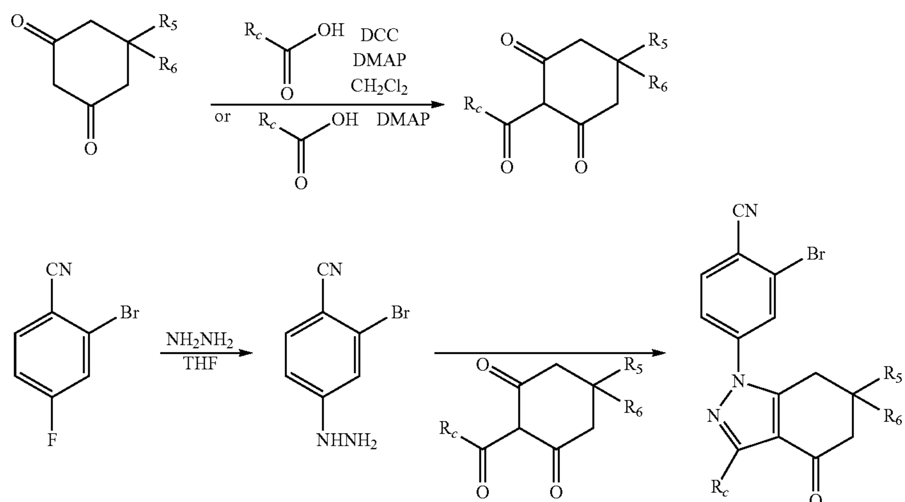
Scheme 2
