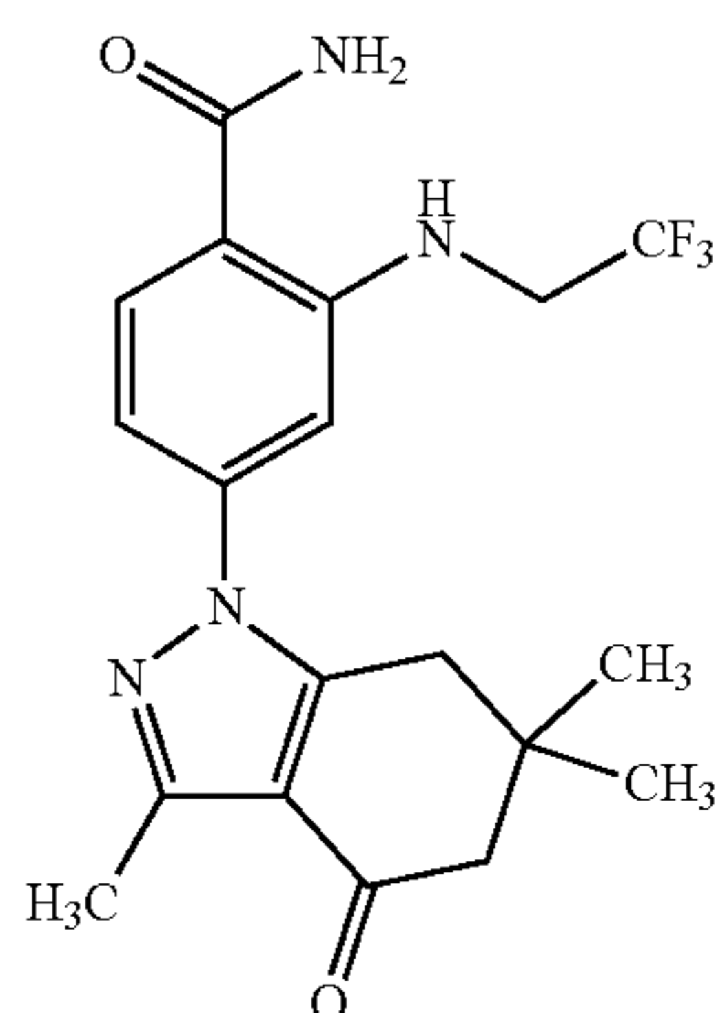
2-(2,2,2-Trifluoro-ethylamino)-4-(3,6,6-trimethyl-4-oxo-4,5,6,7-tetrahydro-indazol-1-yl)-benzamide (Compound 35)
