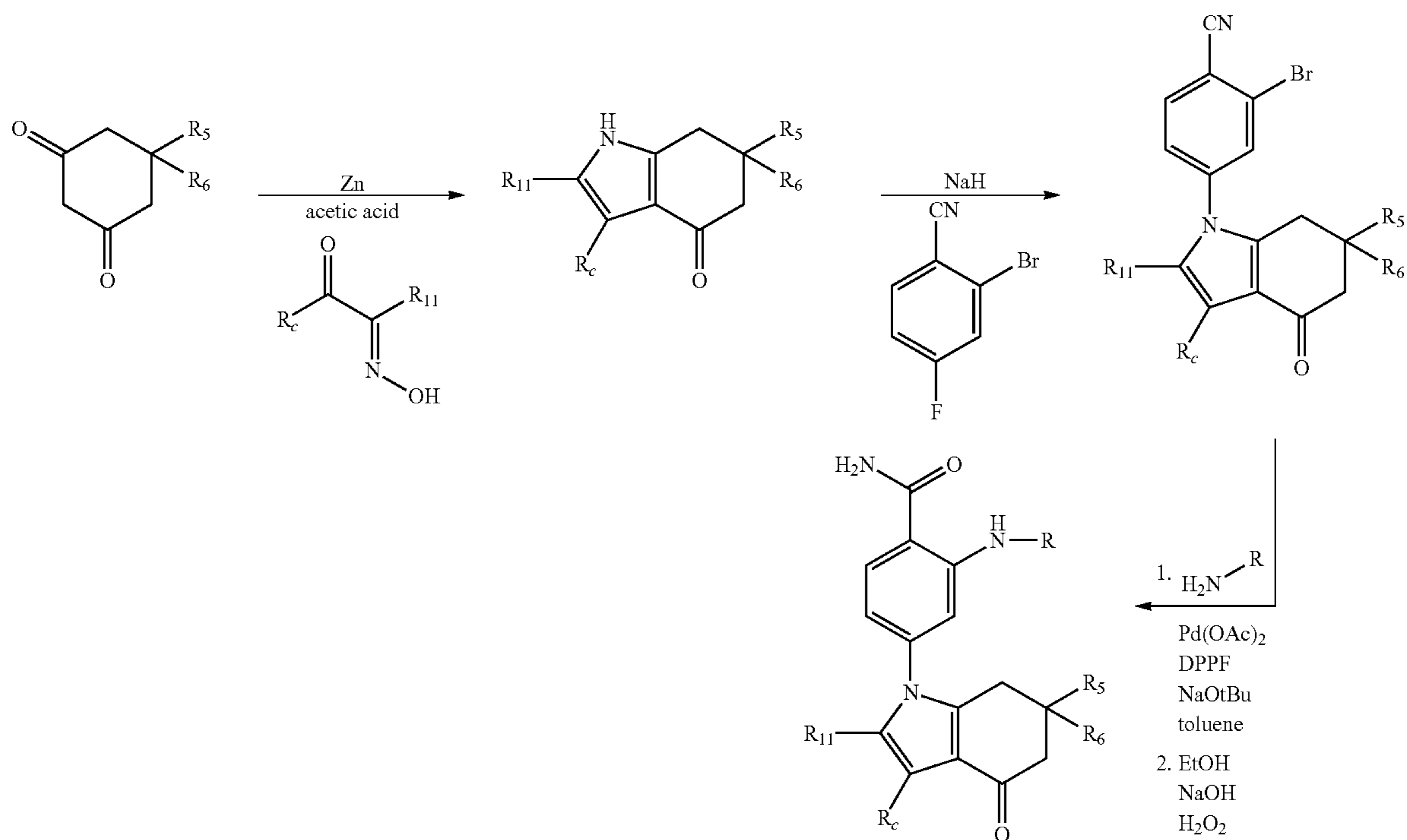
Scheme 1
