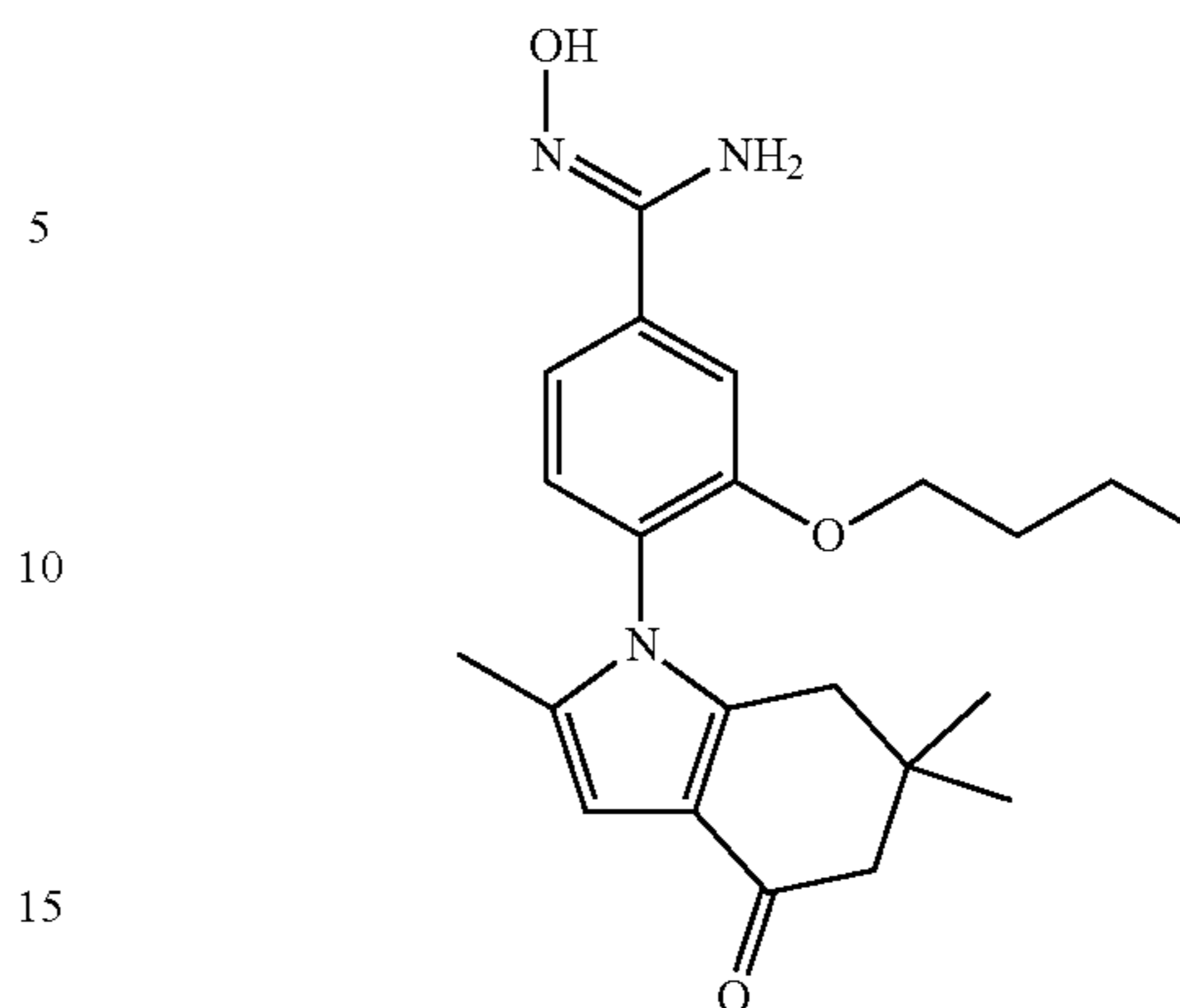
(Z)-3-butoxy-N'-hydroxy-4-(2,6,6-trimethyl-4-oxo-4,5,6,7-tetrahydro-1H-indol-1-yl)benzimidamide (Compound 62)
