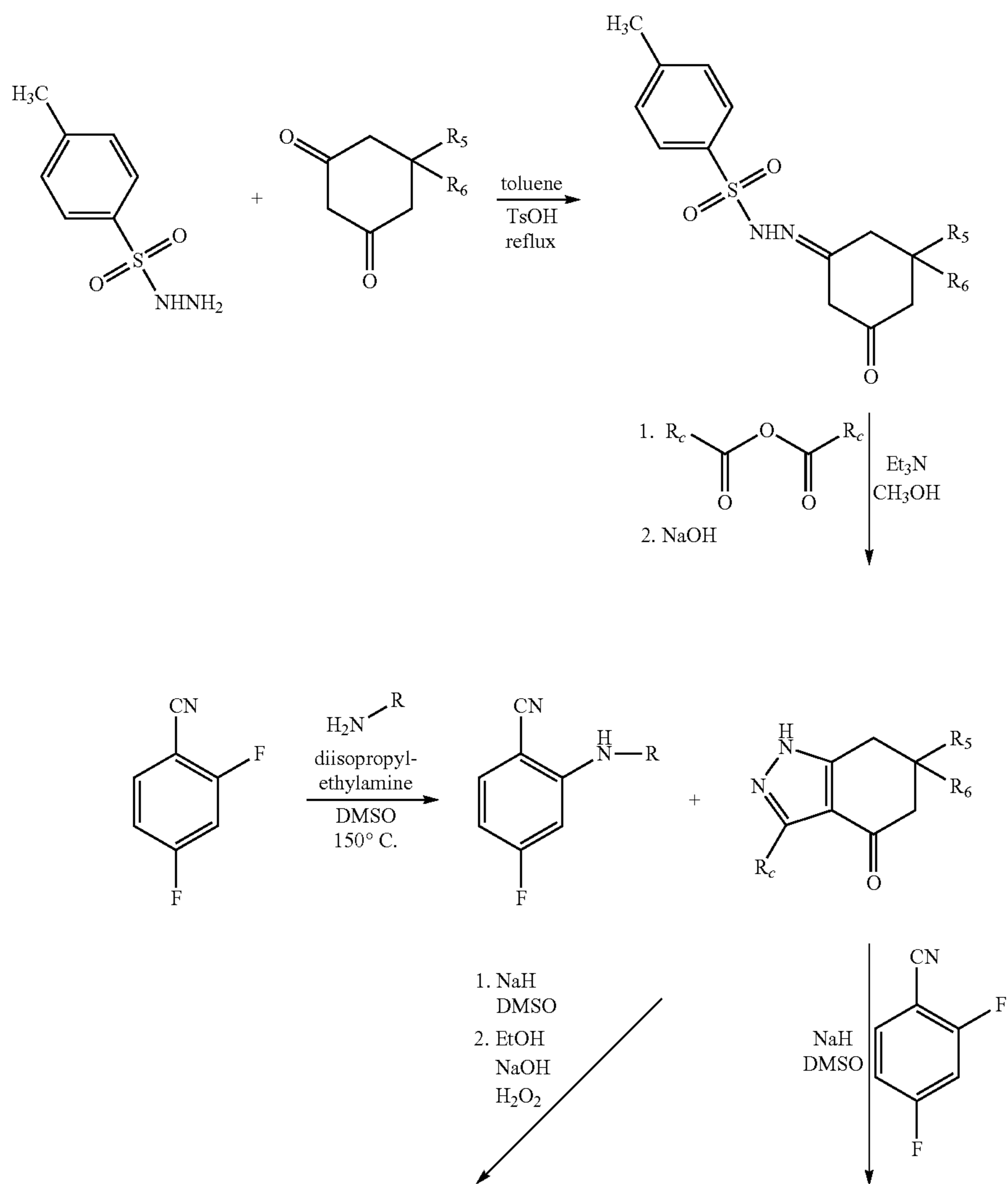
Scheme 5
