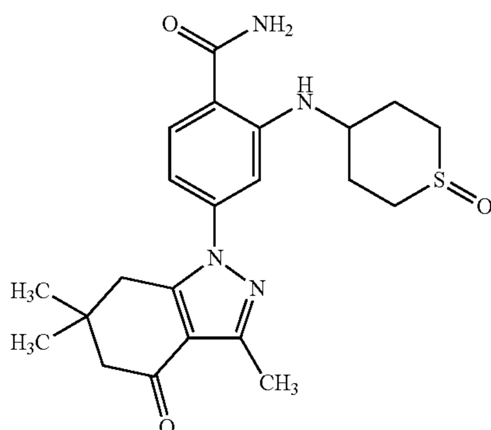
2-(1-Oxo-hexahydro-1-Tetrahydrothiopyran-4-ylamino)-4-(3,6,6-trimethyl-4-oxo-4,5,6,7-tetrahydroindazol-1-yl)benzamide (Compound 14)
