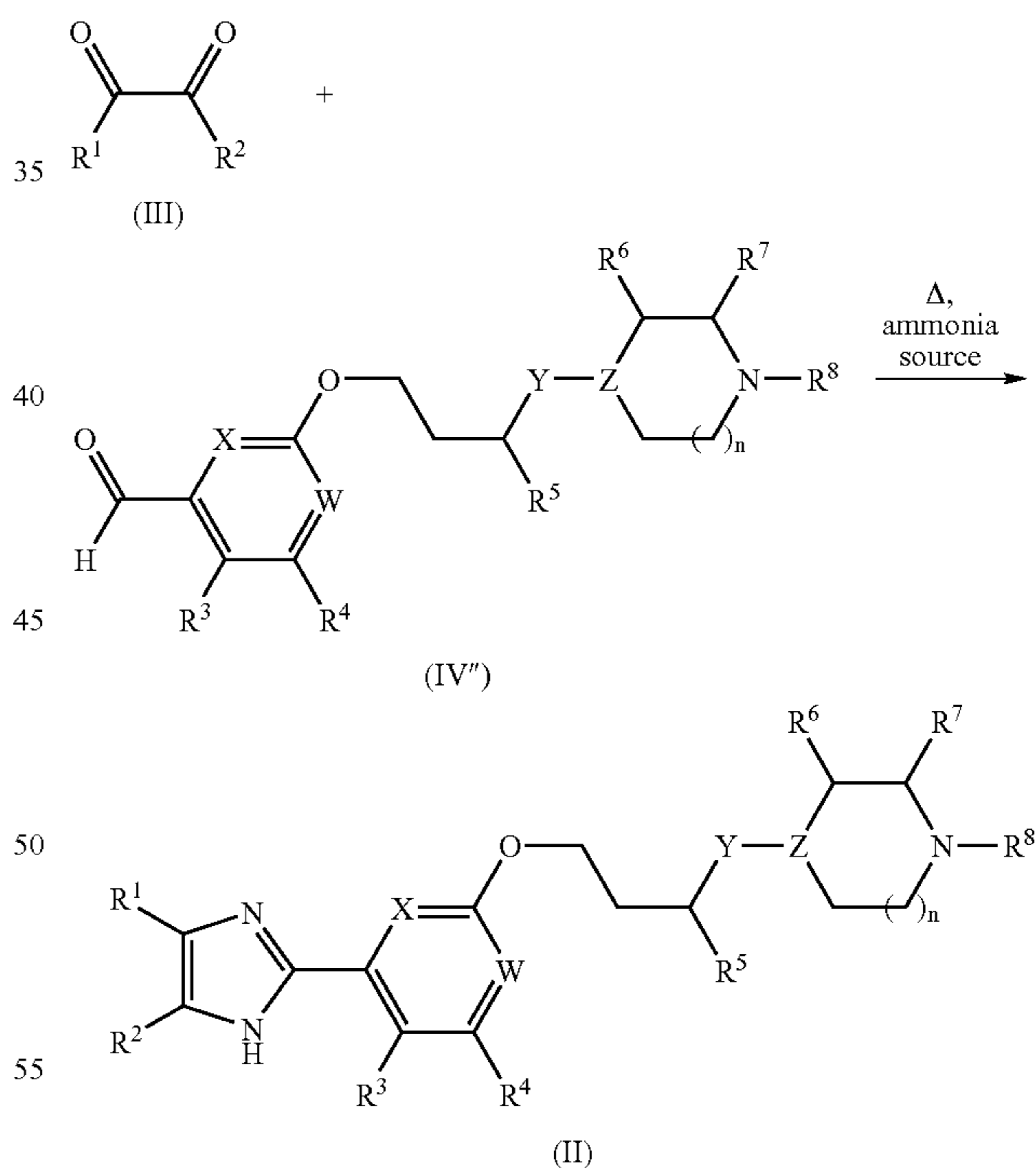
SCHEME 2
