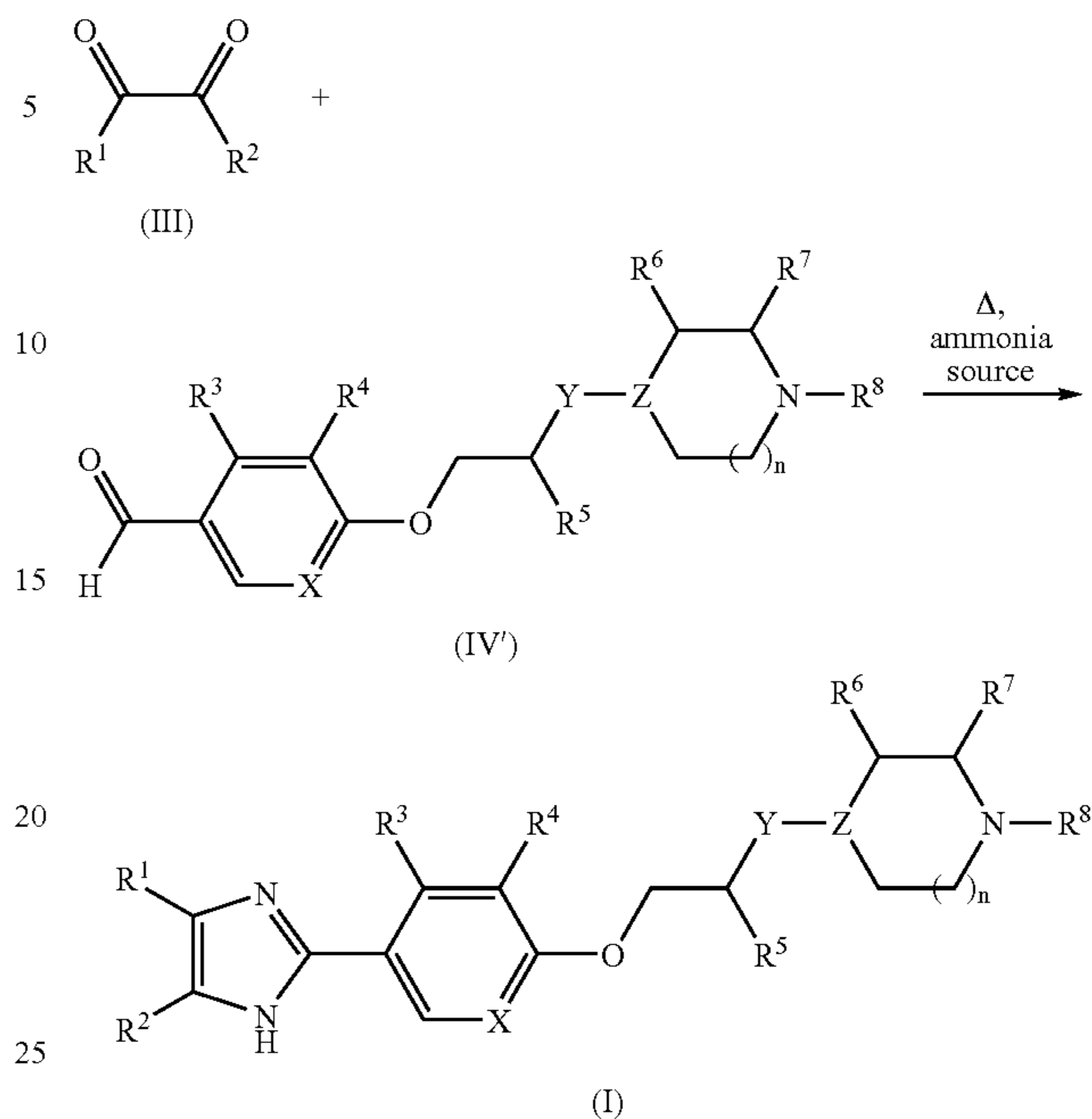
SCHEME 1
