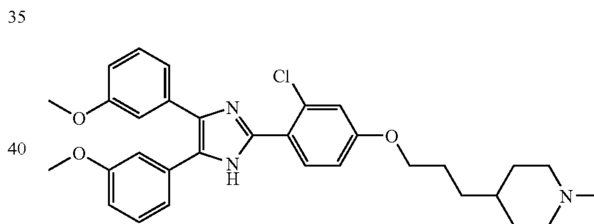
4-(3-{4-[4,5-Bis-(3-methoxy-phenyl)-1H-imidazol-2-yl]-3-chloro-phenoxy}-propyl)-1-methyl-piperidine.
