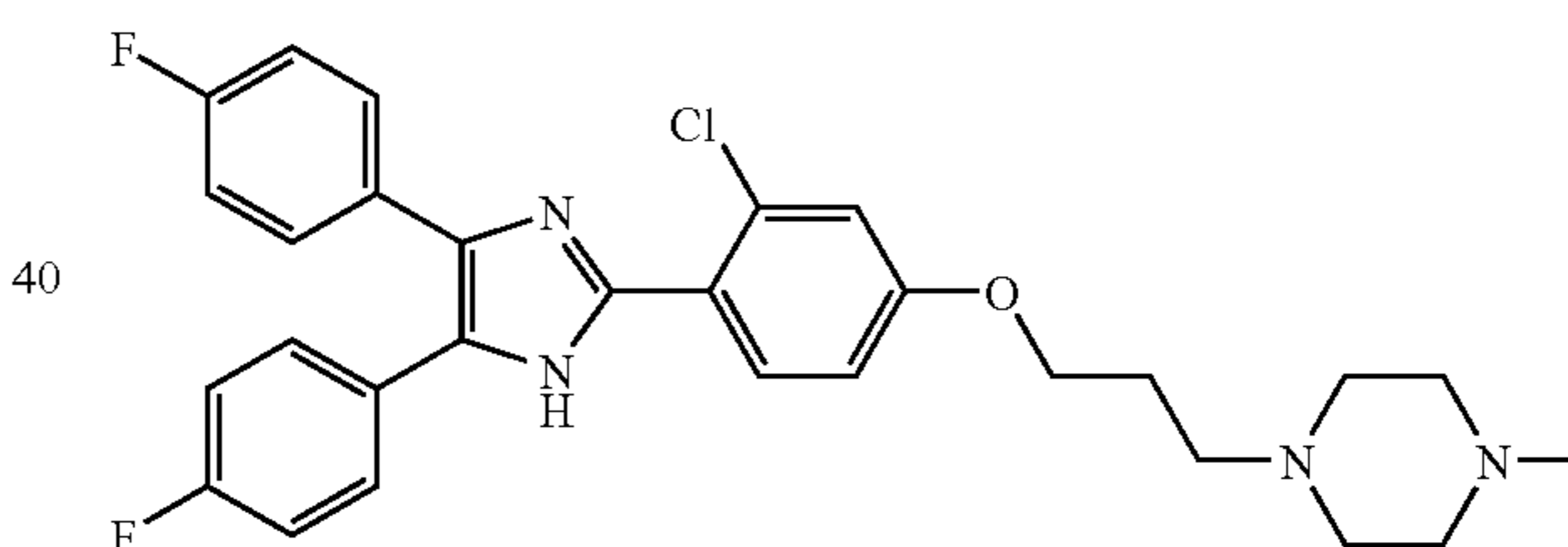
1-(3-[4-[4,5-Bis-(4-fluoro-phenyl)-1H-imidazol-2-yl]-3-chloro-phenoxy]propyl)-4-methyl-piperazine.
