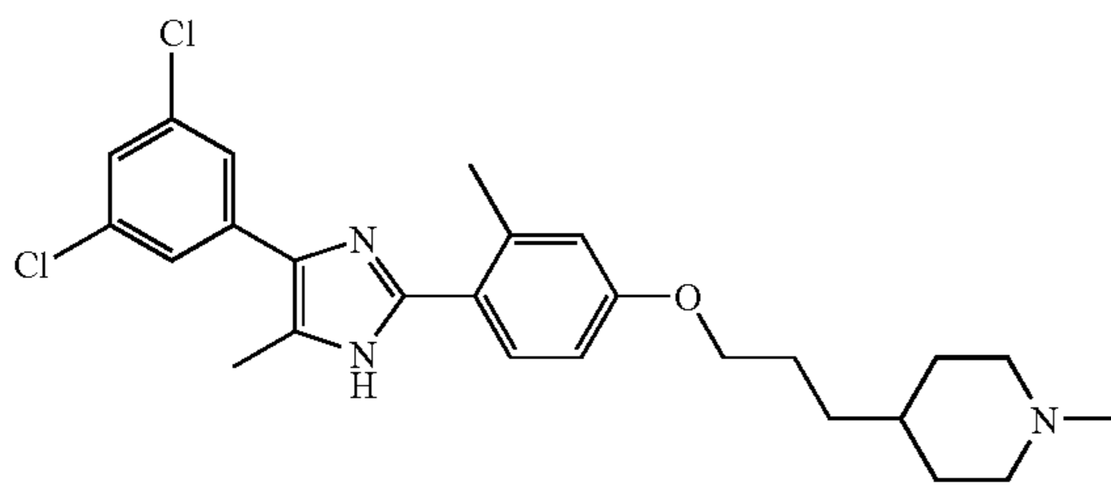
4-(3-{4-[4-(3,5-Dichloro-phenyl)-5-methyl-1H-imidazol-2-yl]-3-methyl-phenoxy}-propyl)-1-methyl-piperidine.
