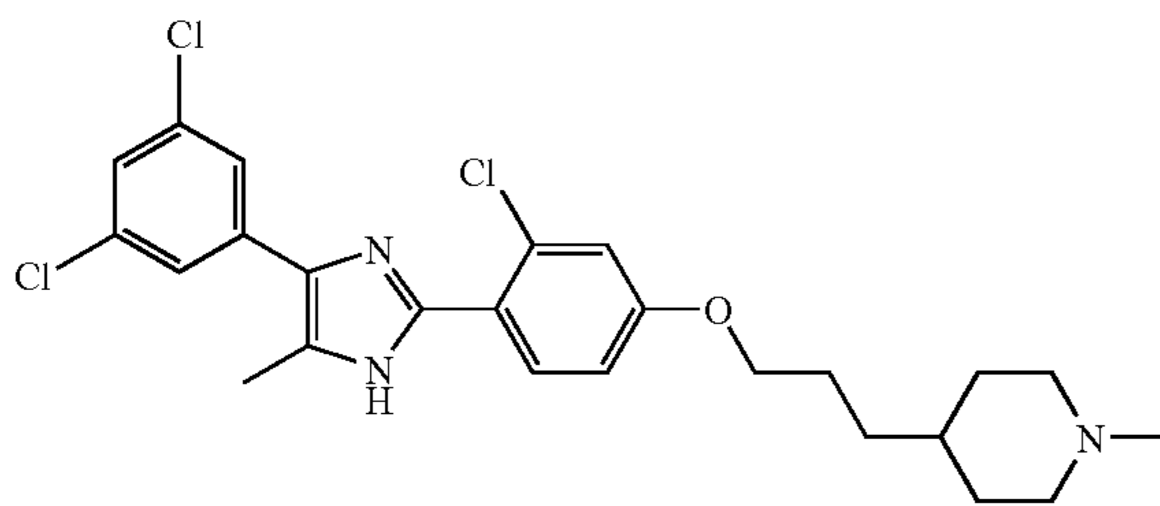
4-(3-{3-Chloro-4-[4-(3,5-dichloro-phenyl)-5-methyl-1H-imidazol-2-yl]-phenoxy}-propyl)-1-methyl-piperidine.
