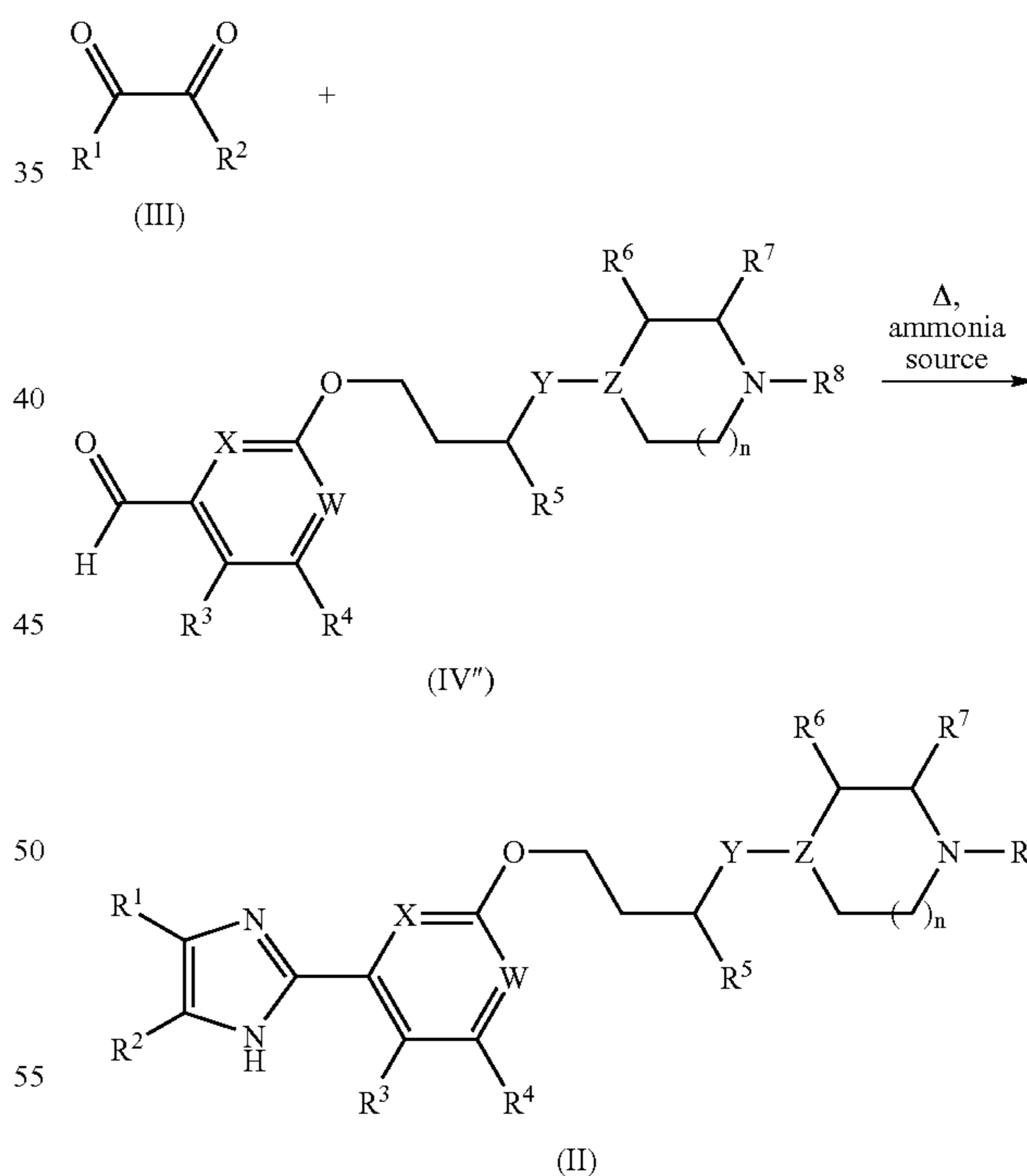
SCHEME 2
