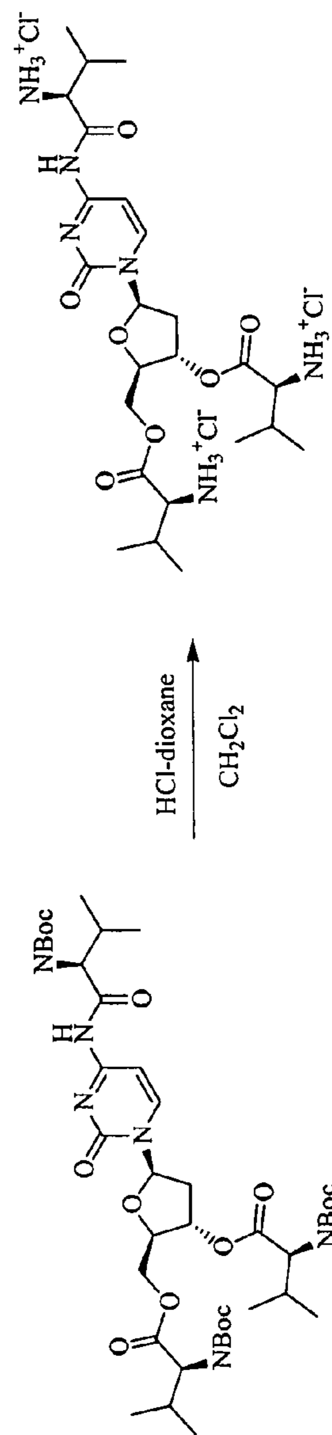
Figure 6 Synthesis of N'-Boc-valinyl ester of 2'-deoxy-β-L-cytidine
