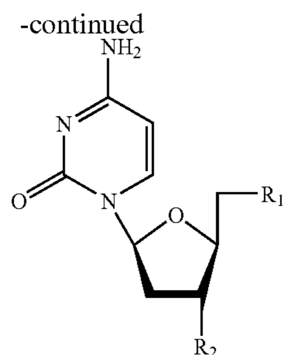
3'- or 5'-O-valinyl ester of L-dC
