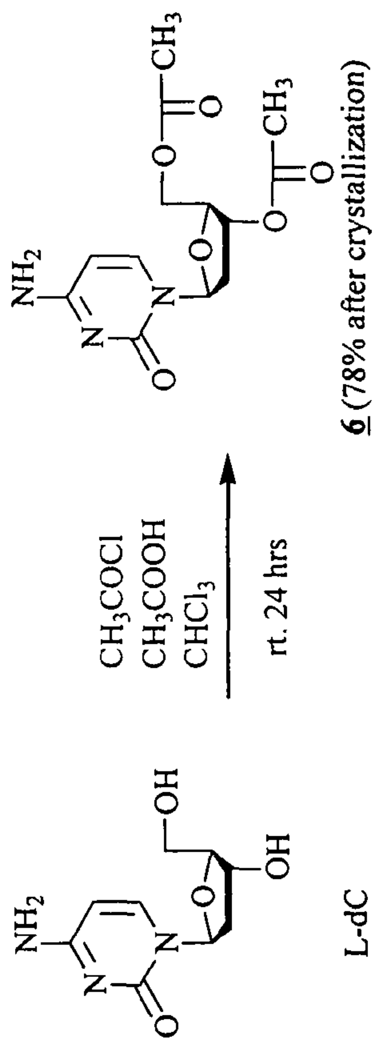
Figure 4 Synthesis of 3',5'-di- O -acetyl-2'-deoxy- \beta -L-cytidine
