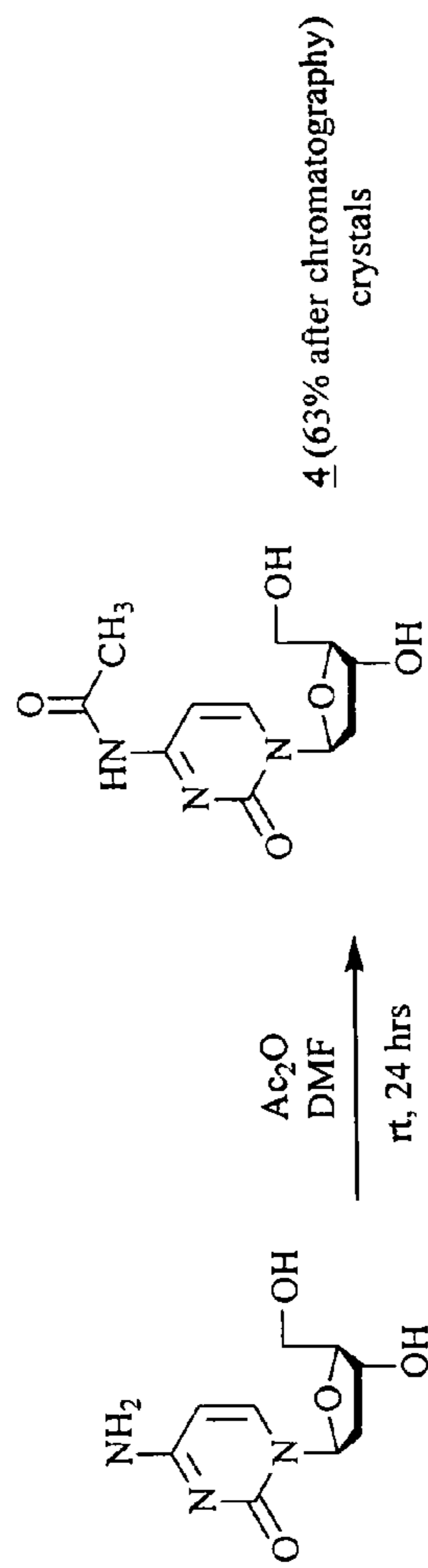
Figure 1 Synthesis of 5'-valinyl esters of 2'-deoxy-β-L-cytidine
