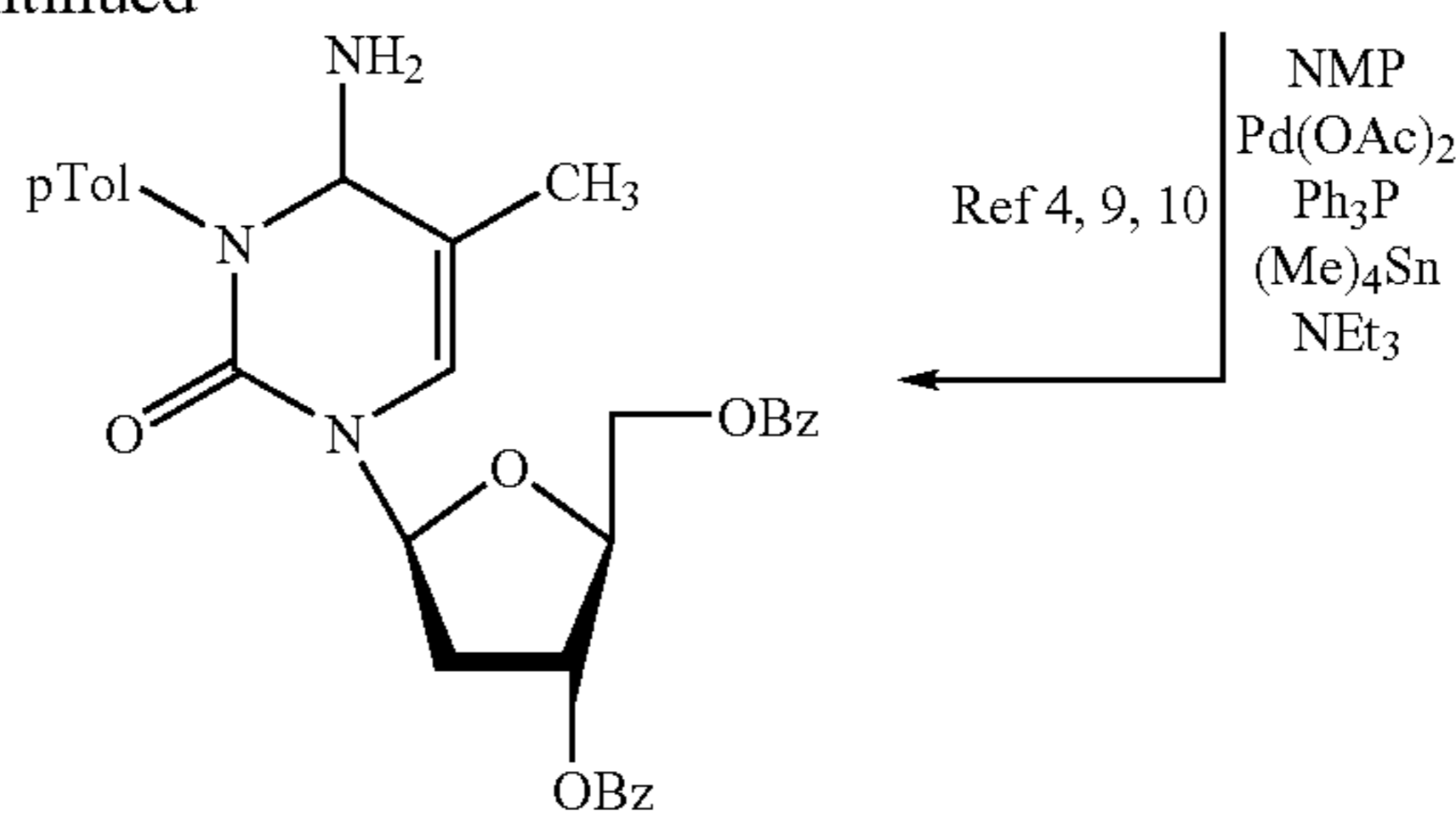
13 (48.3%, 2 steps) solid after purification
