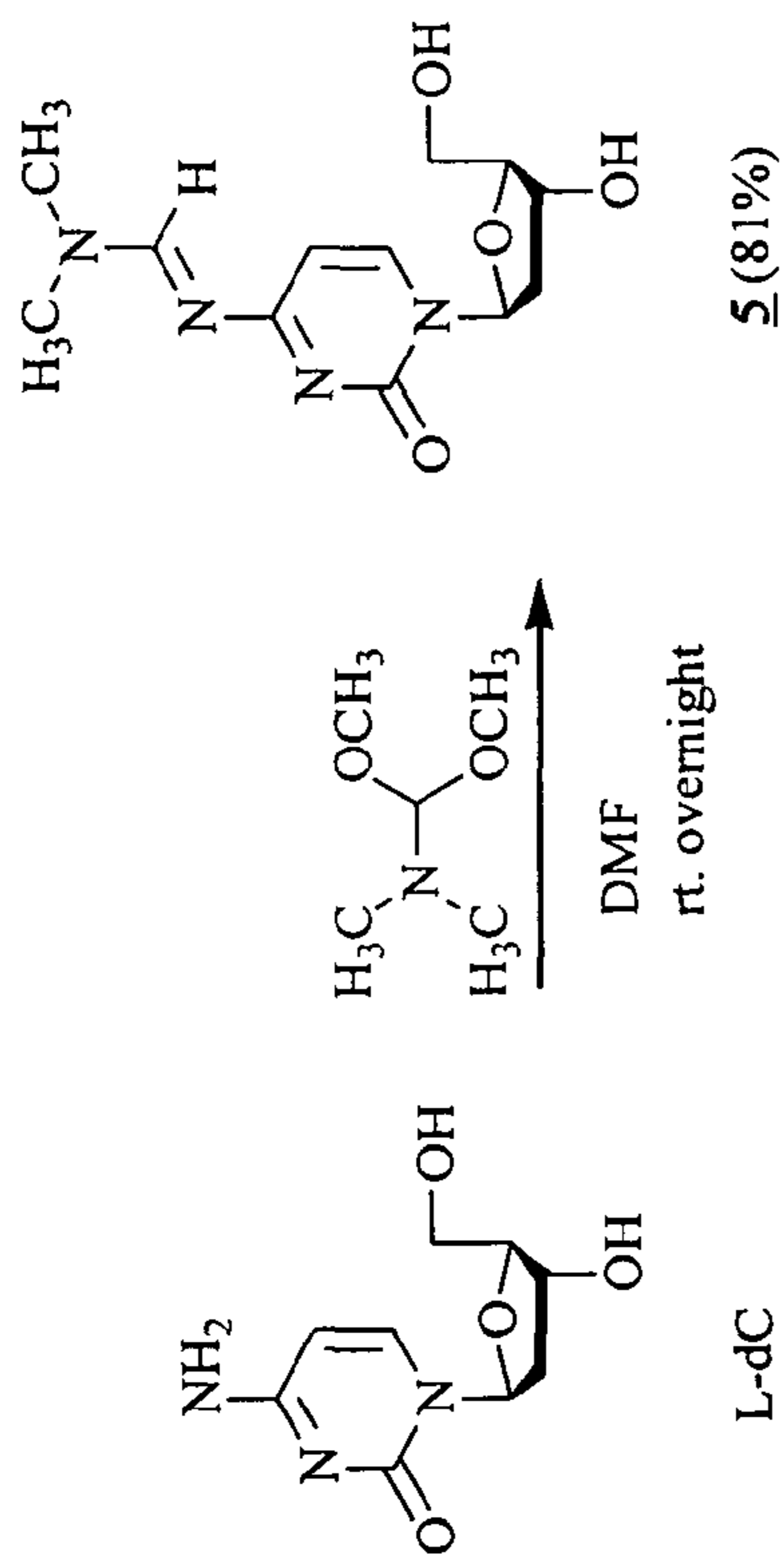
Figure 3 Synthesis of N 4 -[(dimethylamino)methylene]-2'-deoxy-β-L-cytidine
