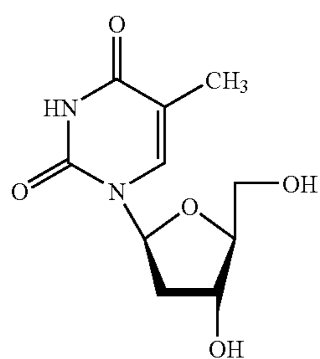
\beta -L-dT (64.8%) crystals after purification
