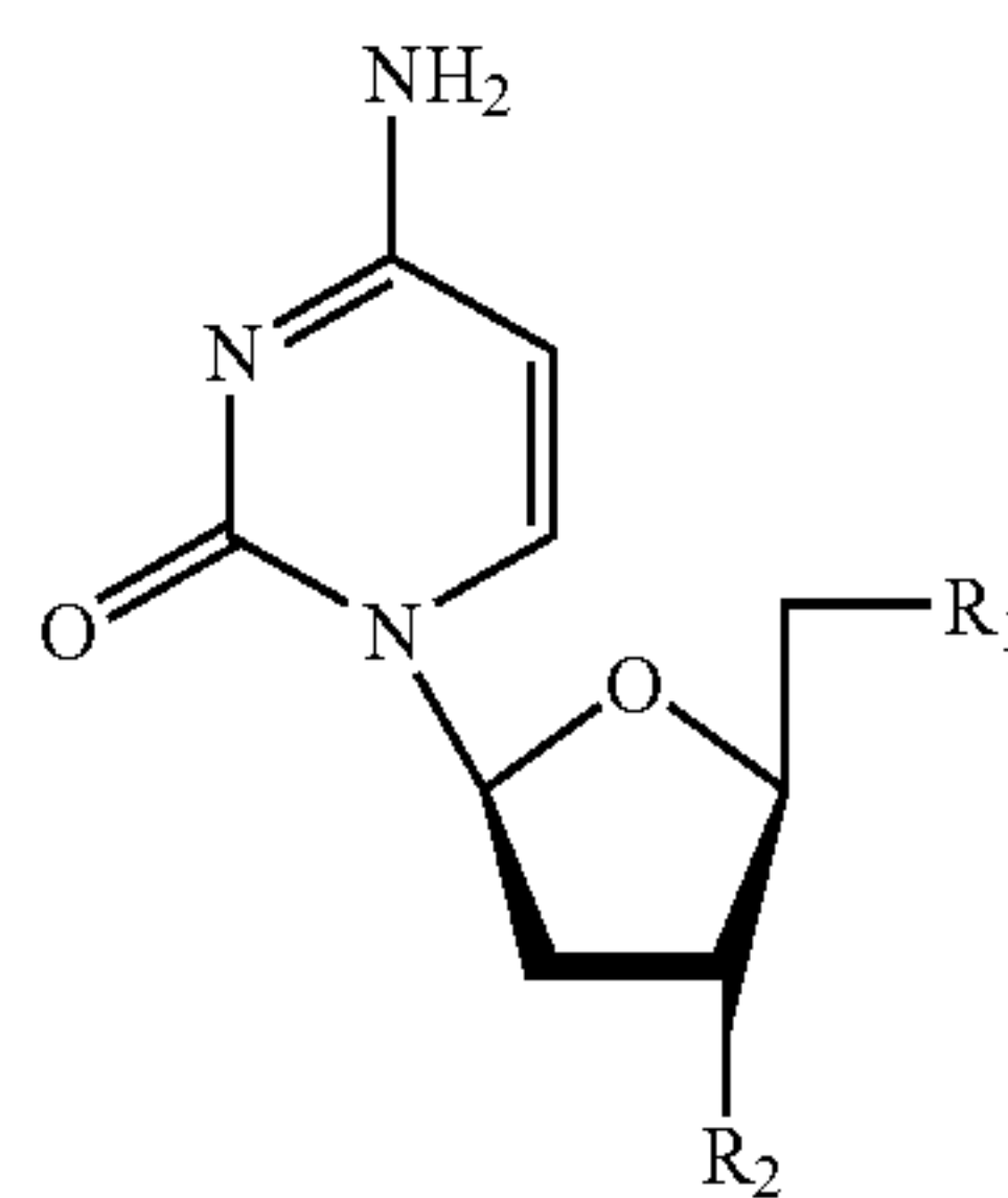
Scheme 5
