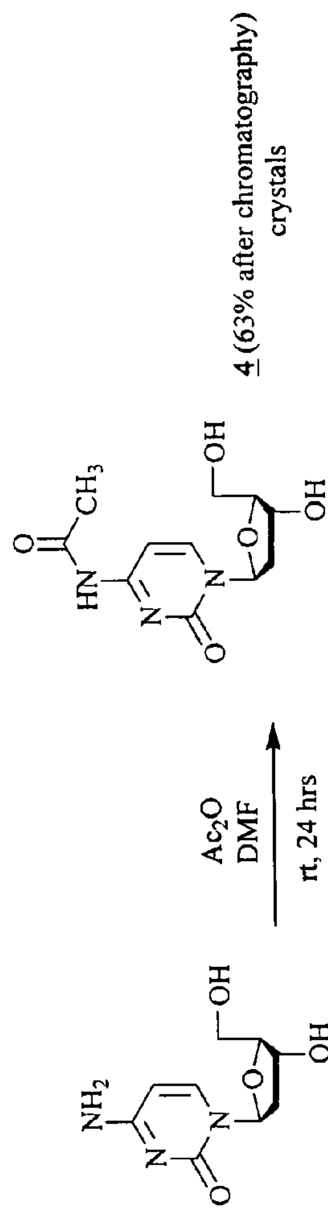
Figure 1 Synthesis of 5'-valinyl esters of 2'-deoxy-β-L-cytidine
