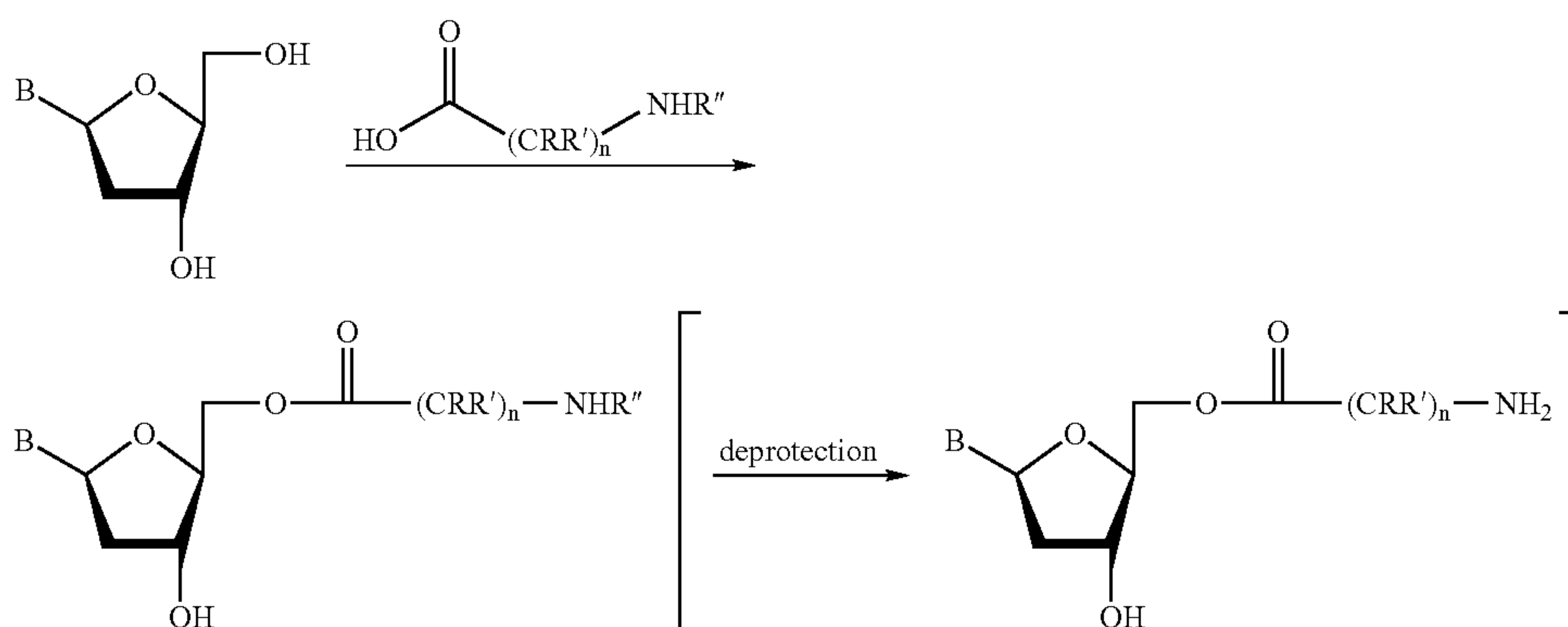
Scheme 1
