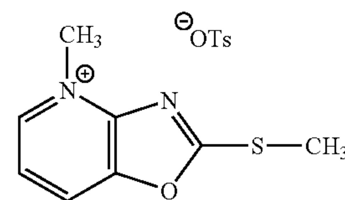
4-methyl-2-methylthioxazolo[4,5-b]pyridinium tosylate
