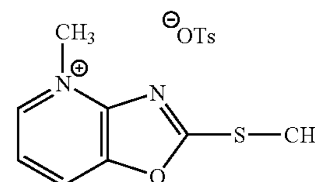
4-methyl-2-methylthioxazolo[4,5-b]pyridinium tosylate
