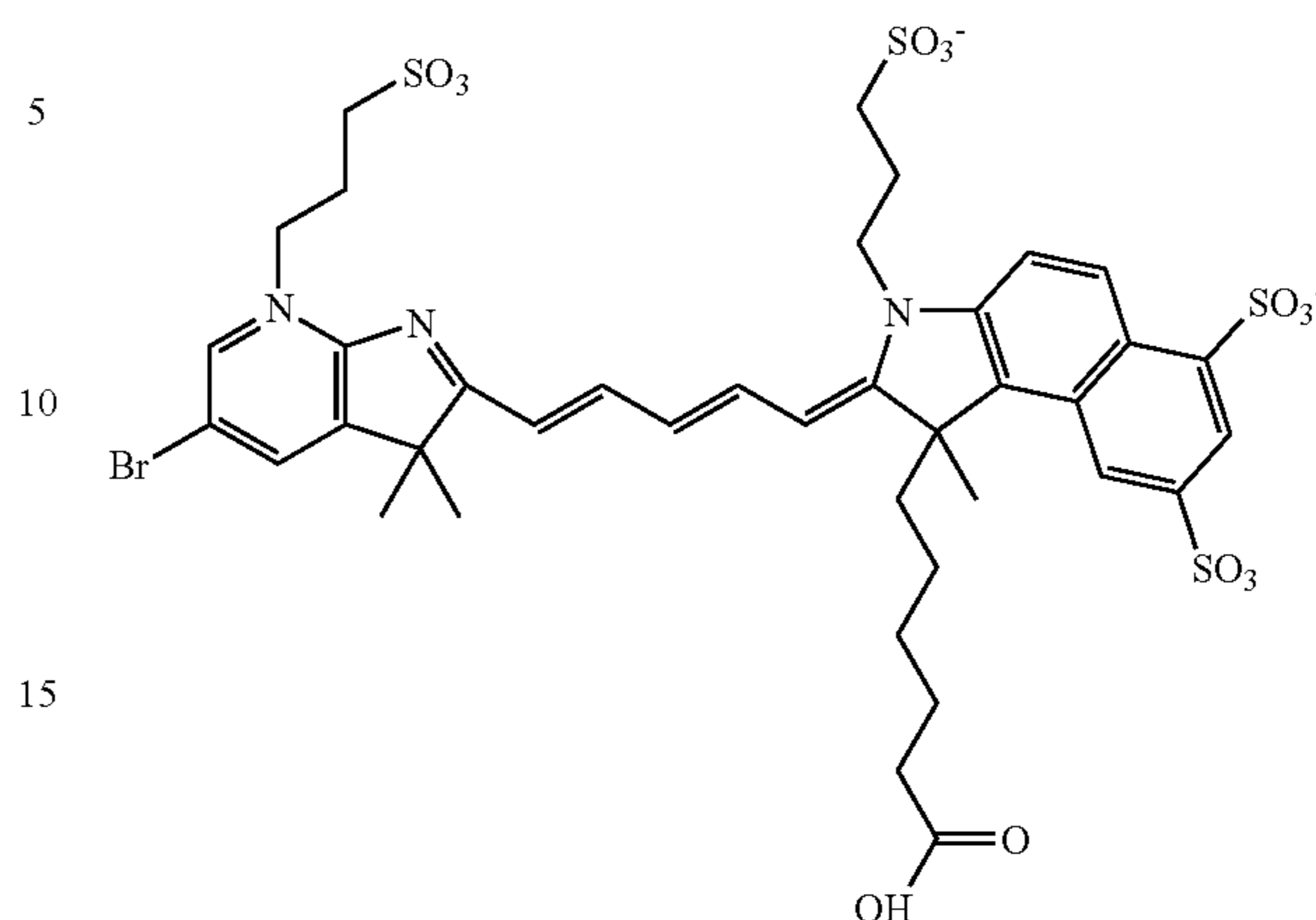
Compound 86
