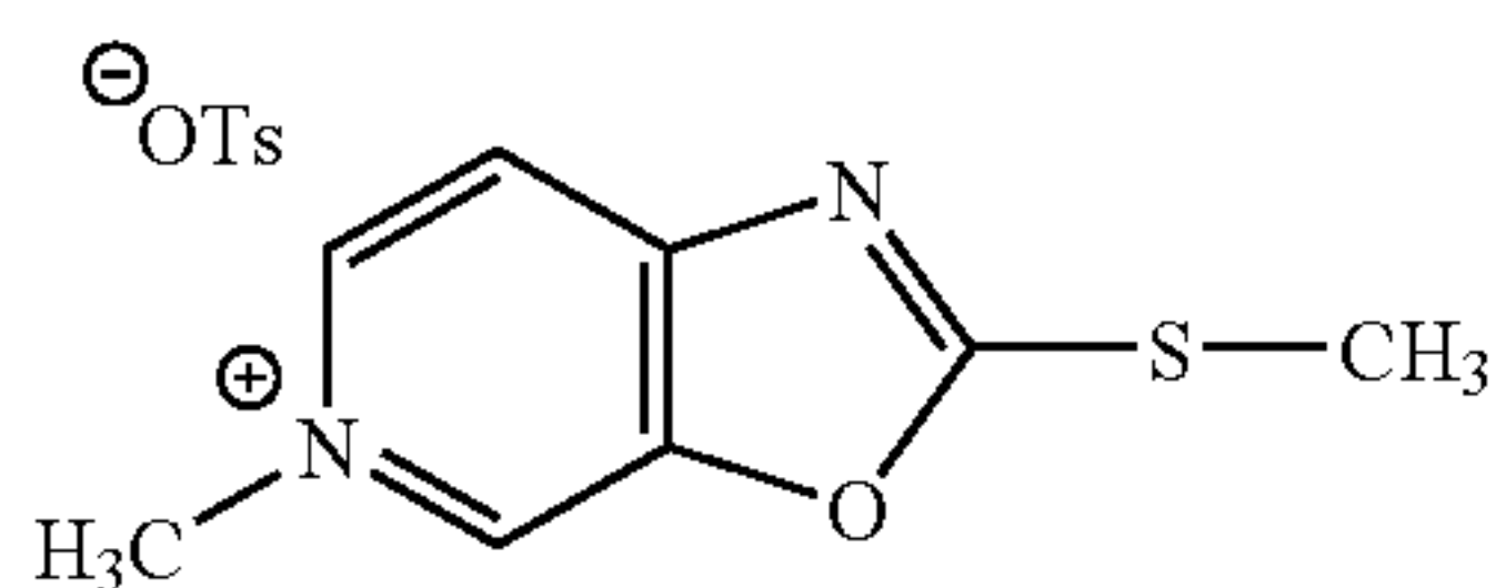
6-methyl-2-methylthioxazolo[5,4-c]pyridinium tosylate
