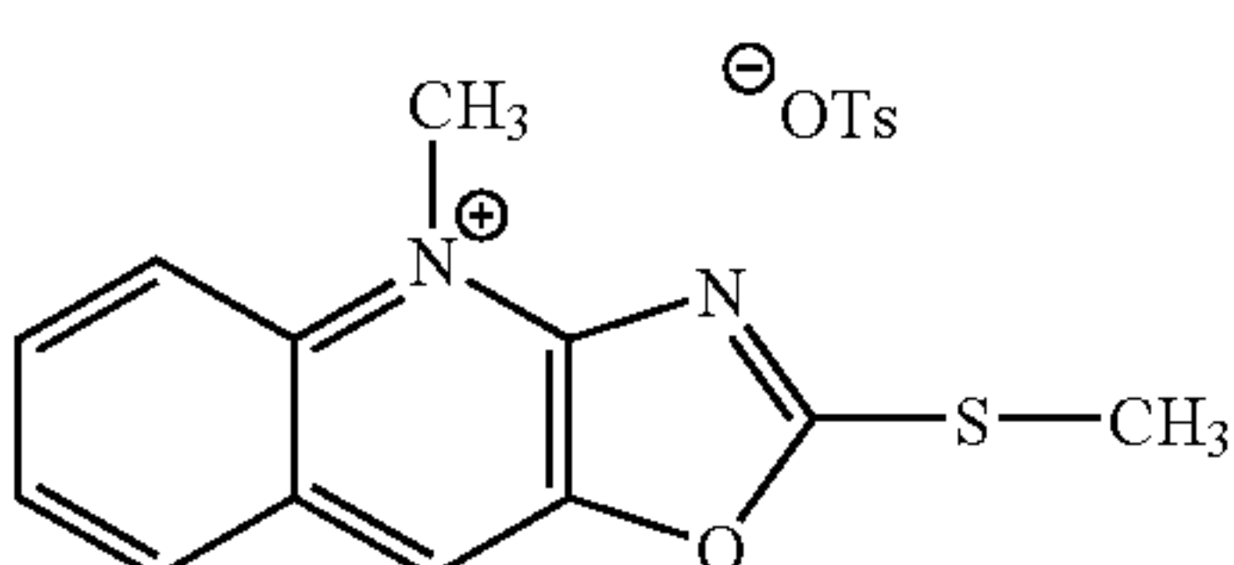
4-methyl-2-methylthioxazolo[4,5-b]quinolinium tosylate
