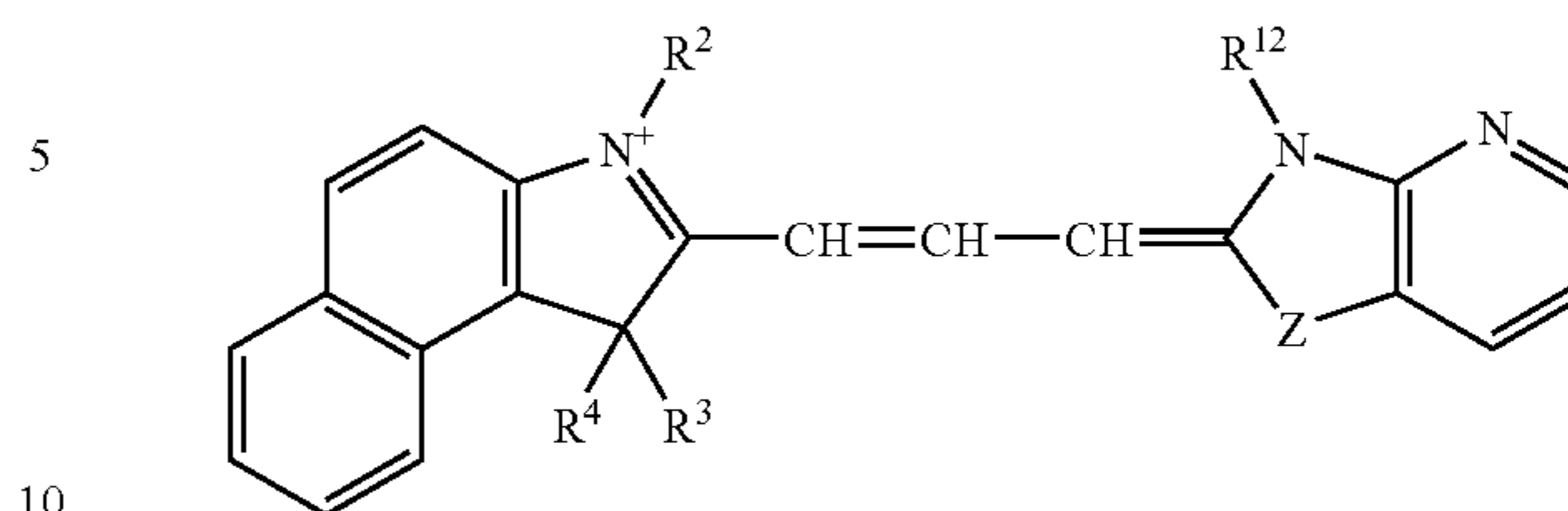
Formula XXIII
