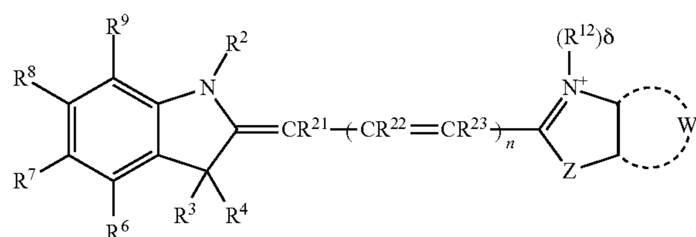
Formula XI
