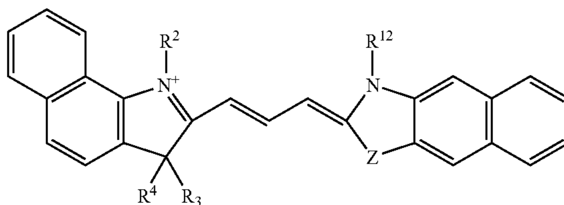
Formula XX
