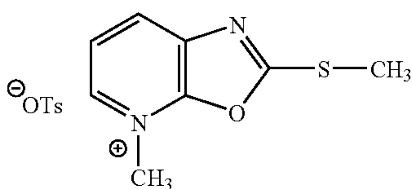
7-methyl-2-methylthioxazolo[5,4-b]pyridinium tosylate
