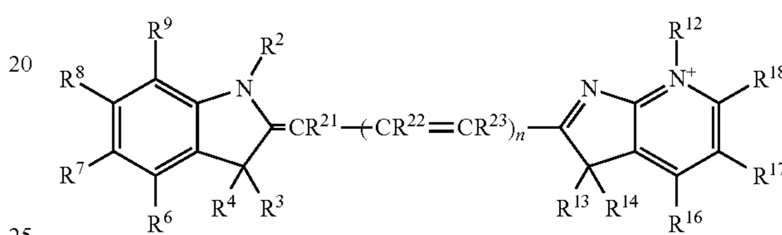
Formula XXII
