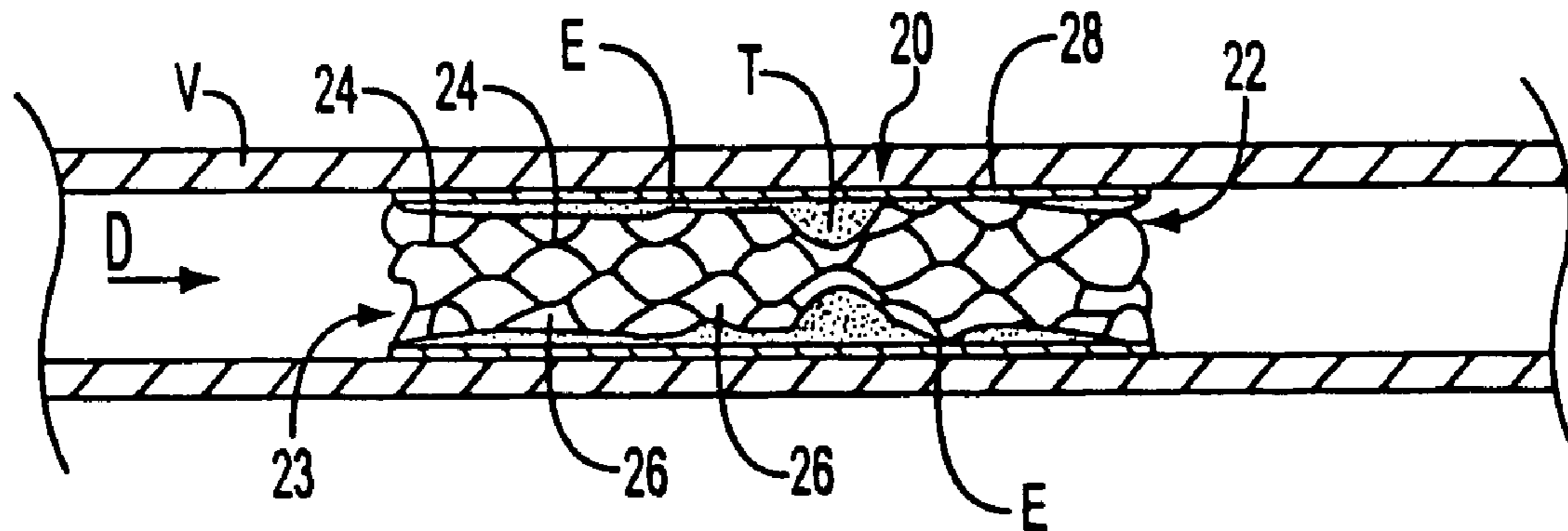
FIG. 7 (PRIOR ART)
