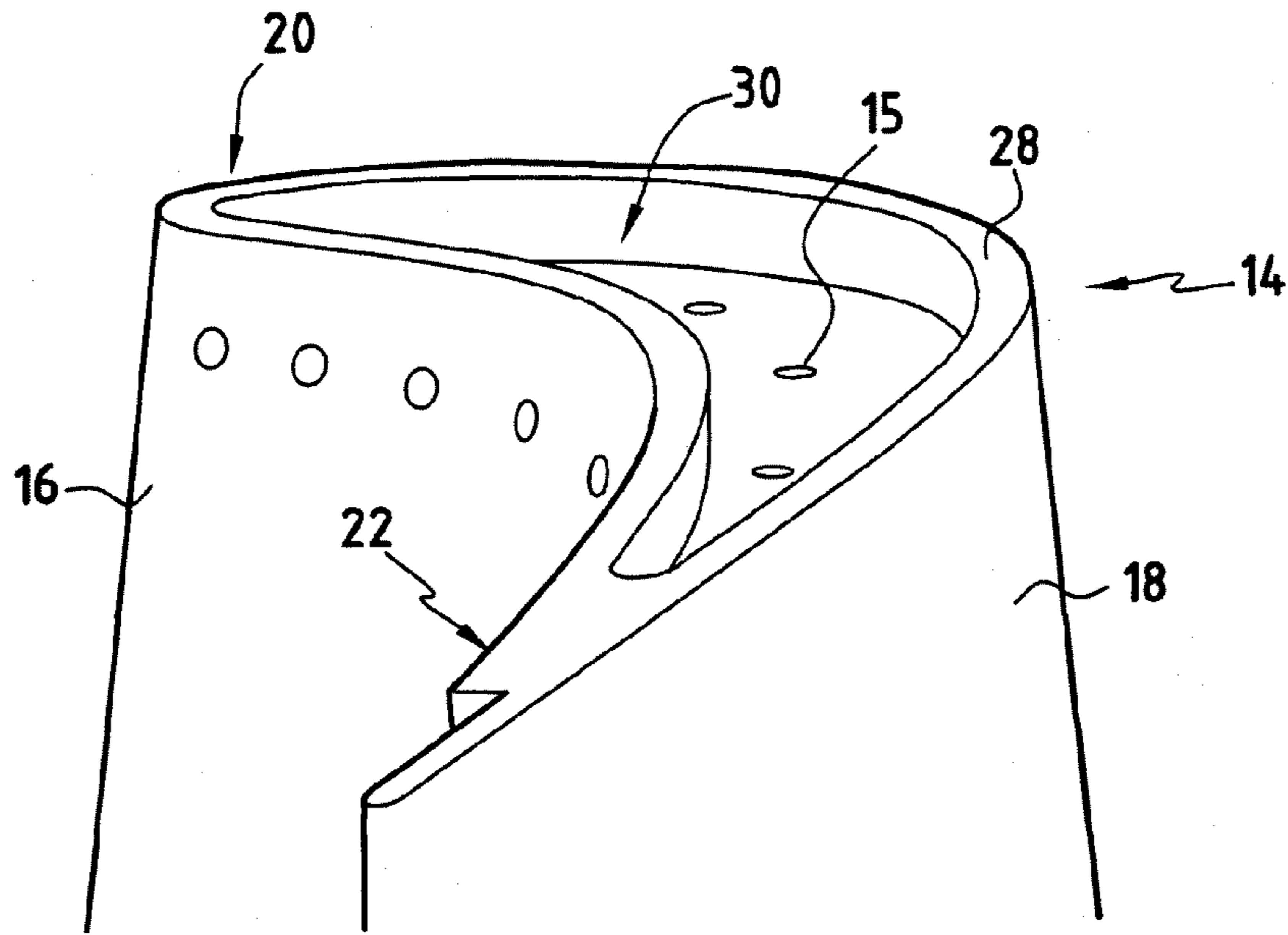
FIG. 2 PRIOR ART
