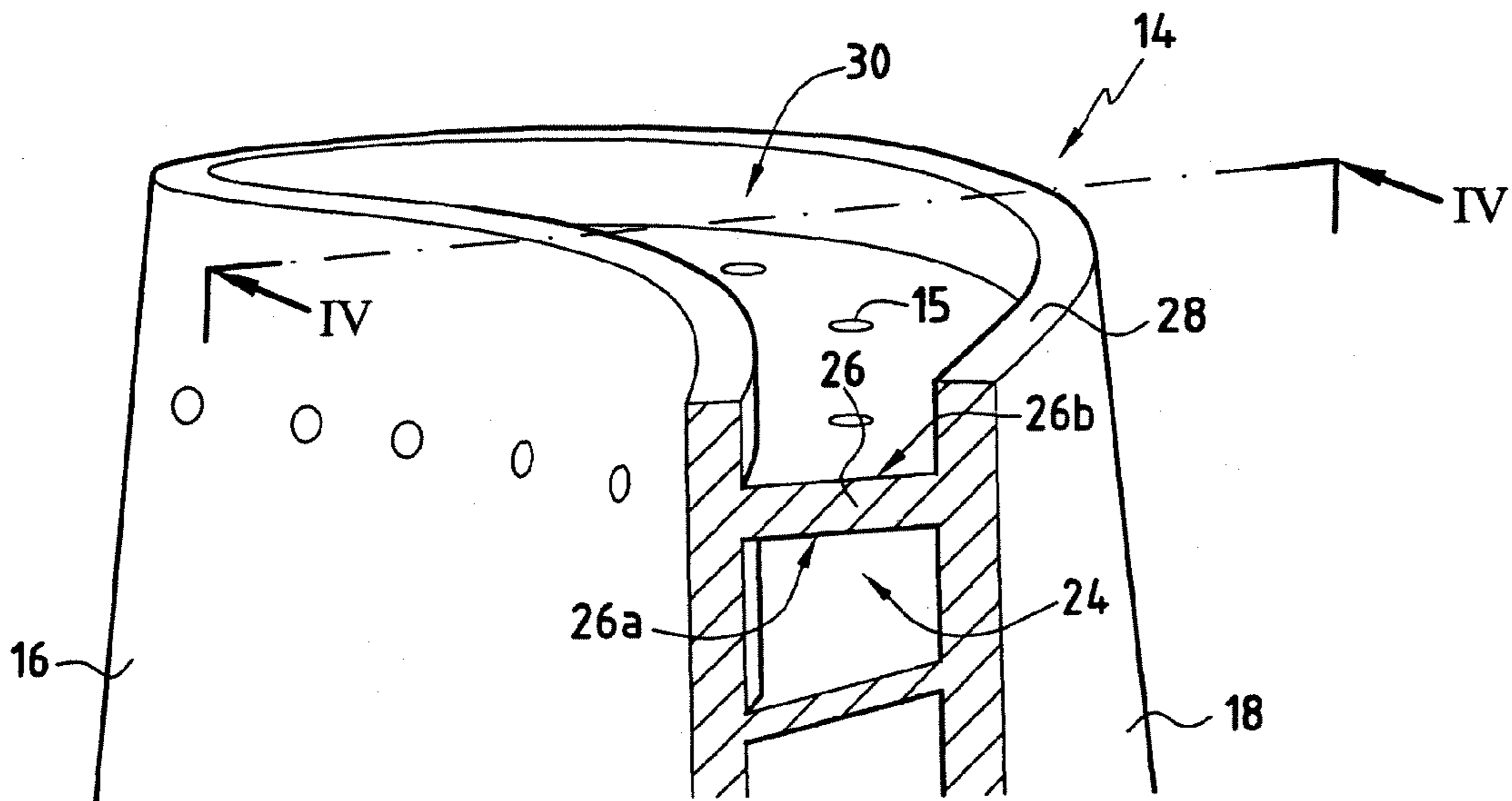
FIG. 3 PRIOR ART
