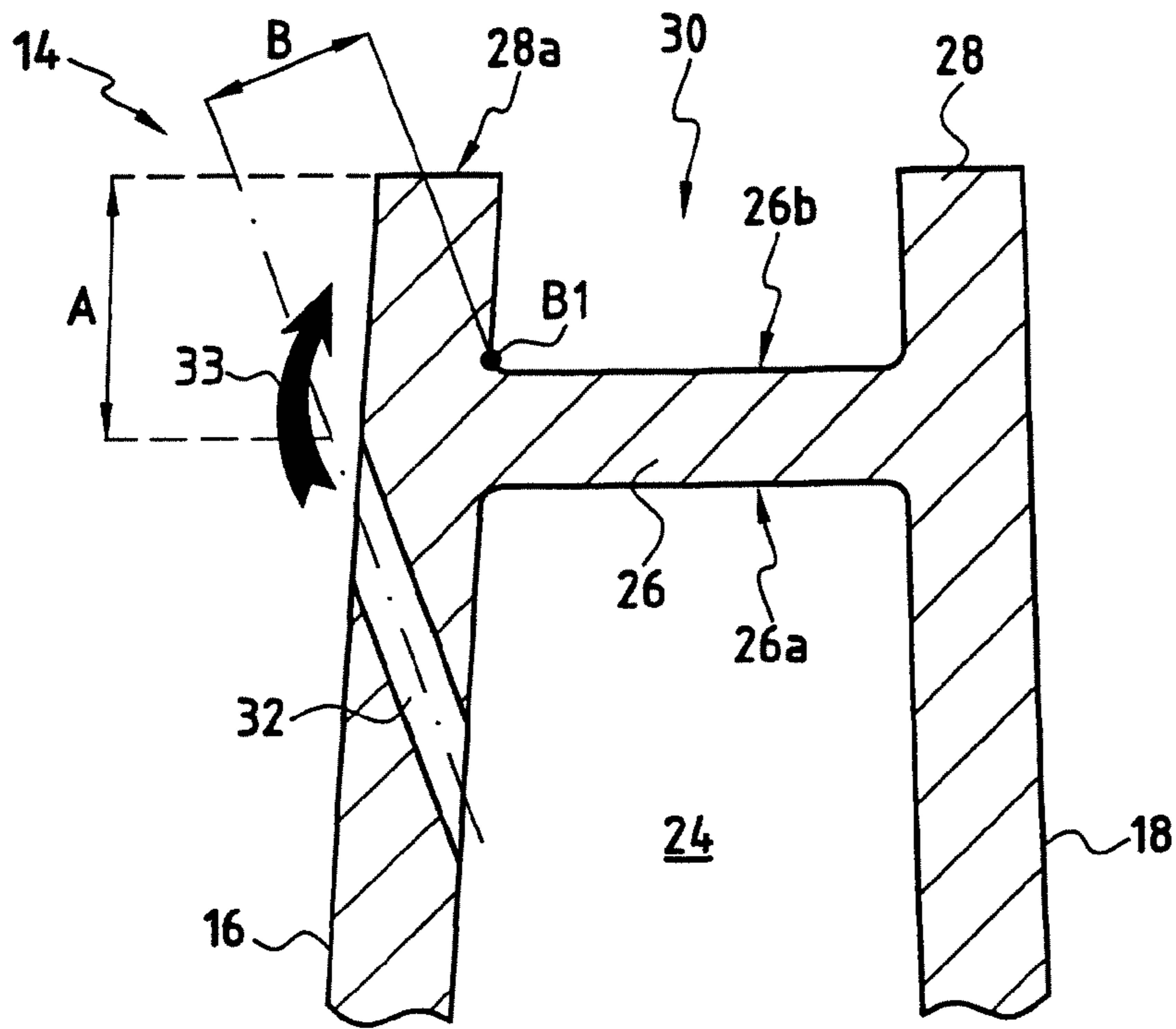
FIG. 4 PRIOR ART
