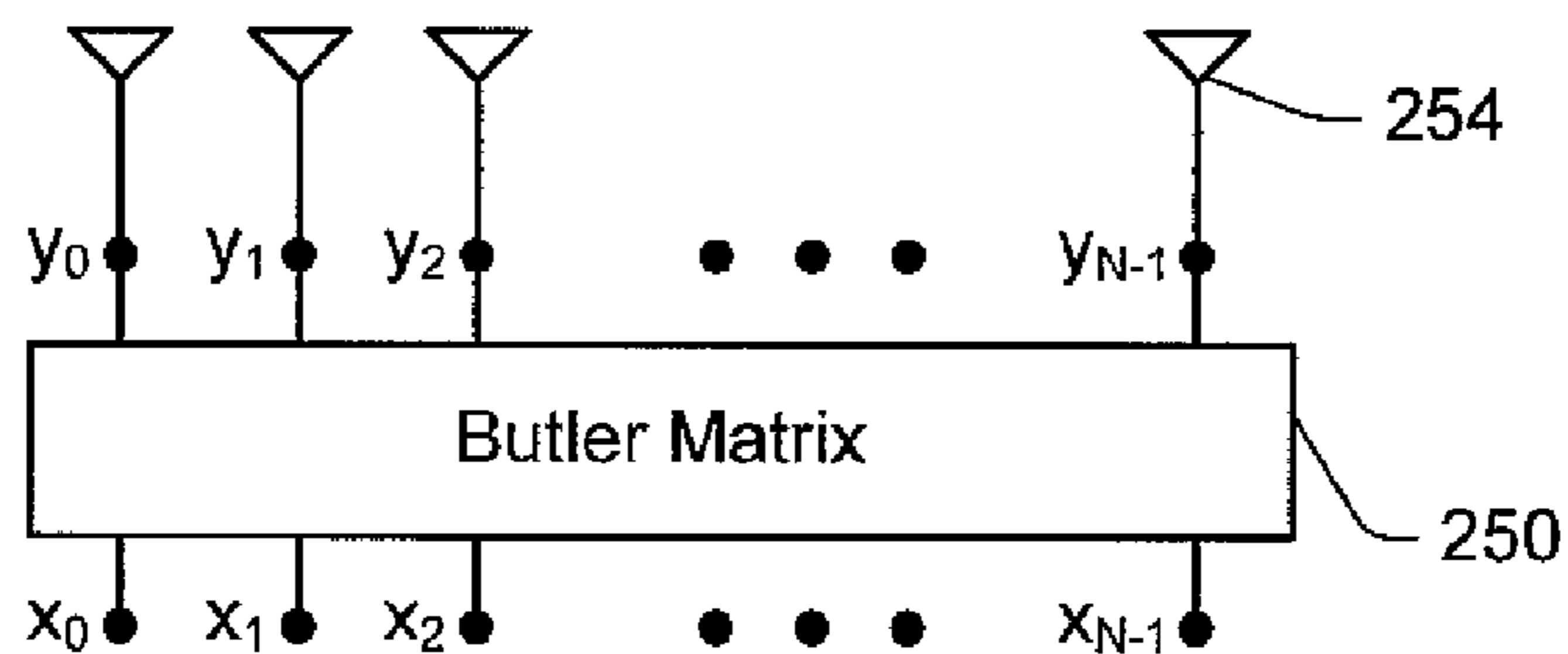
Fig. 4 (Prior Art)
