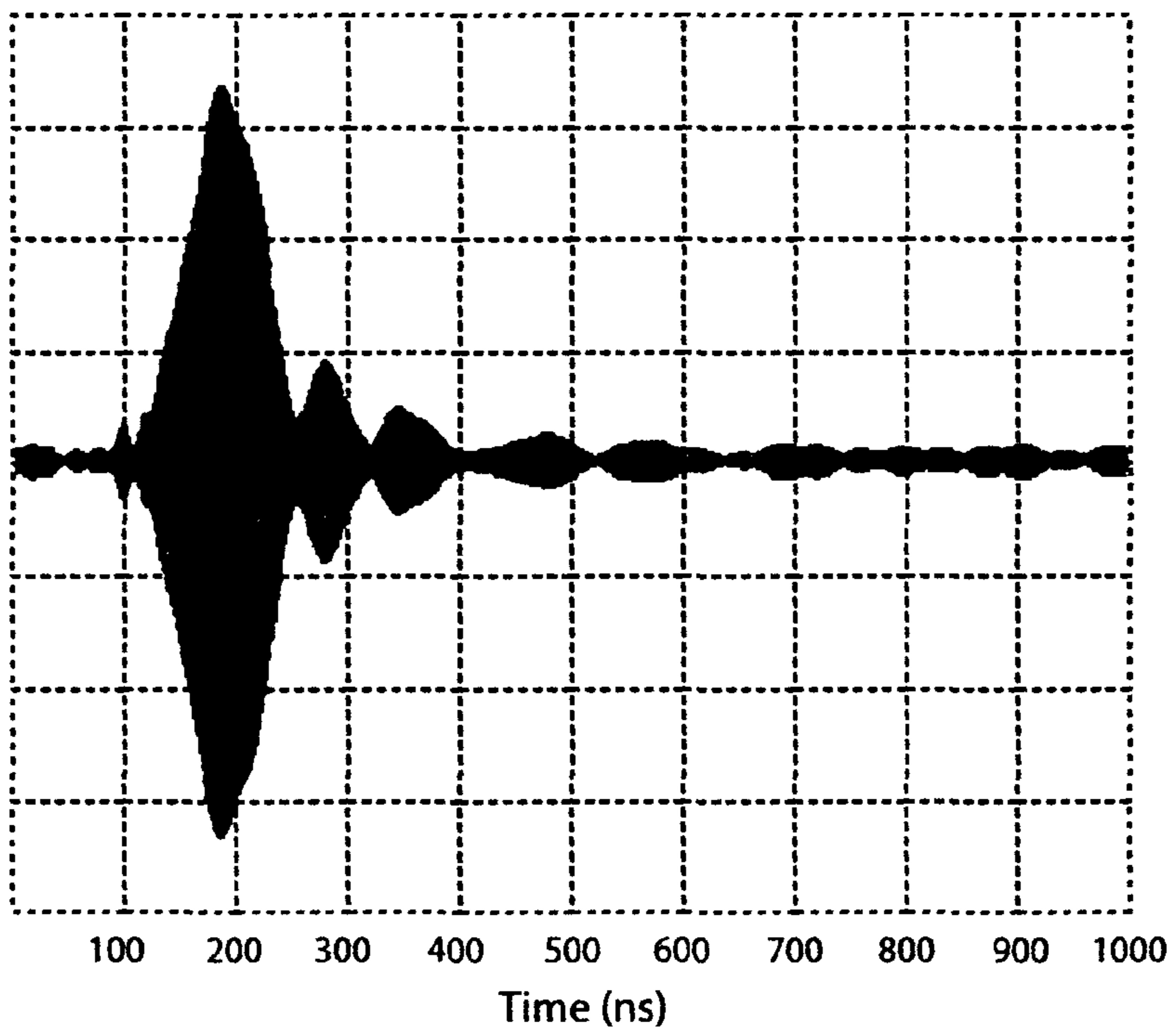
Output response of the 14MHz SAW filter
