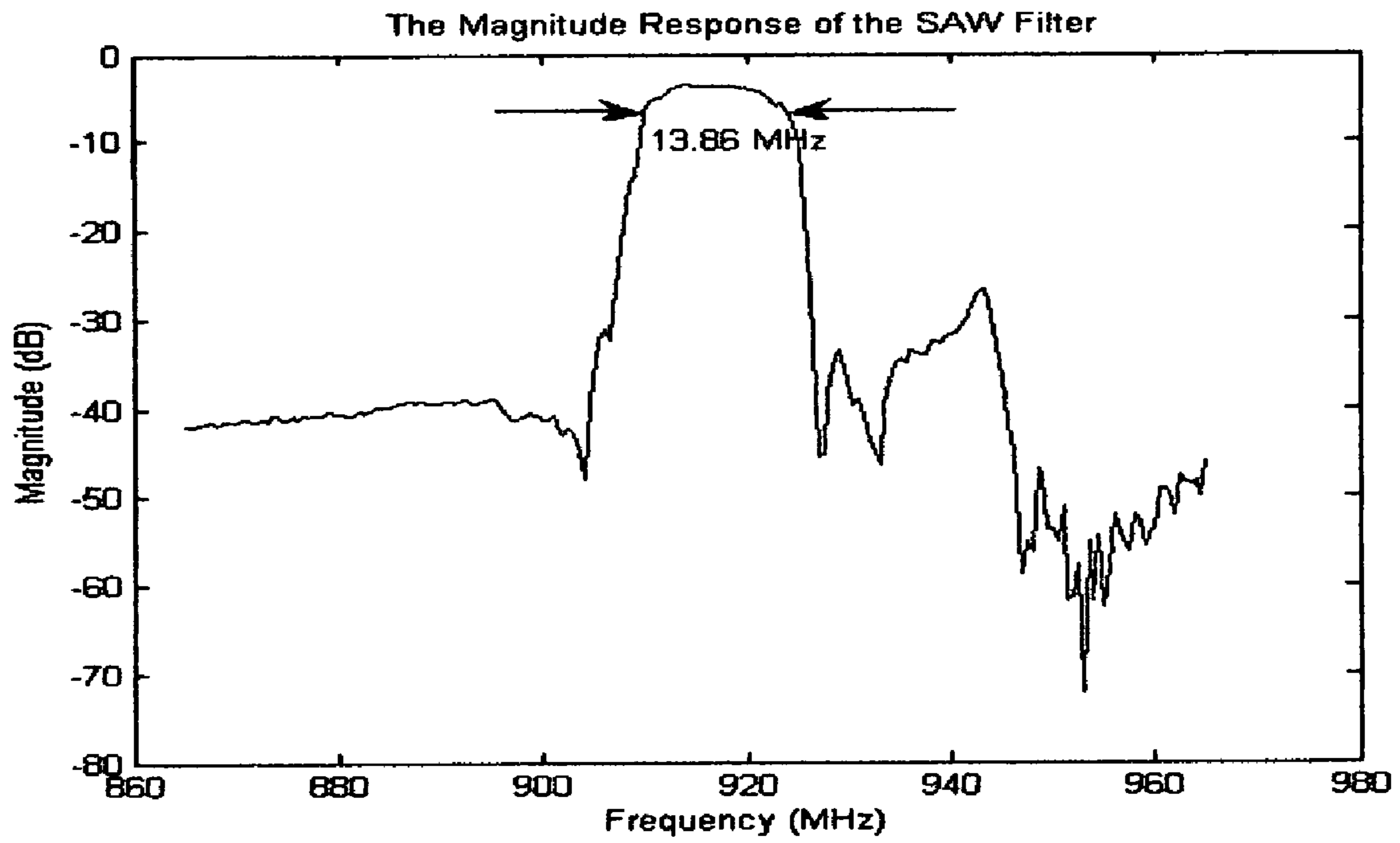
Frequency response of SAW filter
