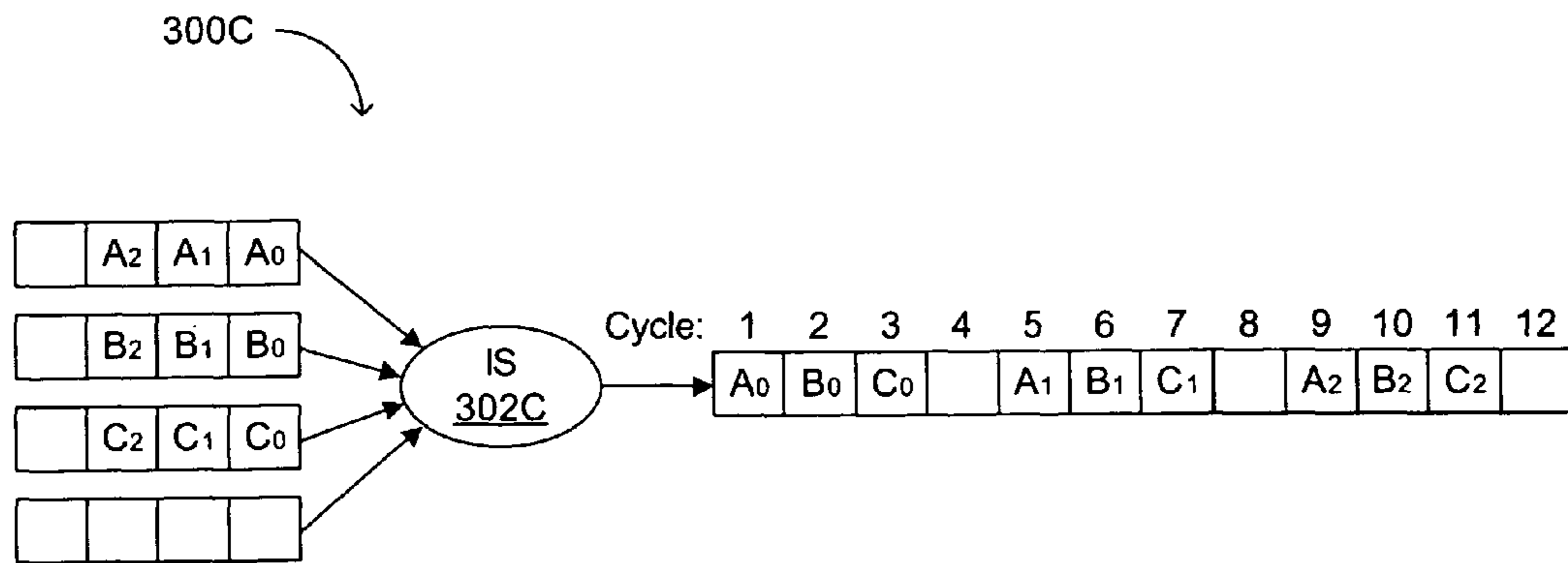
FIG. 3C (conventional)
