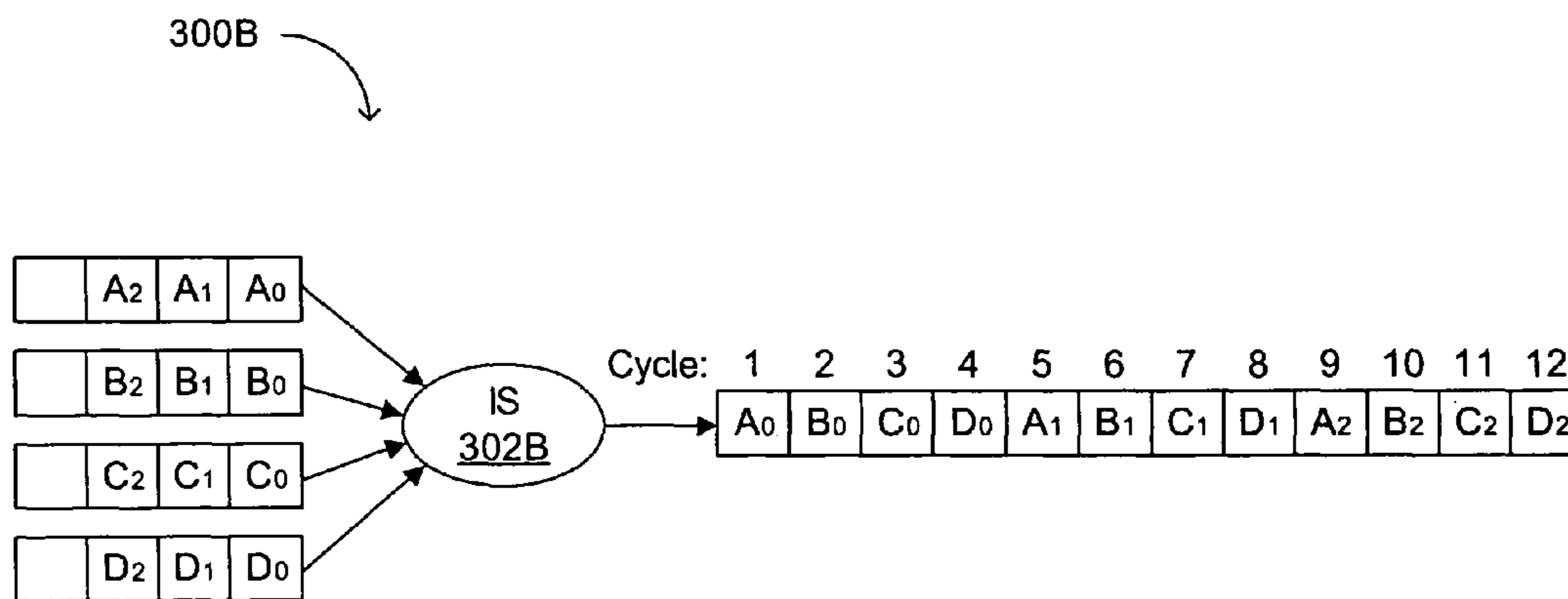
FIG. 3B (conventional)
