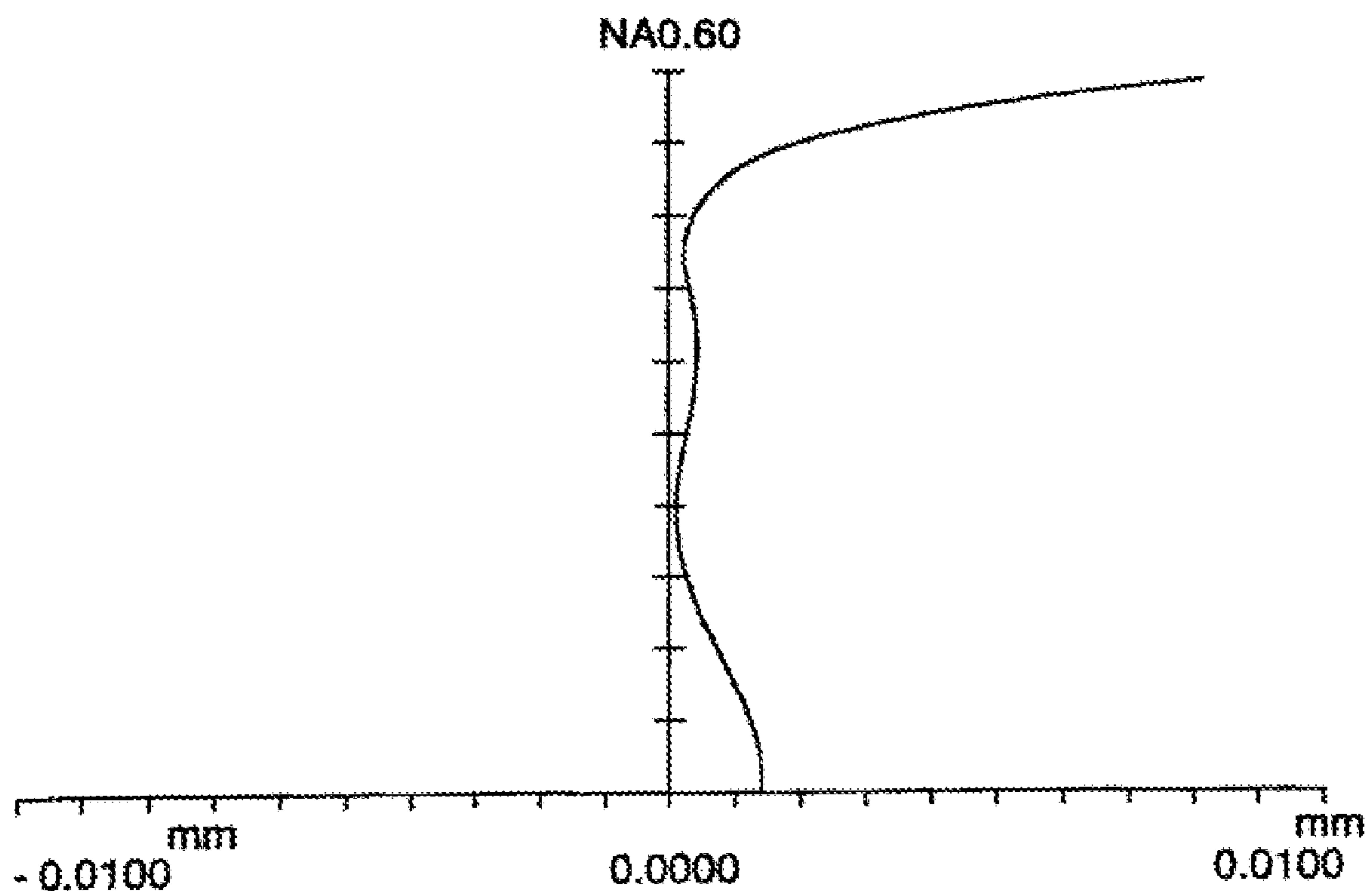
DIAGRAM SHOWING SPHERICAL ABERRATION FOR WAVELENGTH \lambda = 780\text{nm} (NA0.60) IN EXAMPLE 7
