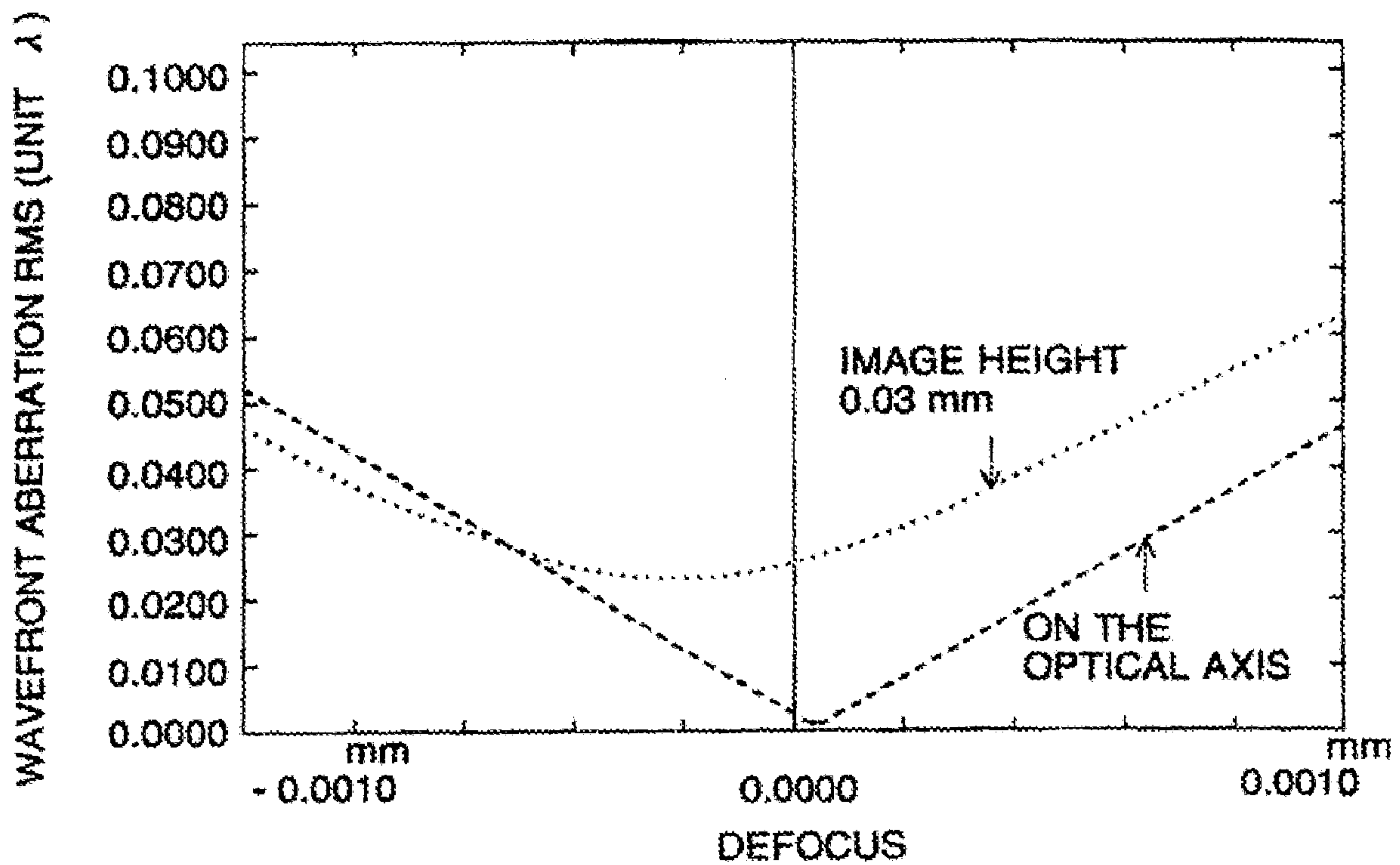
DIAGRAM SHOWING WAVEFRONT ABERRATION RMS FOR WAVELENGTH \lambda = 780\text{nm} (NA0.5) IN EXAMPLE 6
