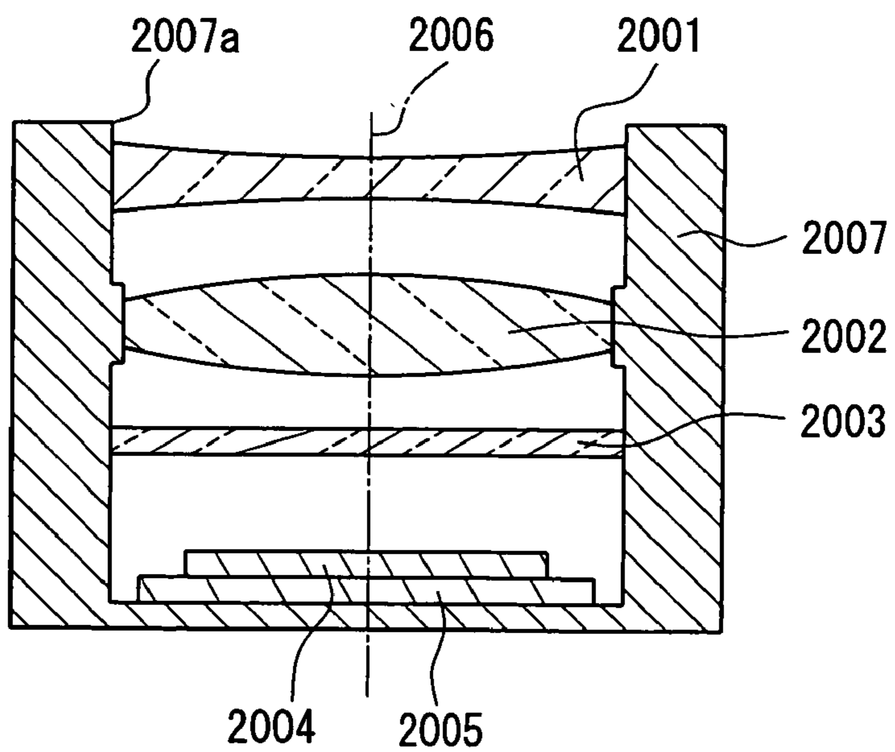
FIG. 33 PRIOR ART
