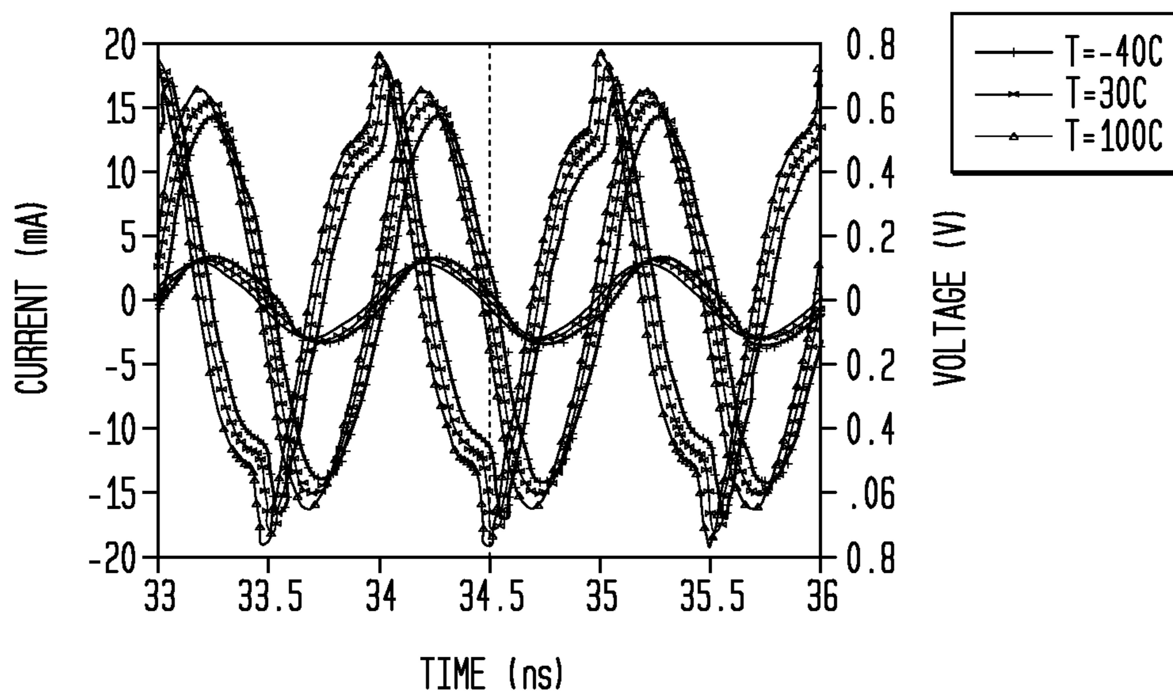
TEMPERATURE/BIAS DEPENDENCE
