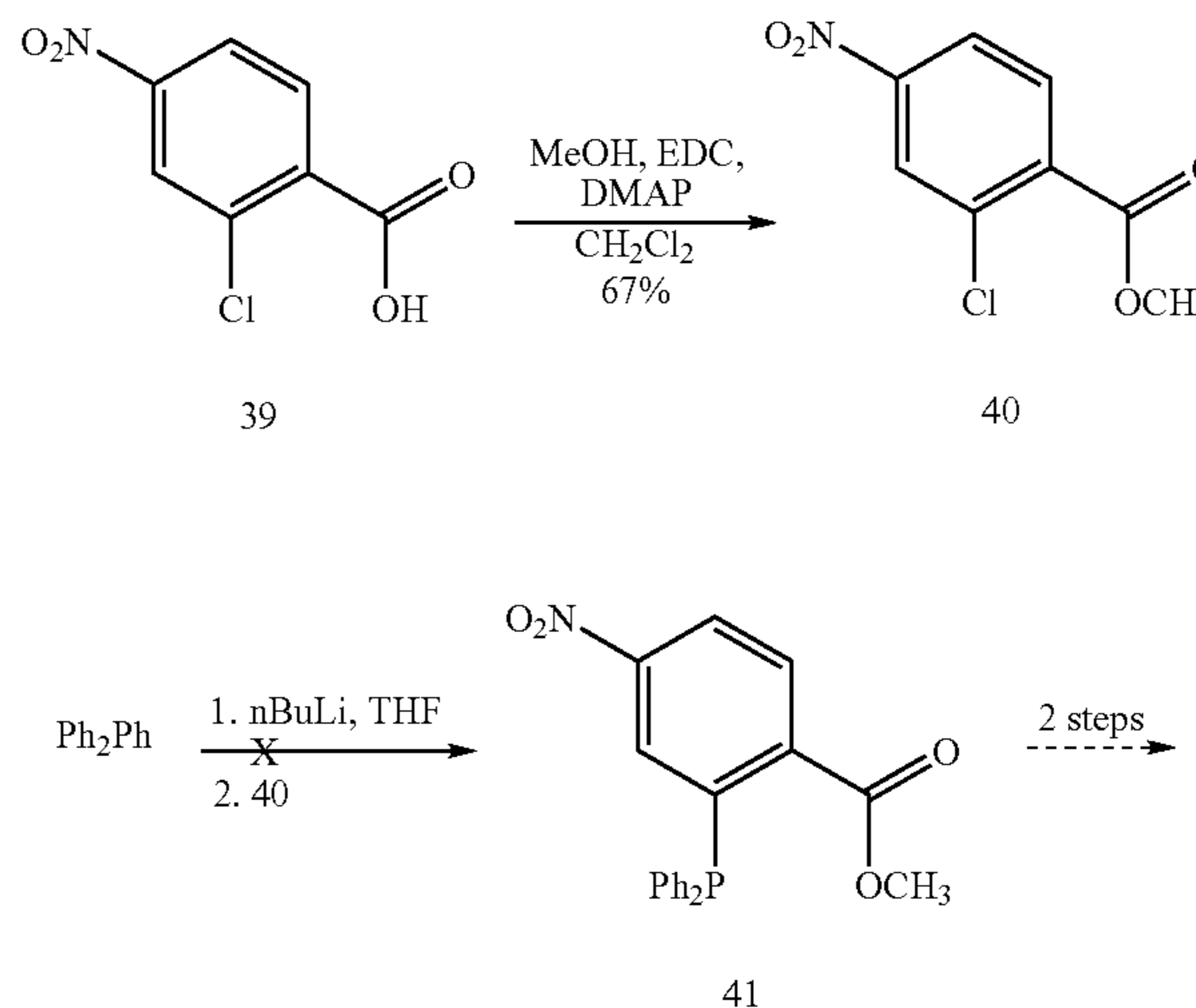
Scheme 12
