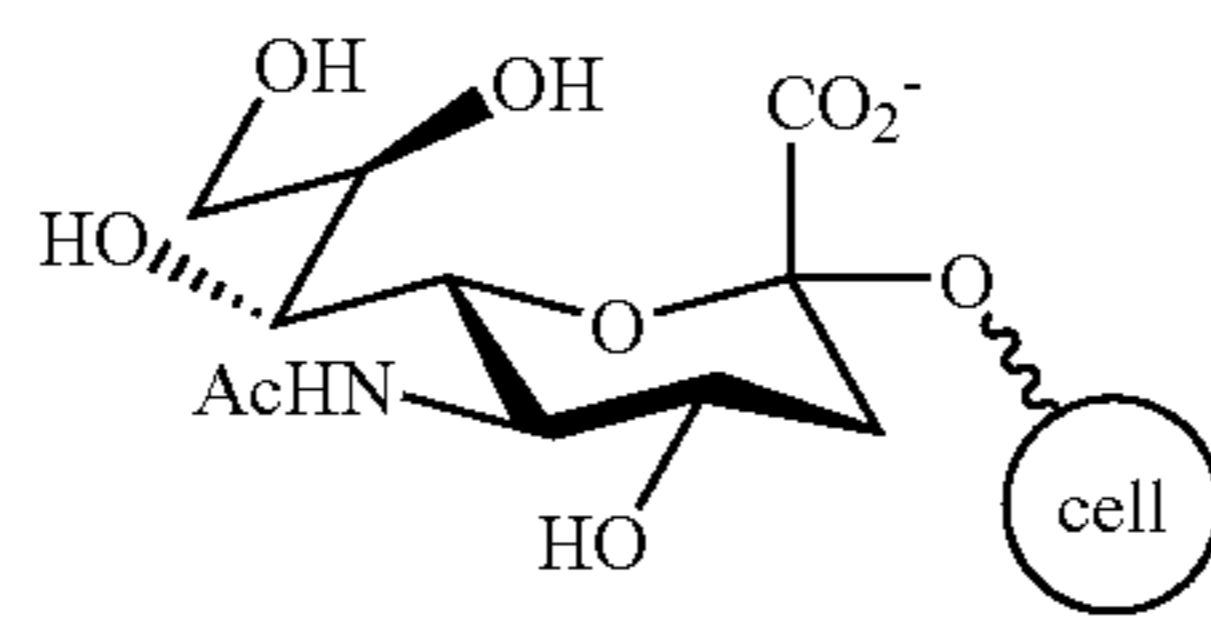
Sialic Acid 2
