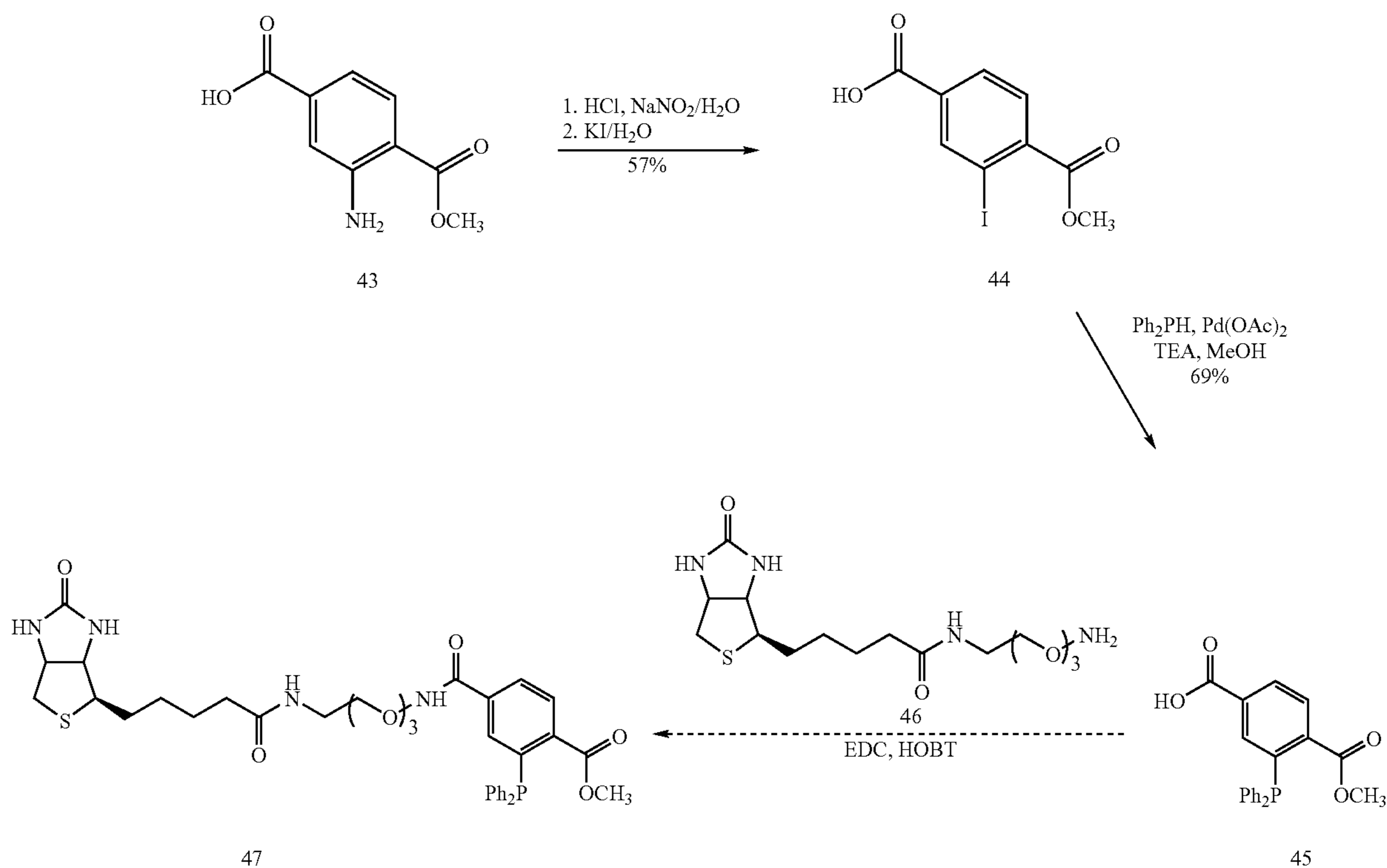
Scheme 13
