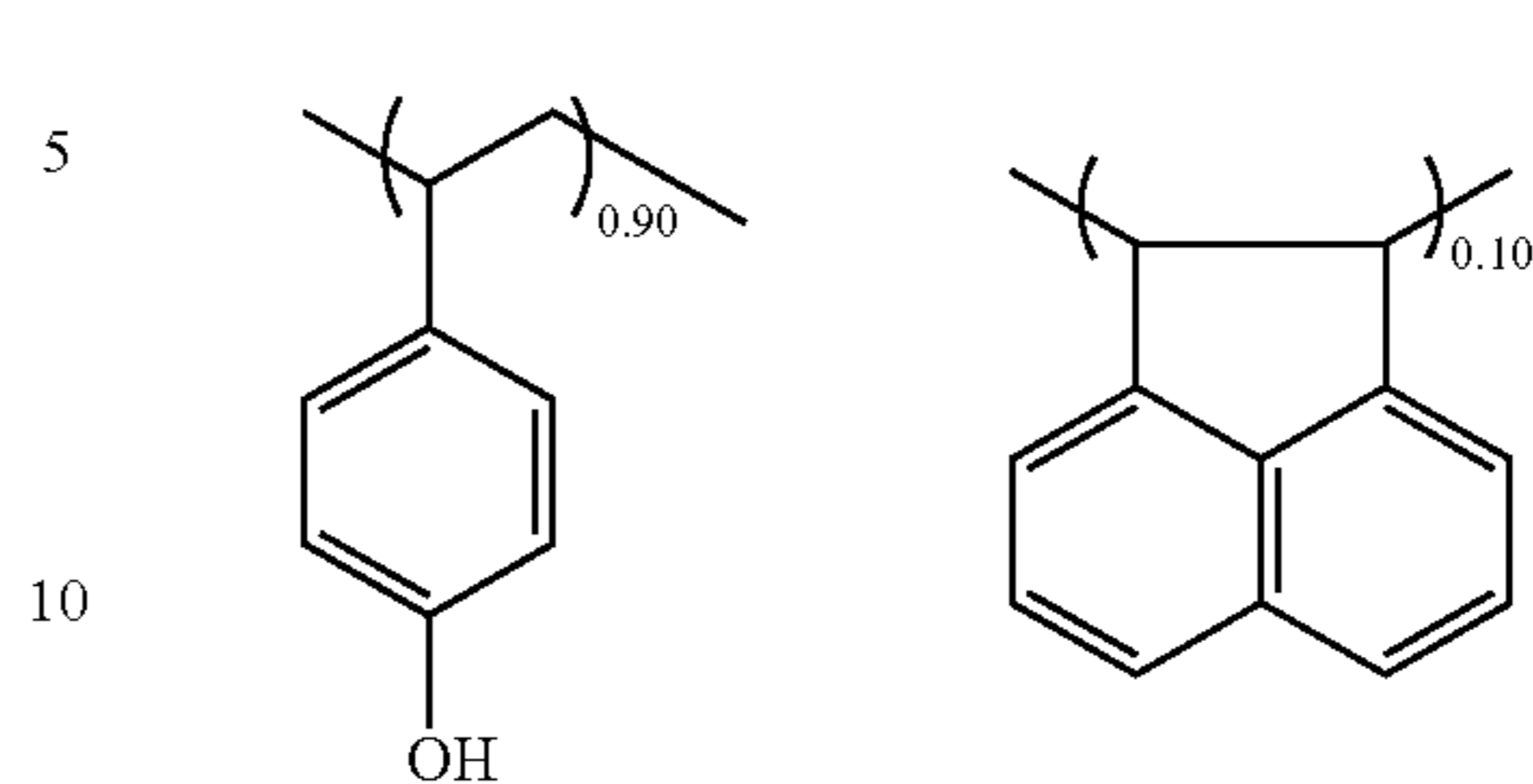
Synthetic Example 6
