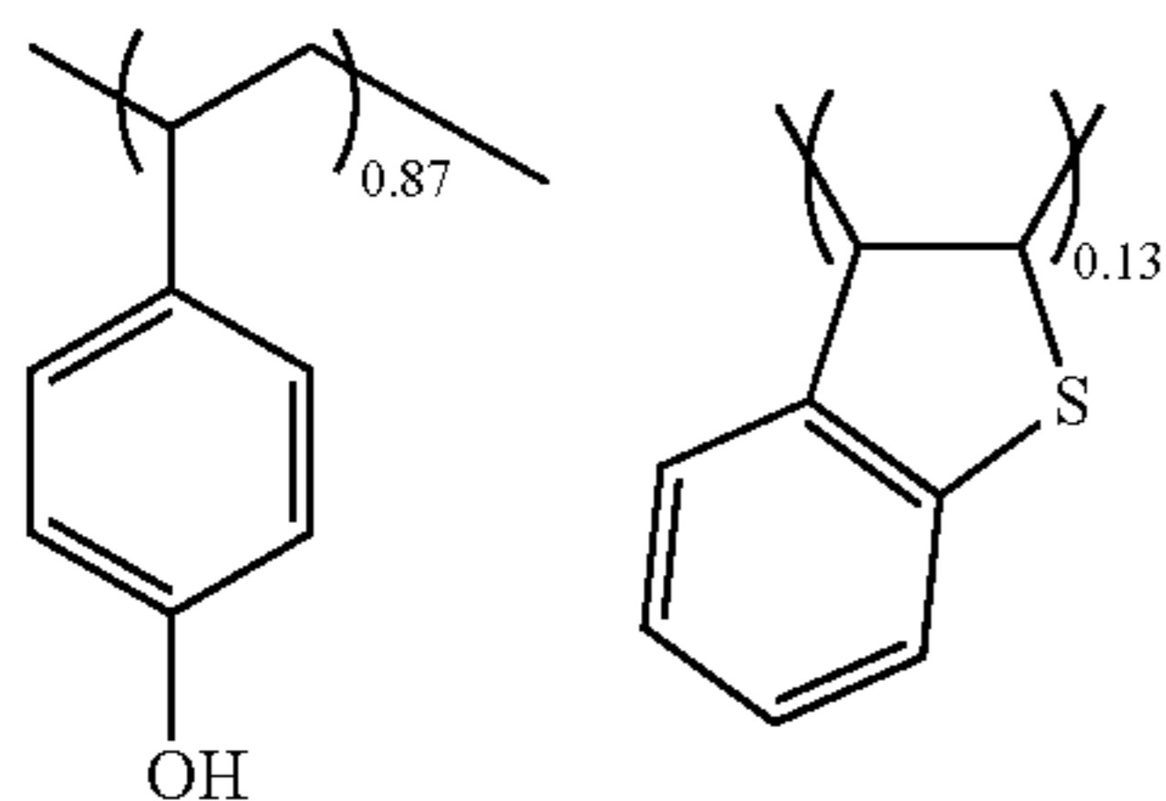
Synthetic Example 5
