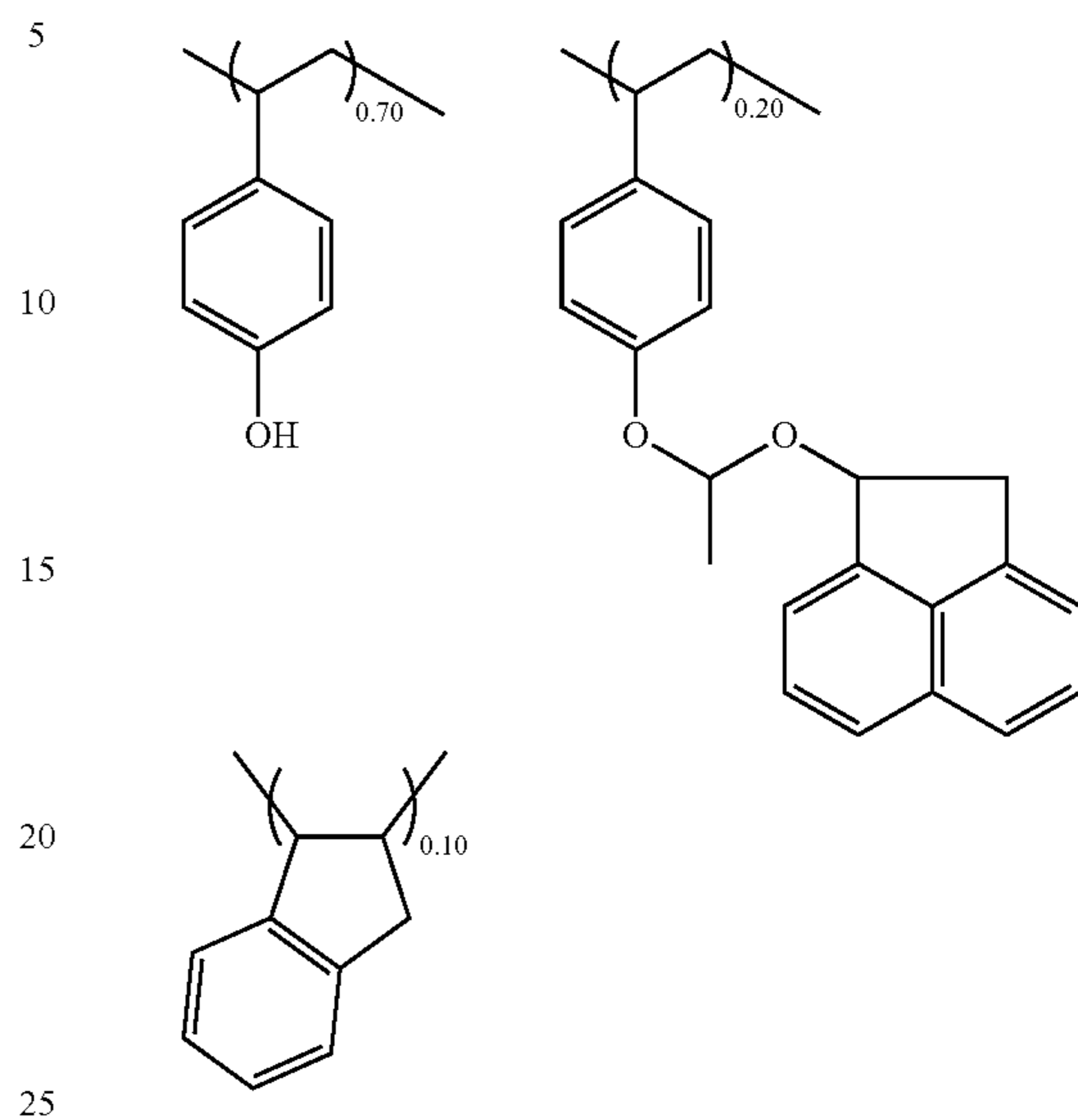
Synthetic Example 15
