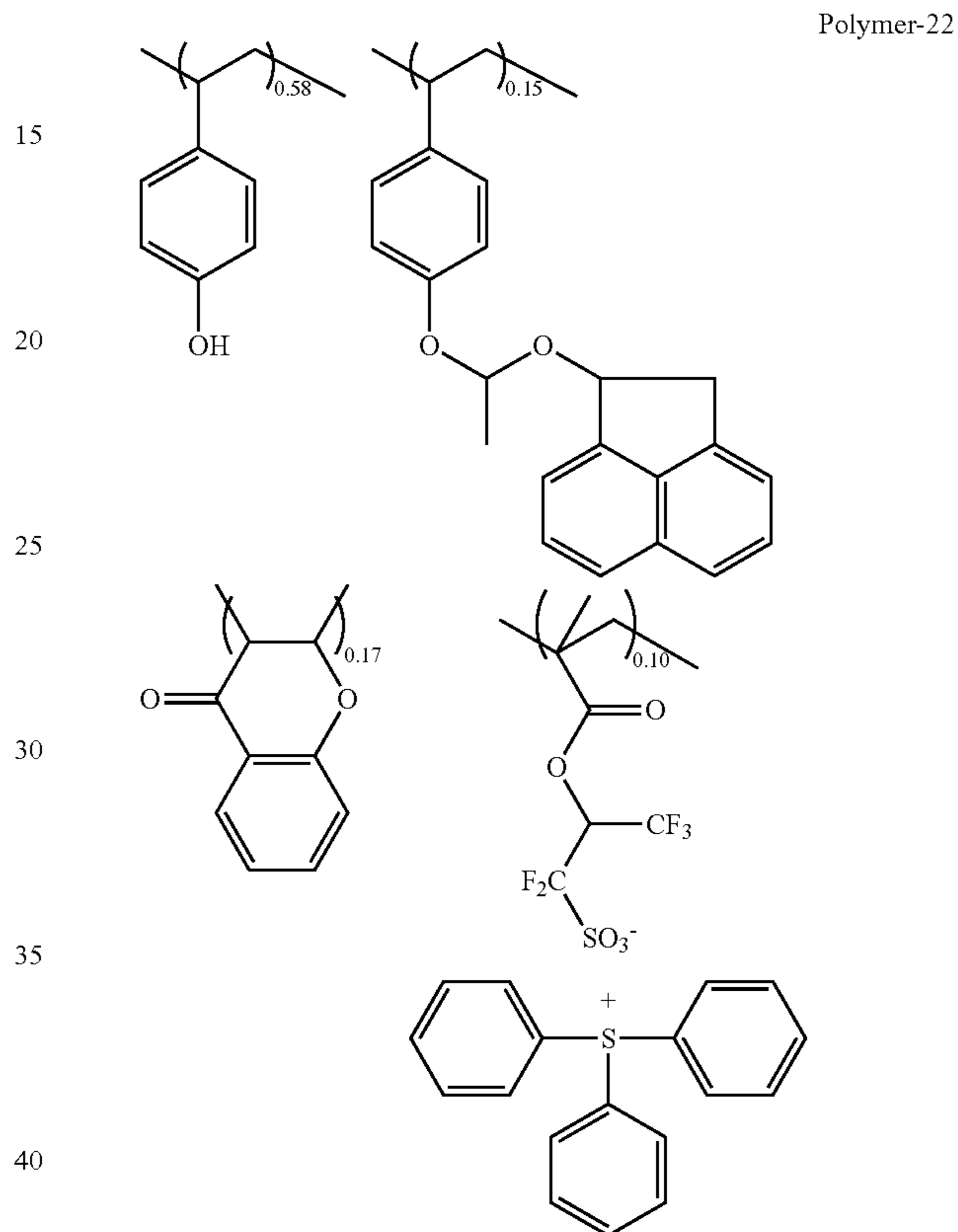
Synthetic Example 23
