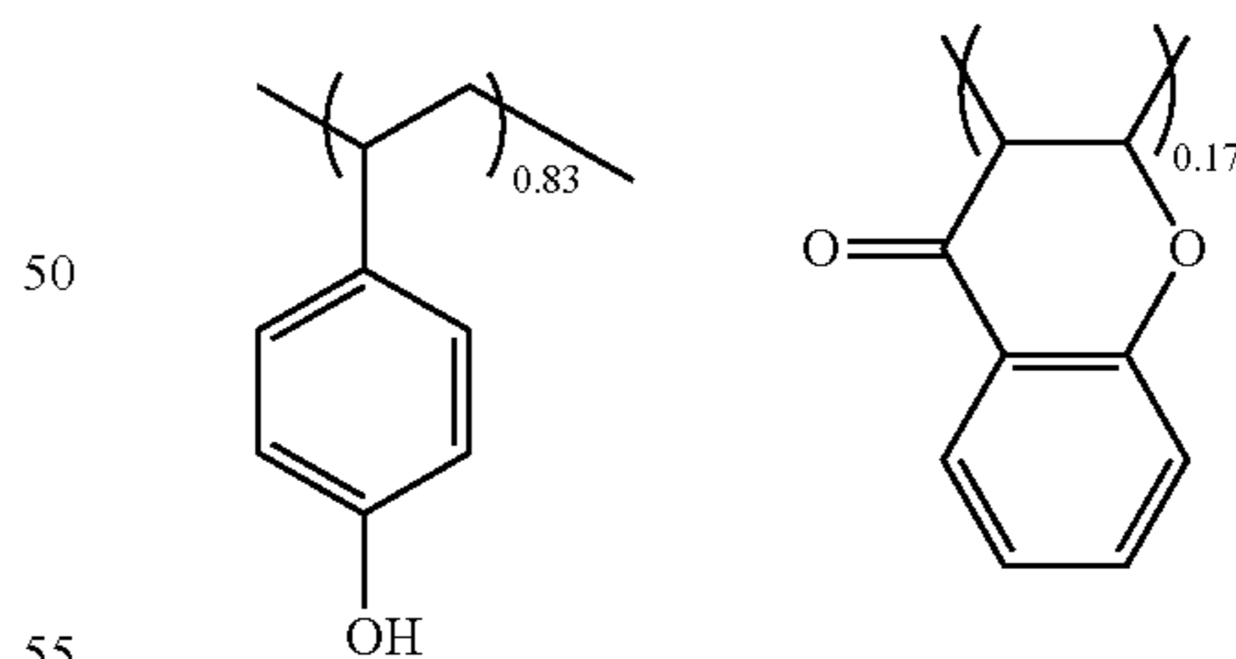
Synthetic Example 7
