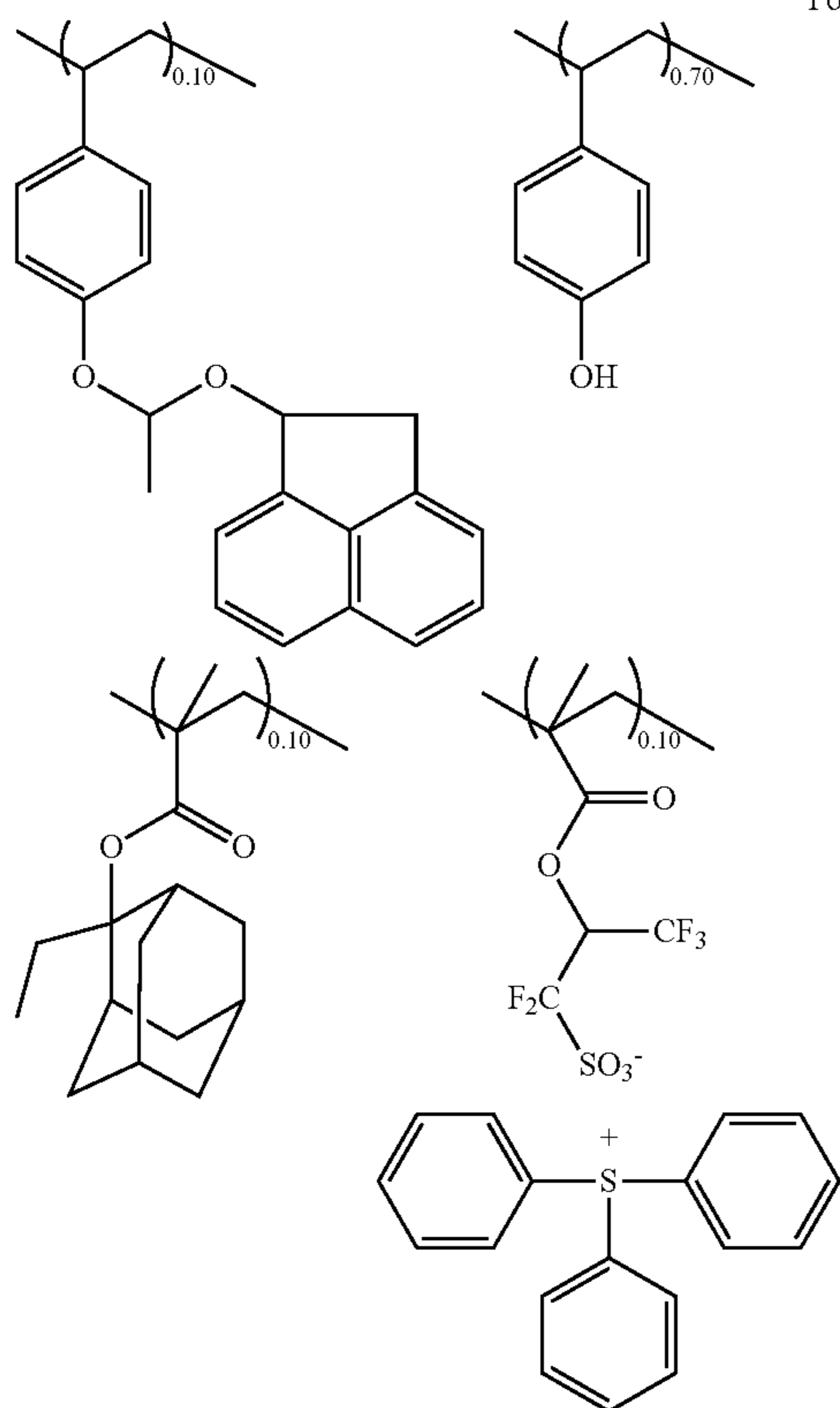
Synthetic Example 24
