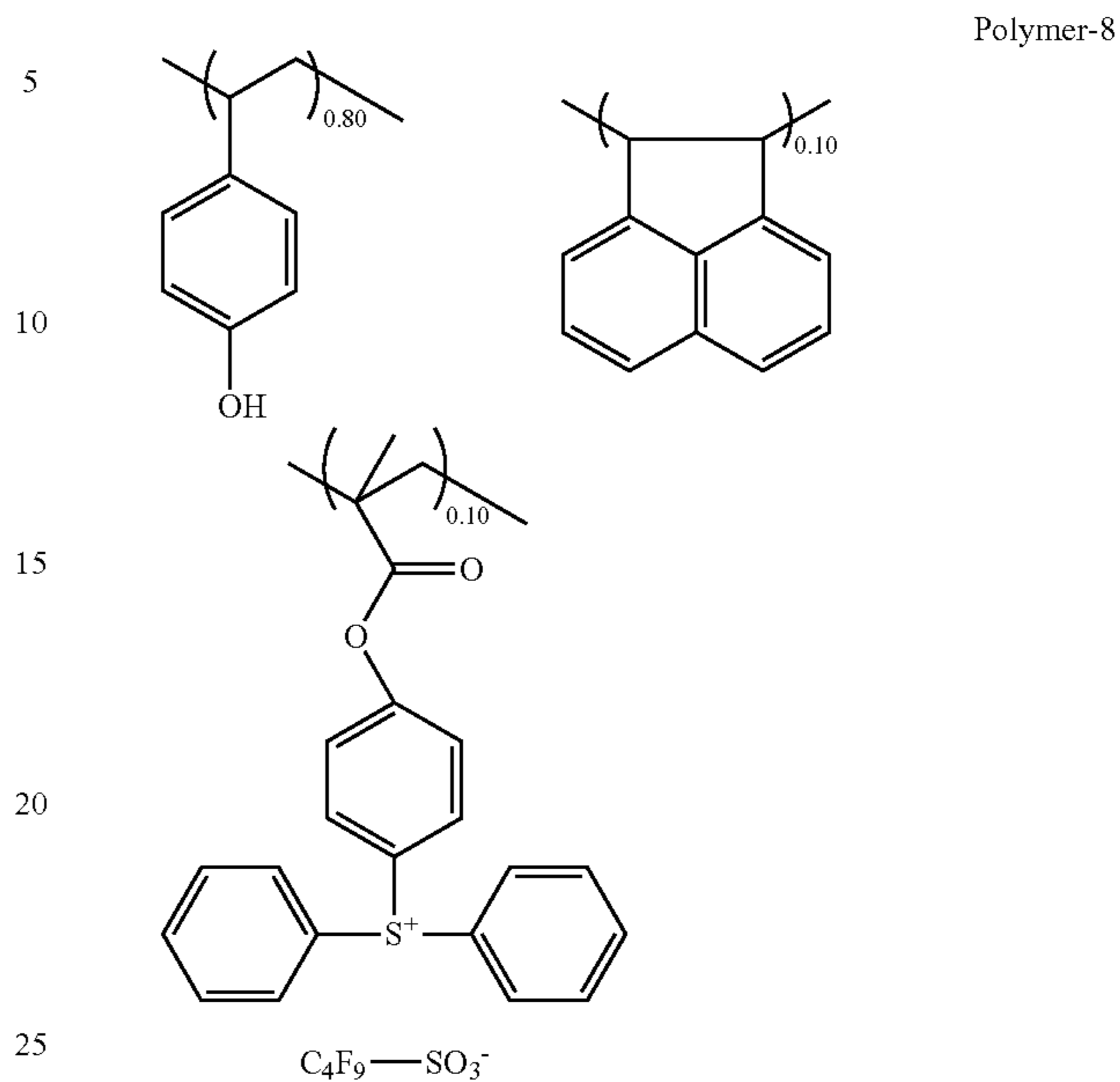
Synthetic Example 9
