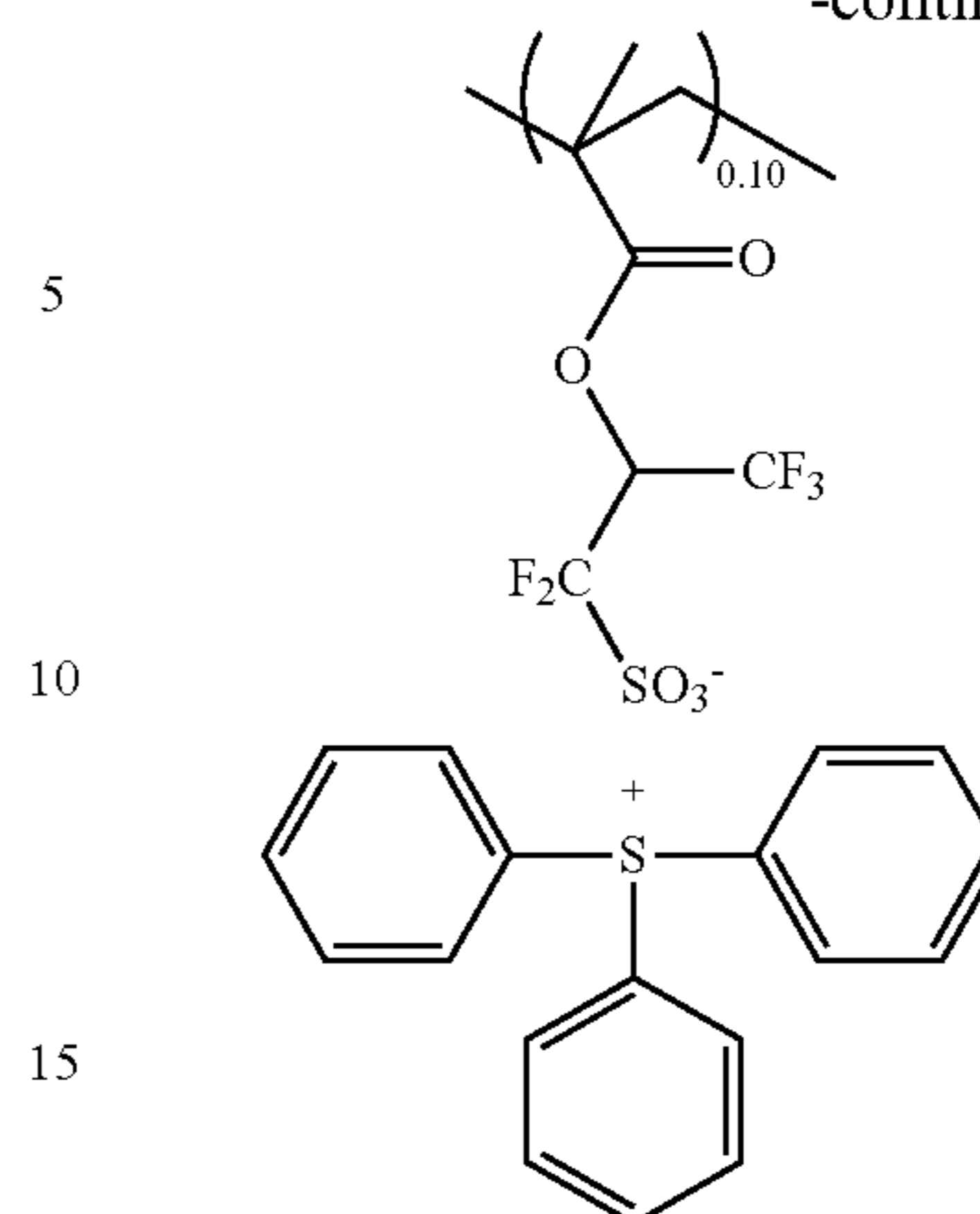
Synthetic Example 11
