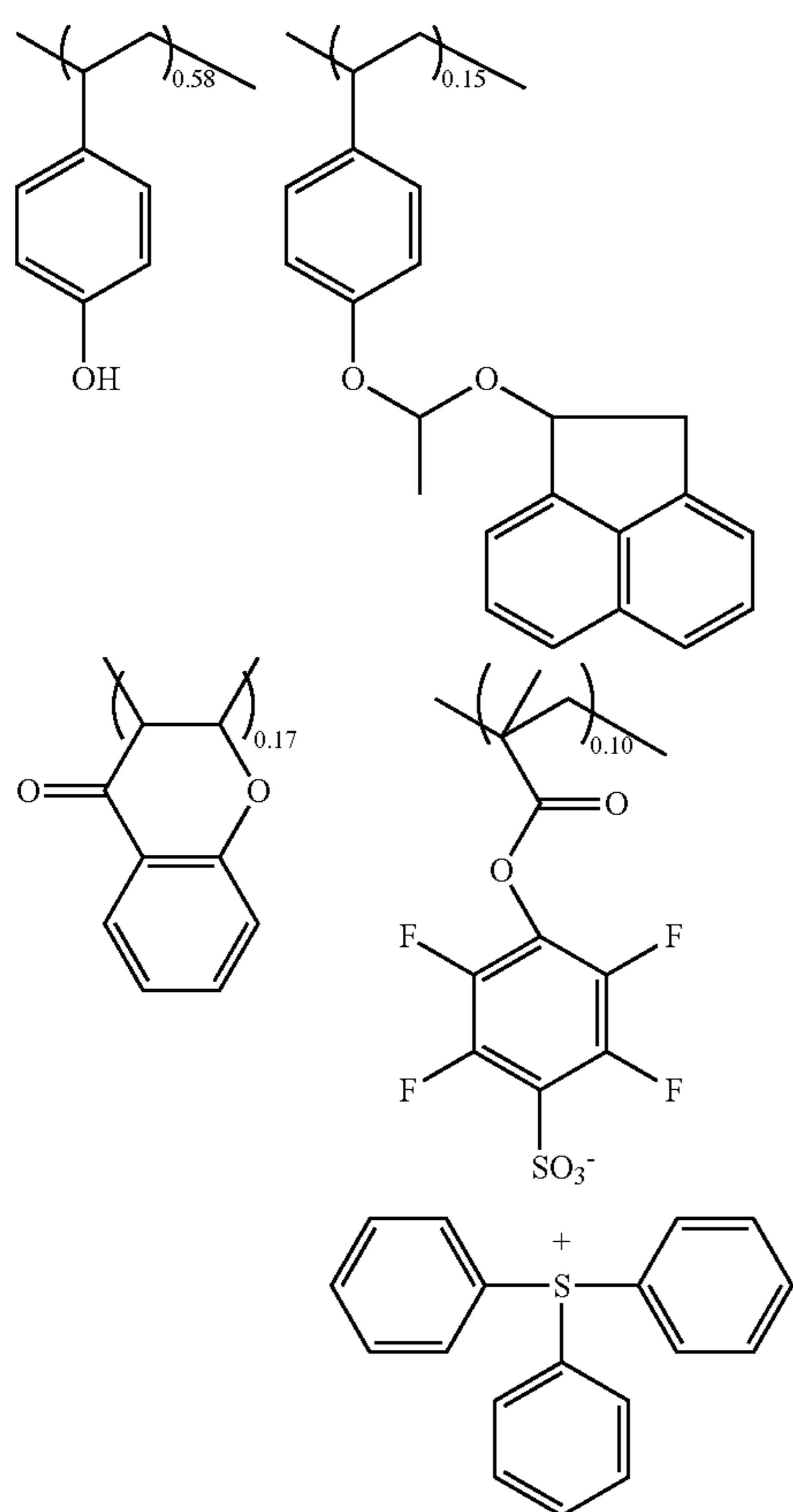
Synthetic Example 22
