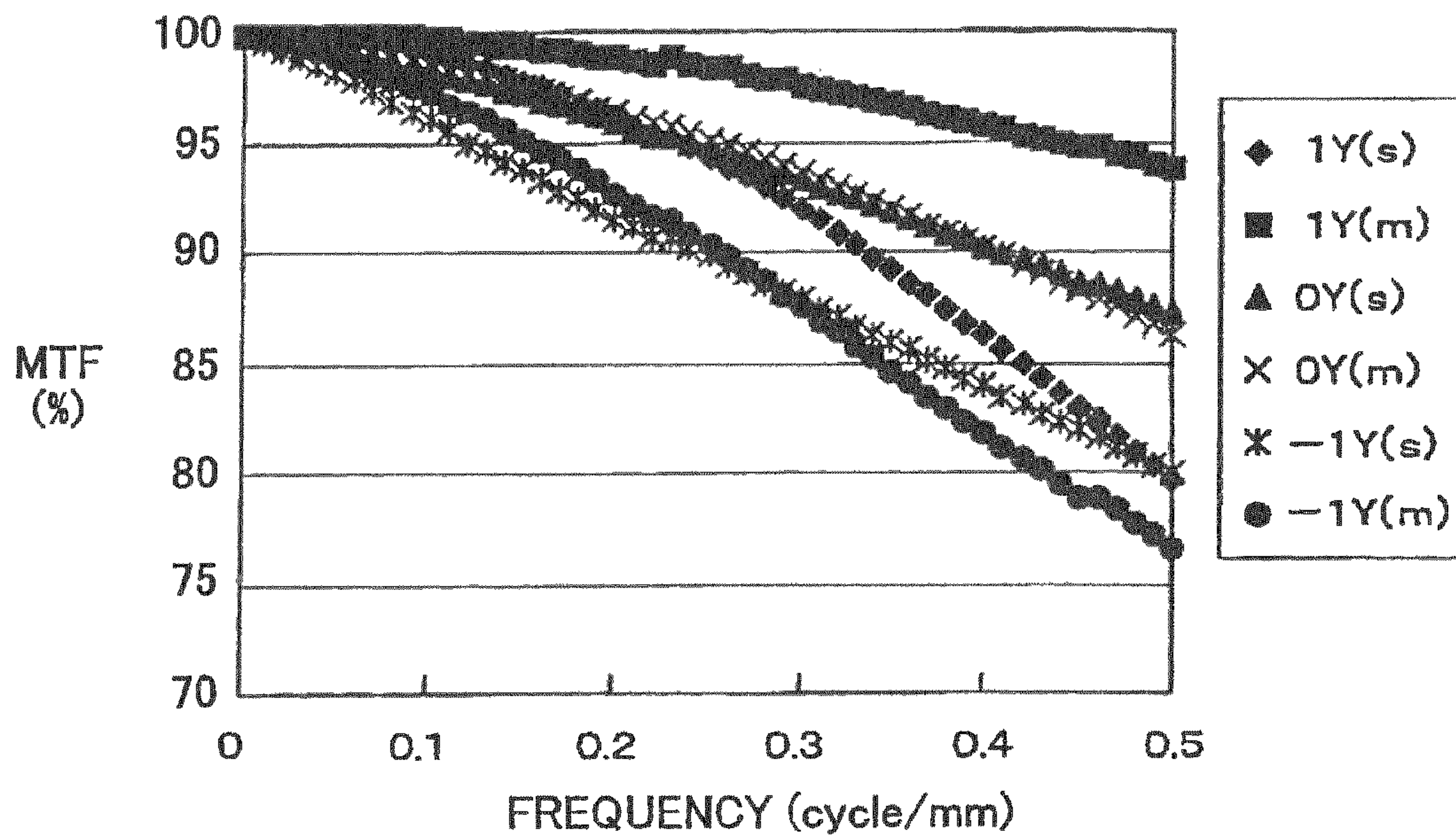
MTF CHARACTERISTICS 2 0.5X
