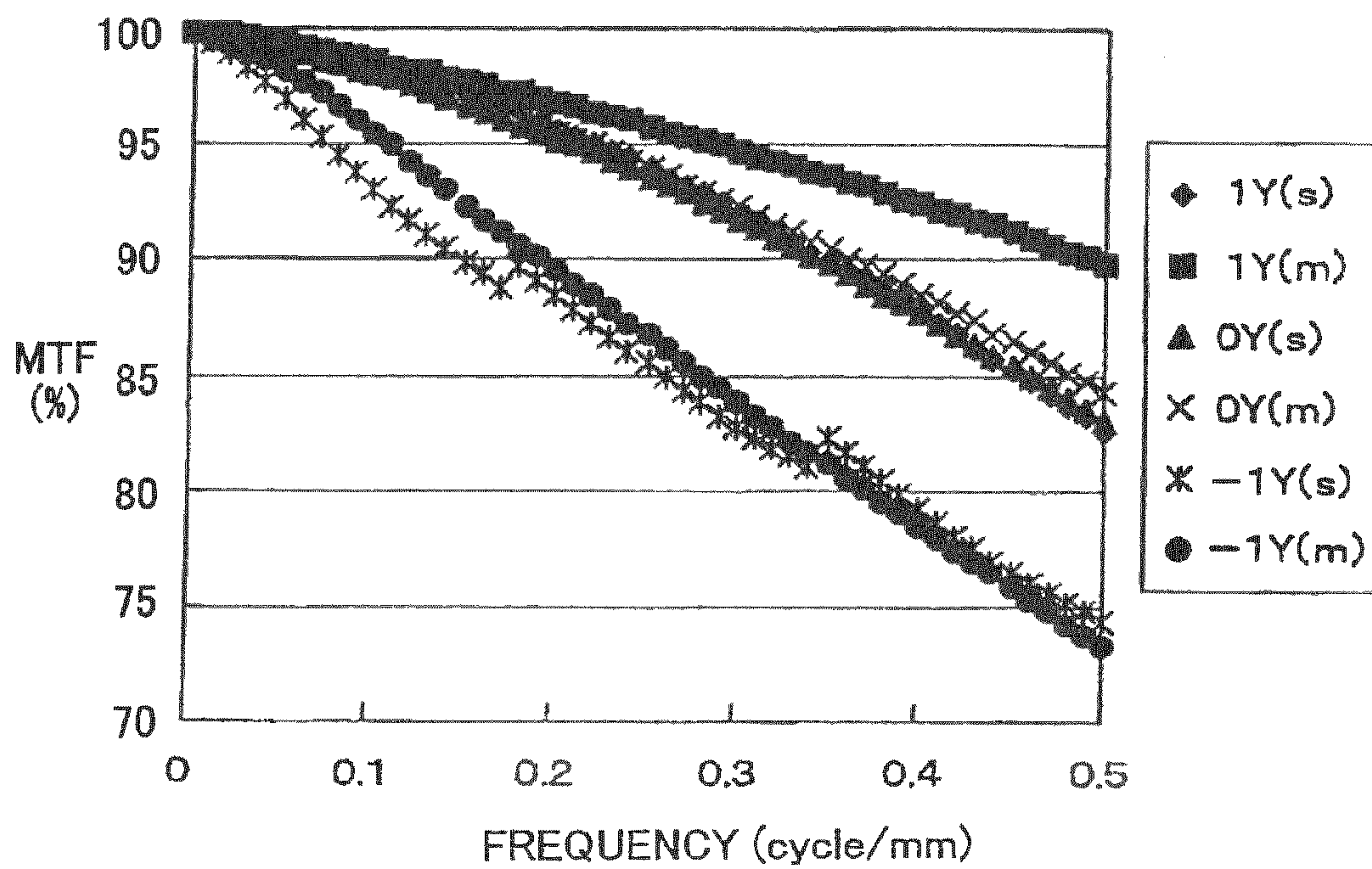
MTF CHARACTERISTICS 3 1.0X
