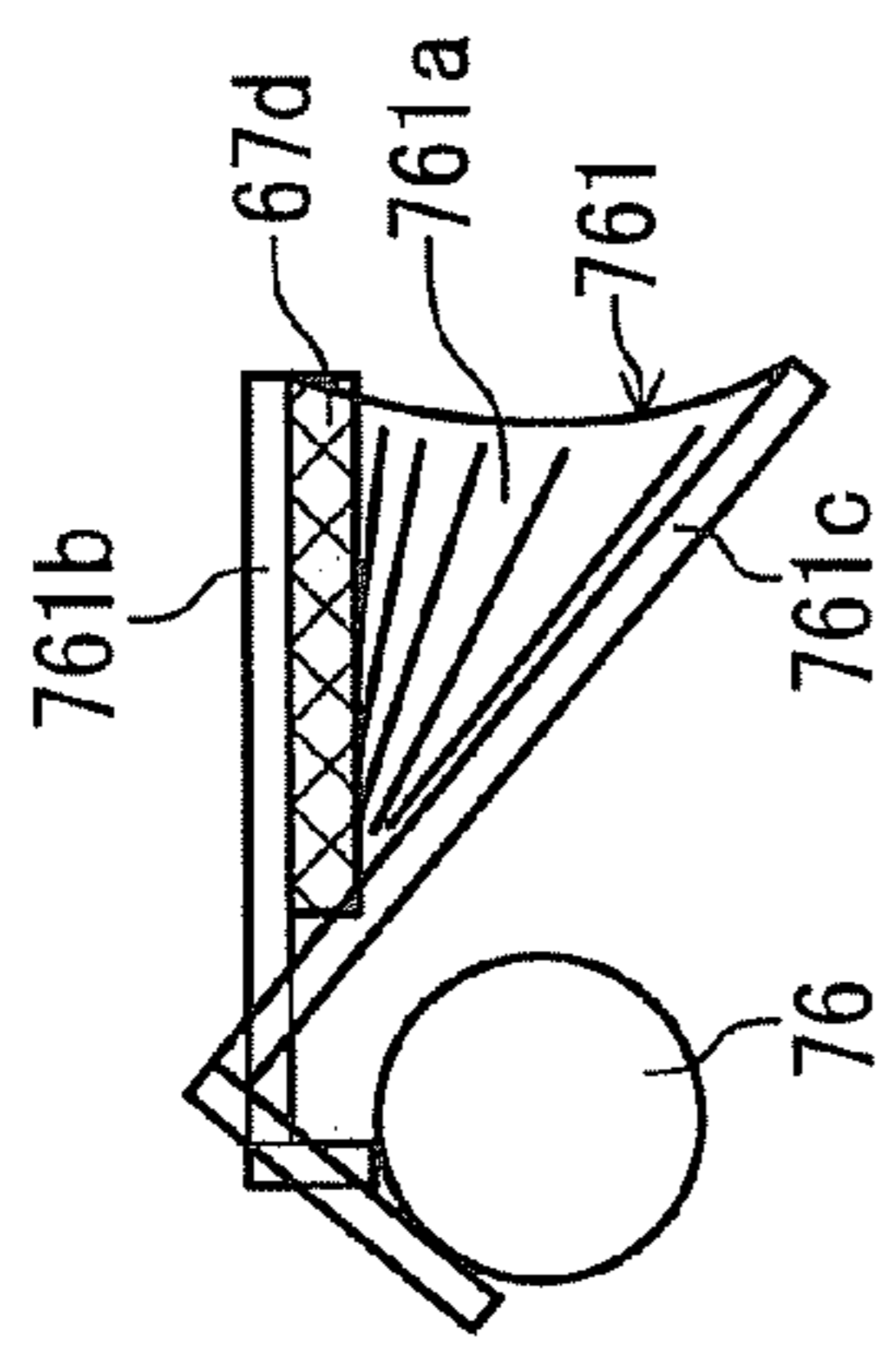
AT ROLLER UNIT MOVEMENT (AT FOLD LINE REINFORCING OPERATION)
