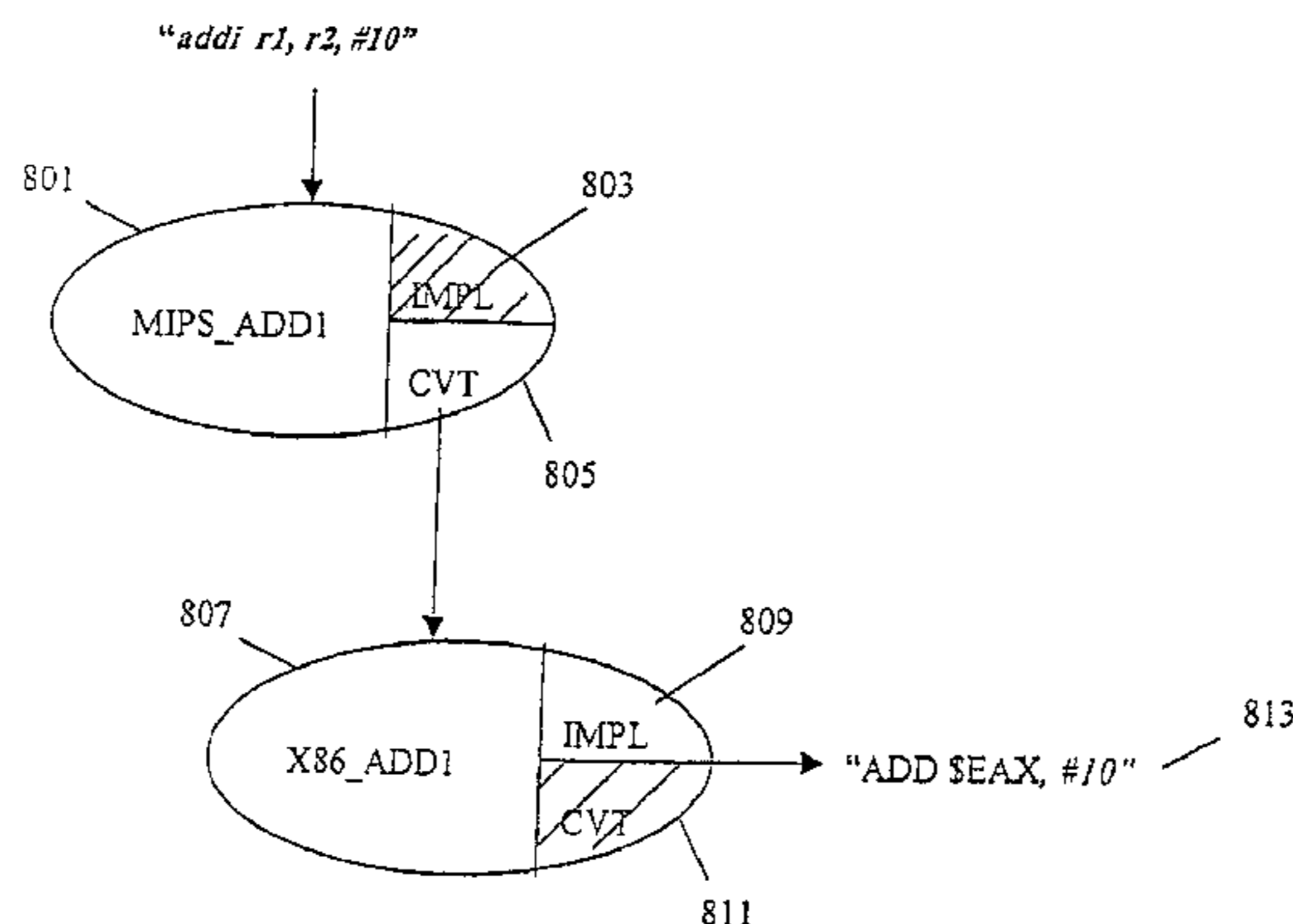
MIPS-X86 TRANSLATOR
