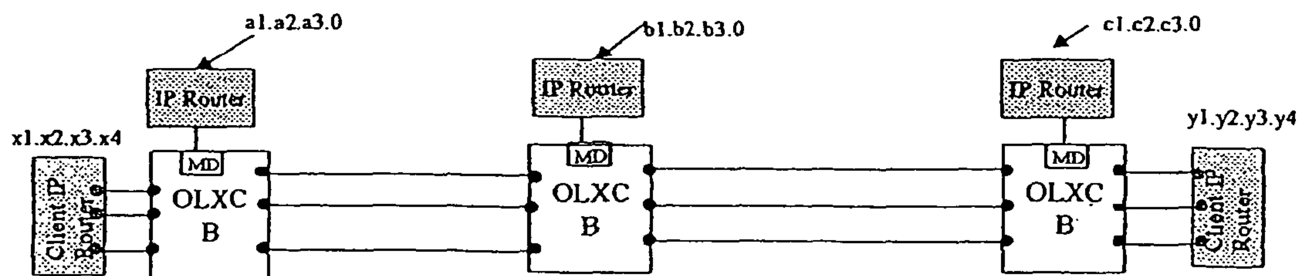
Figure 2. Example addressing scheme in the optical network
