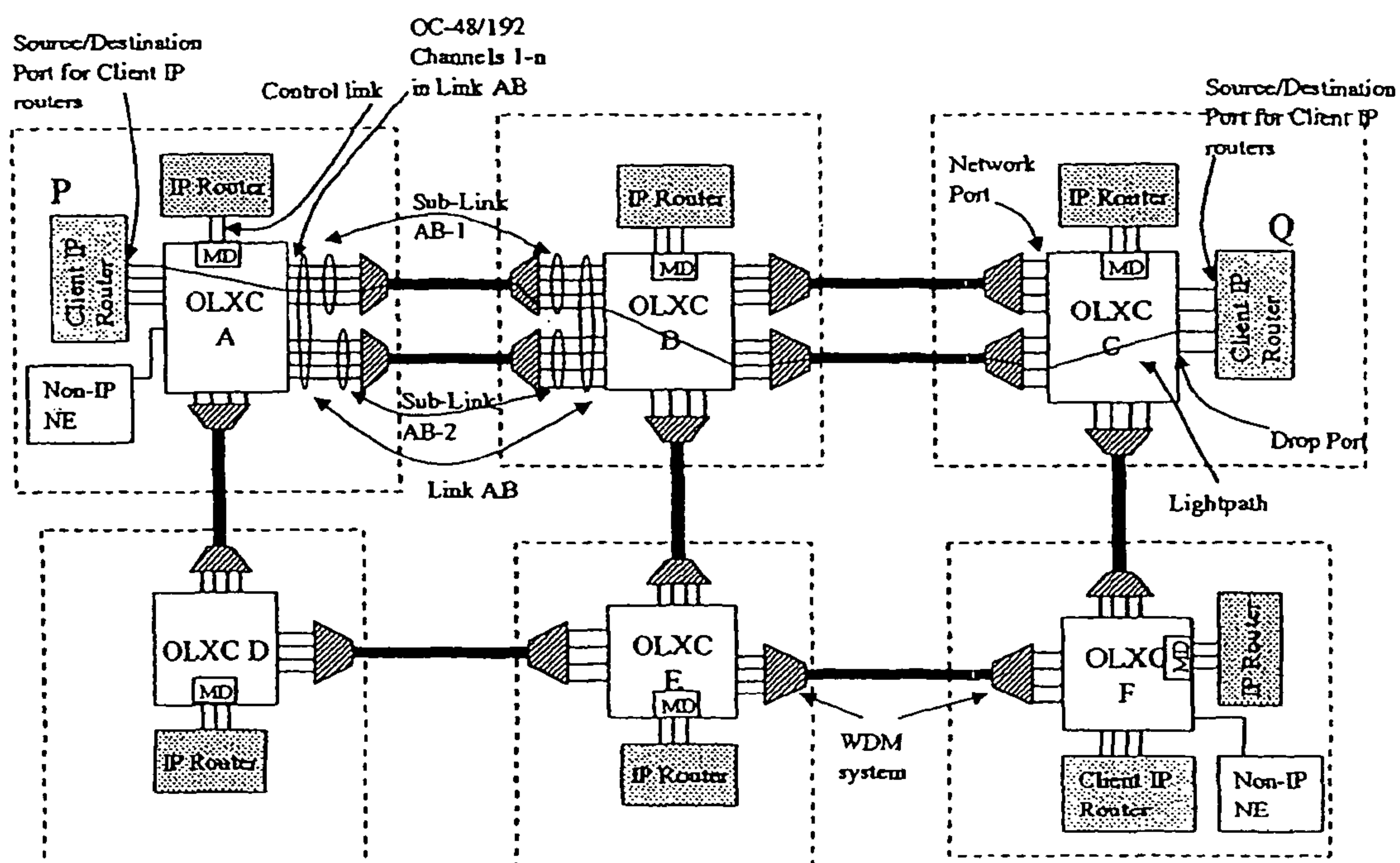
Figure 1. Example optical network illustrating defined network elements
