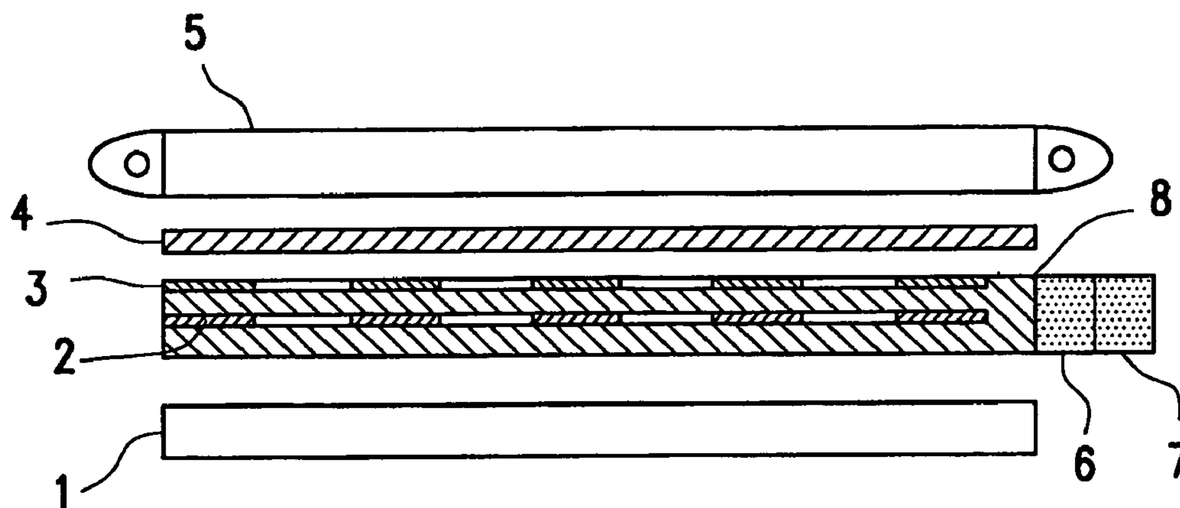
FIG. 3A(PRIOR ART)
