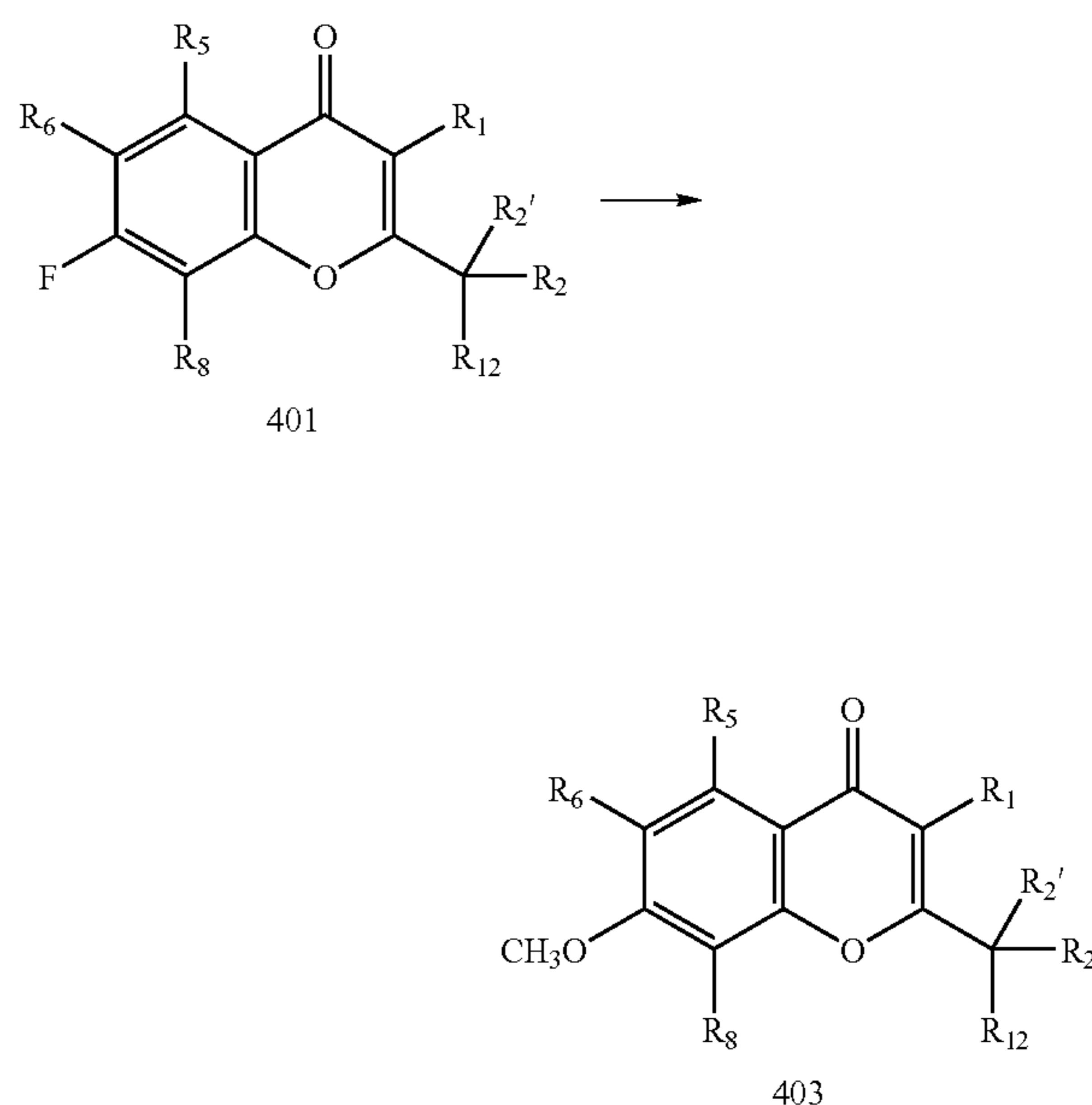
Reaction Scheme 4
