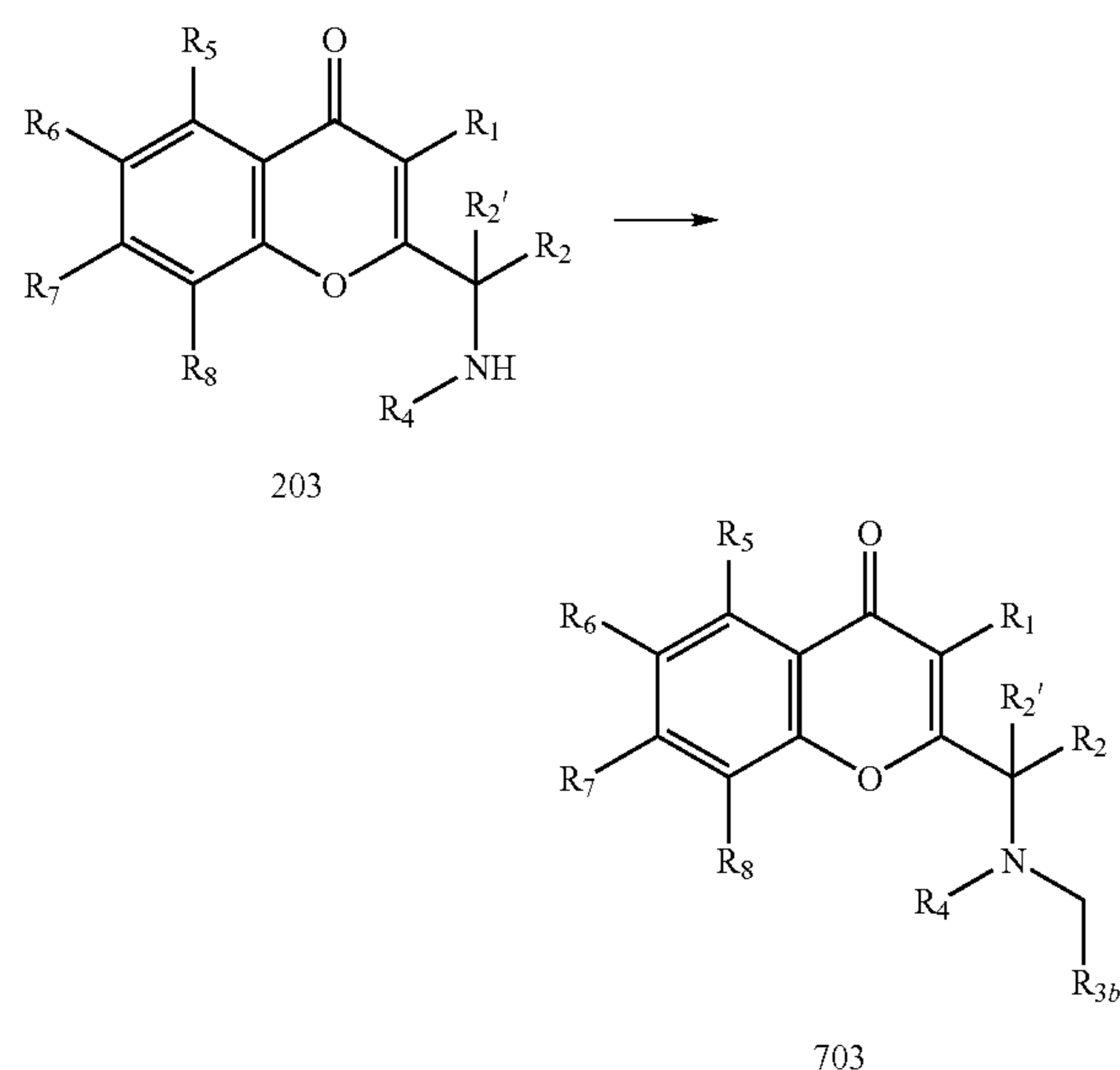
Reaction Scheme 7
