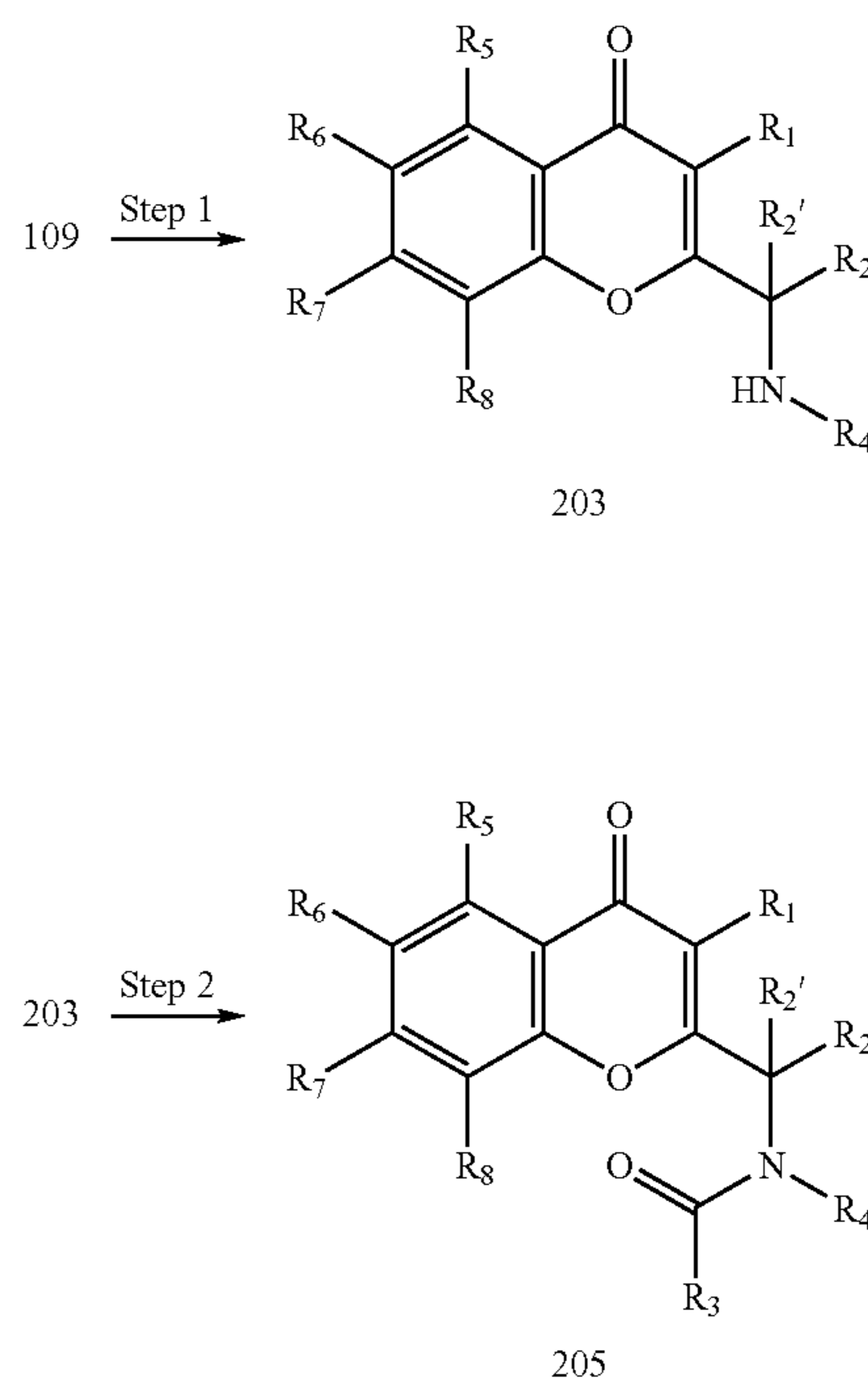
Reaction Scheme 2
