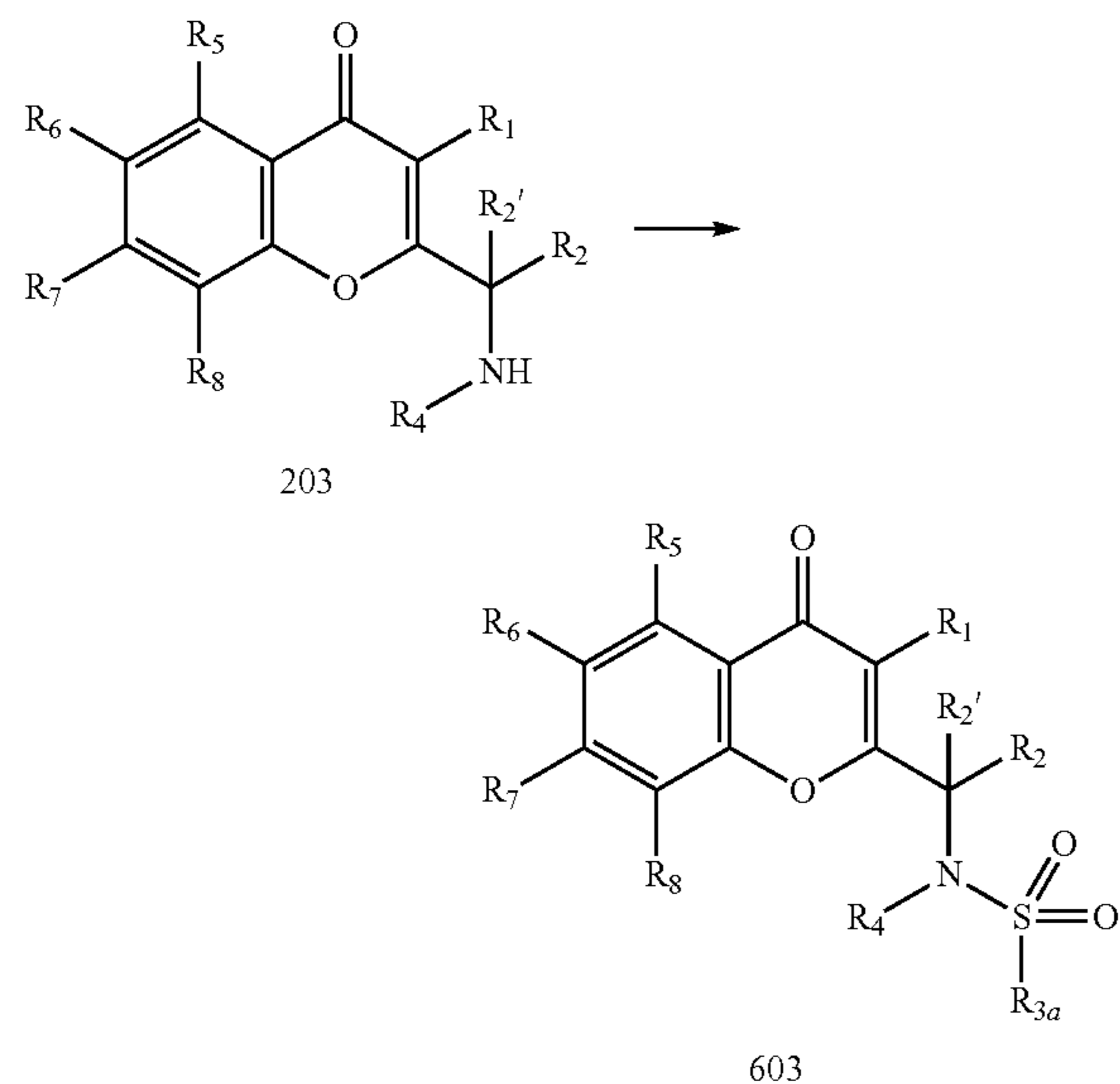
Reaction Scheme 6
