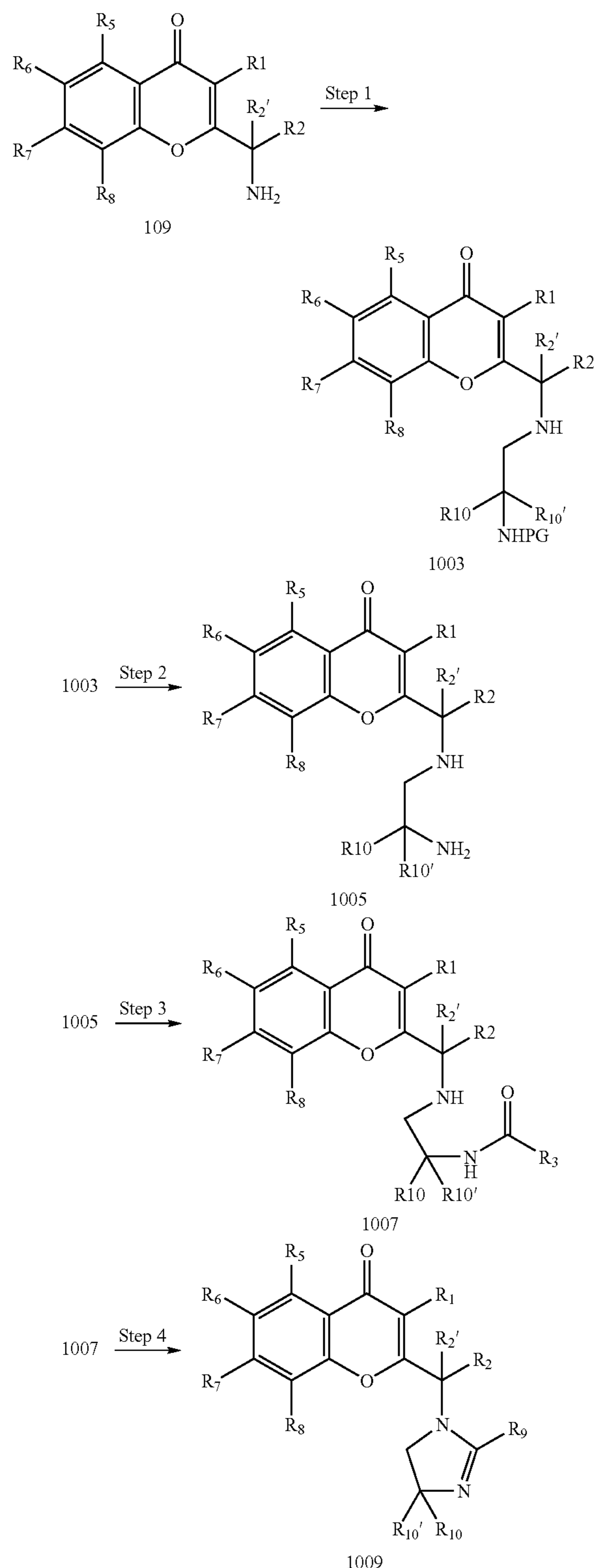
Reaction Scheme 10
