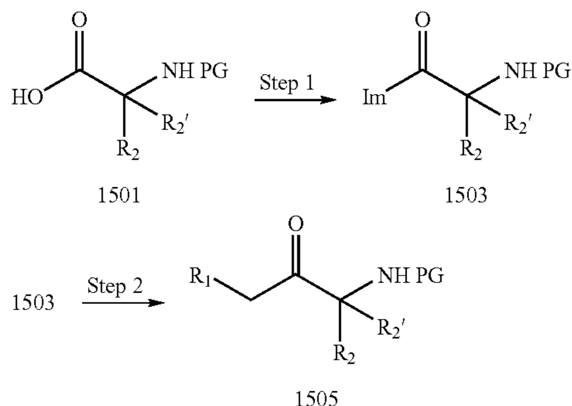
Reaction Scheme 15
