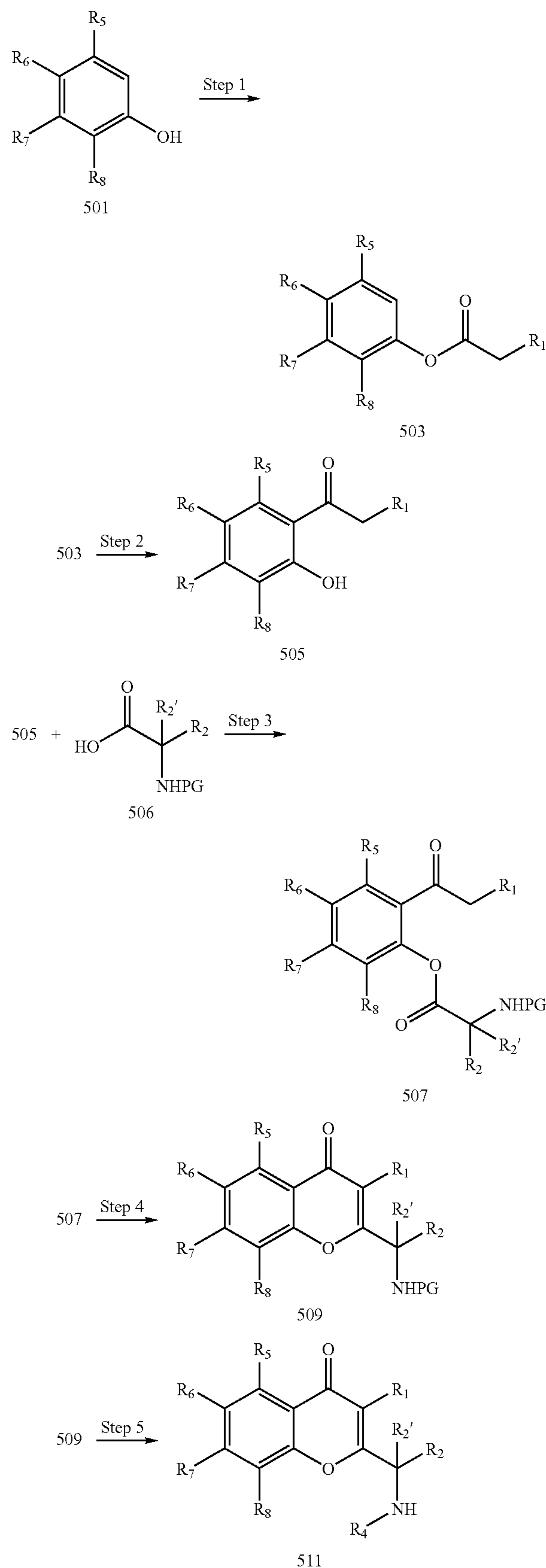
Reaction Scheme 5
