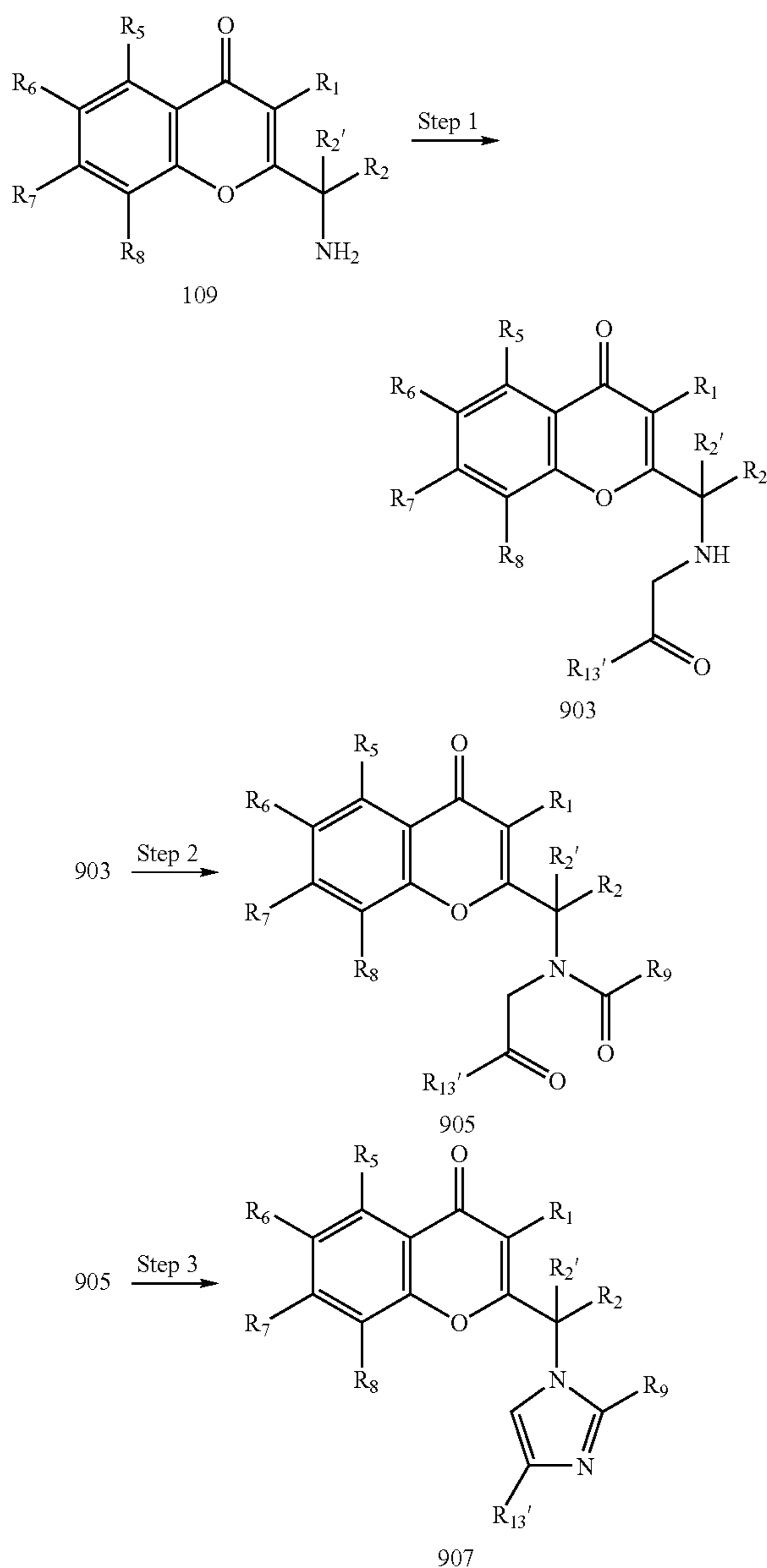
Reaction Scheme 9
