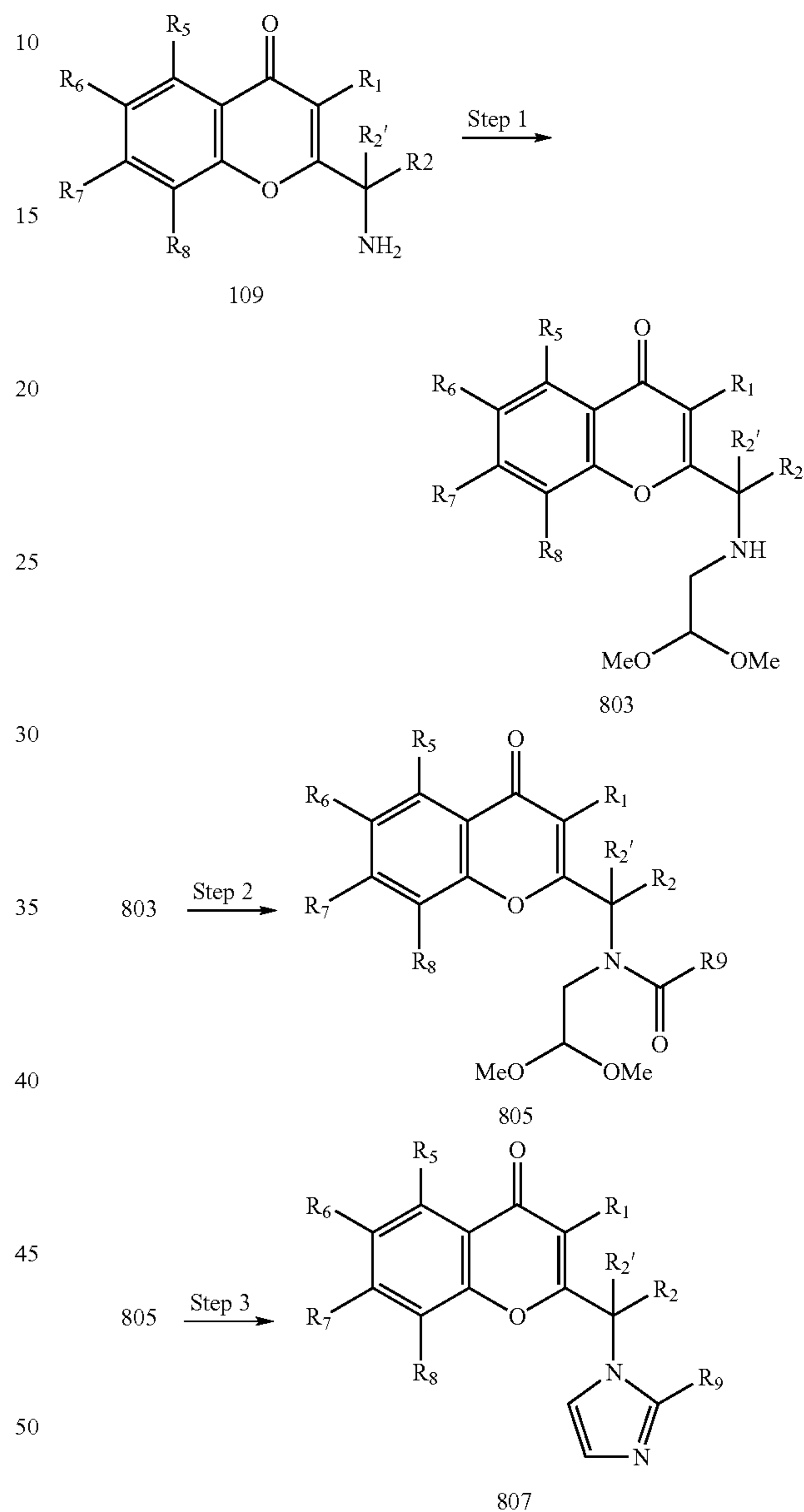
Reaction Scheme 8
