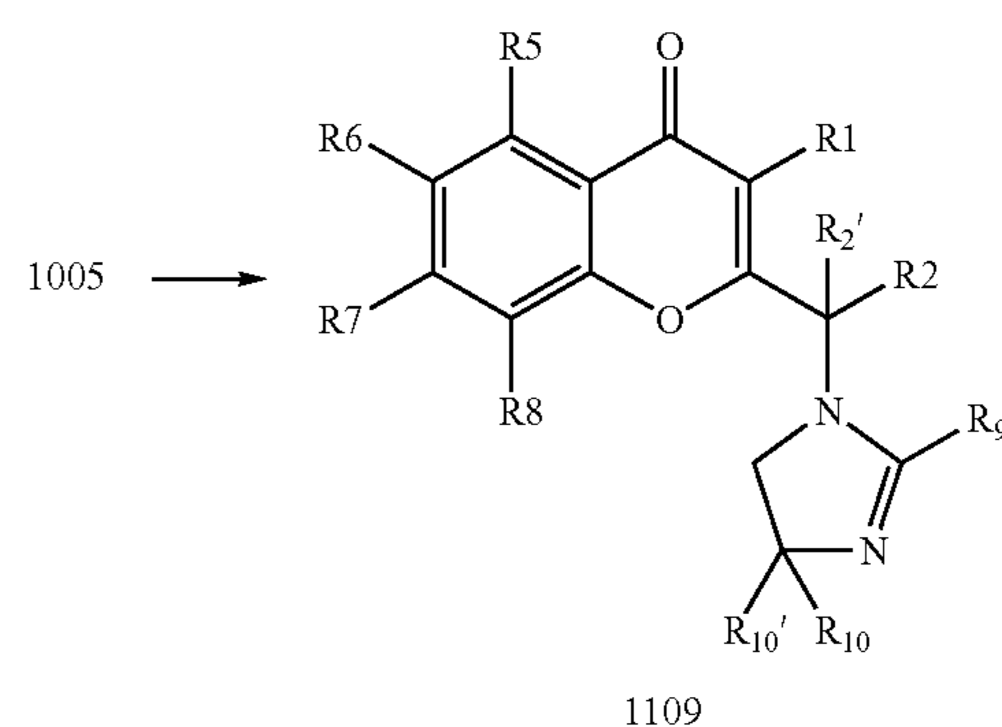
Reaction Scheme 11
