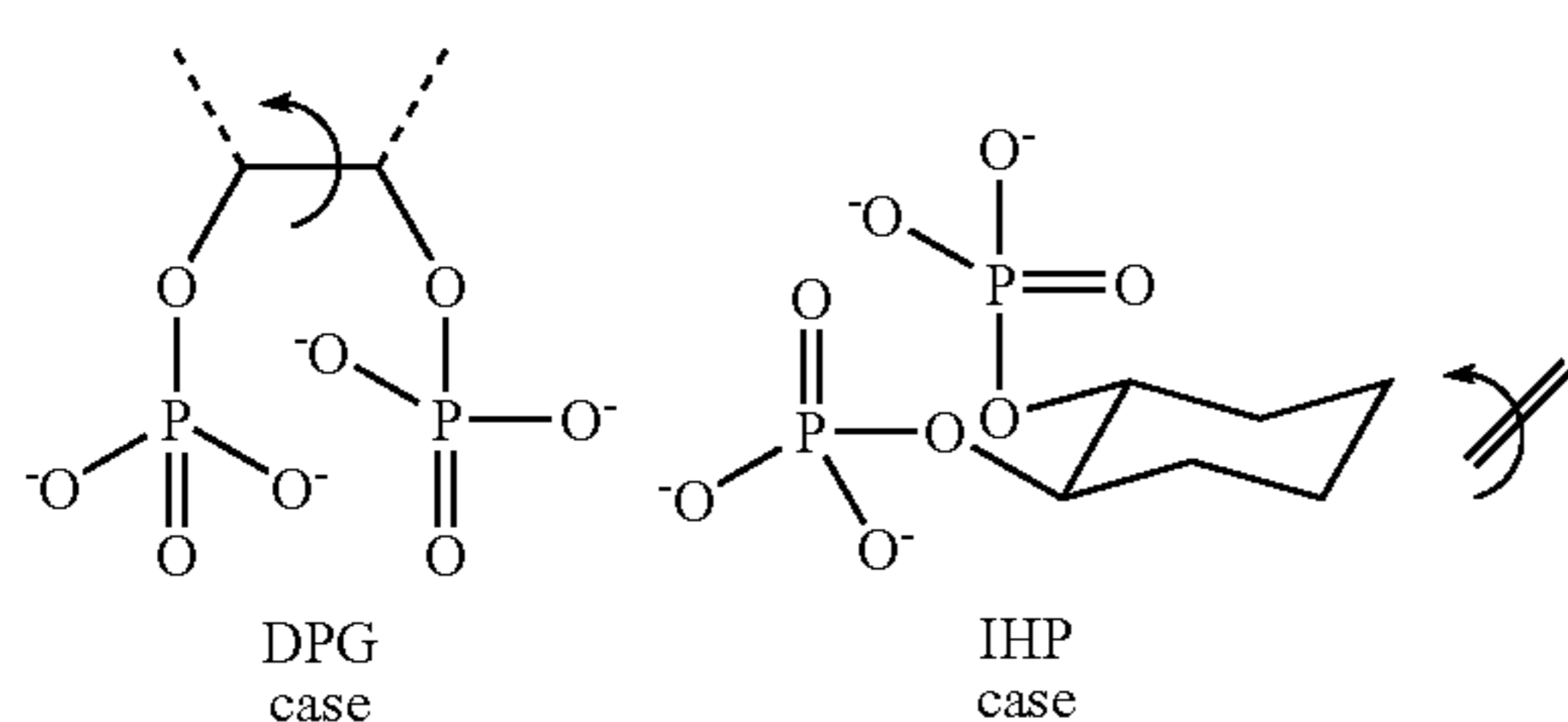
Scheme 5. Explanation of the behaviour of DPG and IHP toward acyl anhydrides.
