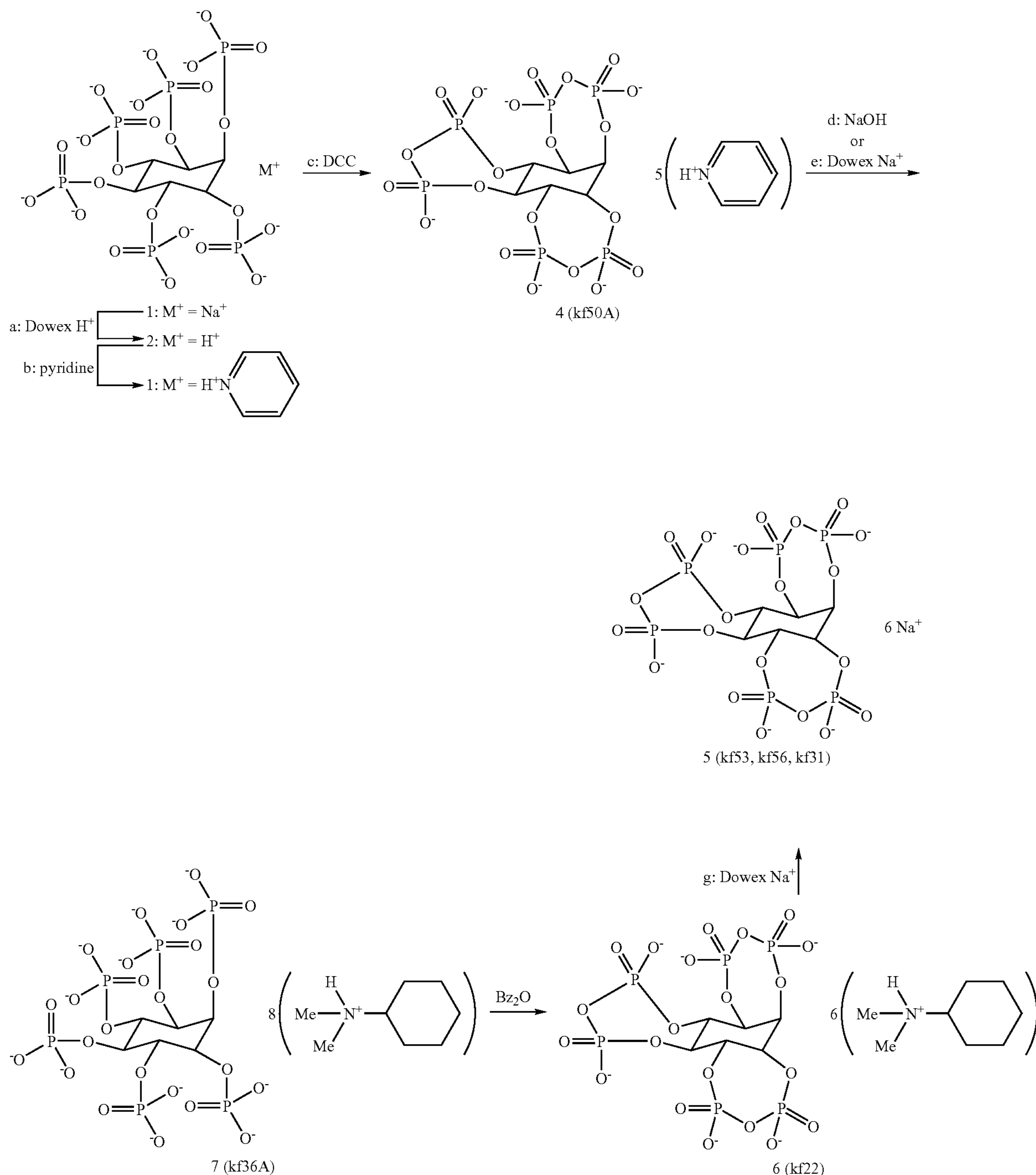
Scheme 3. The ITPP Na salts formation.
