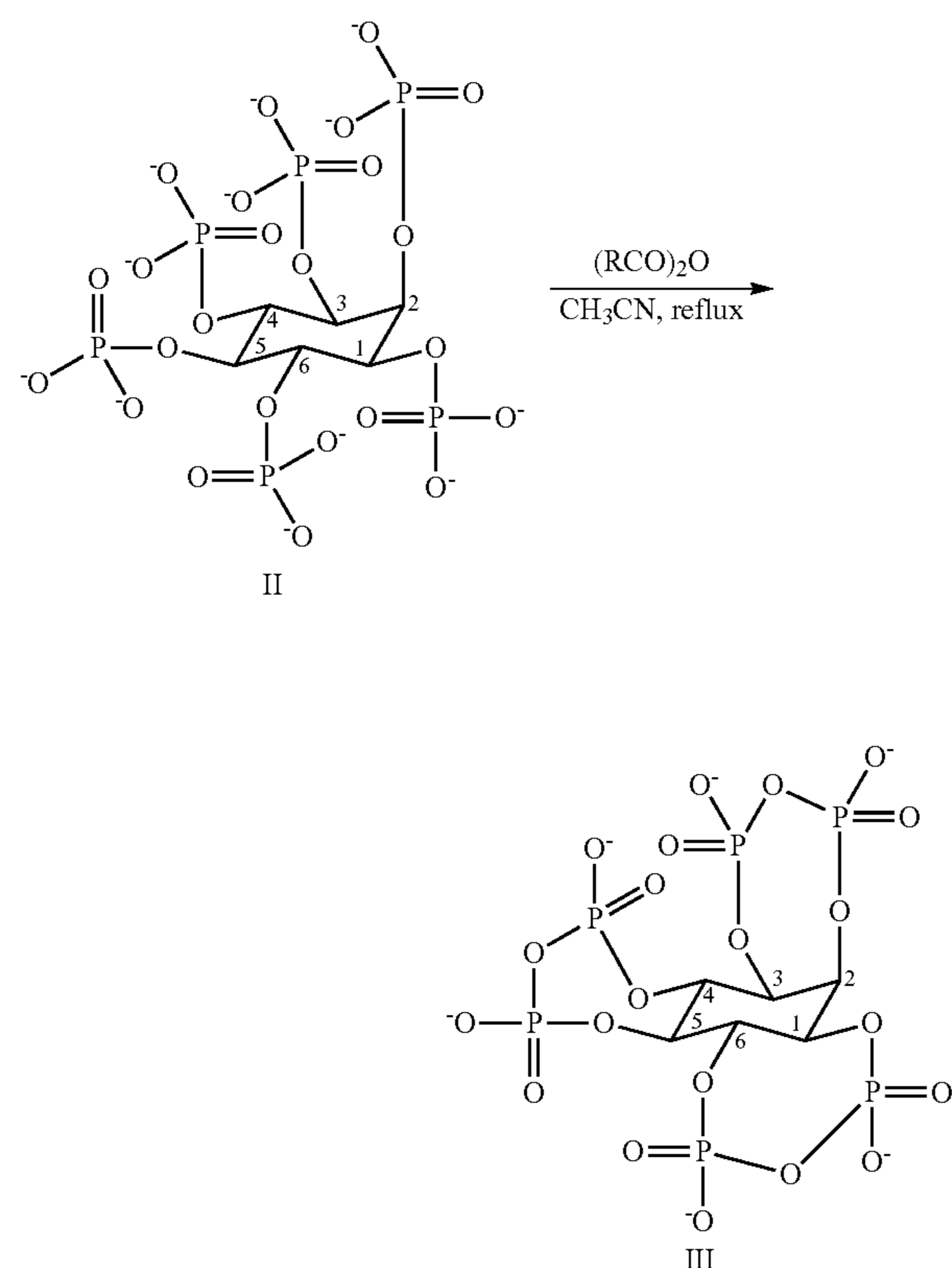
Scheme 1. Synthesis of IHP-tripyrophosphate.
