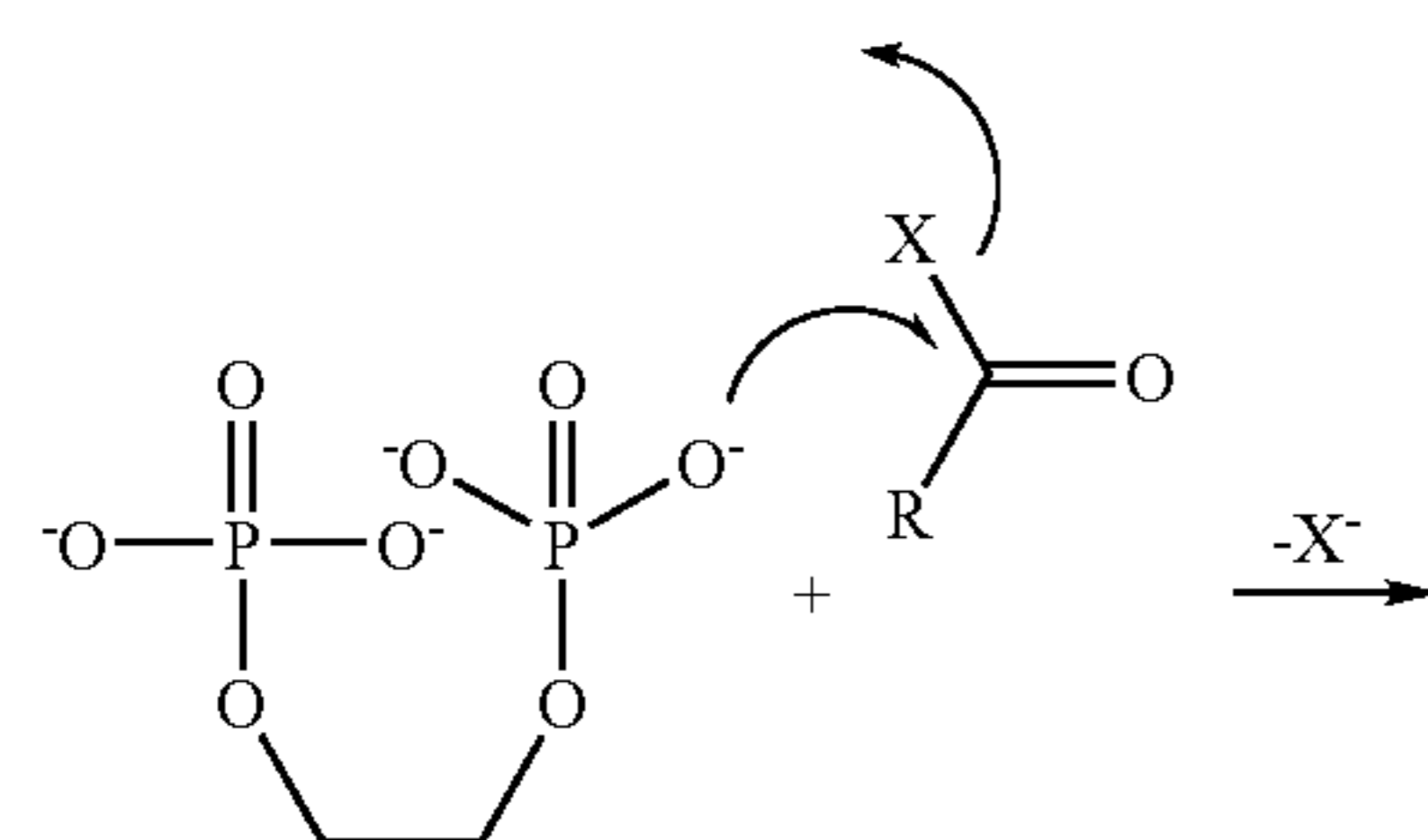
Scheme 2. Mechanism of internal pyrophosphate formation.
