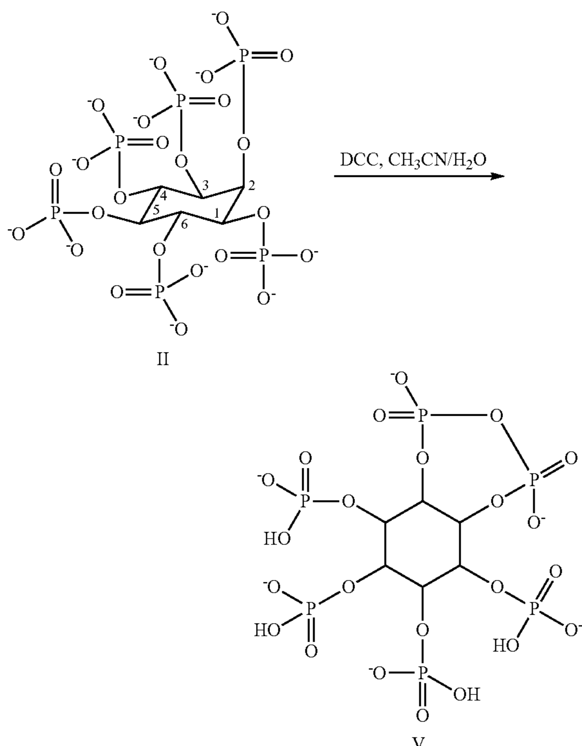
Scheme 8. Synthesis of hexa N,N-dimethylcyclohexylammonium salts of IHP monopyrophosphates.
