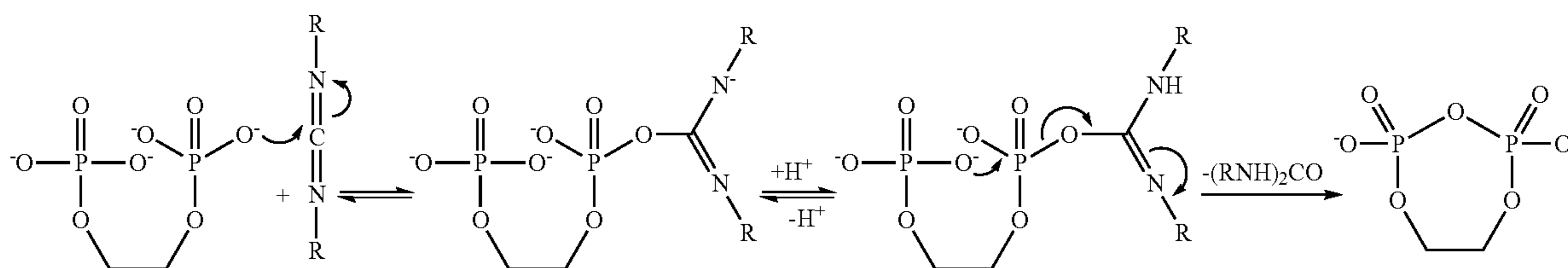
Scheme 4. Mechanistic pathways of the formation of pyrophosphates through a reaction with DCC.
