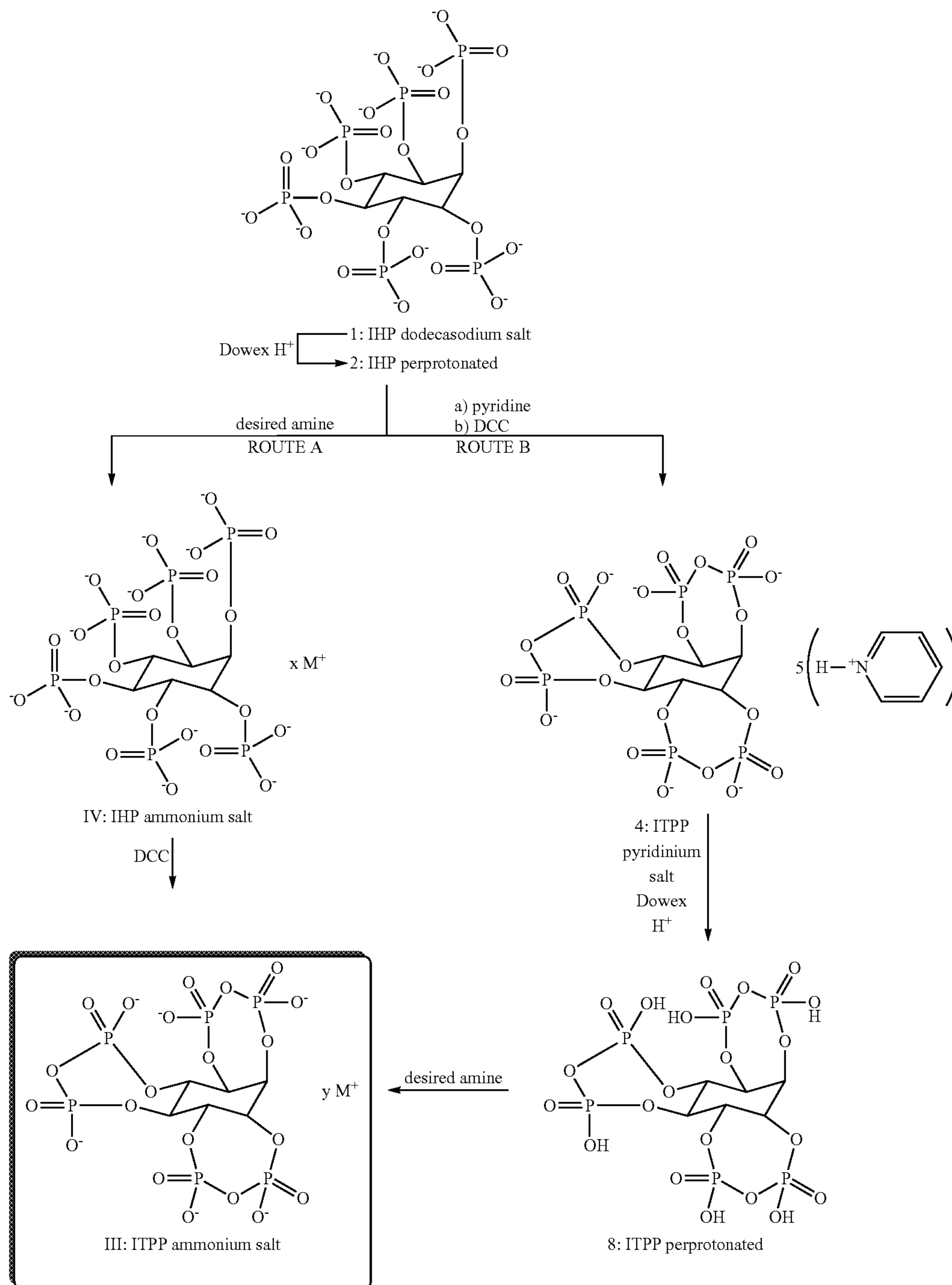
Scheme 6. General routes for the synthesis of ITPP ammonium salts.
