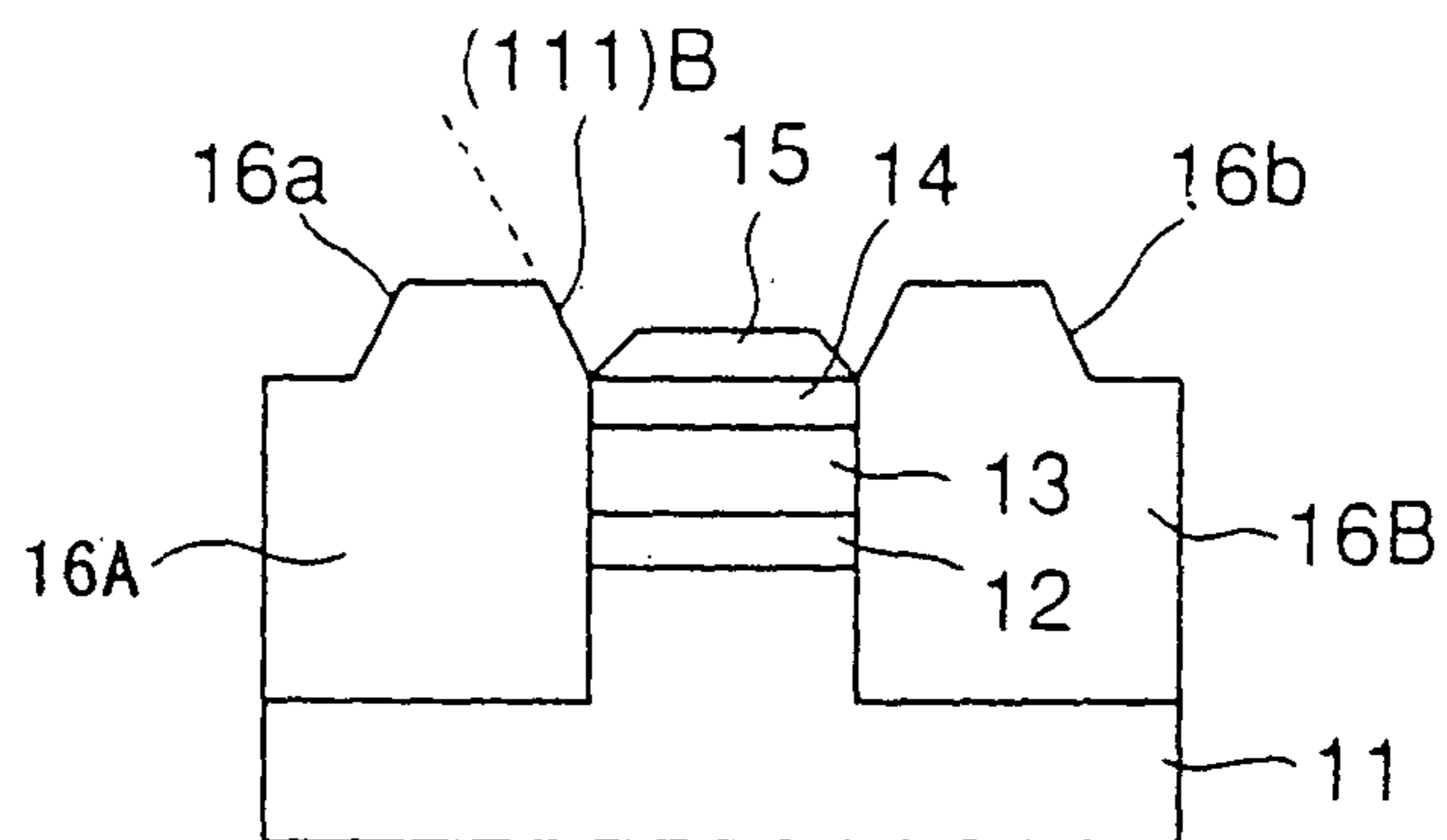
FIG. 1C PRIOR ART
