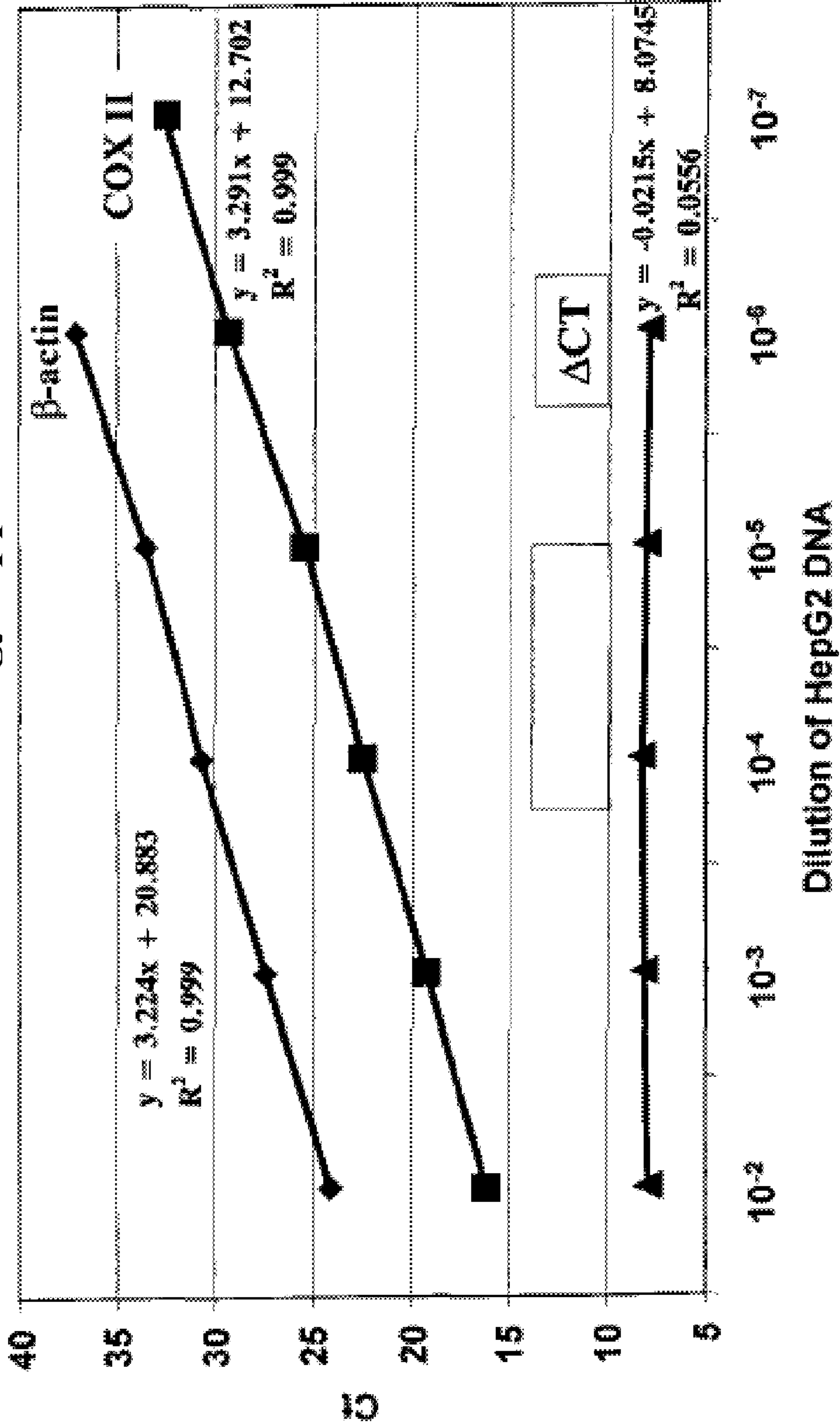
Figure 1E: Standard Curves and DCt Value for the Molecular Toxicology Approach
