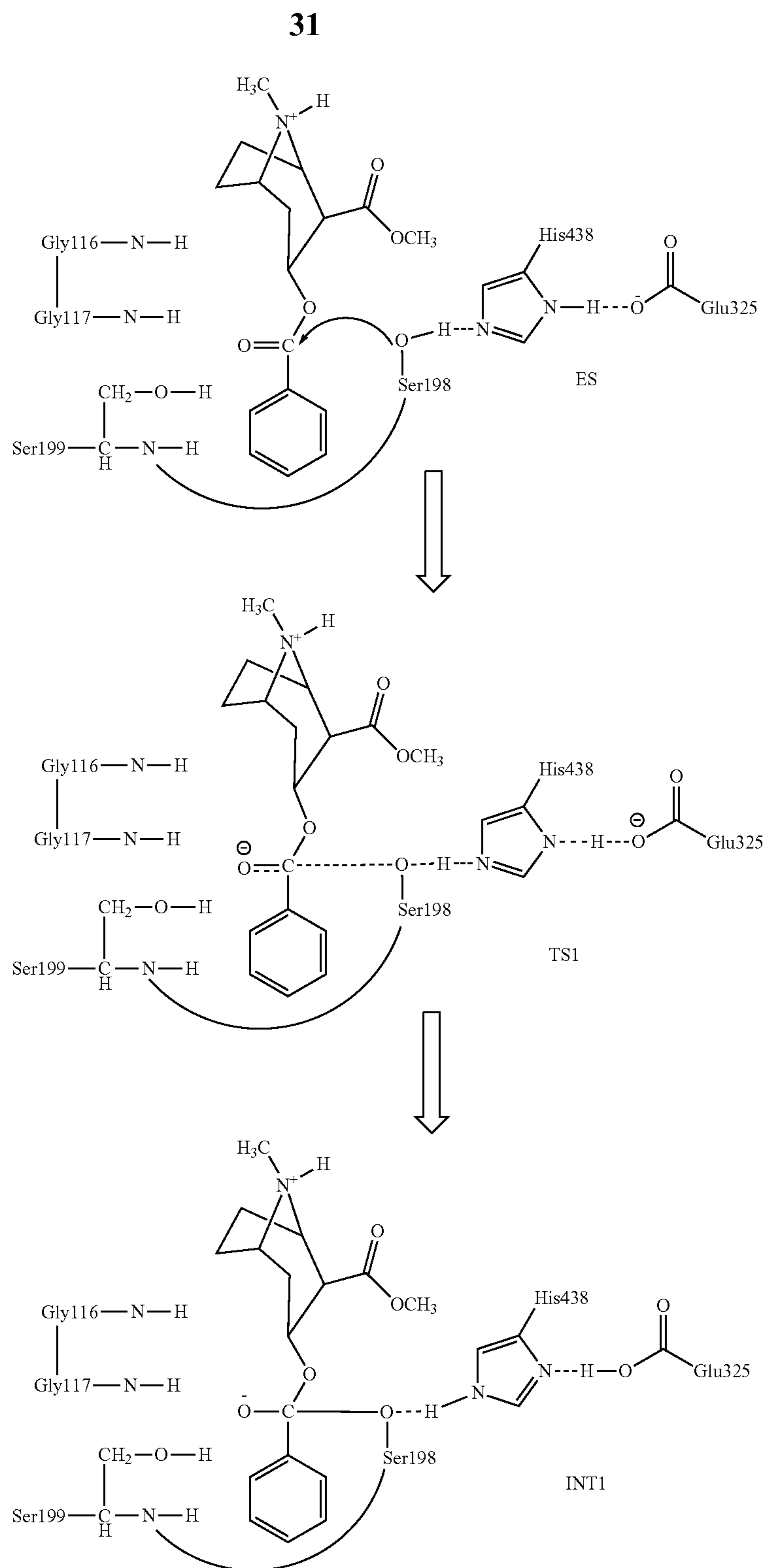
Scheme 4. Schematic representation of the first reaction step for (-)-cocaine hydrolysis catalyzed by a BChE mutant with an A199S mutation.
