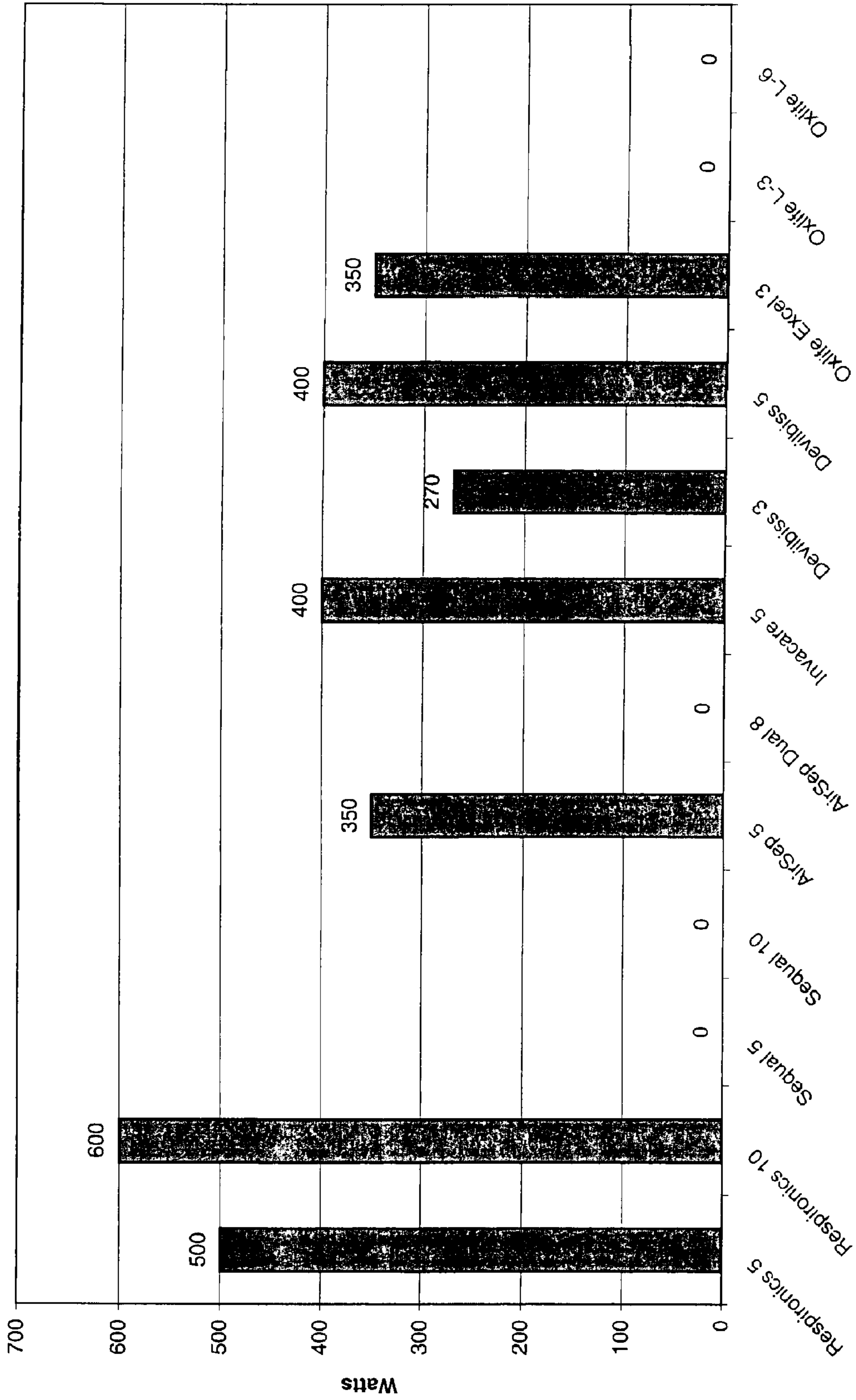
FIG 11 Power Consumption
