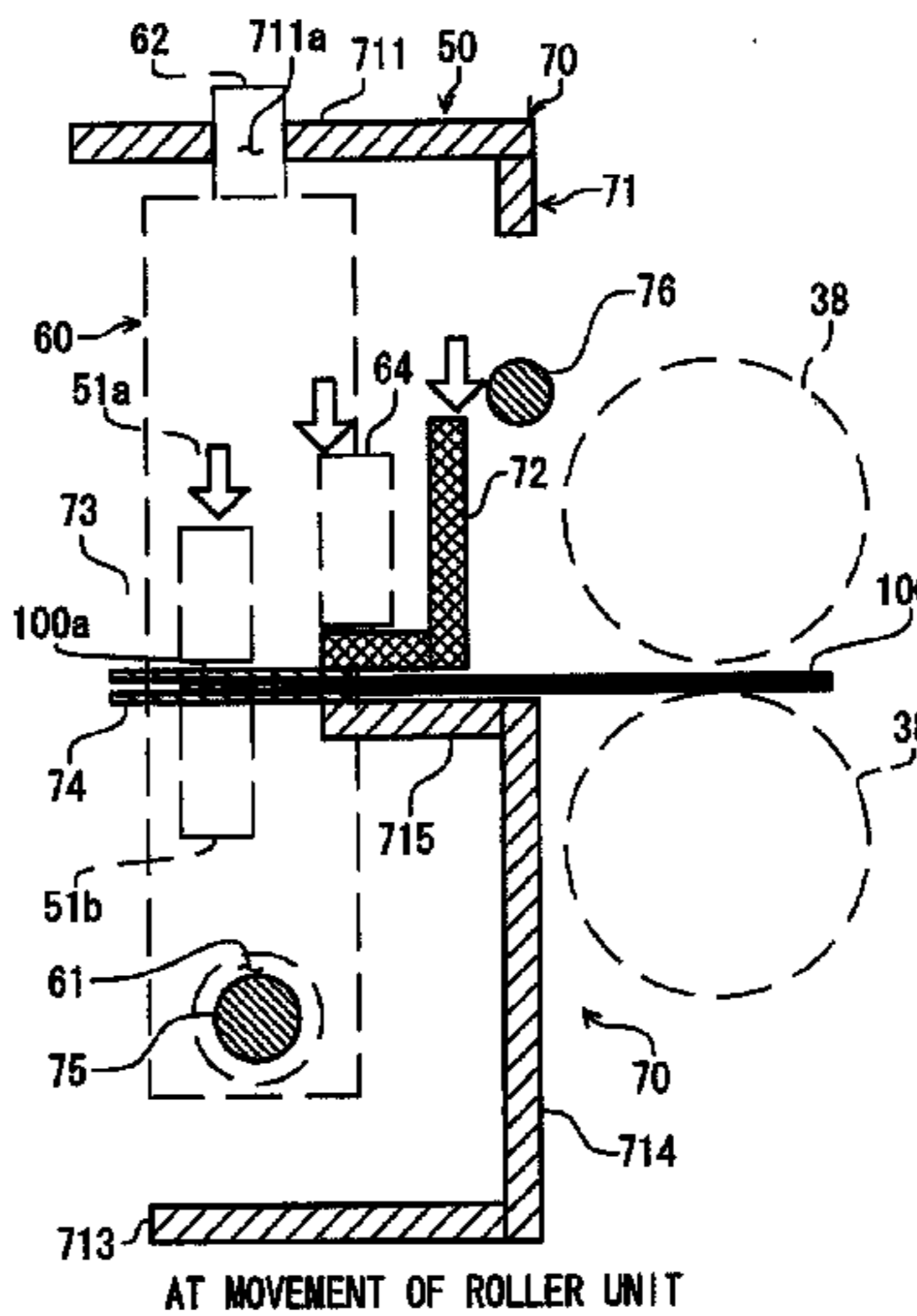
AT MOVEMENT OF ROLLER UNIT (AT FOLD LINE REINFORCING OPERATION)
