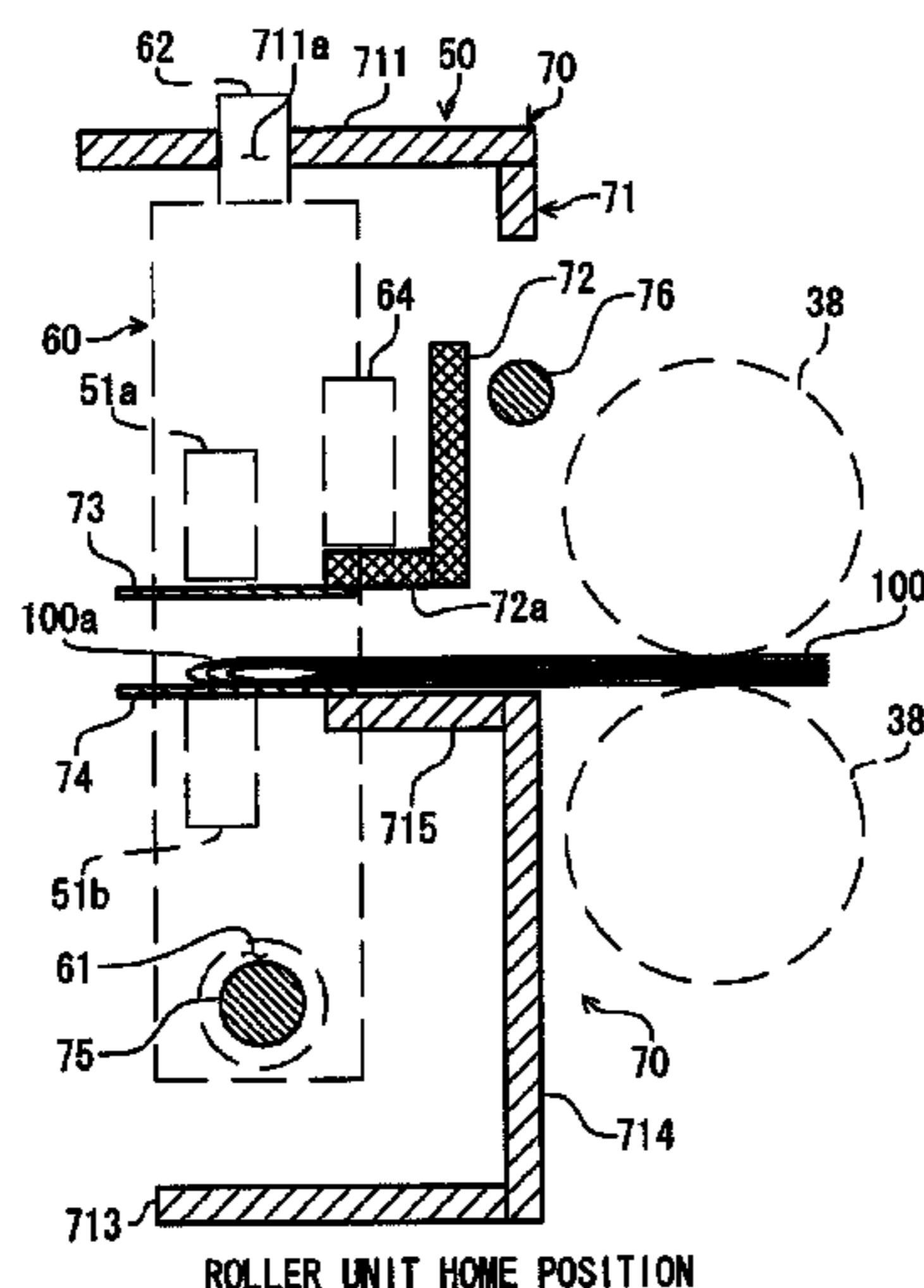
ROLLER UNIT HOME POSITION
