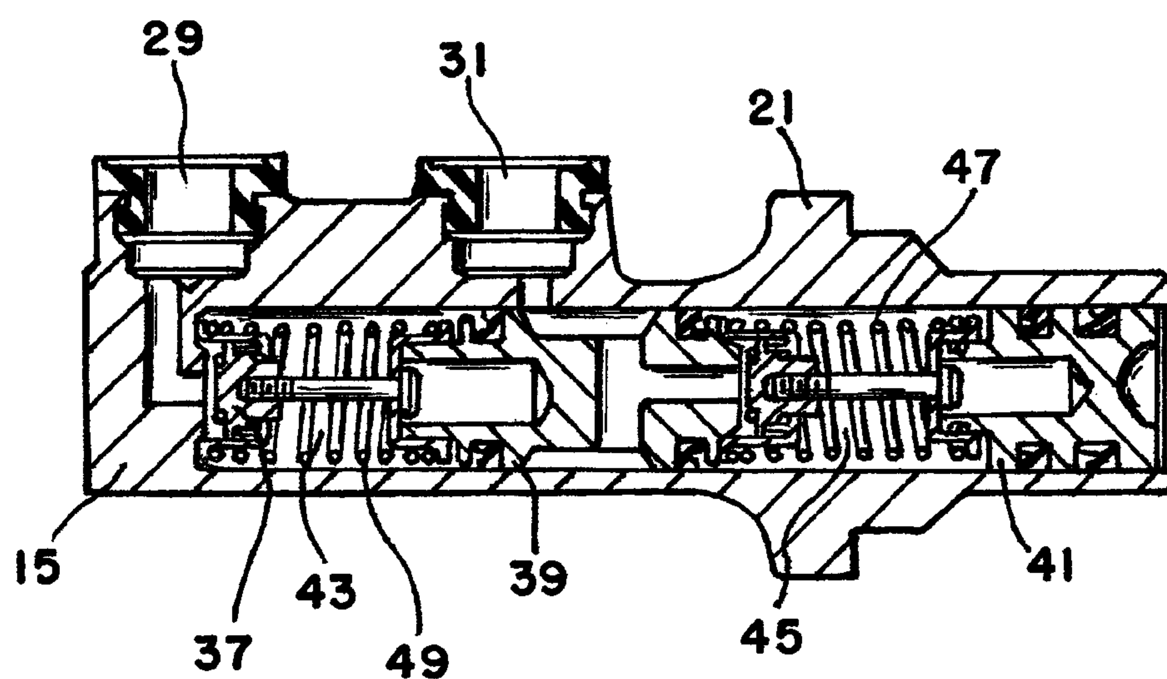
FIG. 2 (prior art)
