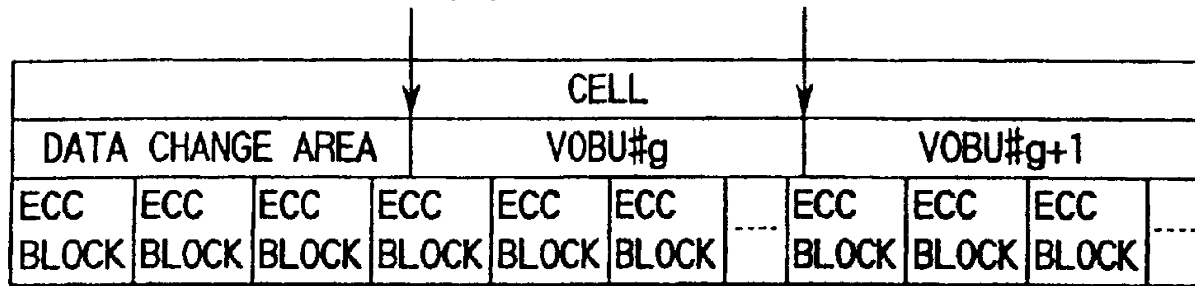
POSITIONS OF SHIFT PRODUCED BETWEEN ECC BLOCK BOUNDARY AND VOBU BOUNDARY
