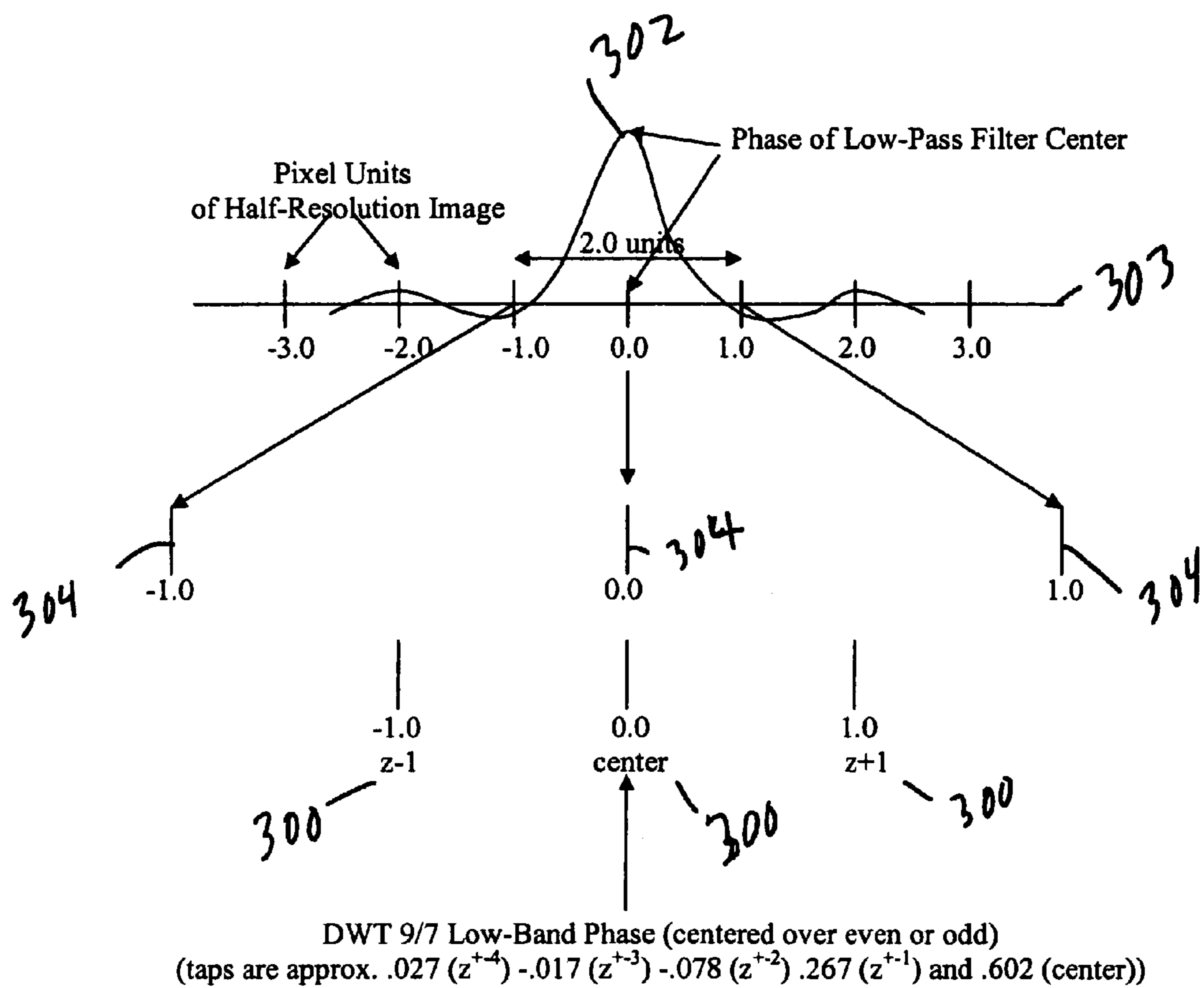
Fig. 3 (Prior Art)
