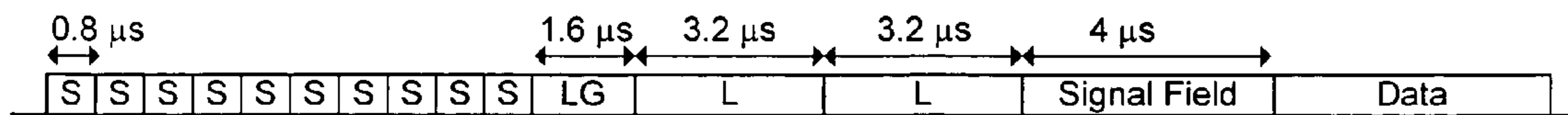
FIG. 1 (PRIOR ART)
