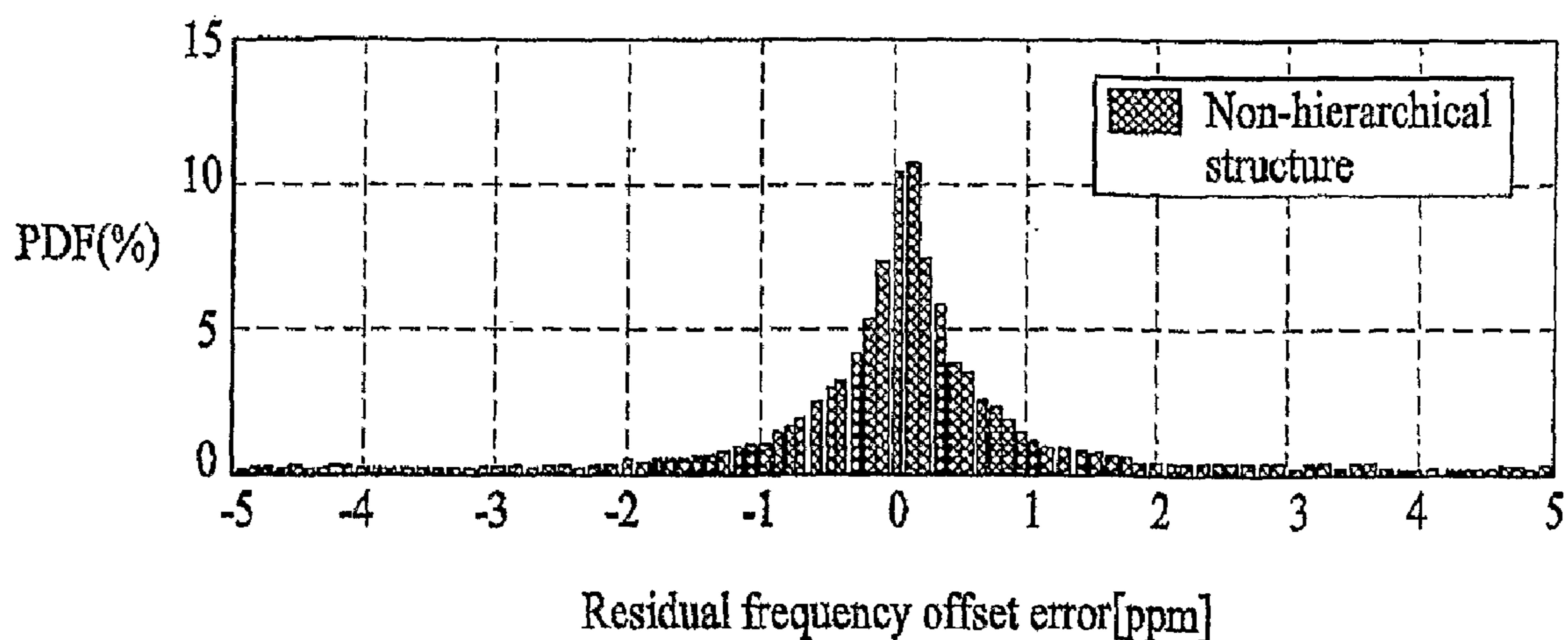
PDF of residual frequency offset error, Asynchronous network
