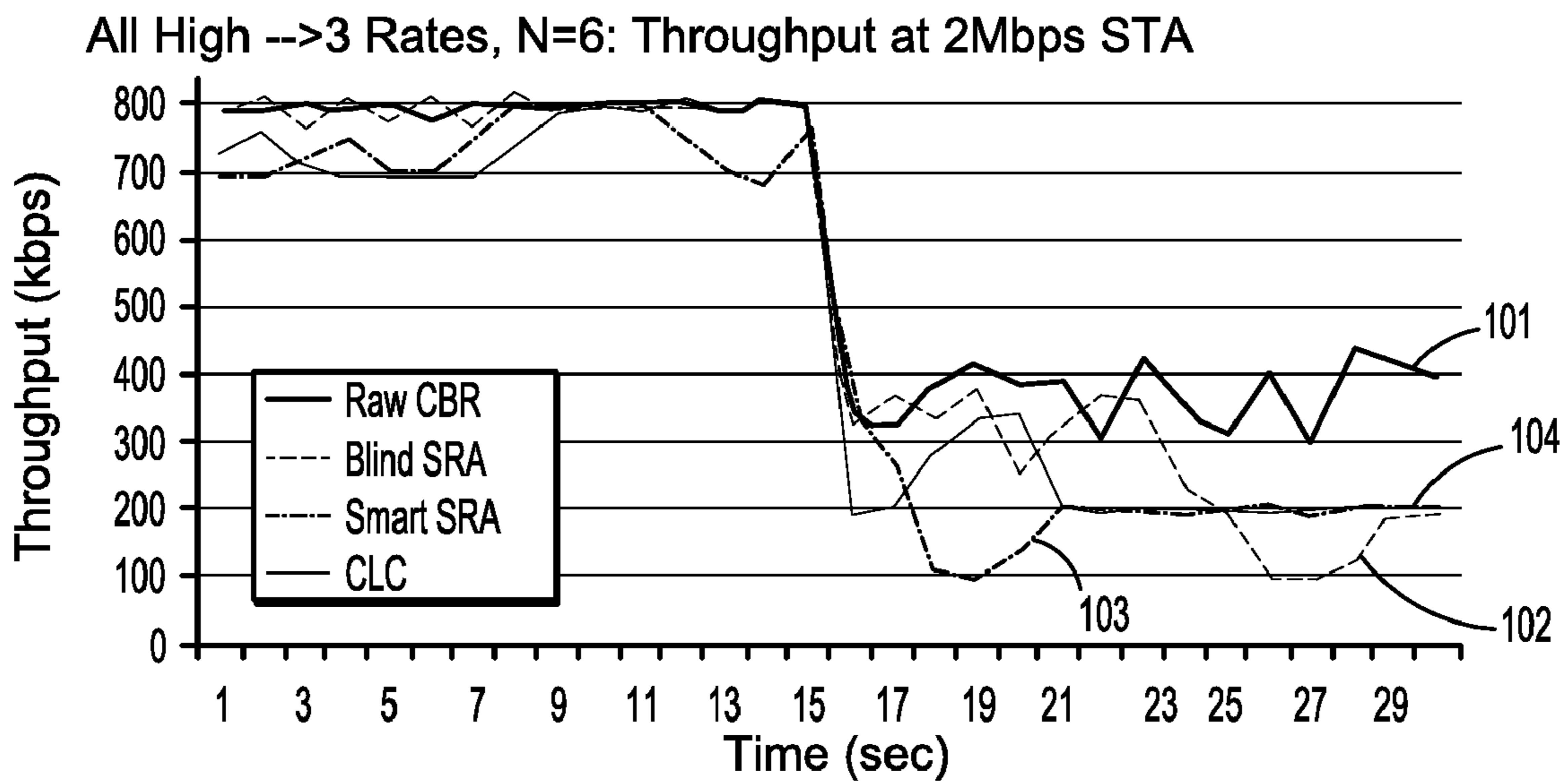
FIG. 10(b) 2 Mbps STA Throughput
