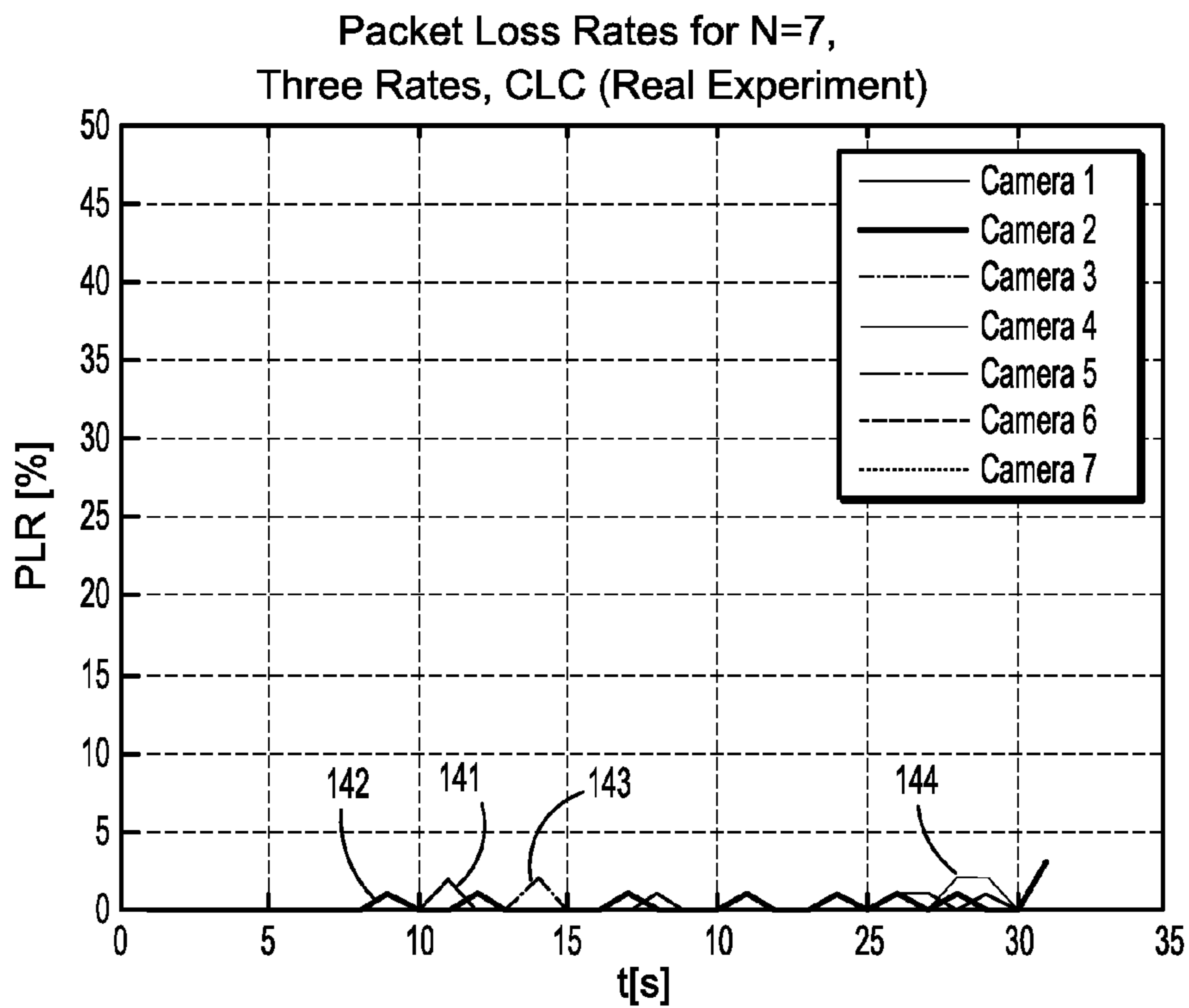
FIG. 14(b) CLC Packet Loss
