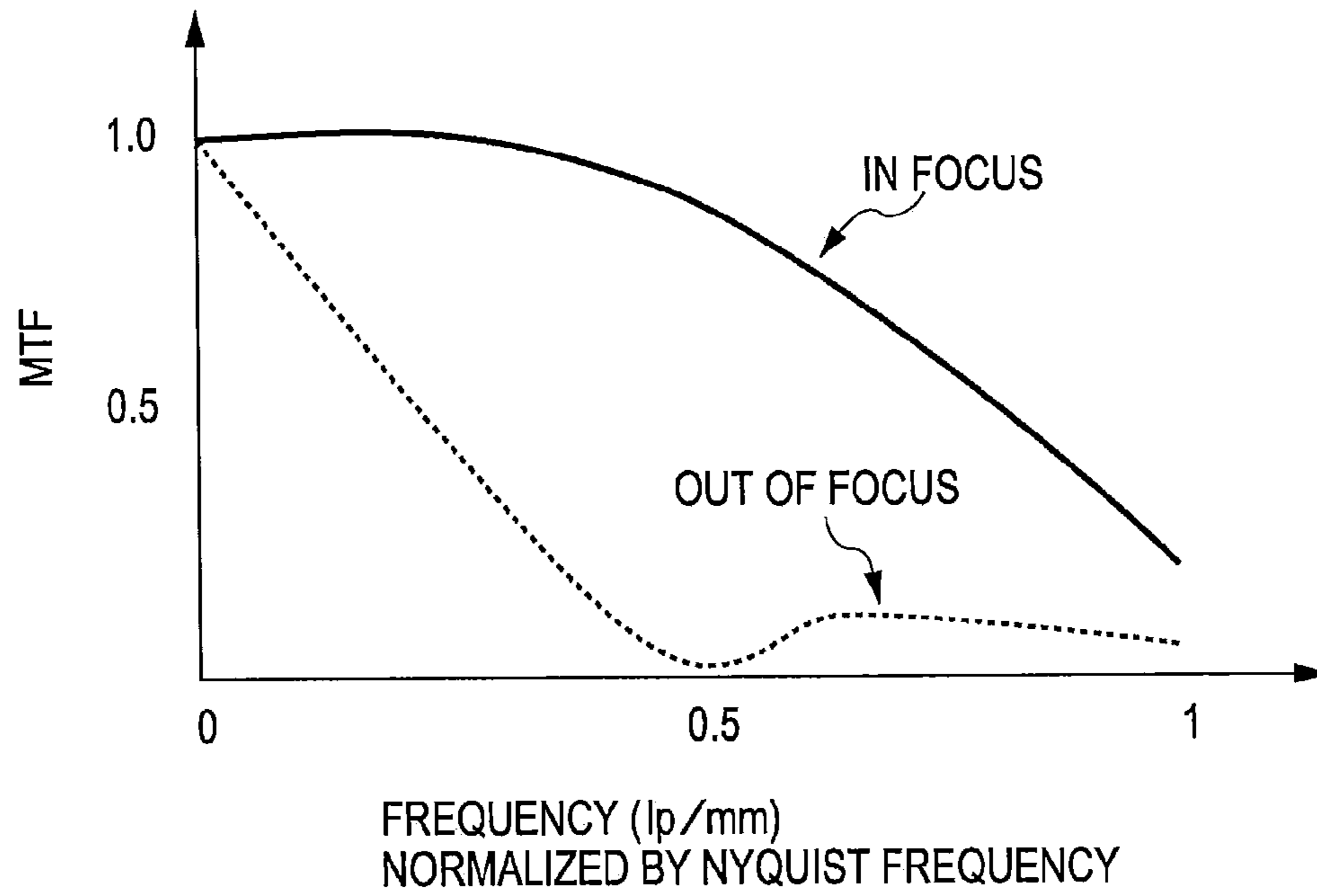
FIG. 24 (PRIOR ART)
