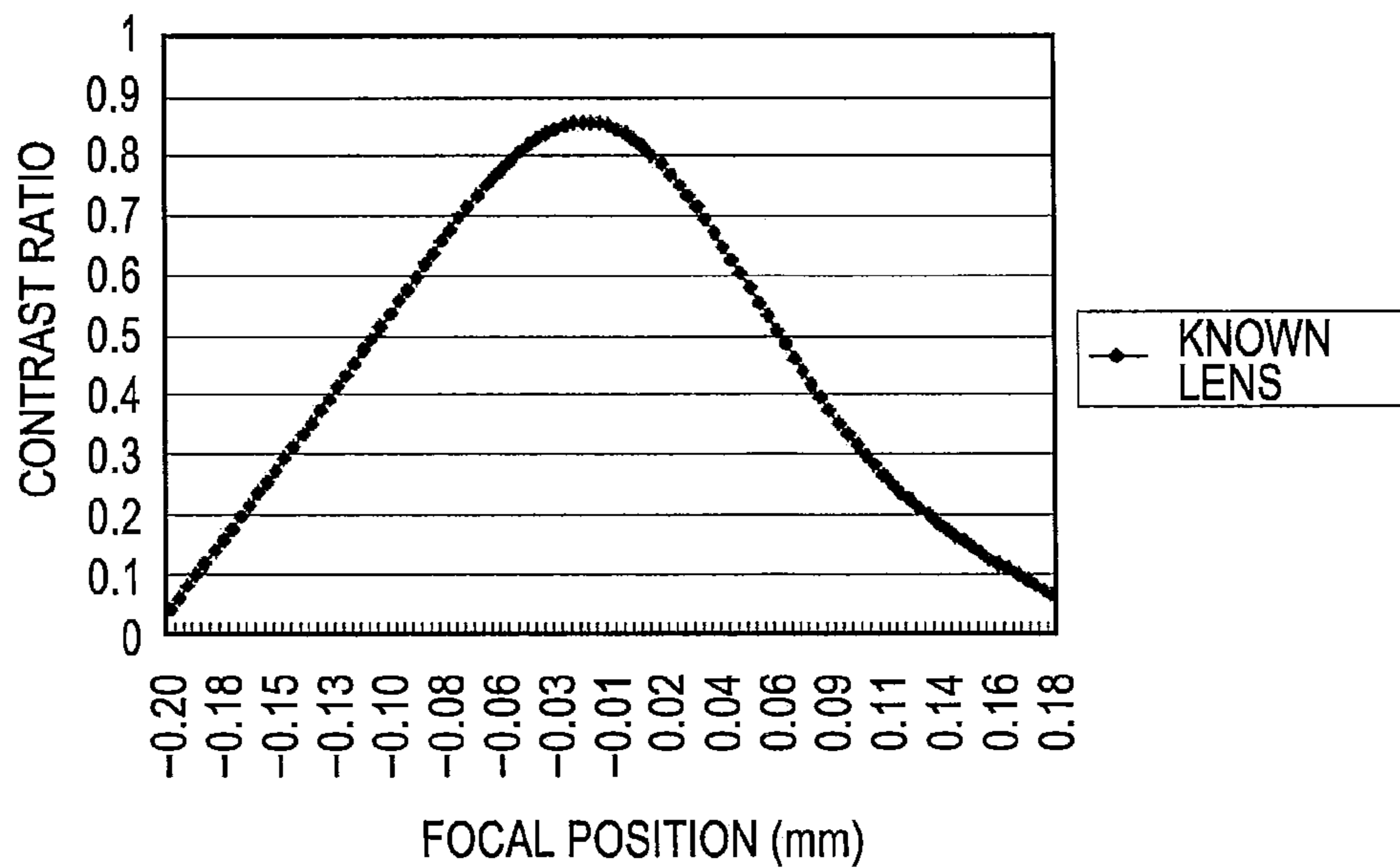
FIG. 16 (PRIOR ART)
