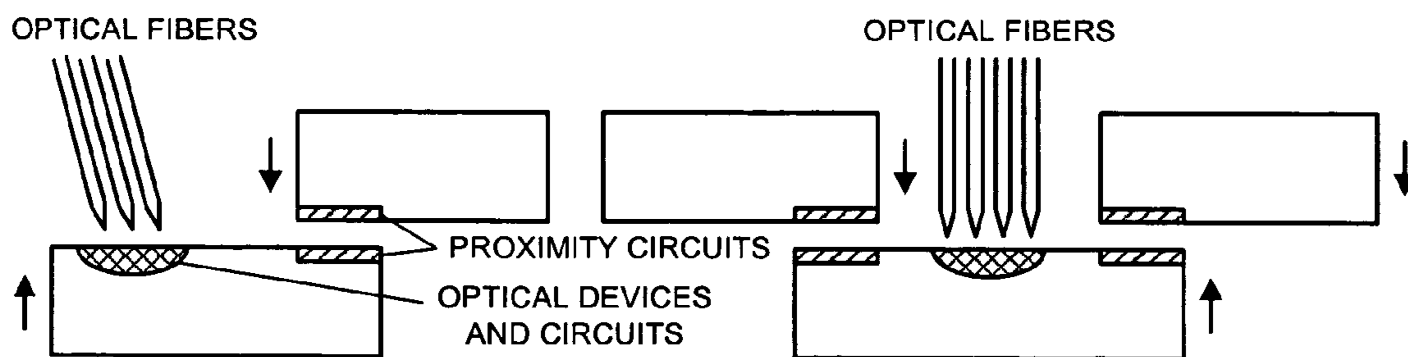
FIG. 3 (PRIOR ART)
