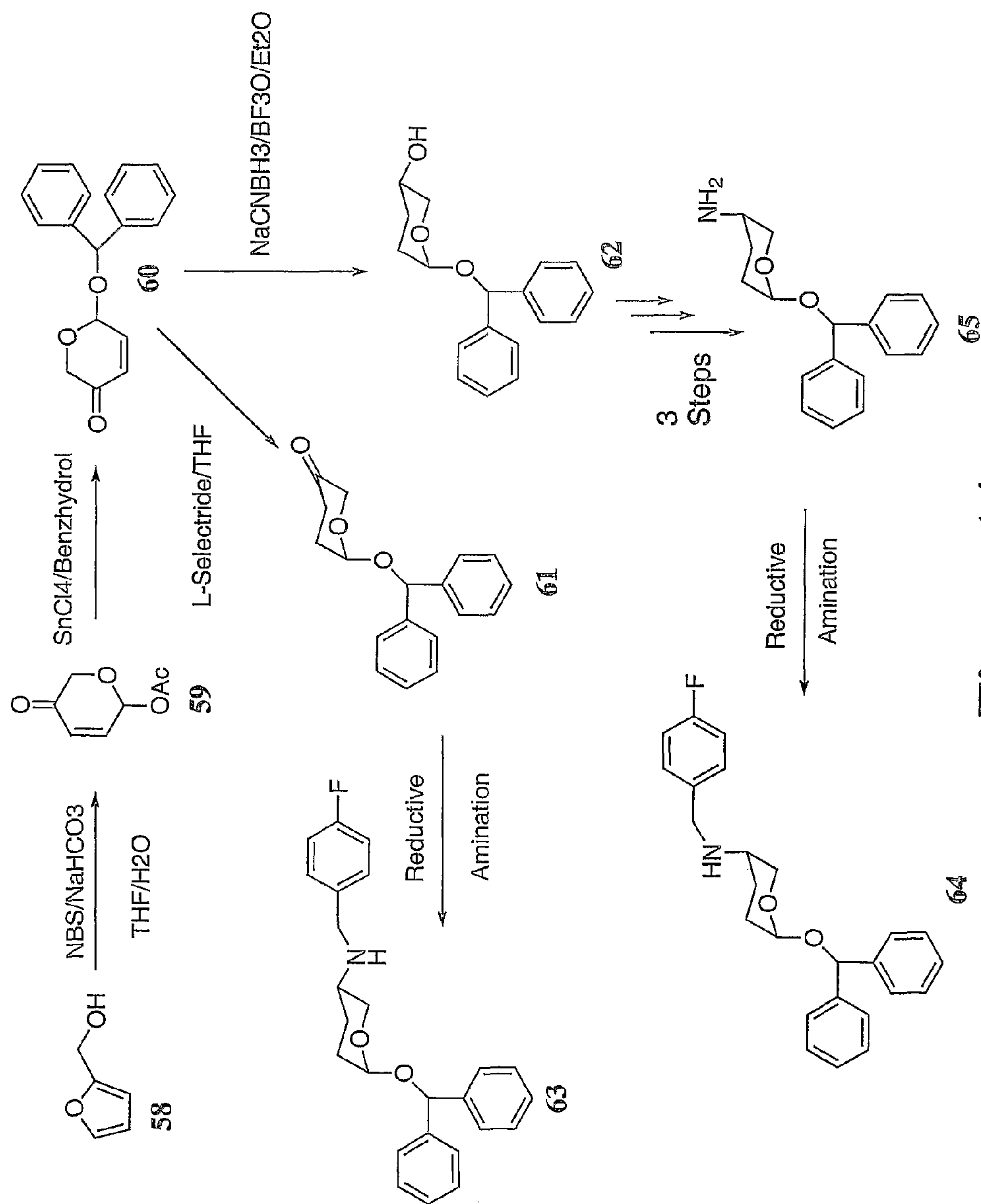
Scheme 9
