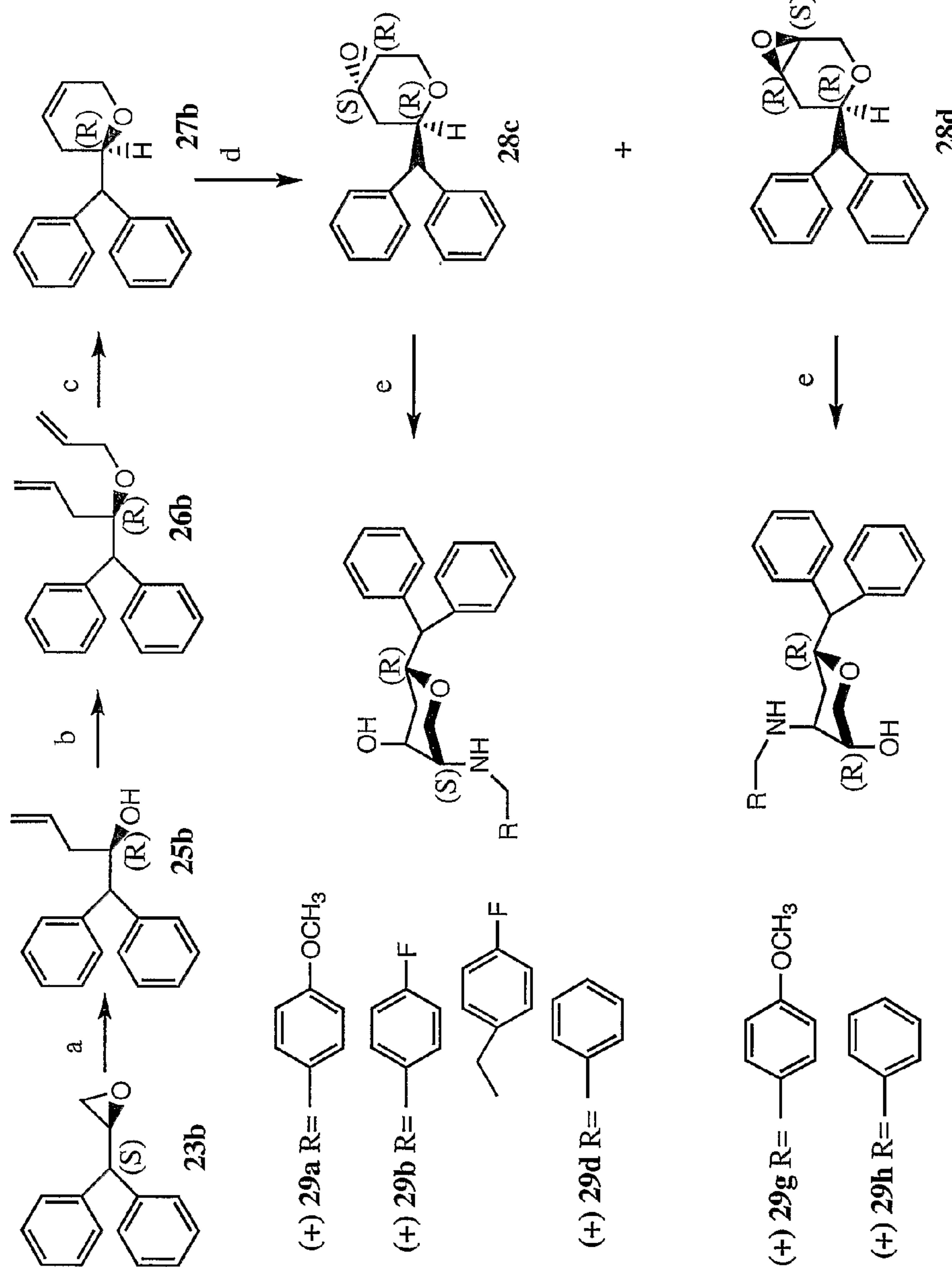
Scheme 3
