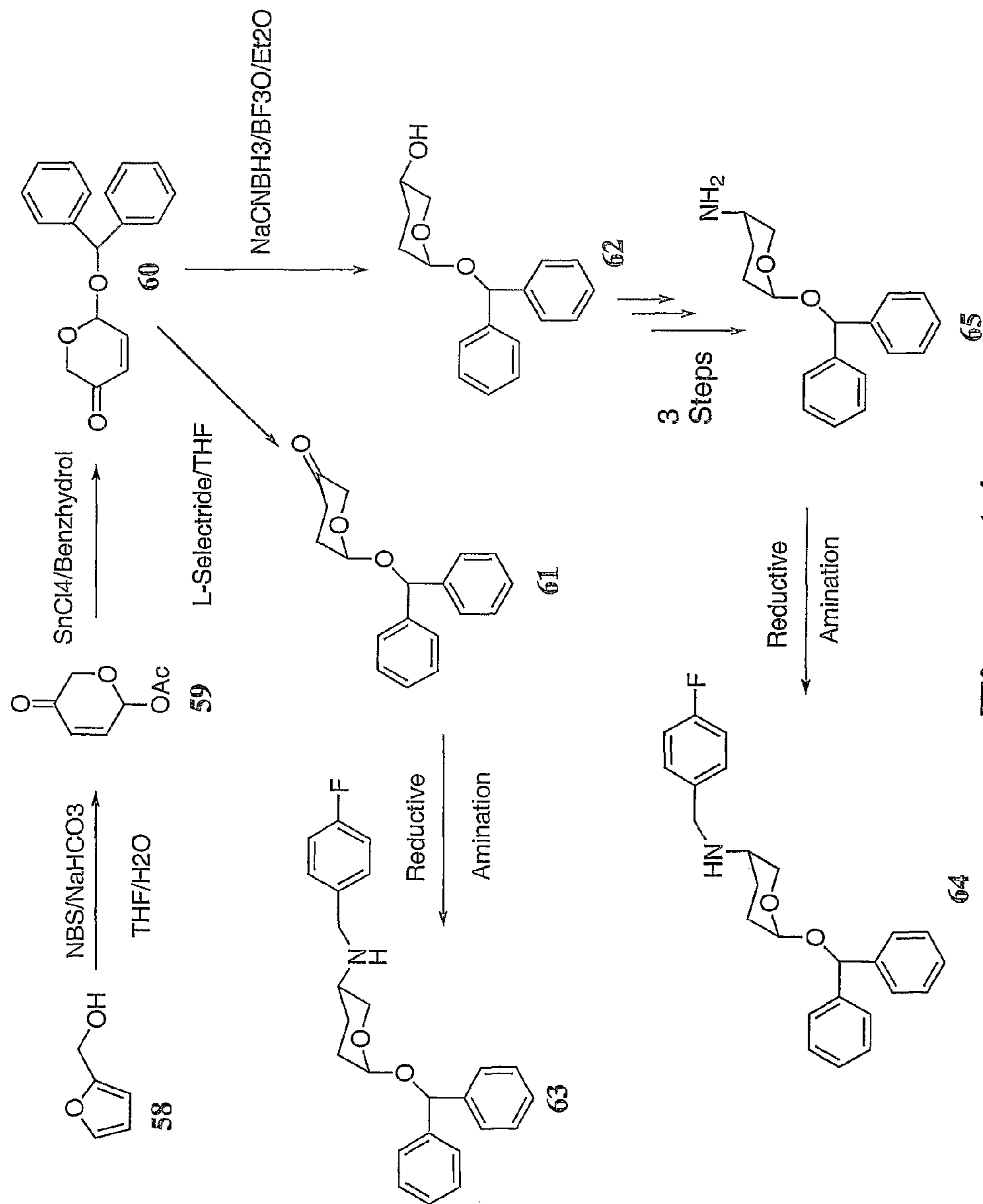
Scheme 9
