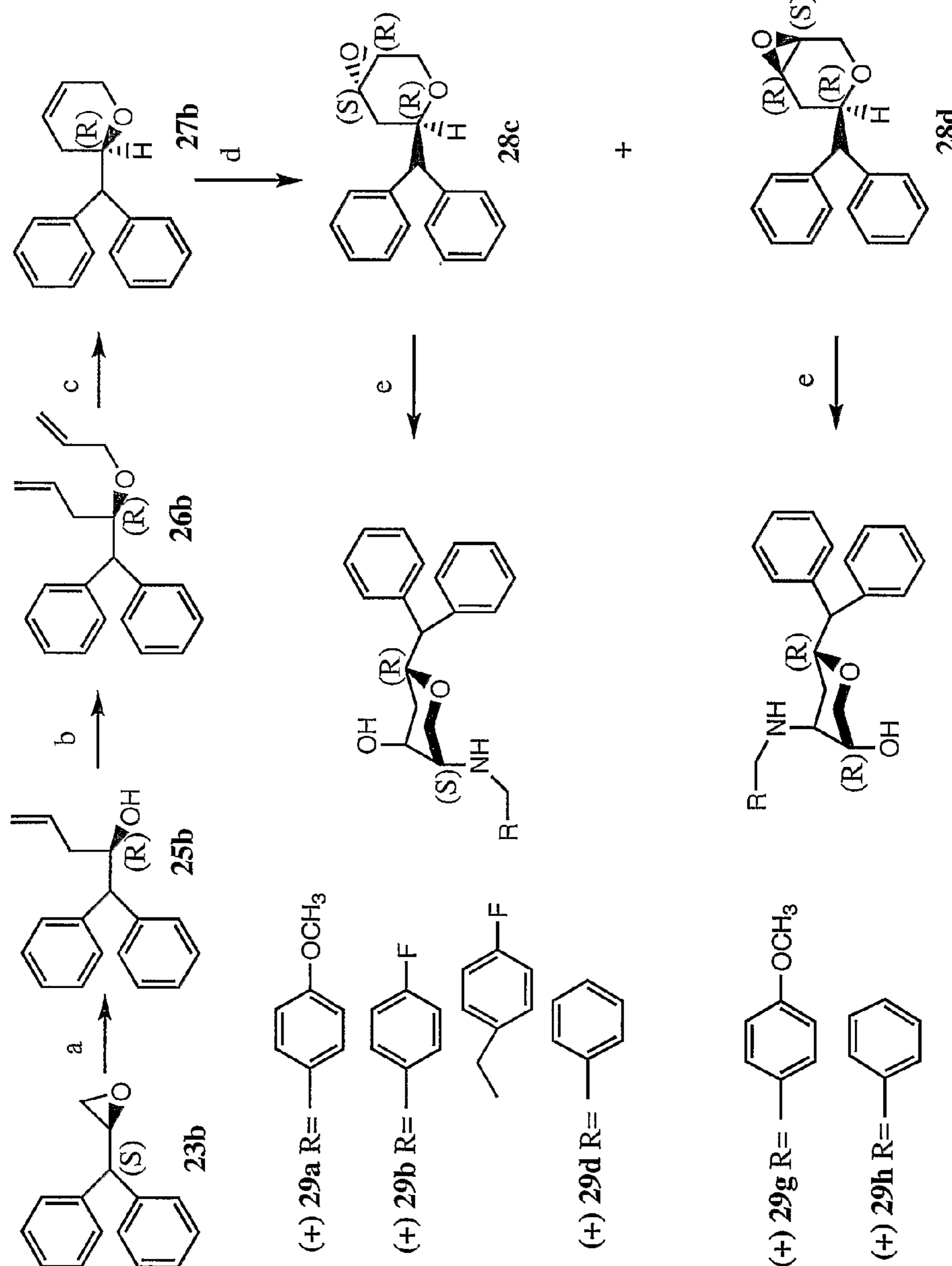
Scheme 3
