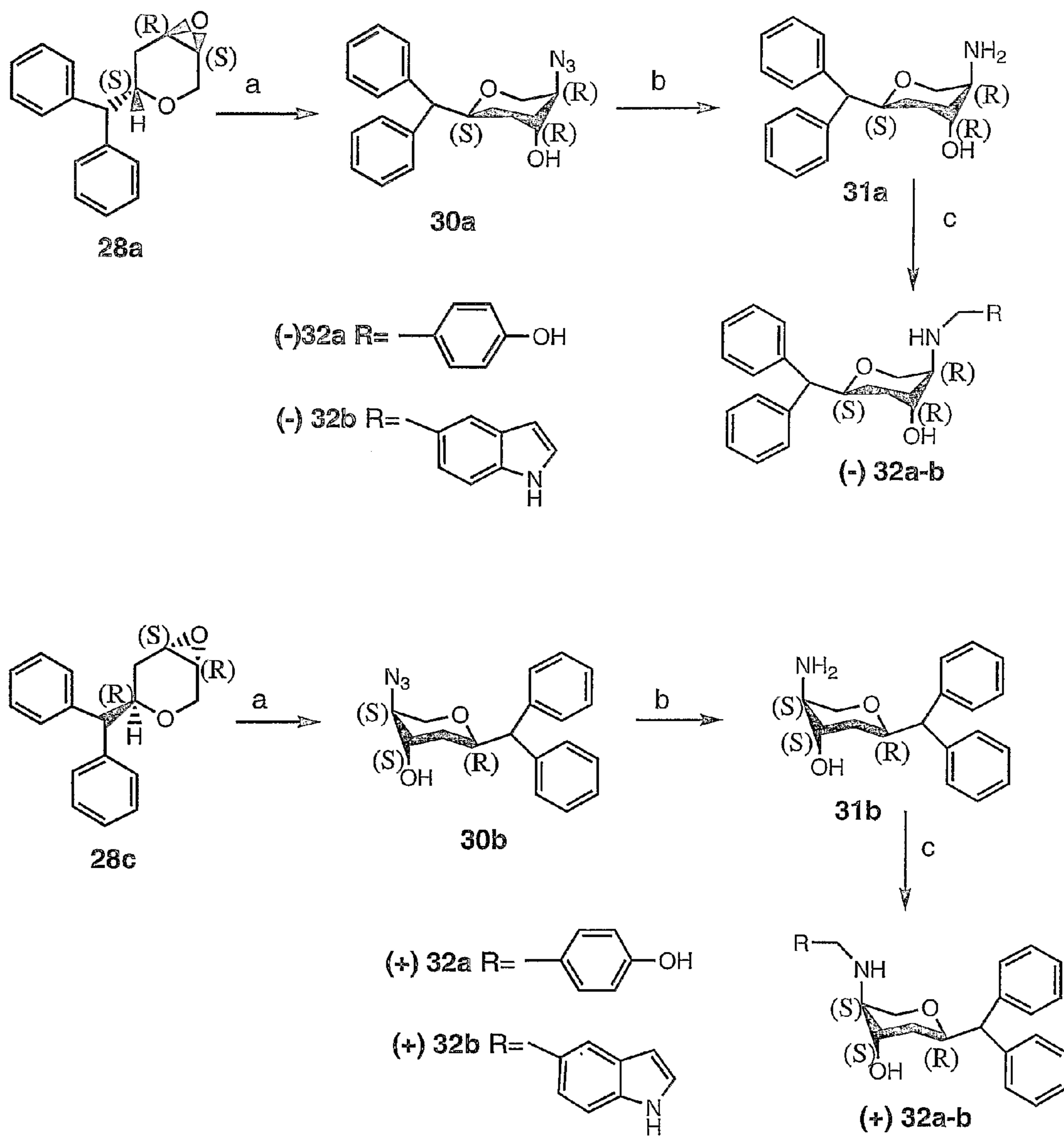
Scheme 4
