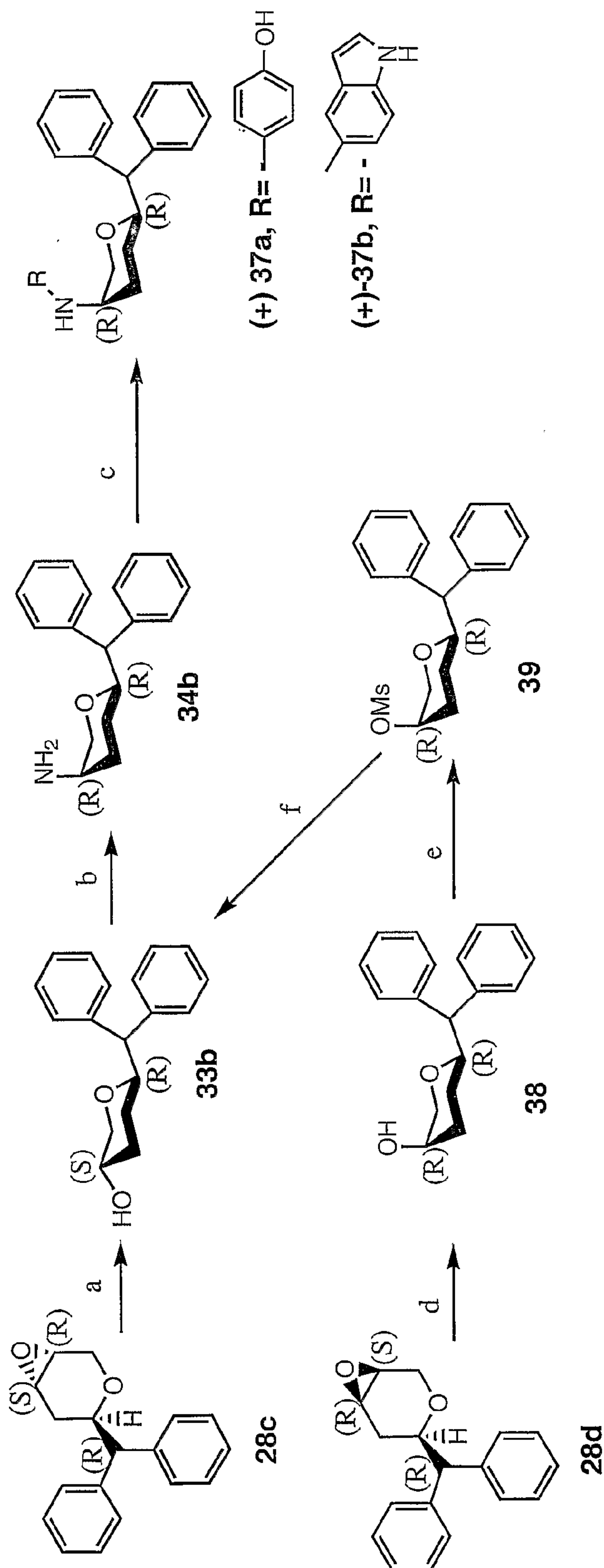
Scheme 6
