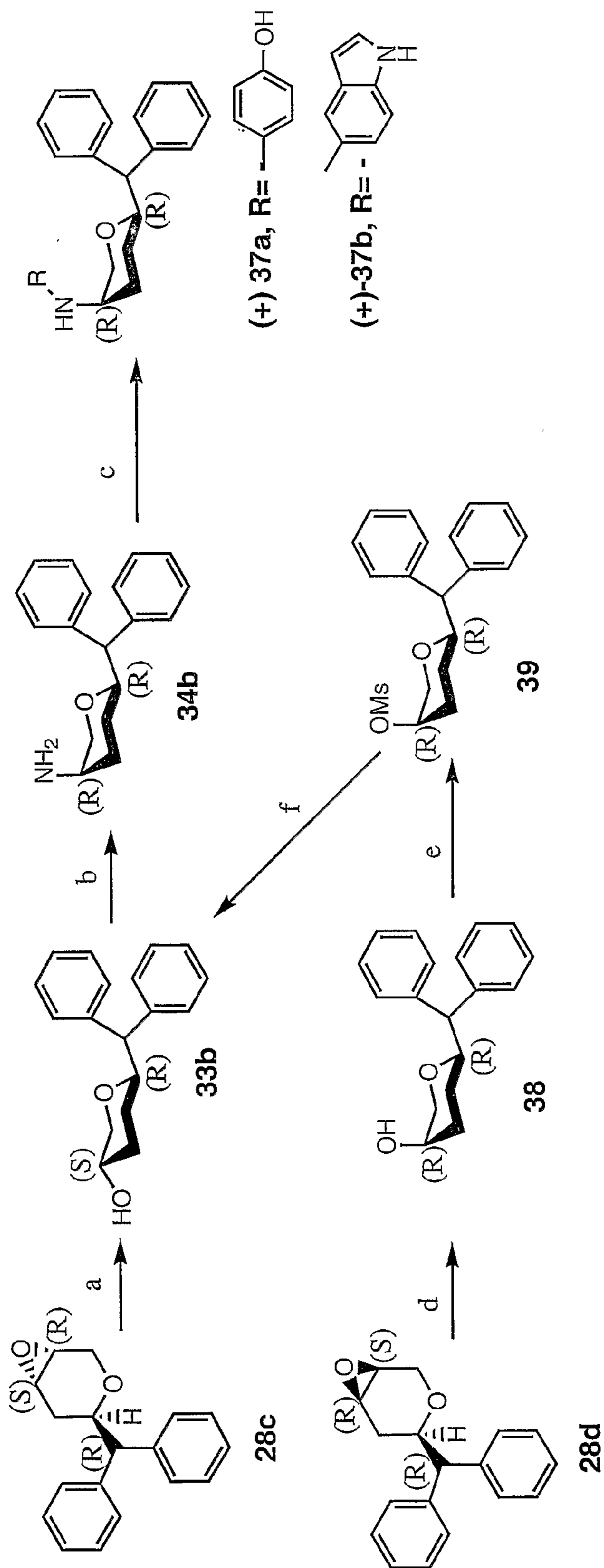
Scheme 6
