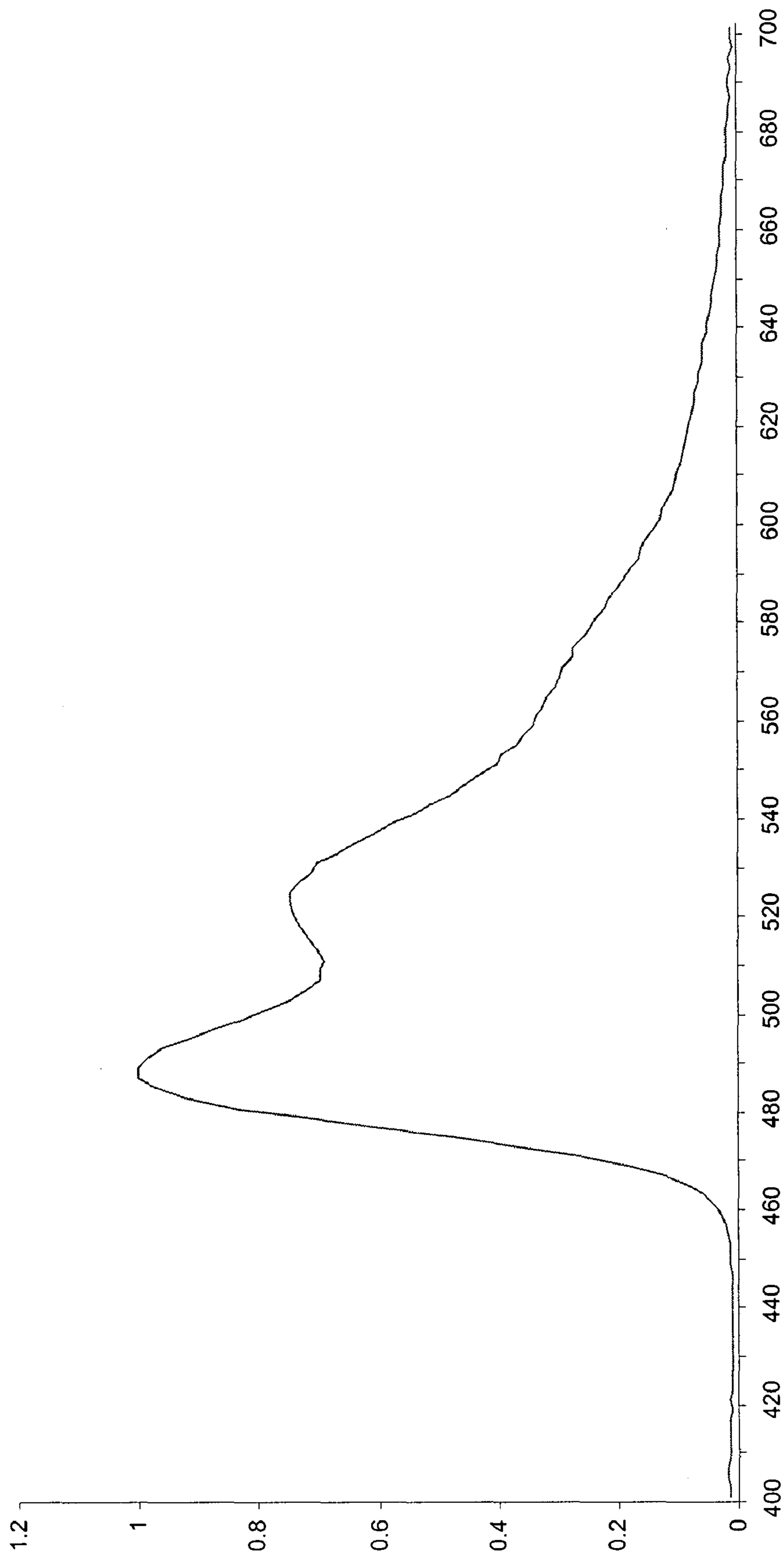
Figure 14. Emission spectrum of es101 in methylene chloride solution
