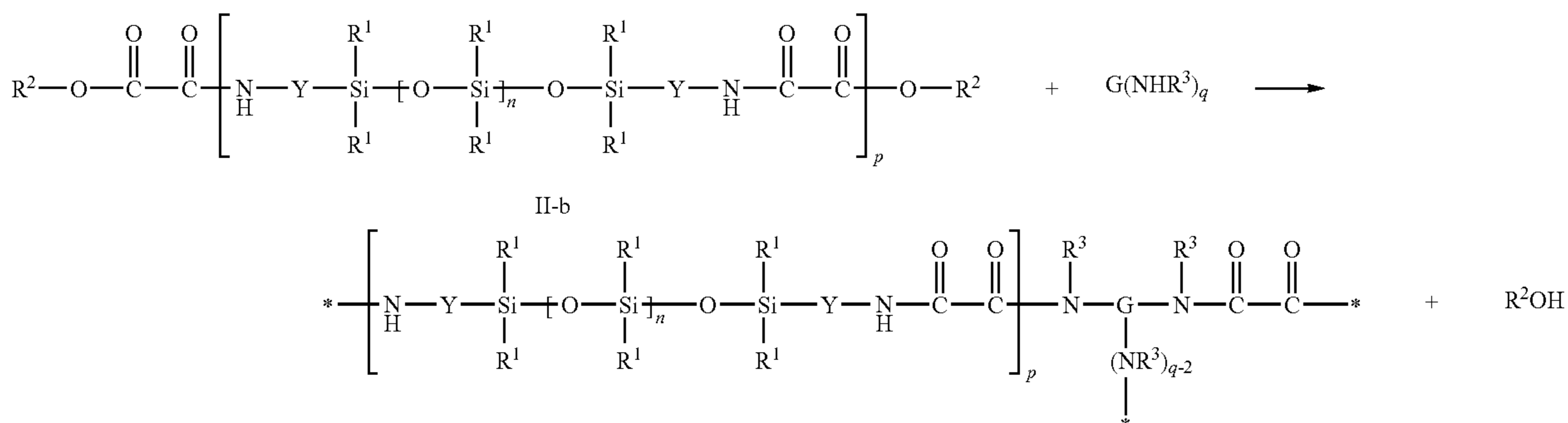
Reaction Scheme A-2
