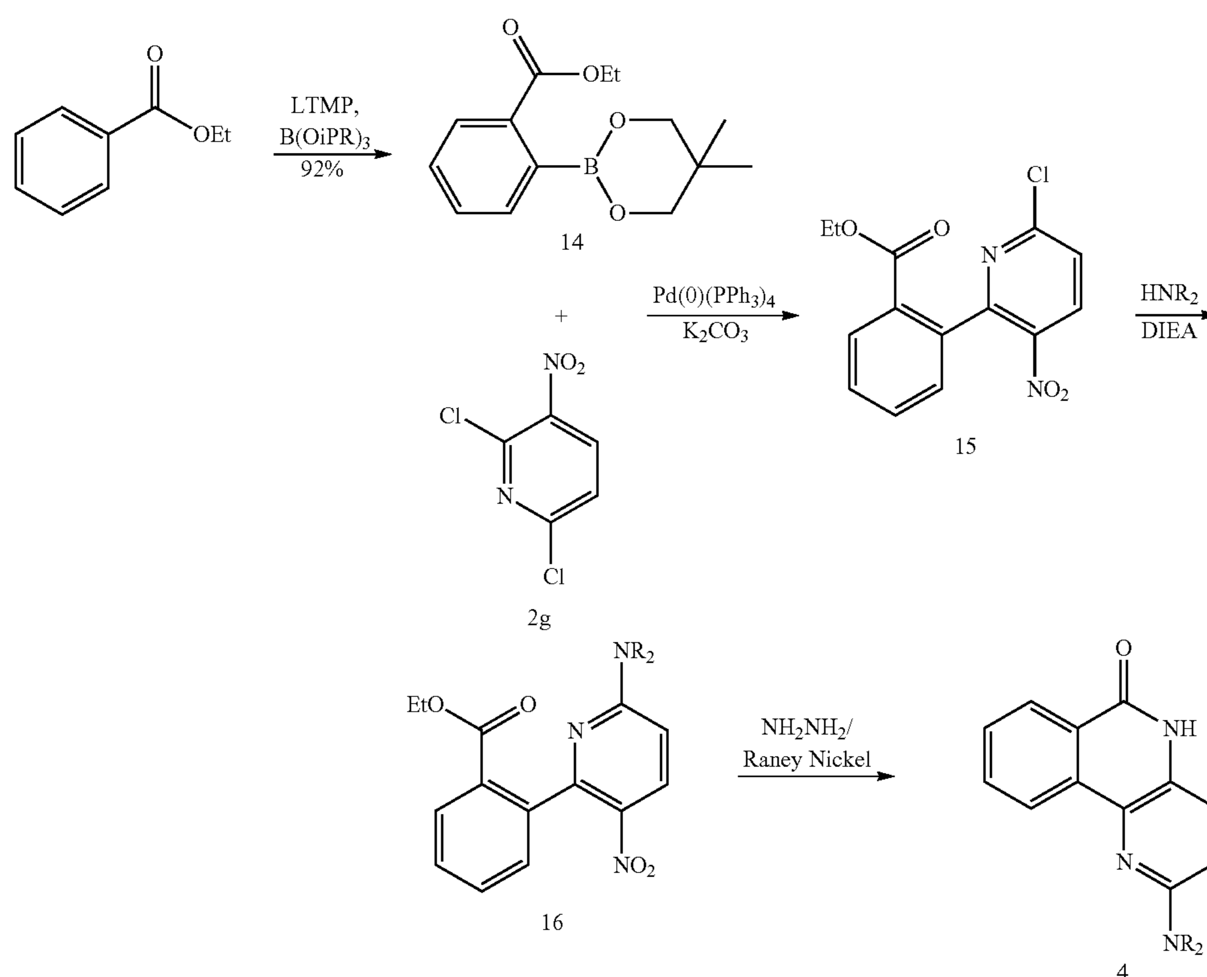
Scheme 9-5. Alternate synthesis of amines 4a-x.
