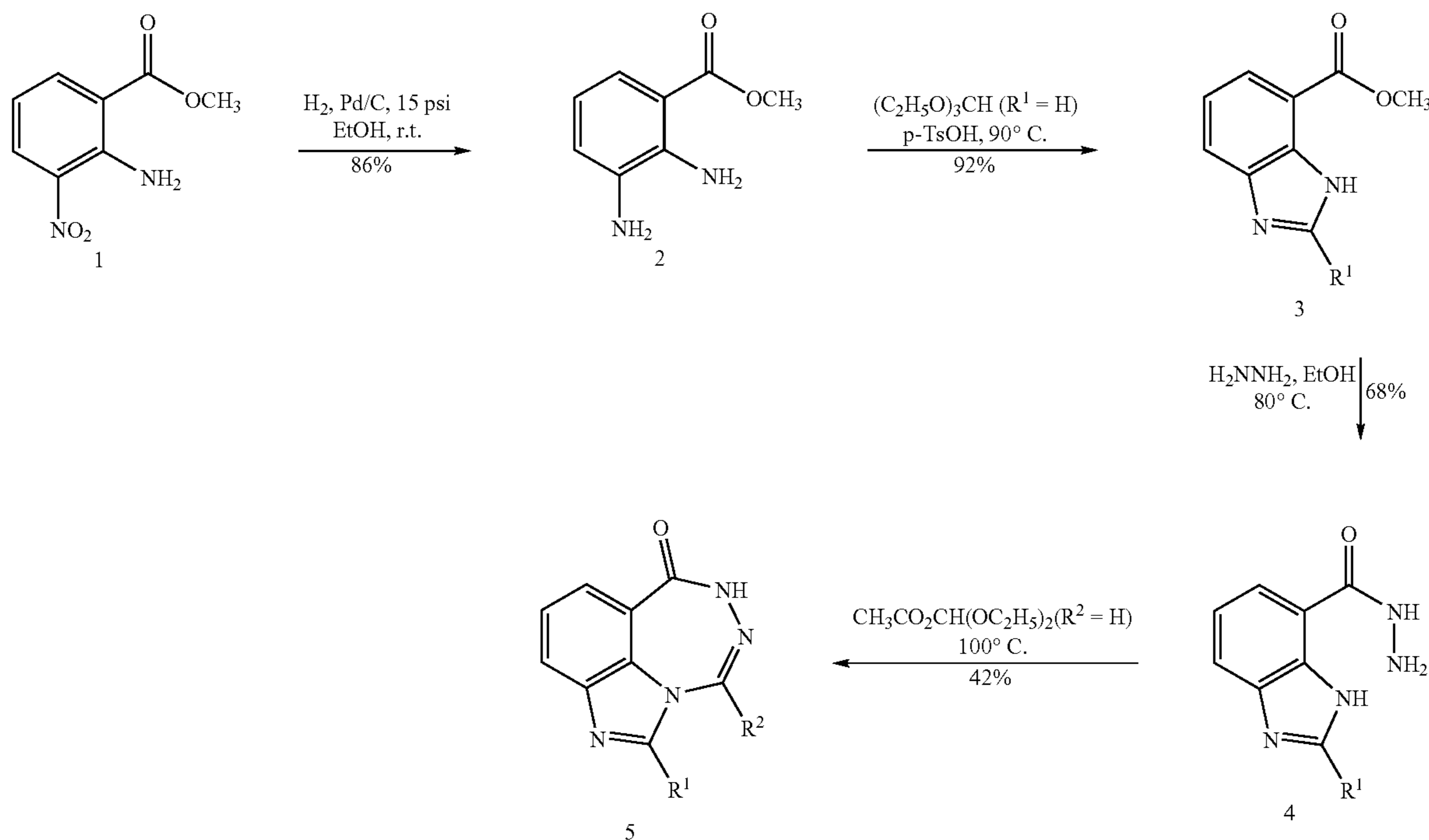
Scheme 1-7 Synthesis of Imidazolobenz-1,3,4-triazepin-5-one
