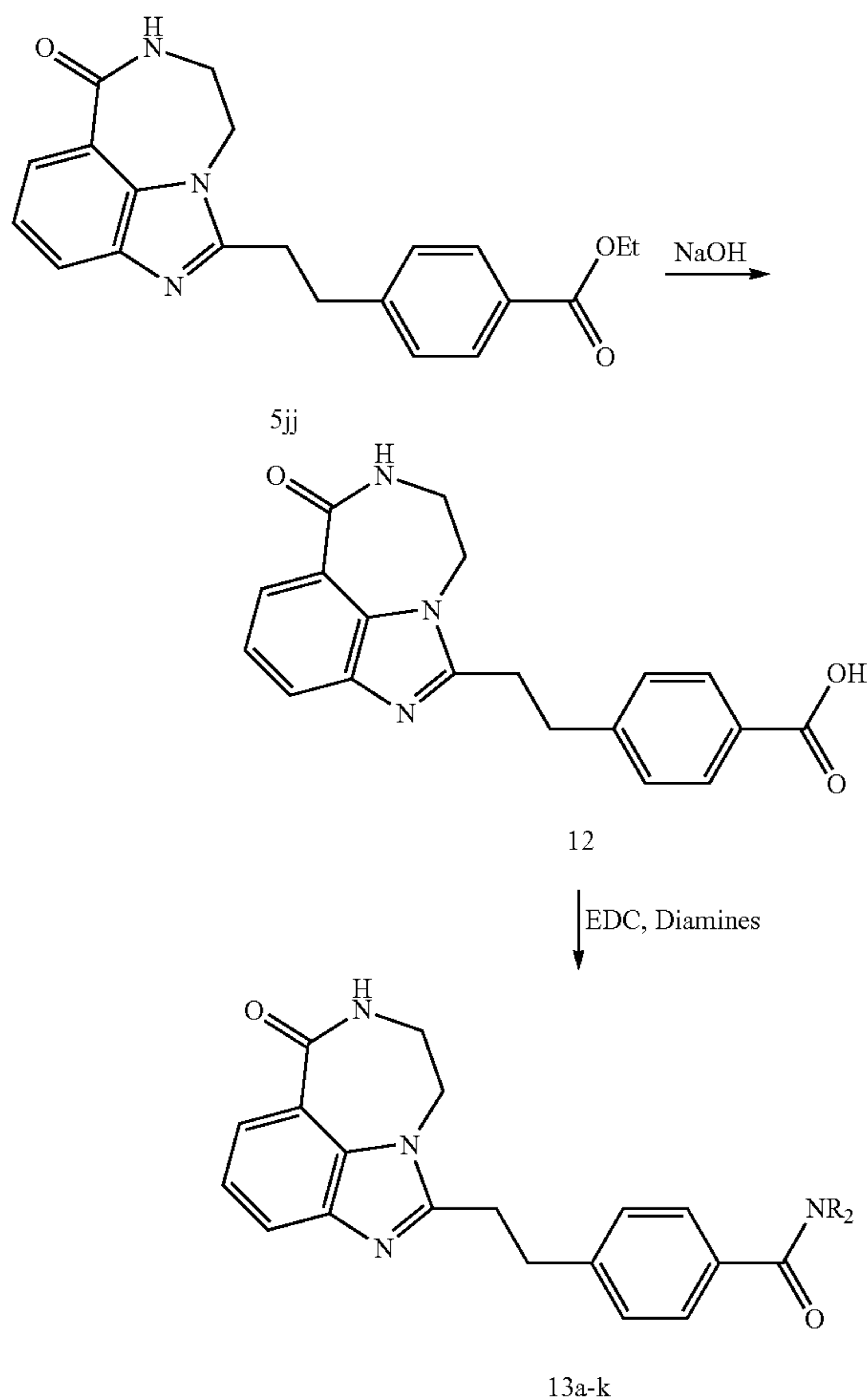
Scheme 7-4. Synthesis of amides 13a-k.
