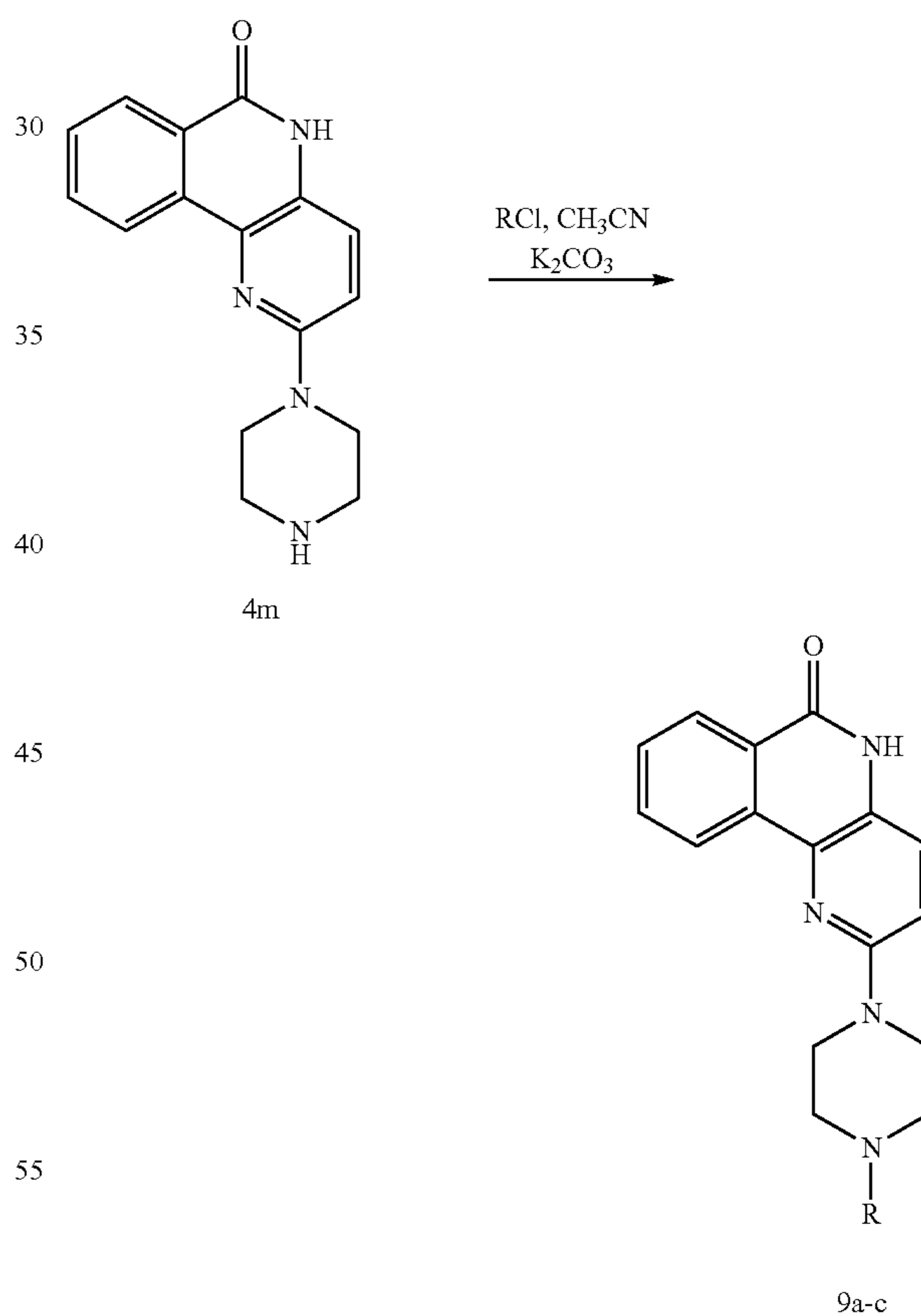
Scheme 6-5. Synthesis of amines 9a-c.
