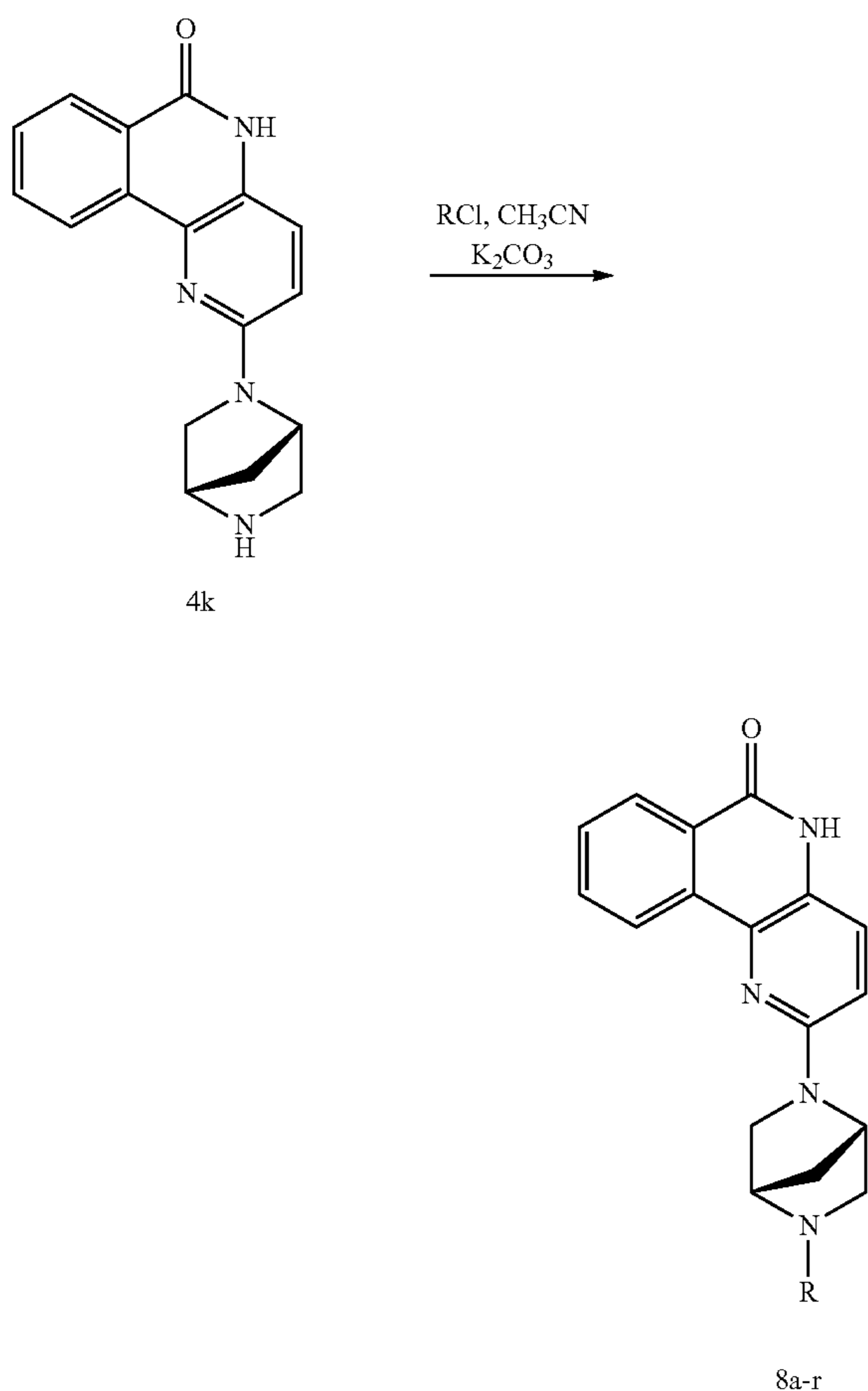
Scheme 5-5. Synthesis of the amines 8a-r.
