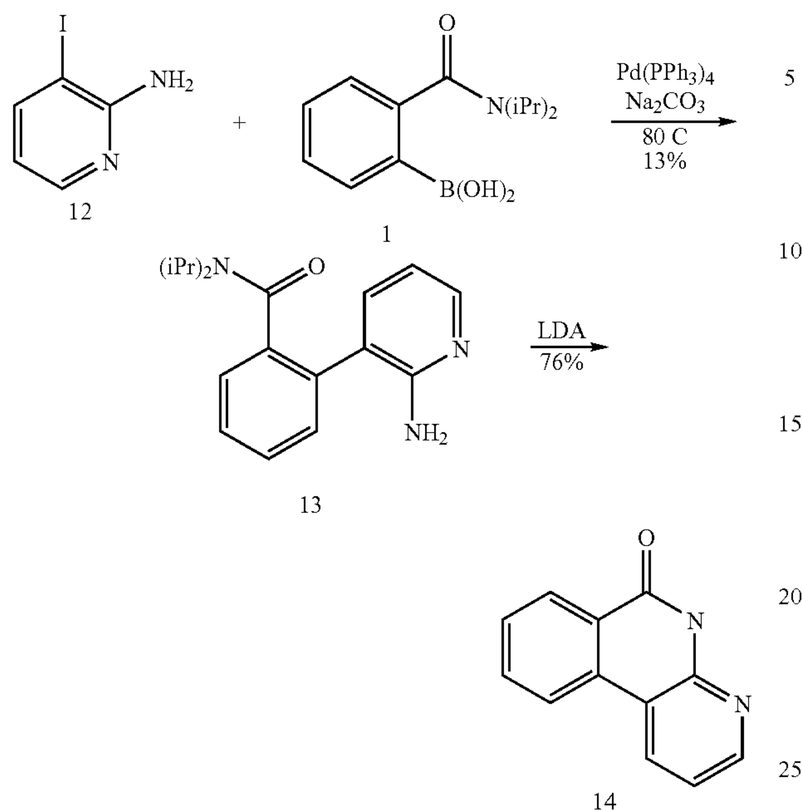
Scheme 1-9. General synthesis of 4-azaphenanthridones 14.
