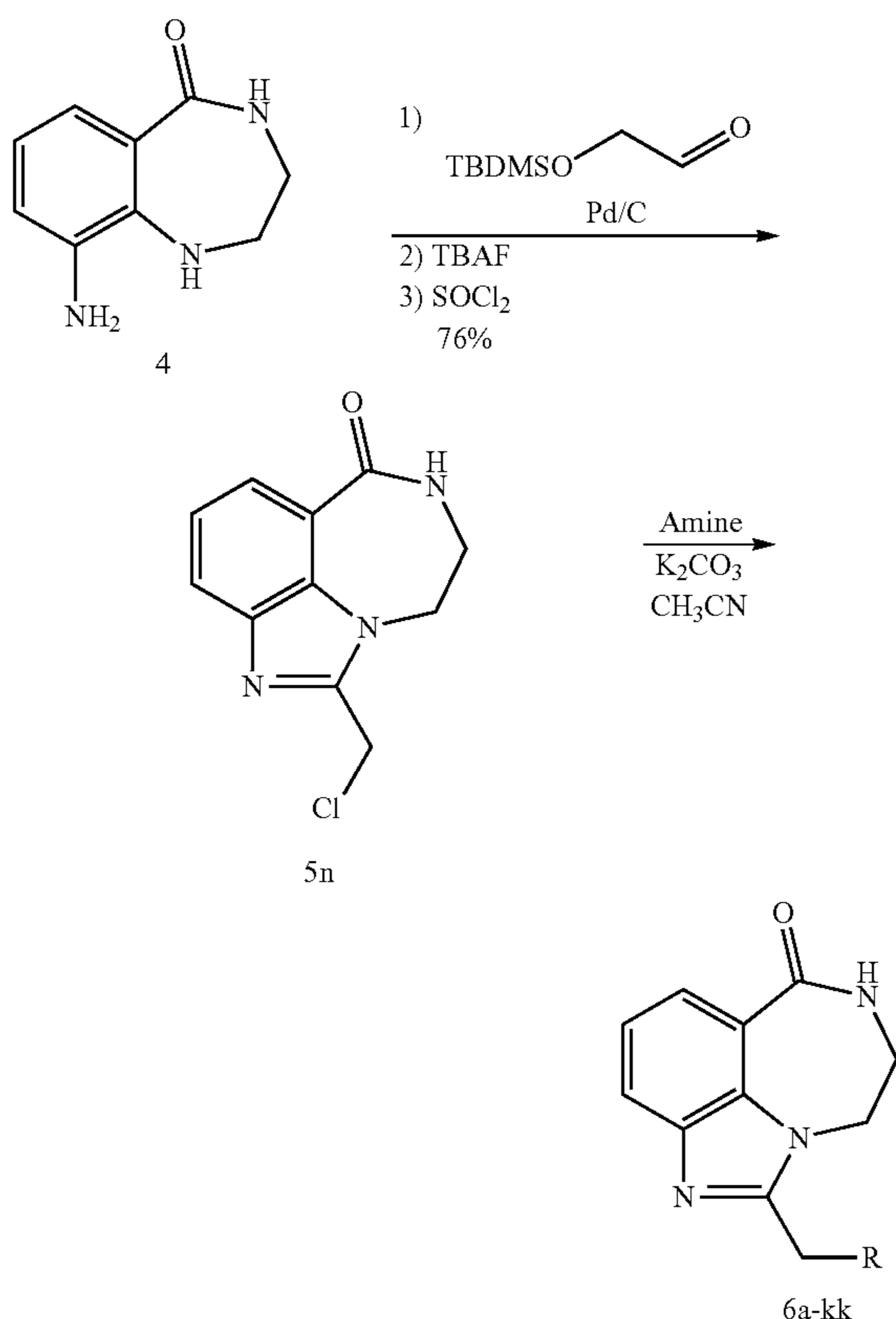
Scheme 3-4a Alternate Synthesis of imidazobenzodiazepine amines 6a-kk
