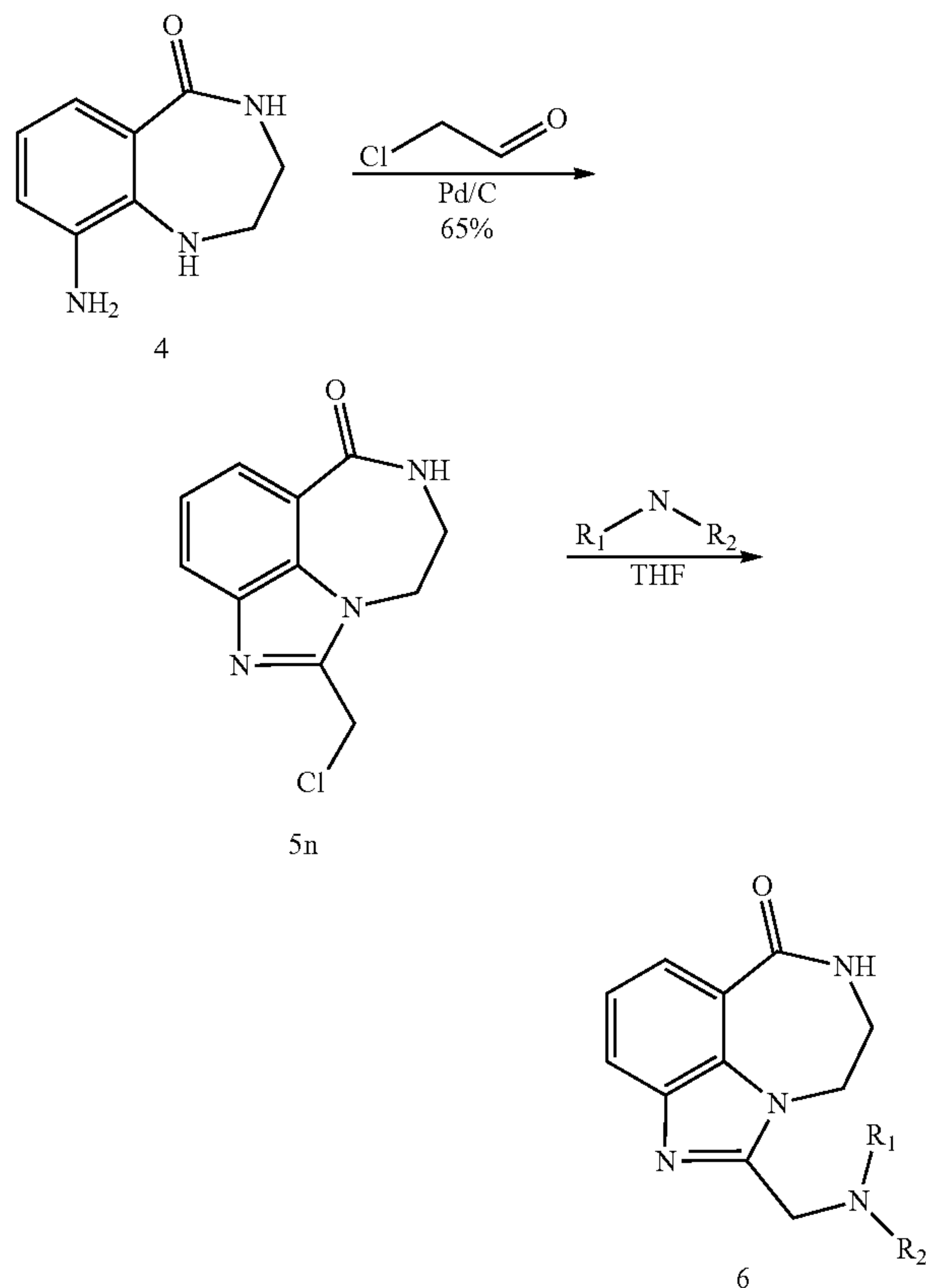
Scheme 3-4 Synthesis of imidazobenzodiazepine amines 6a-dd.
