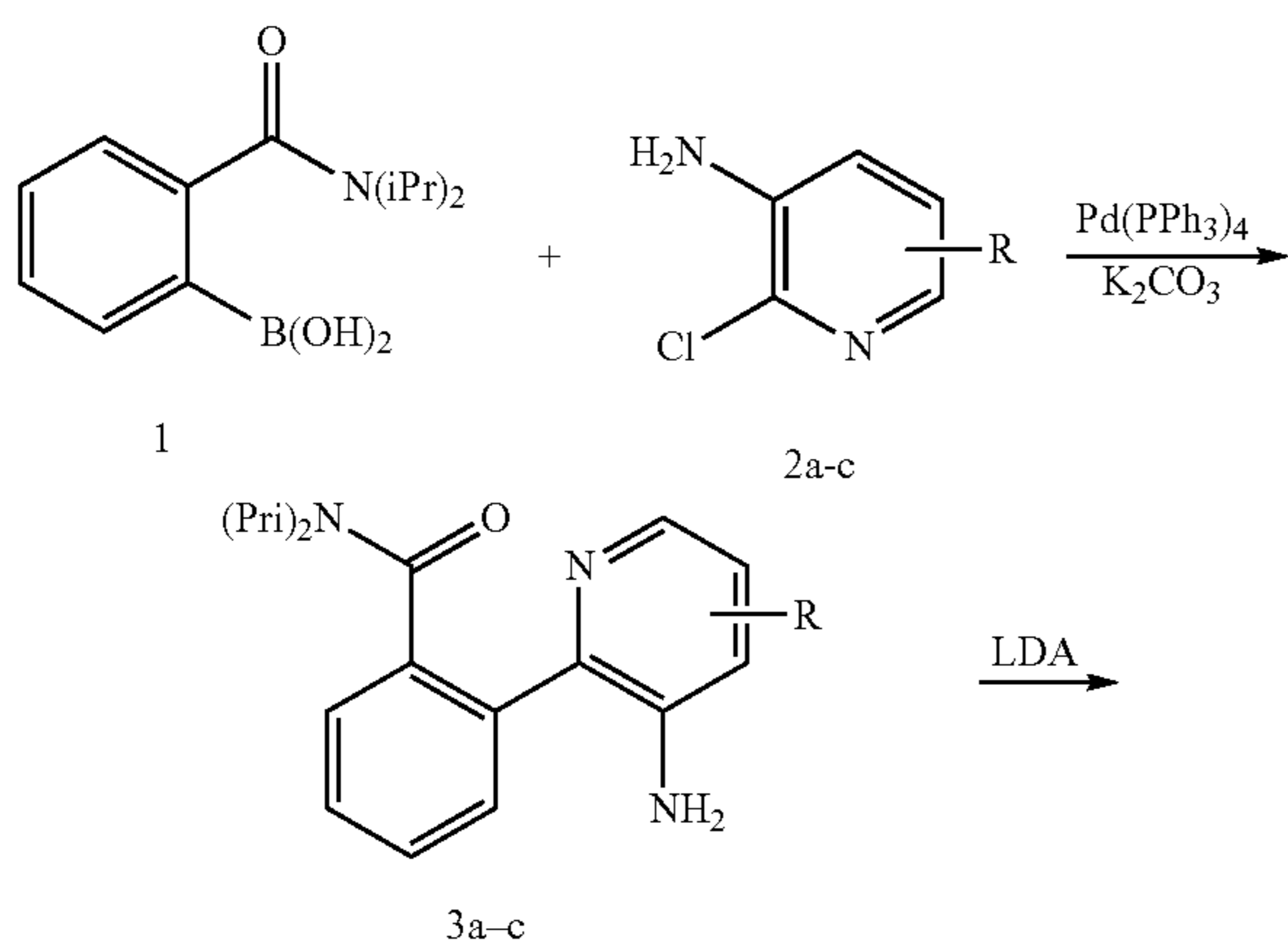
Scheme 1-5. General Scheme for synthesis of azaphenanthridones 4a-c.
