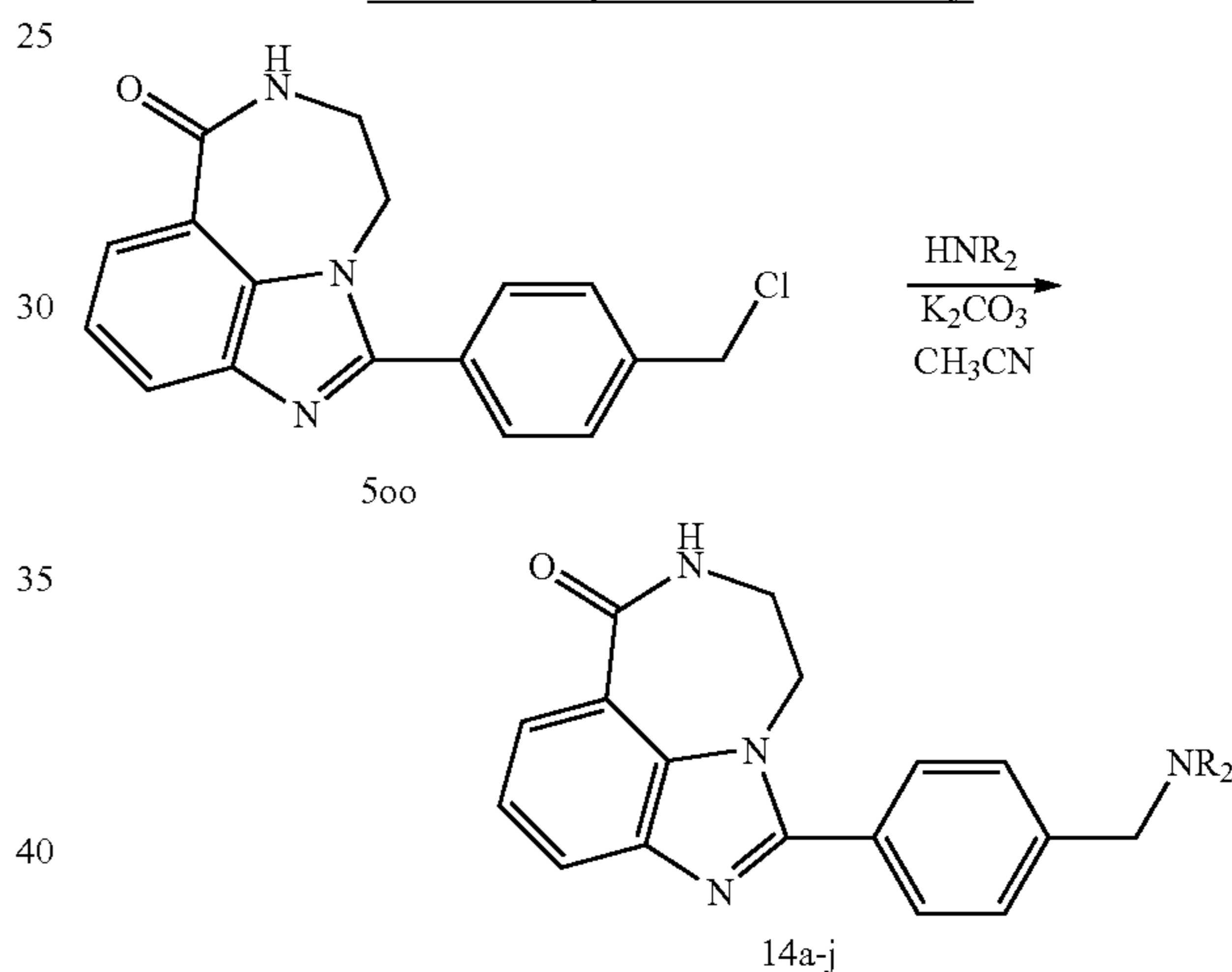
Scheme 8-4. Synthesis of amides 14a-j.
