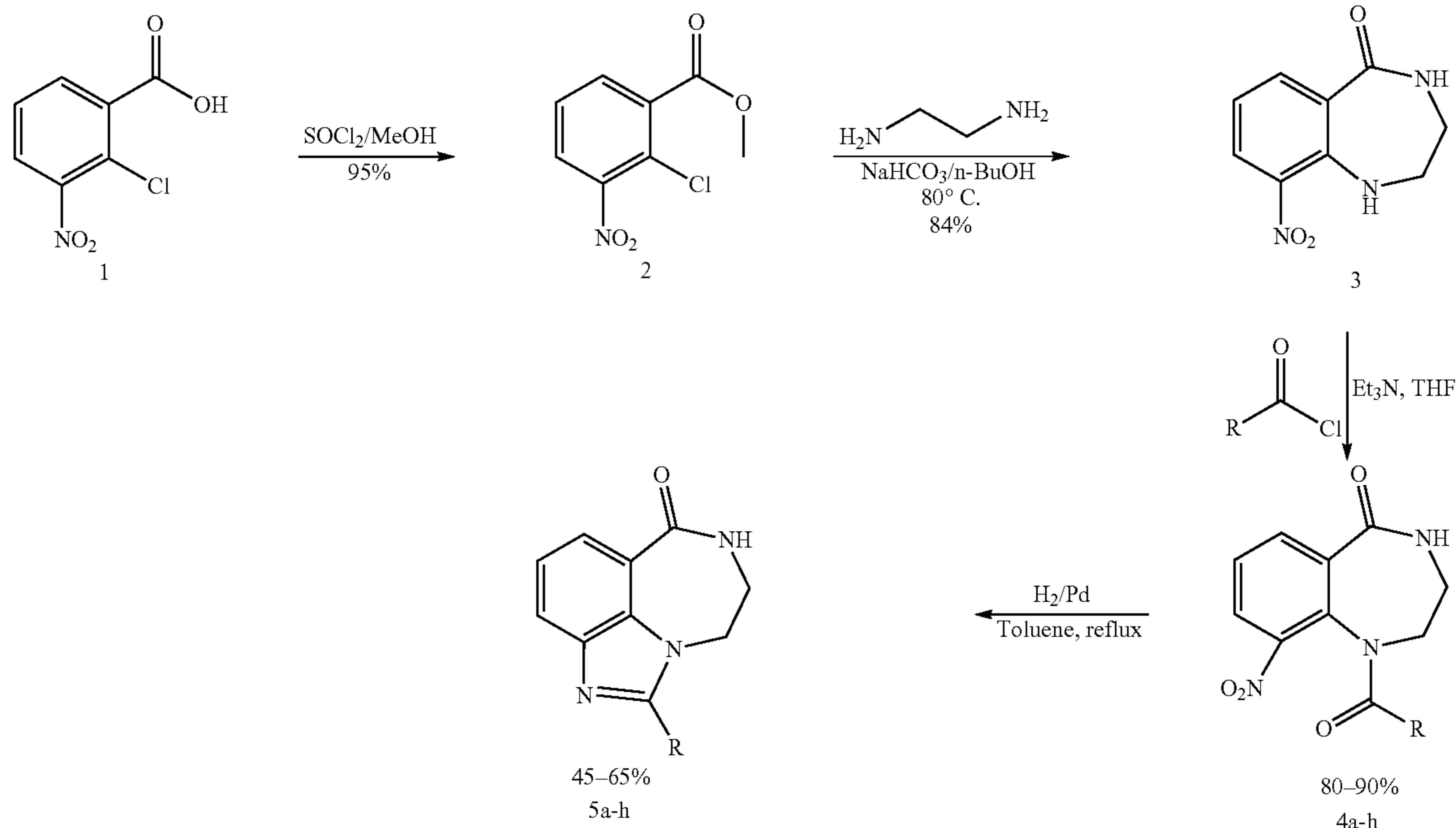
Scheme 1-4. General Synthesis of imidazo benzodiazepines:
