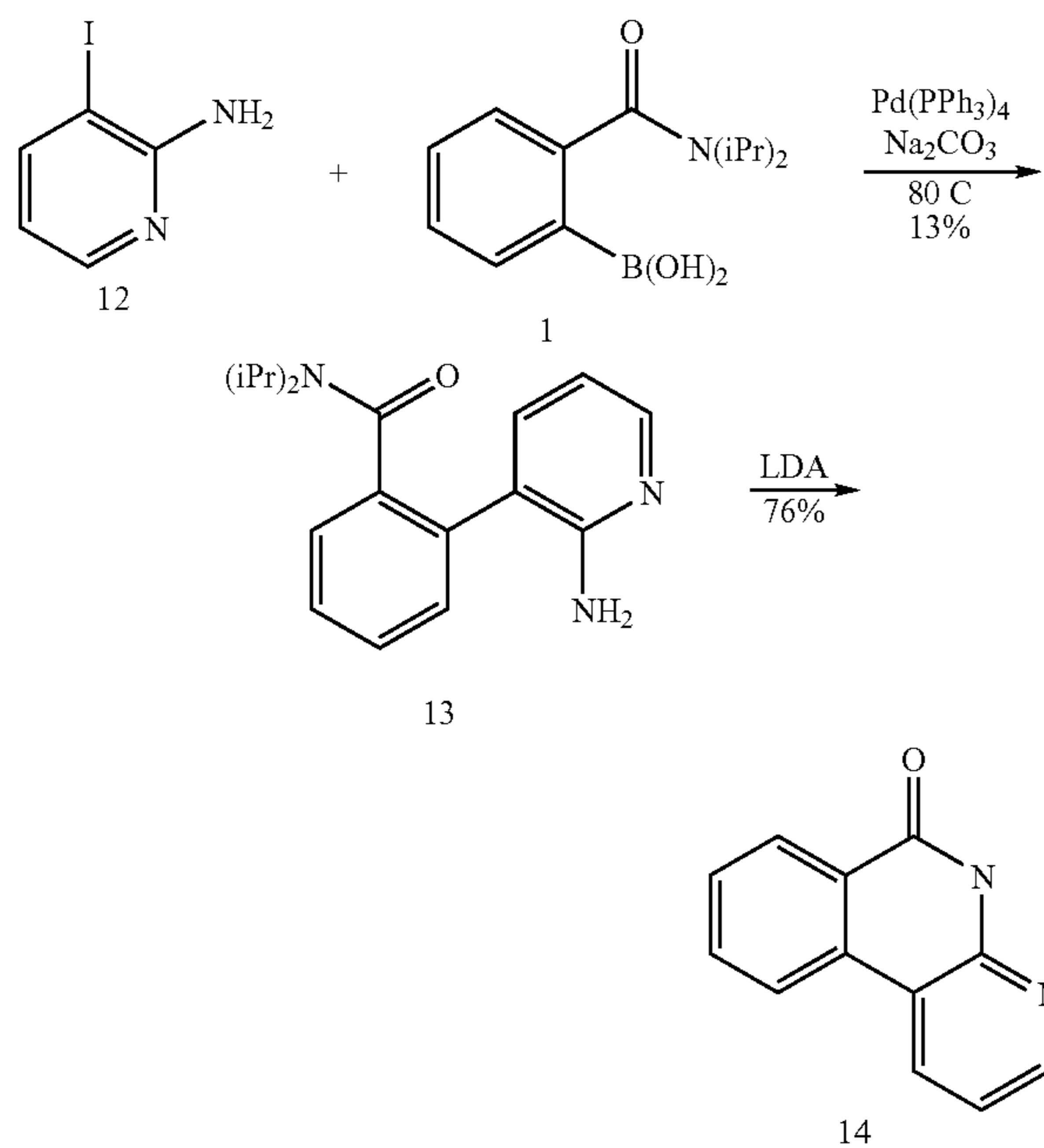
Scheme 1-9. General synthesis of 4-azaphenanthridones 14.
