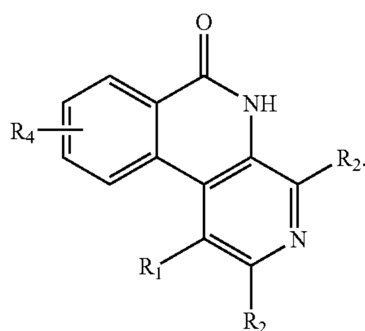
Scheme 1-10. General Synthesis of 3-azaphenanthridones.
