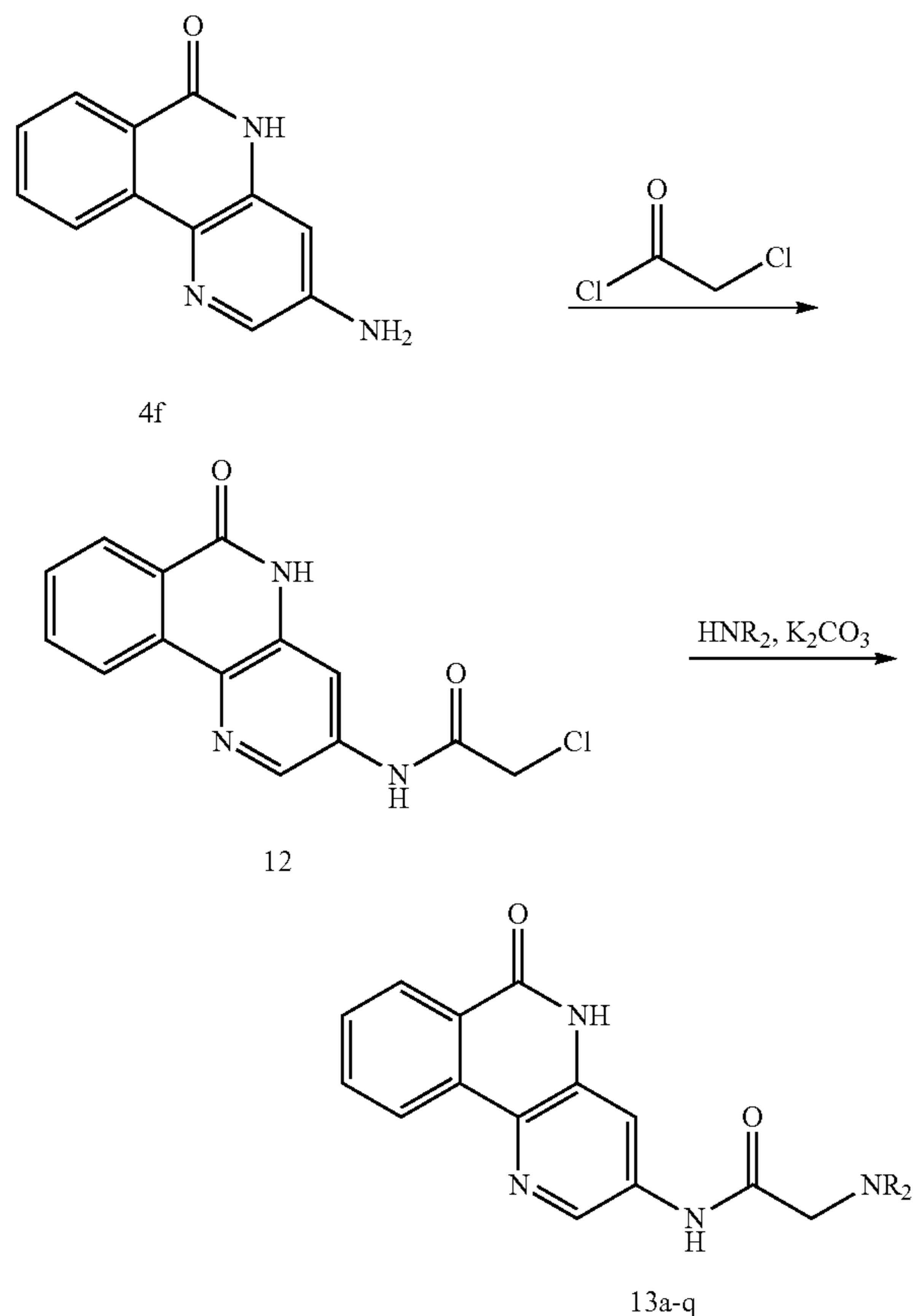
Scheme 8-5. Amide derivatives of aniline 4f.
