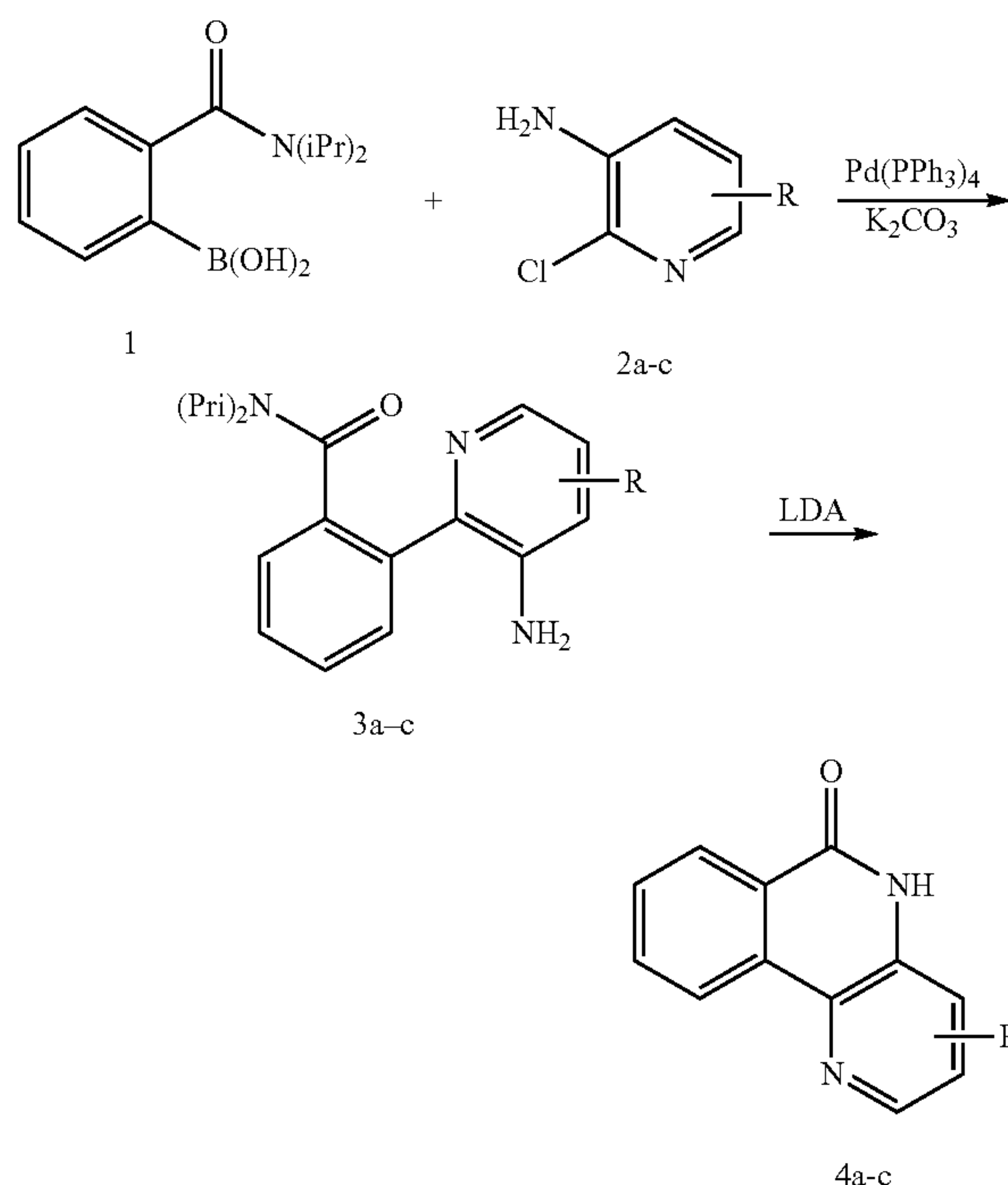
Scheme 1-5. General Scheme for synthesis of azaphenanthridones 4a-c.
