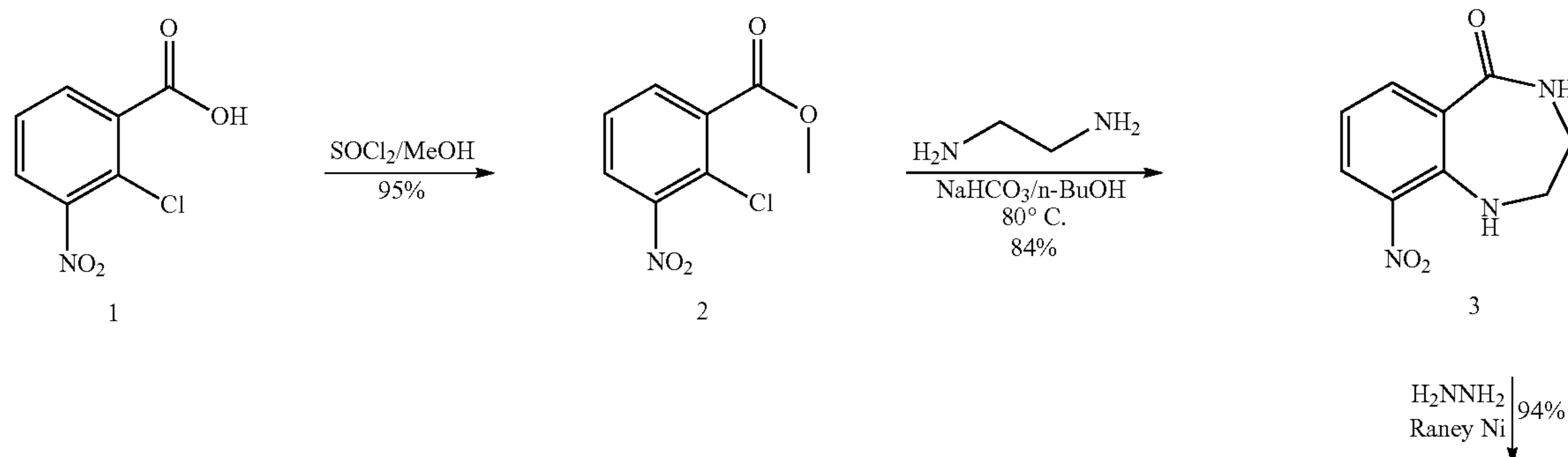
Scheme 2-4. General Synthesis of aminobenzodiazepine derivatives 5a-v.
