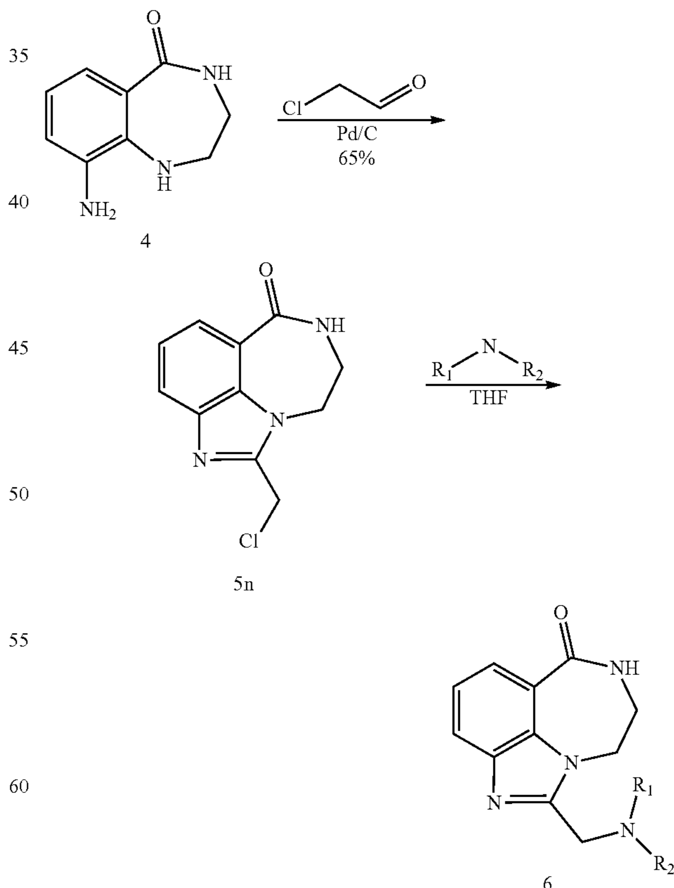
Scheme 3-4 Synthesis of imidazobenzodiazepine amines 6a-dd.
