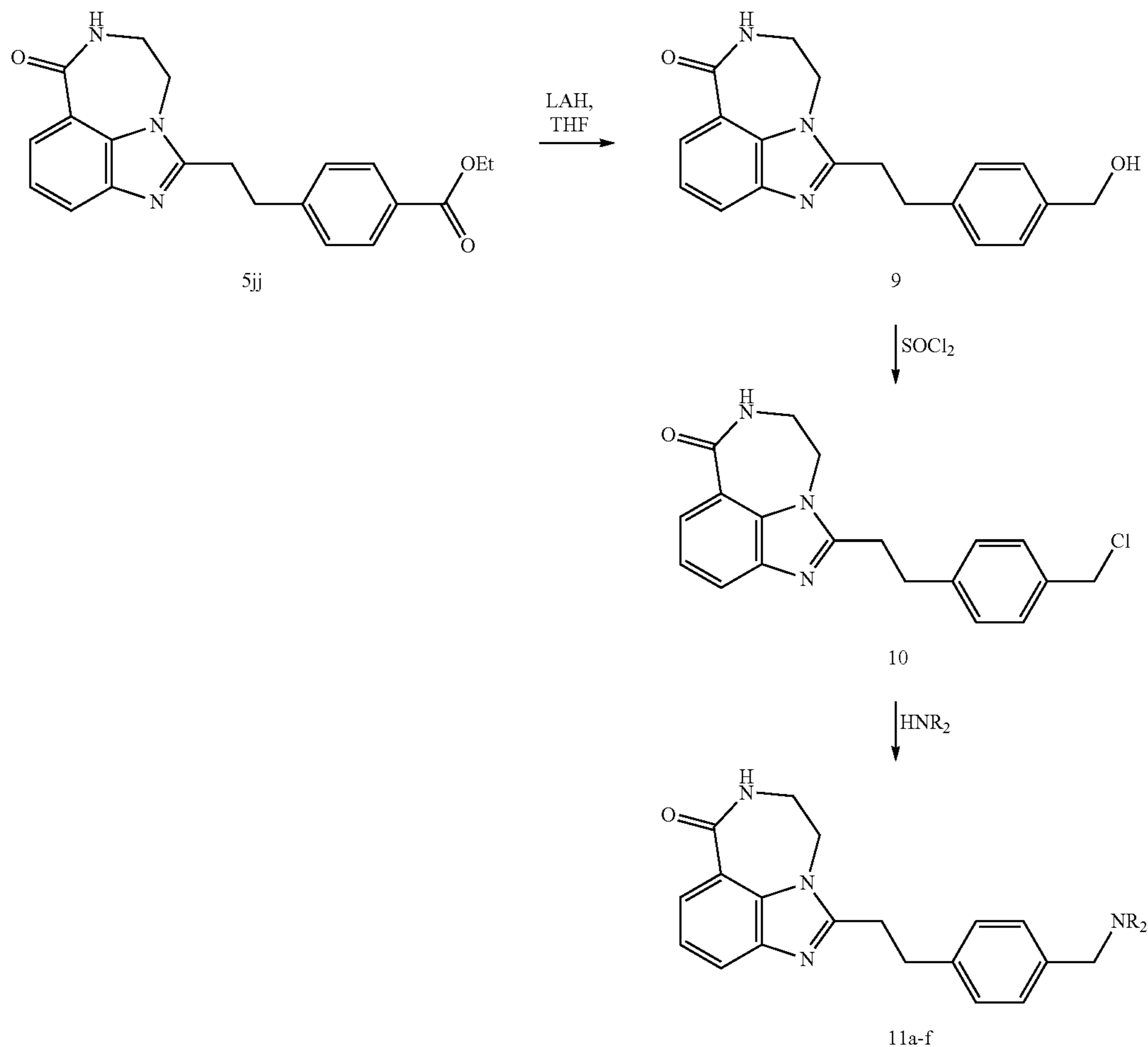
Scheme 6-4. Synthesis of amines 11a-f.
