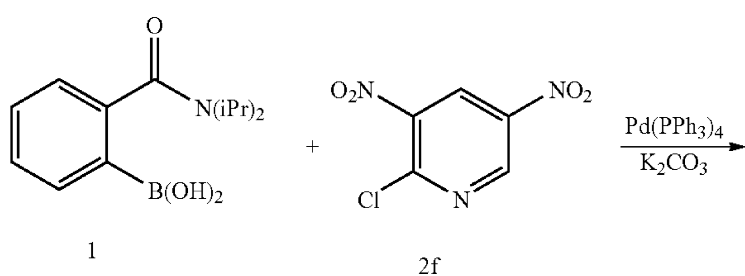
Scheme 2-5. Synthesis of Aminoazaphenanthridone 4f.
