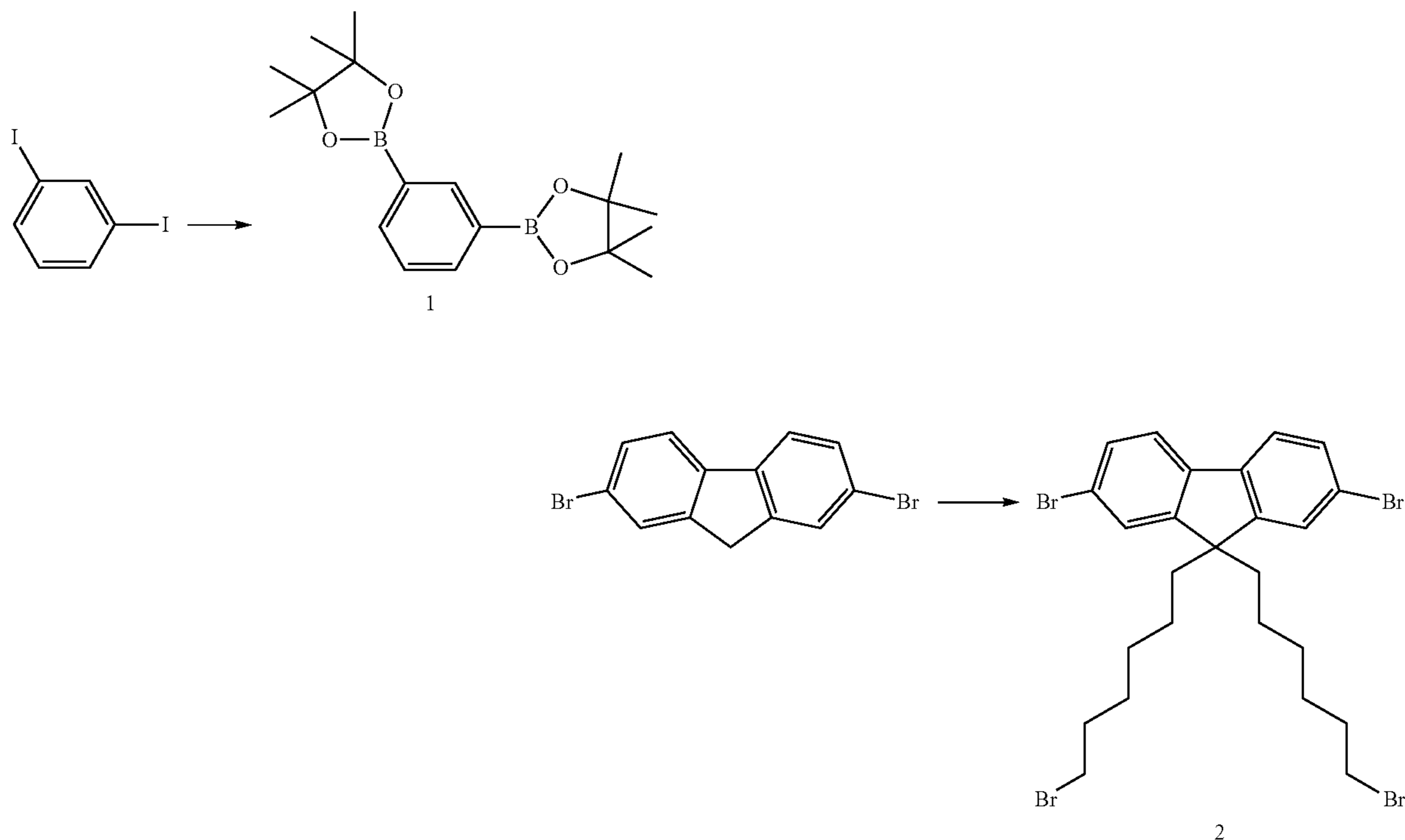
Scheme 1. Synthetic procedure for cationic water-soluble polymers.
