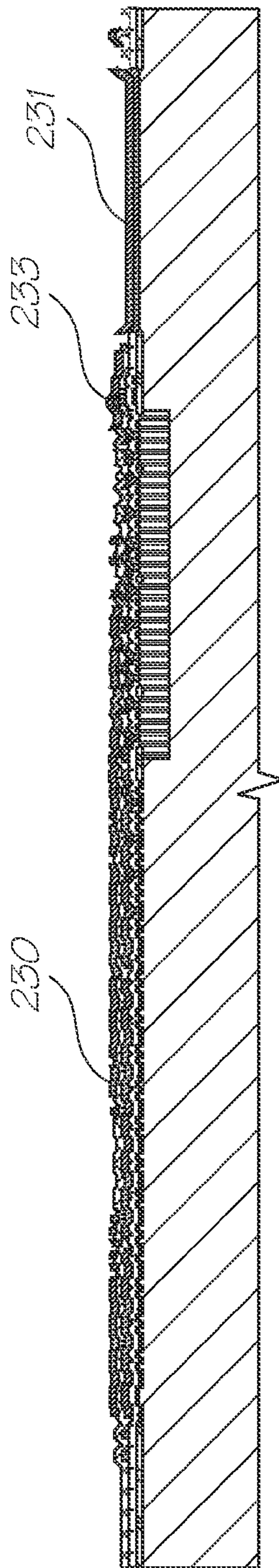
Deposit metal 2
