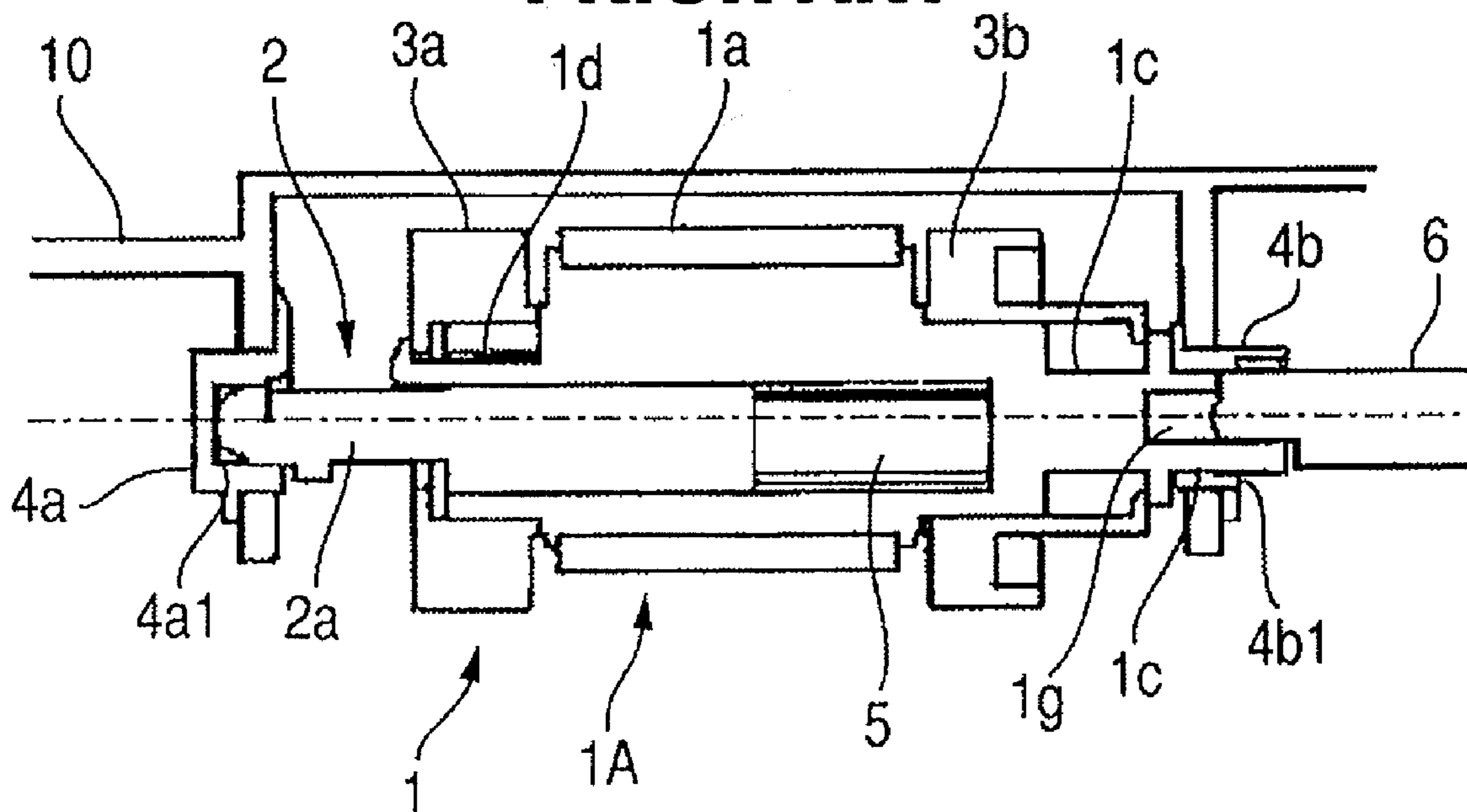
FIG. 15B PRIOR ART
