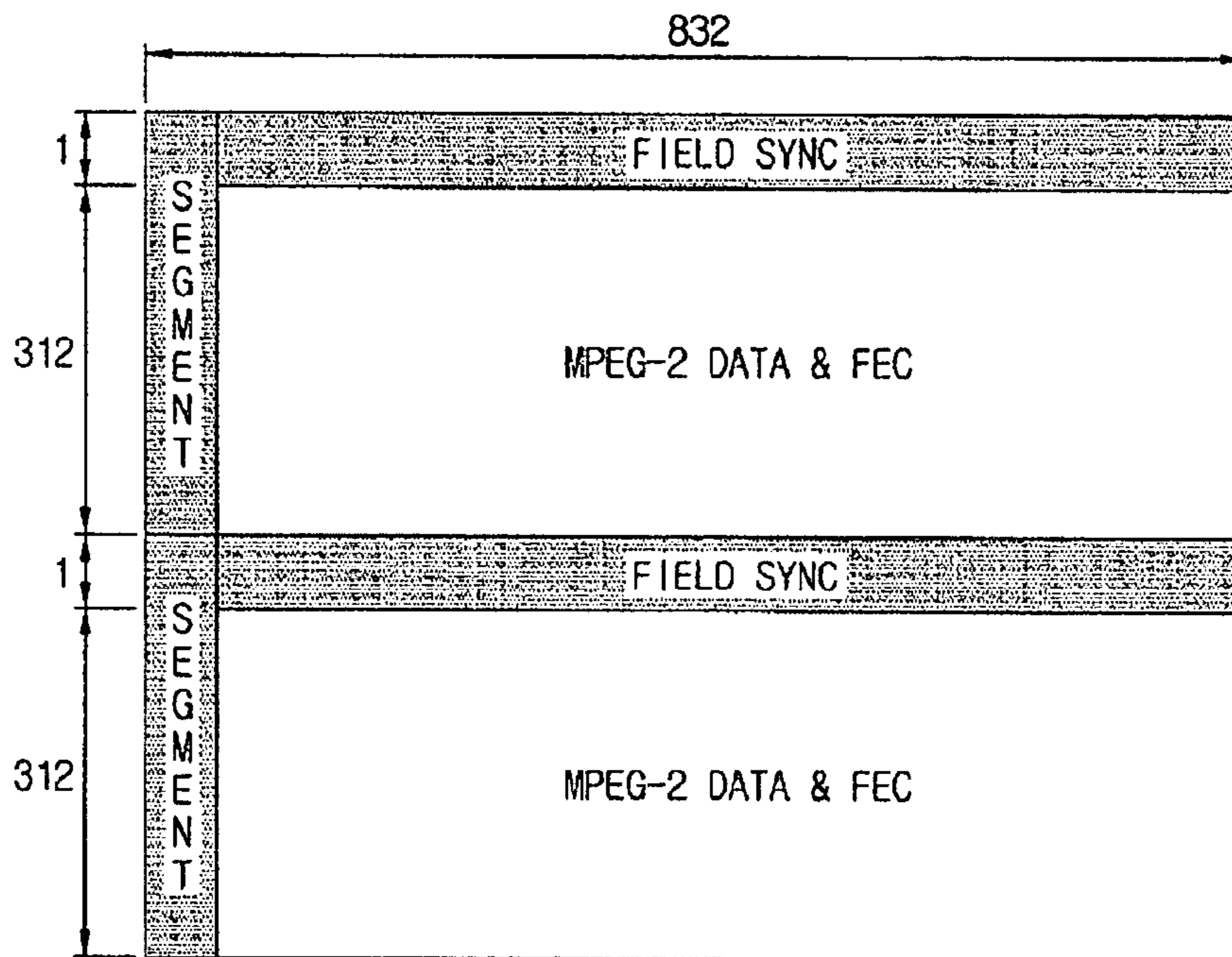
FIG. 2 (RELATED ART)
