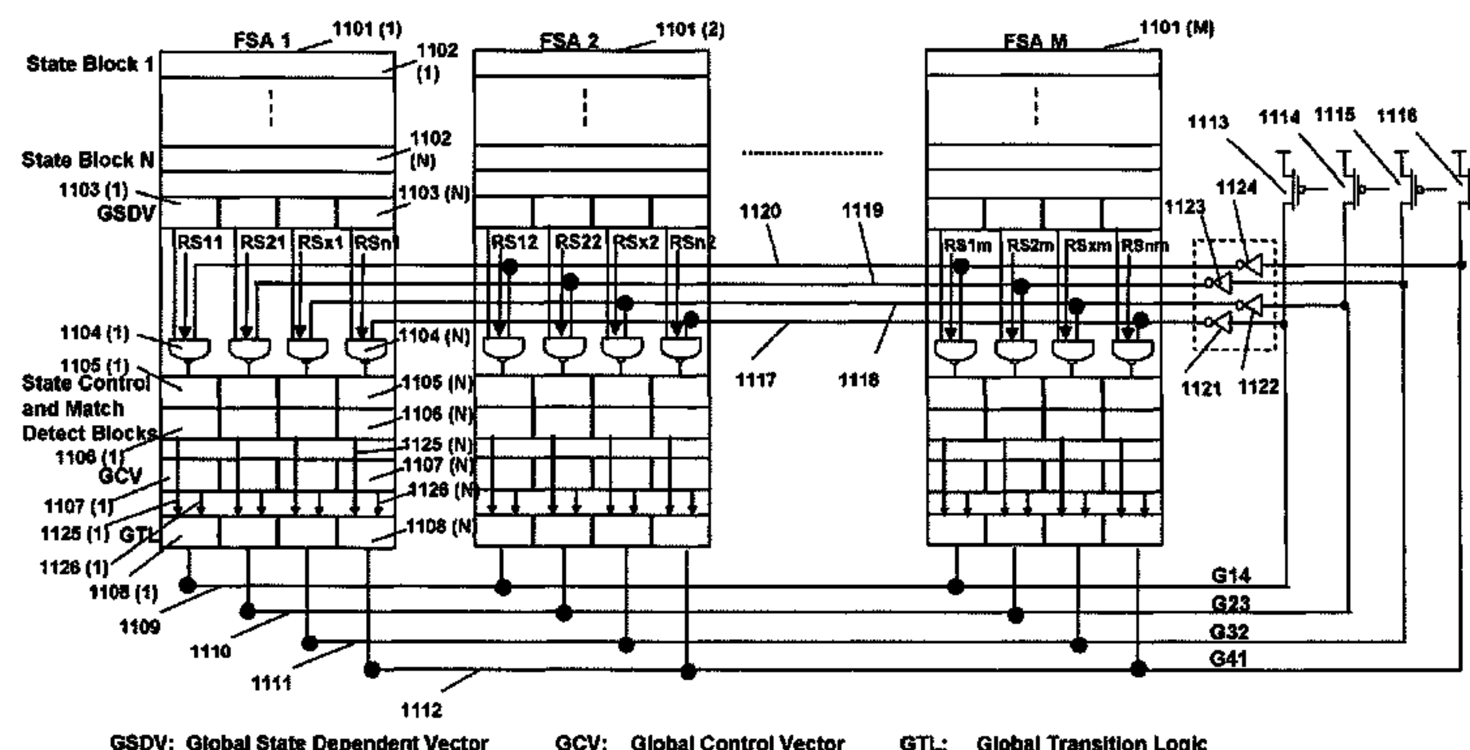
PRISM Row-Wise FSA Extension
