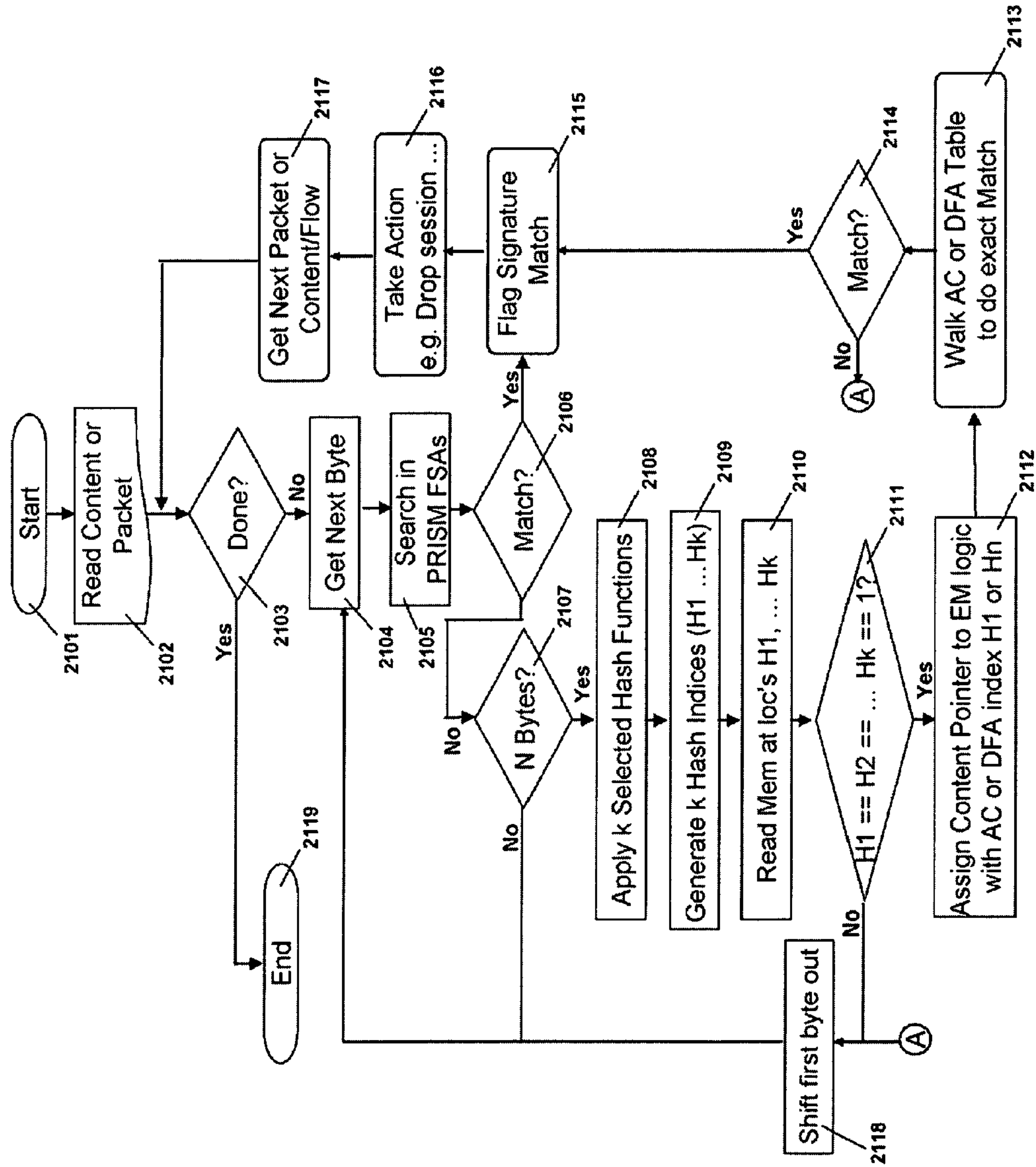
Fig. 21 PRISM Signature Search Flow
