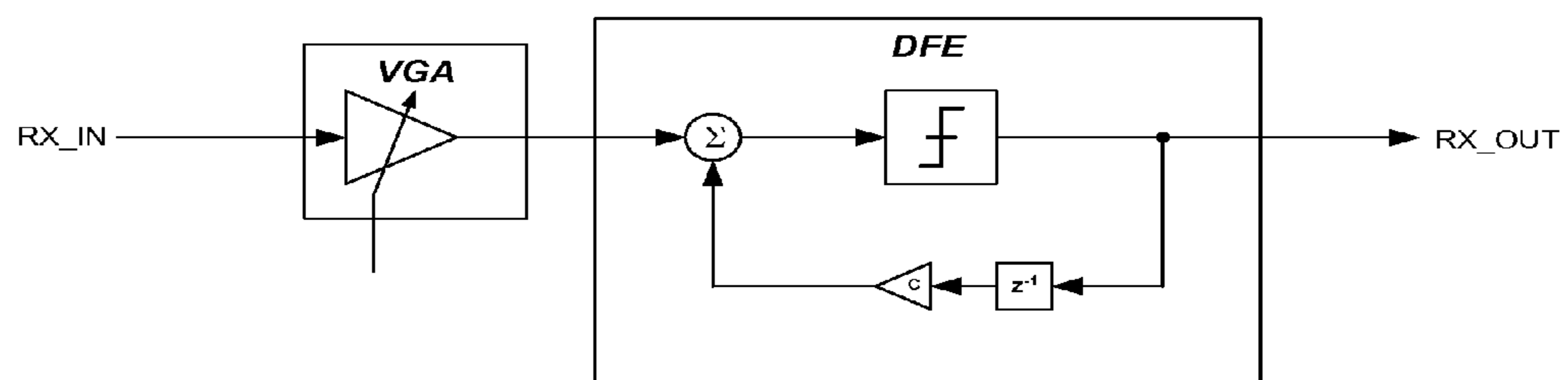
Figure 6 PRIOR ART
