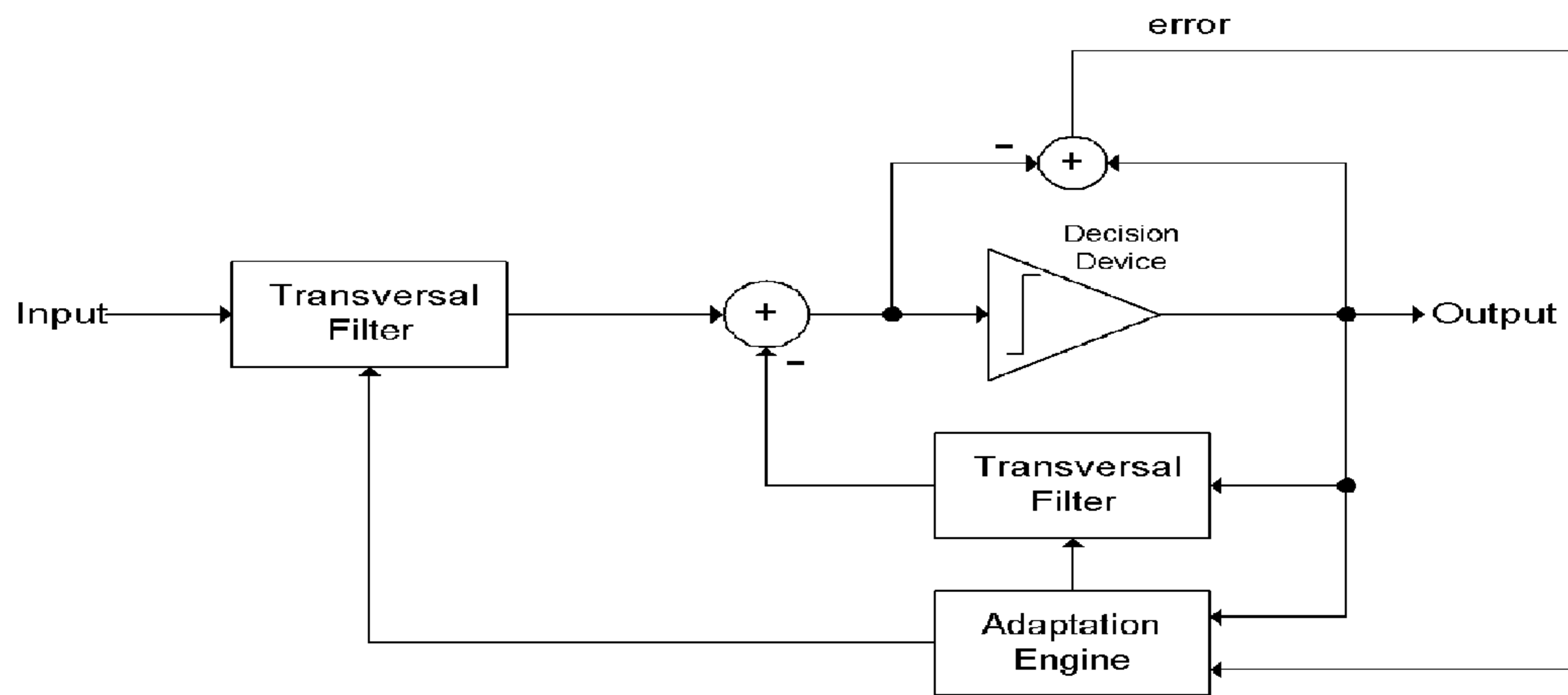
Figure 4 PRIOR ART
