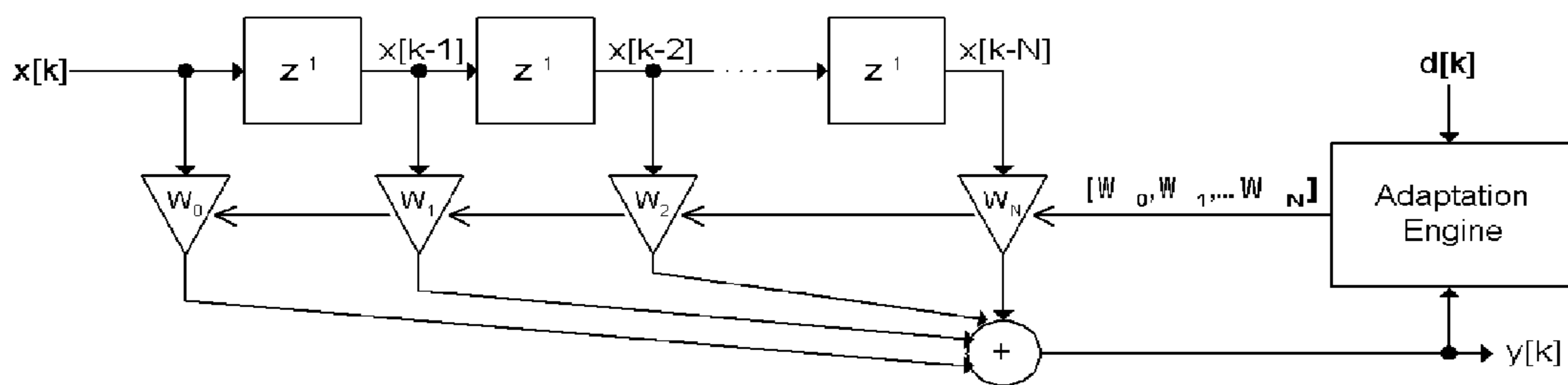
Figure 2 PRIOR ART
